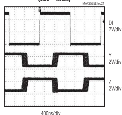
DRIVER PROPAGATION DELAY ( \overline{SLO} = HIGH )
