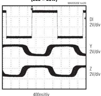
DRIVER PROPAGATION DELAY ( \overline{SLO} = LOW )
