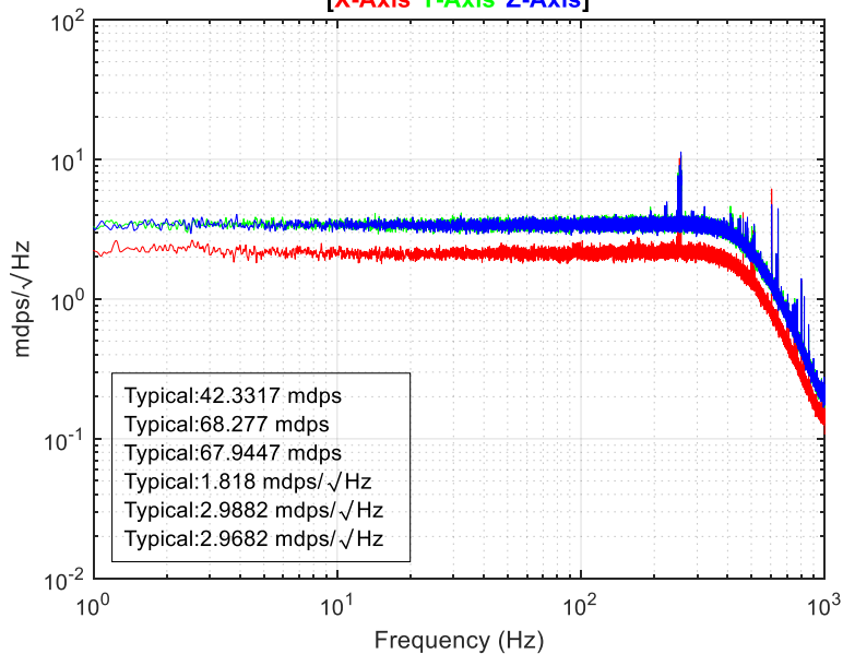
ADIS1646x-2 Power Spectral Density Typical (20 DUTs)
