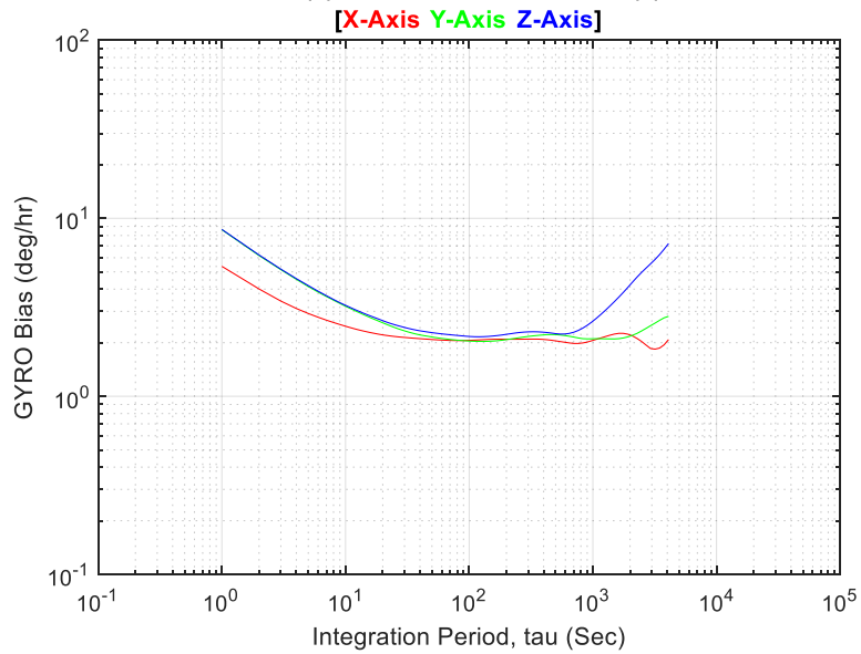
ADIS1646x-3 Allan Deviation of (14 DUTs) Initial (4) Hrs Excluded from total (7) Hrs
