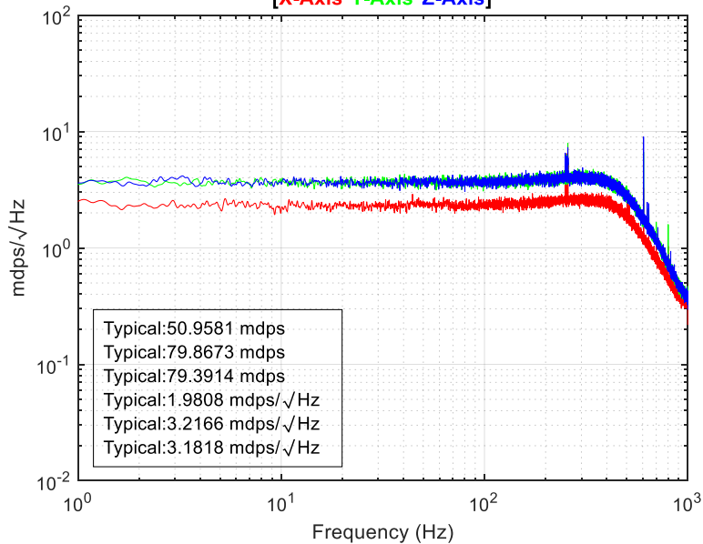
ADIS1646x-3 Power Spectral Density Typical (17 DUTs)
