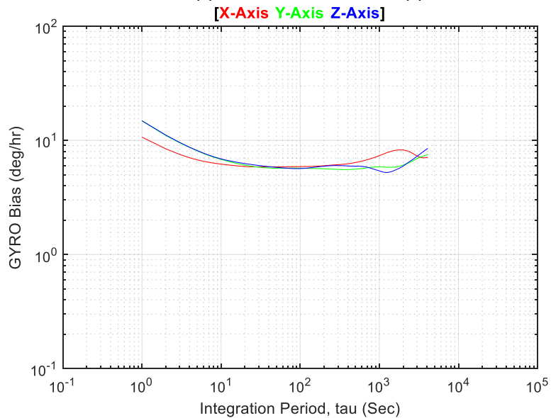
ADIS1646x-3 Allan Deviation of (14 DUTs) Initial (4) Hrs Excluded from total (7) Hrs
