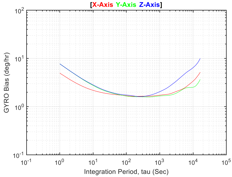
ADIS1646x-2 Allan Deviation of (11 DUTs) Initial (4) Hrs Excluded from total (7) Hrs
