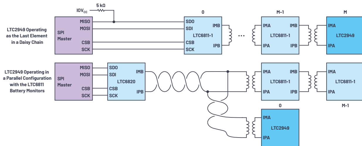
Figure 3. LTC2949 isoSPI configurations.
