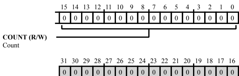
Figure 42-3: \text{SWU\_CNT}[n] Register Diagram
