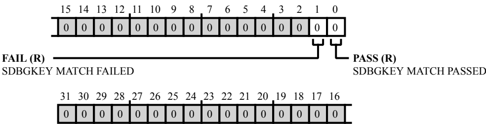
Figure 44-45: TAPC_SDBGKEY_STAT Register Diagram
