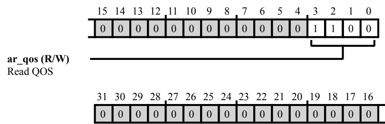
Figure 41-86: SCB0_SPI0RX_READ_QOS Register Diagram
