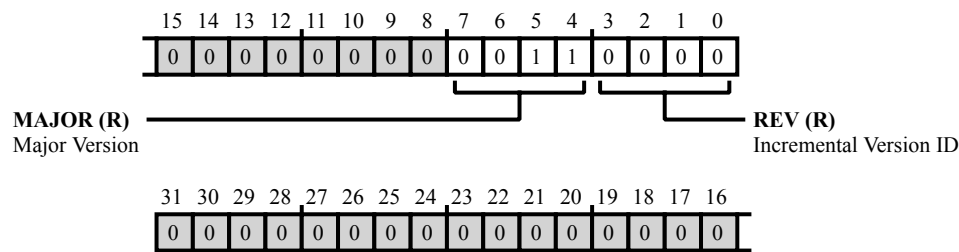
Figure 2-11: CGU_REVID Register Diagram
