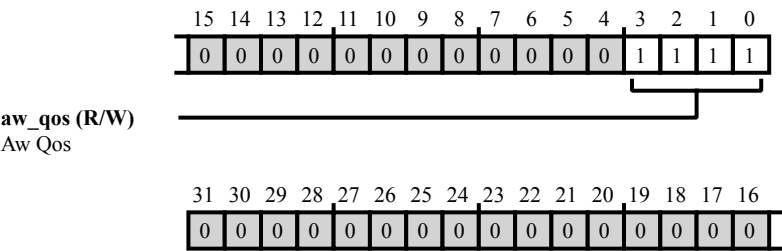
Figure 41-145: SCB4_SHARC_DPORT_WRITE_QOS Register Diagram
