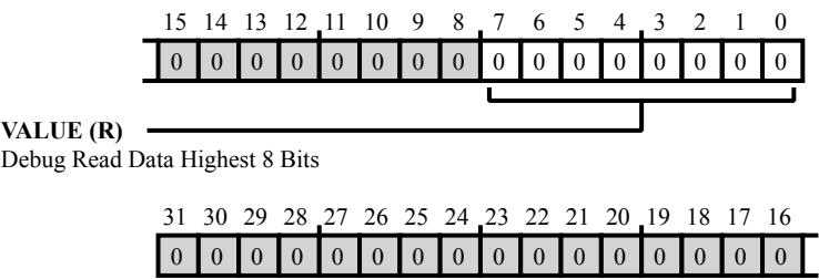
Figure 39-16: IIR_DBG_RDDAT_HI Register Diagram
