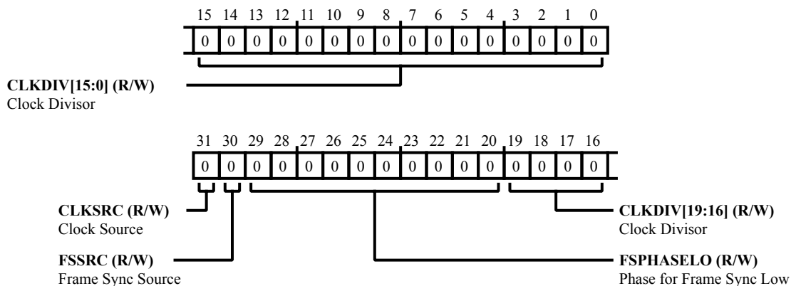
Figure 24-8: PCG_CTLA1 Register Diagram
