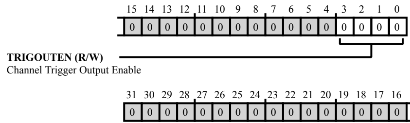
Figure 44-71: CTI_CTIOUTEN0 Register Diagram
