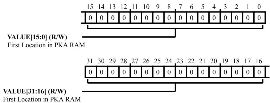
Figure 34-11: PKA_RAM Register Diagram
