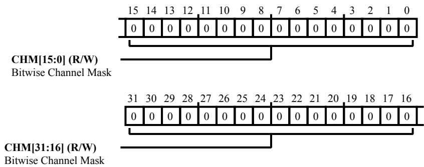
Figure 20-7: MLB_ACMR0 Register Diagram
