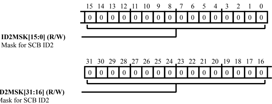
Figure 9-24: DMC_PRIOMSK2 Register Diagram
