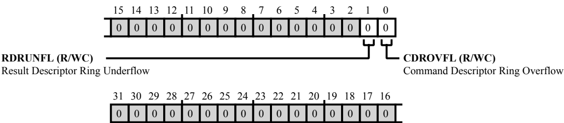
Figure 33-38: PKTE_RING_STAT Register Diagram
