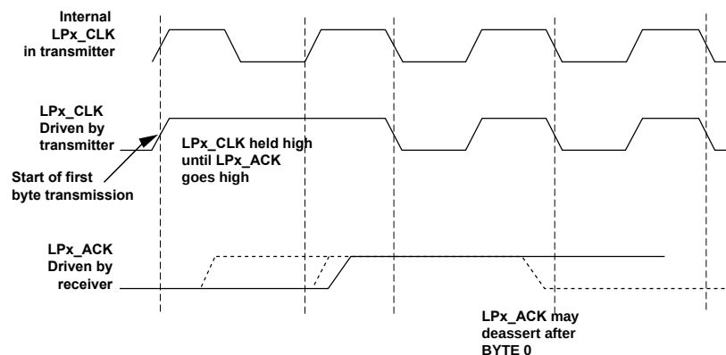
Figure 14-6: Relationship Between Internal Link Port Clock and Link Port Clock at the Pins
