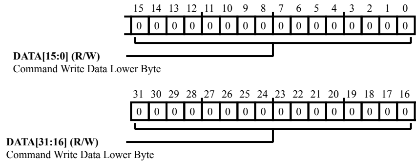
Figure 16-12: OSPI_FCWD_LWR Register Diagram
