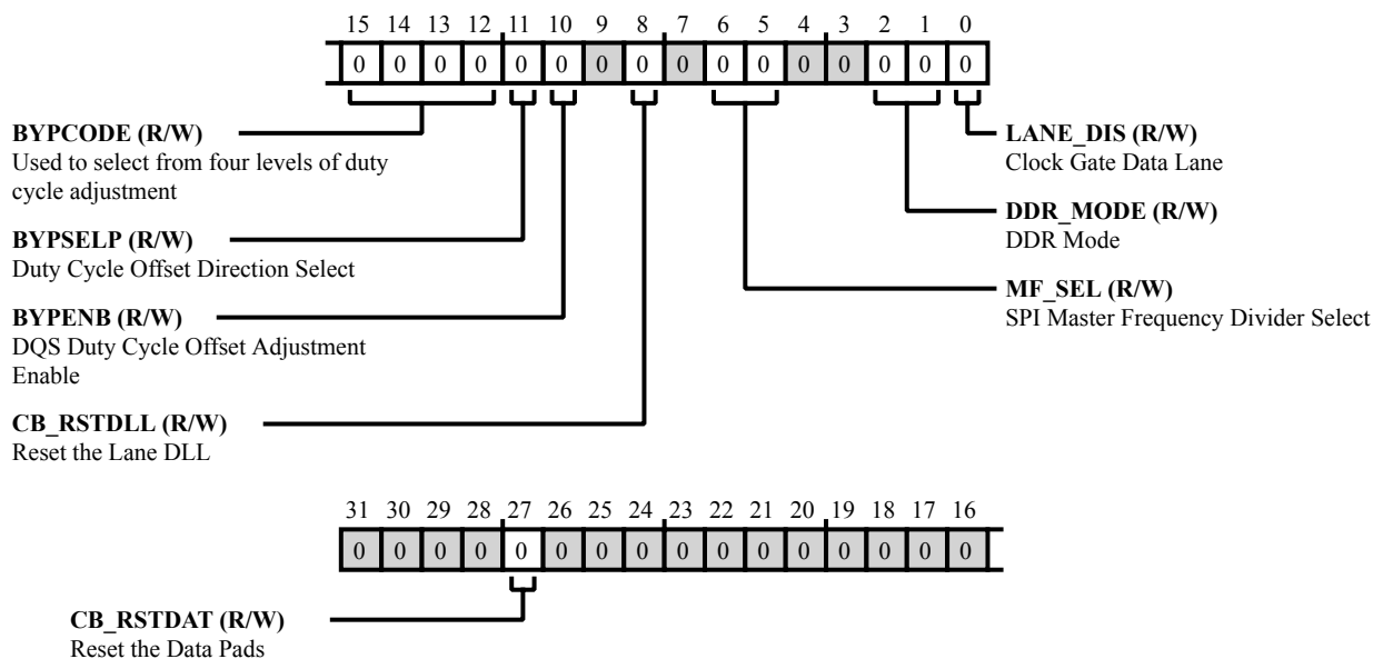
Figure 9-39: DMC_DDR_LANE0_CTL0 Register Diagram
