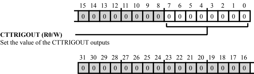
Figure 44-90: CTI_ITTRIGOUT Register Diagram
