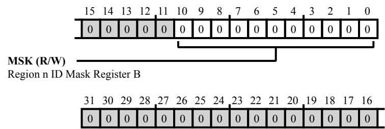
Figure 11-13: SMPU_RIDMSKB[n] Register Diagram
