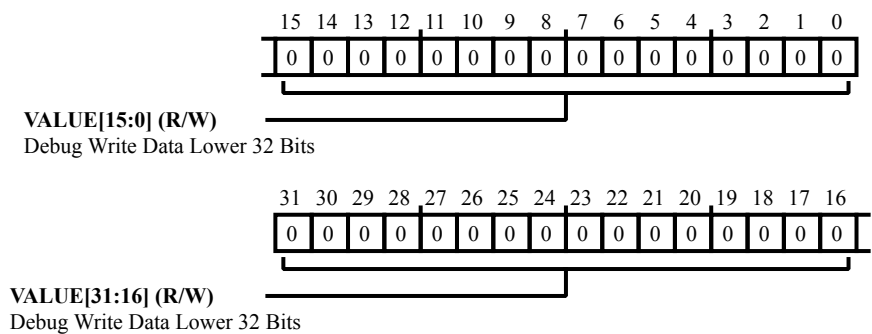
Figure 39-19: IIR_DBG_WRDAT_LO Register Diagram
