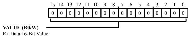
Figure 21-23: TWI_RXDATA16 Register Diagram
