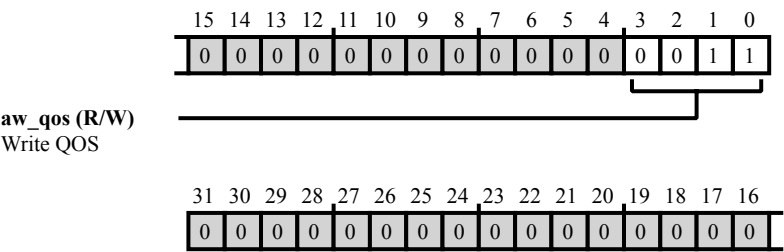
Figure 41-33: SCB0_ETR_WRITE_QOS Register Diagram
