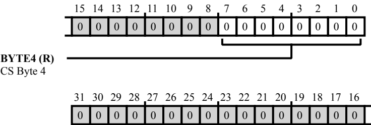
Figure 26-13: SPDIF_RX_STAT1_B Register Diagram
