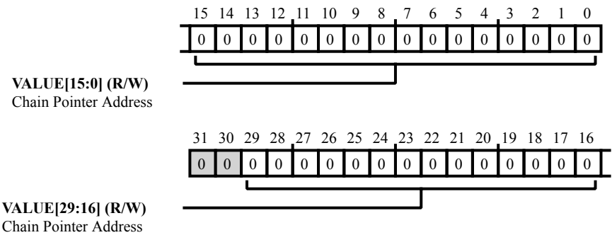
Figure 38-8: FIR_CHNPTR Register Diagram
