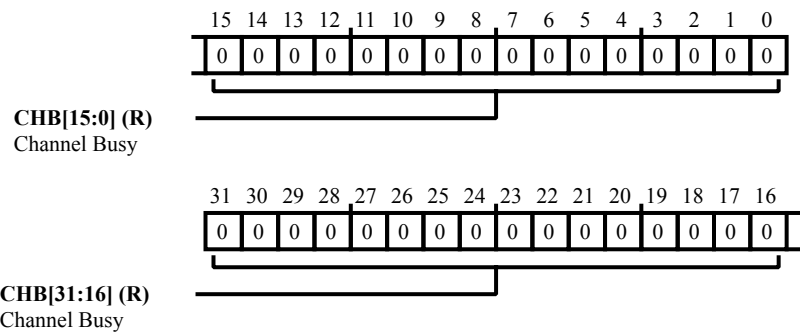
Figure 20-15: MLB_HCBR0 Register Diagram
