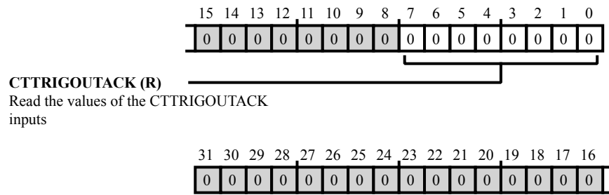
Figure 44-91: CTI_ITTRIGOUTACK Register Diagram
