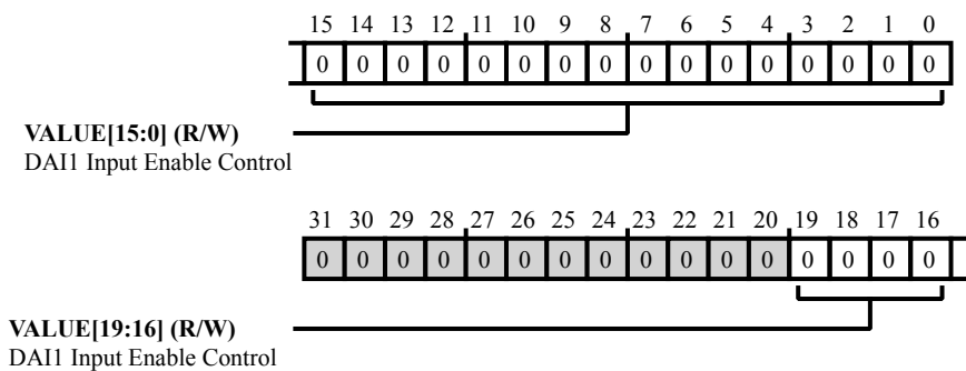
Figure 12-41: PADS_DAI1_IE Register Diagram
