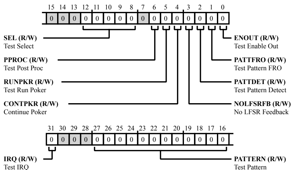
Figure 36-23: TRNG_TEST Register Diagram
