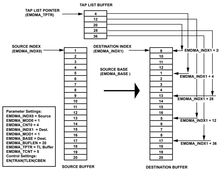
Figure 28-6: Circular Buffering Scatter DMA (Writes)
