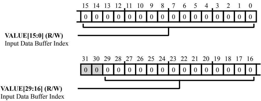
Figure 39-22: IIR_INIDX Register Diagram
