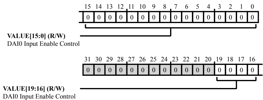
Figure 12-38: PADS_DAI0_IE Register Diagram
