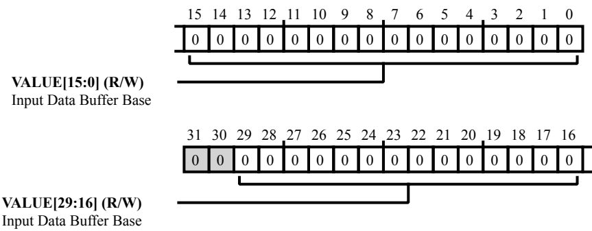
Figure 39-21: IIR_INBASE Register Diagram
