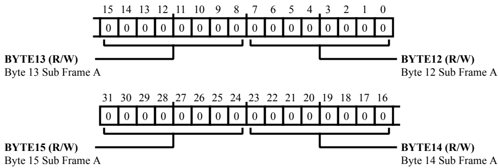
Figure 26-30: SPDIF_TX_UBUFF_A3 Register Diagram
