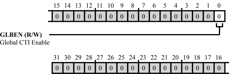
Figure 44-60: CTI_CTICONTROL Register Diagram
