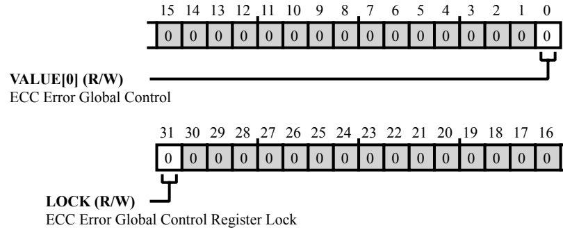
Figure 43-12: MEC_EEIRQ_GCTL[q] Register Diagram
