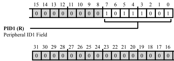
Figure 44-95: CTI_PERIPHID1 Register Diagram
