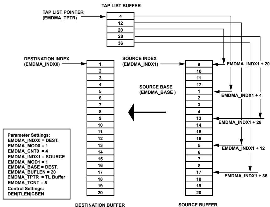
Figure 28-7: Circular Gather DMA (Reads)
