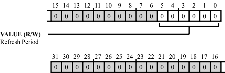
Figure 37-12: TMU_REFR_CNTR Register Diagram
