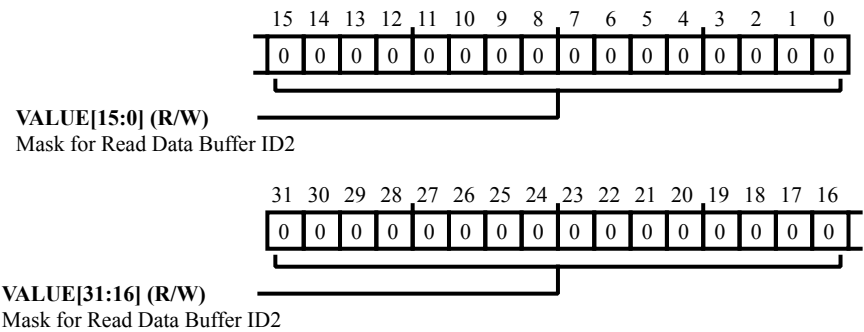
Figure 9-28: DMC_RDDATABUFMSK2 Register Diagram
