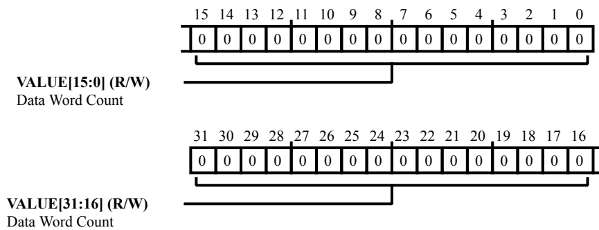
Figure 29-5: CRC_DCNT Register Diagram
