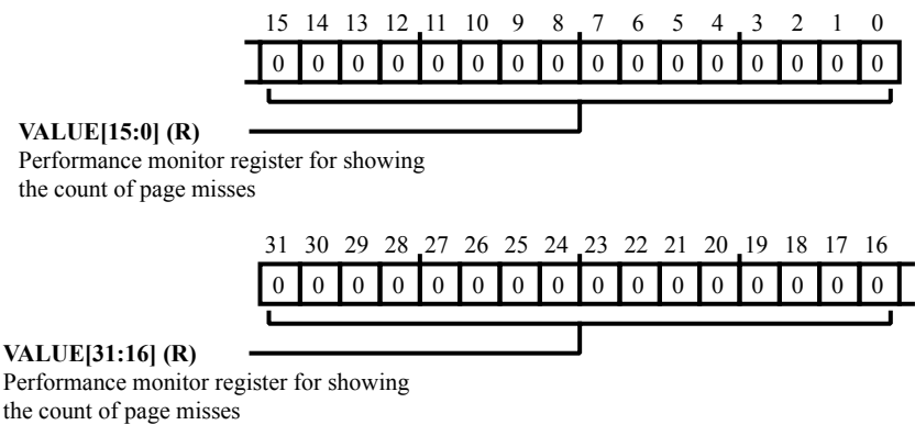
Figure 9-17: DMC_PM_PGMS_CNT Register Diagram
