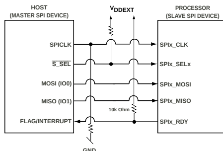
Figure 40-5: Connection between Host (SPI Master) and Processor (SPI Slave) DIOM
