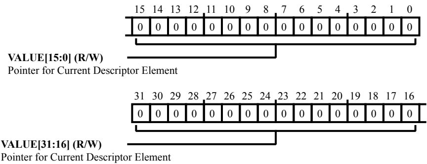
Figure 27-12: DMA_DSCPTR_CUR Register Diagram
