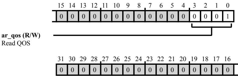
Figure 41-30: SCB0_DLDMA1_CH1_READ_QOS Register Diagram
