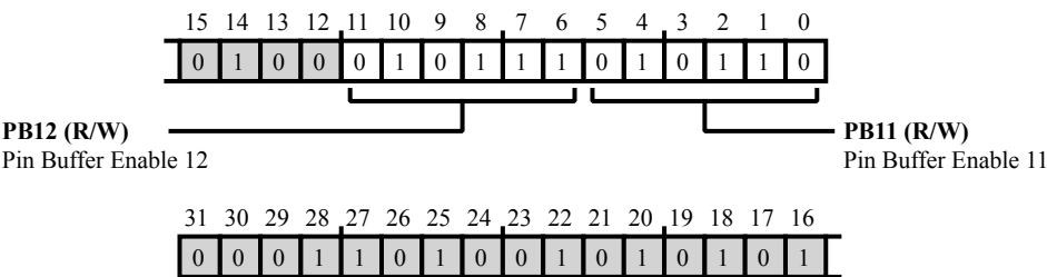
Figure 22-47: DAI_PBEN2 Register Diagram
