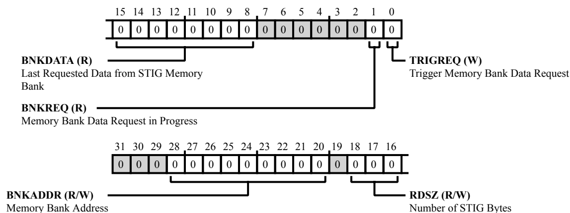
Figure 16-9: OSPI_FCMCTL Register Diagram
