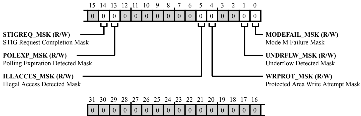
Figure 16-14: OSPI_IMSK Register Diagram
