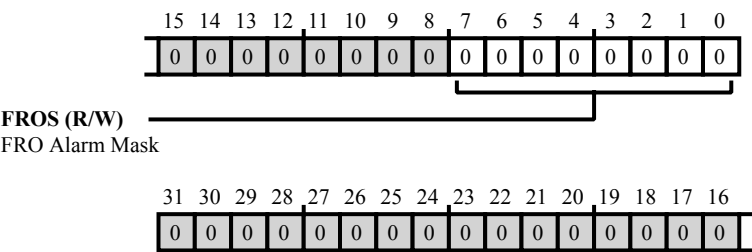
Figure 36-3: TRNG_ALMMSK Register Diagram
