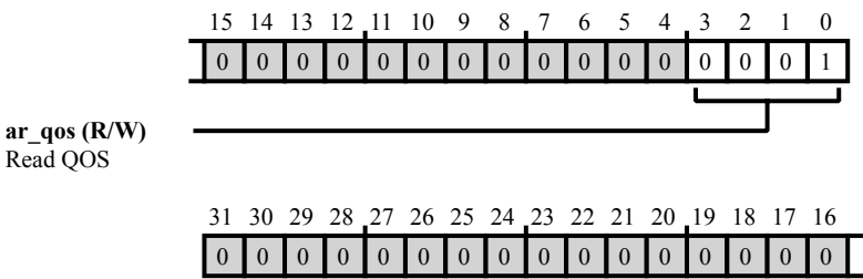
Figure 41-14: SCB0_CRC0_CH1_READ_QOS Register Diagram
