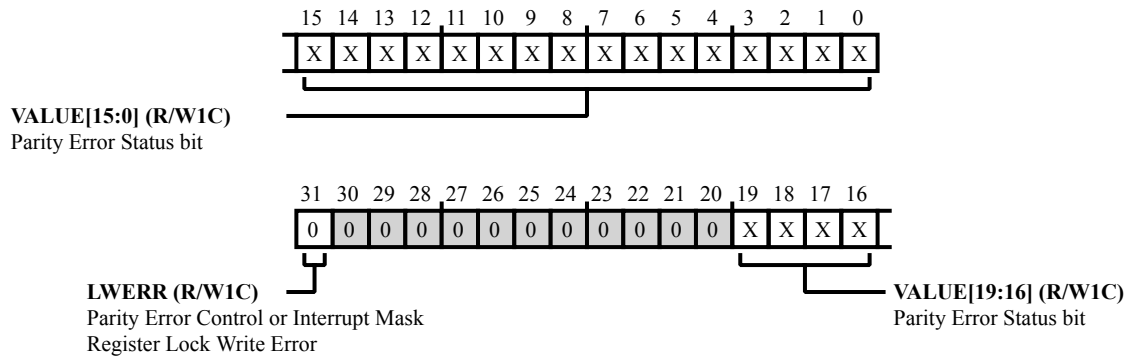
Figure 43-18: MEC_PERR_STAT Register Diagram
