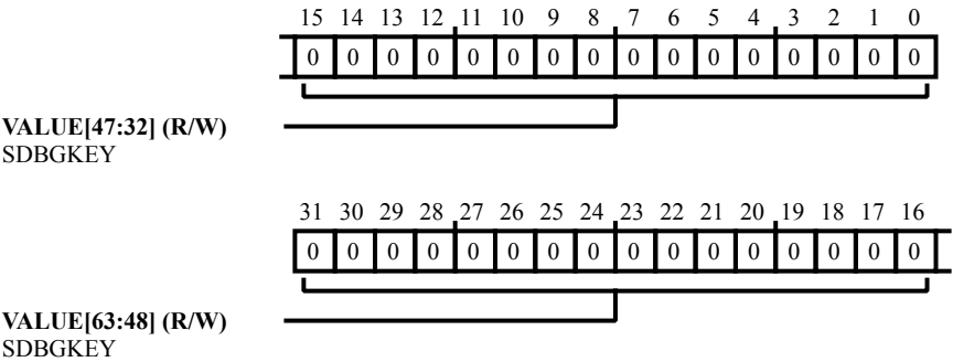
Figure 44-41: TAPC_SDBGKEY1 Register Diagram
