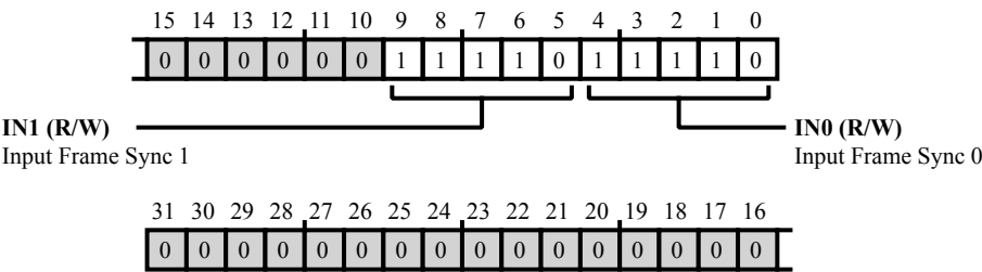
Figure 22-33: DAI_FS4 Register Diagram
