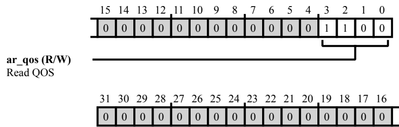
Figure 41-56: SCB0_SP0B_READ_QOS Register Diagram
