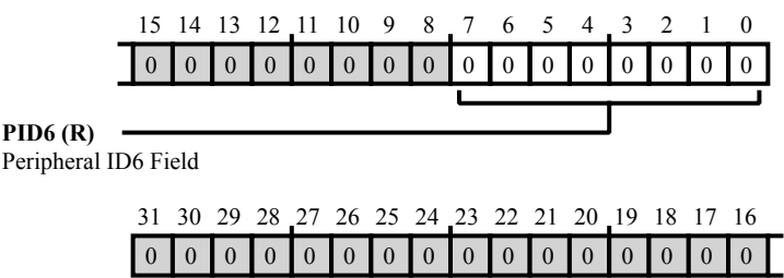
Figure 44-100: CTI_PERIPHID6 Register Diagram
