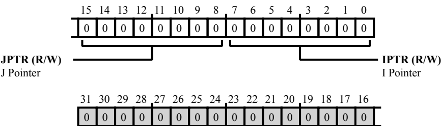
Figure 33-41: PKTE_SA_ARC4IJPTR Register Diagram
