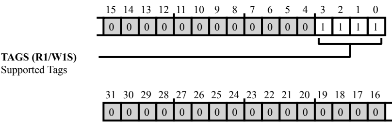
Figure 44-15: CSPFT_CLAIMSET Register Diagram
