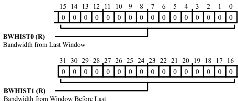
Figure 42-8: SWU_HIST[n] Register Diagram
