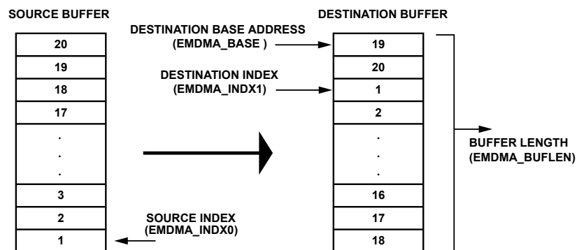
Figure 28-1: Circular Buffering Write DMA
