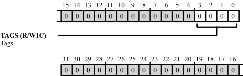
Figure 44-14: CSPFT_CLAIMCLR Register Diagram
