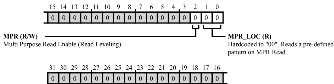
Figure 9-8: DMC_EMR3 Register Diagram
