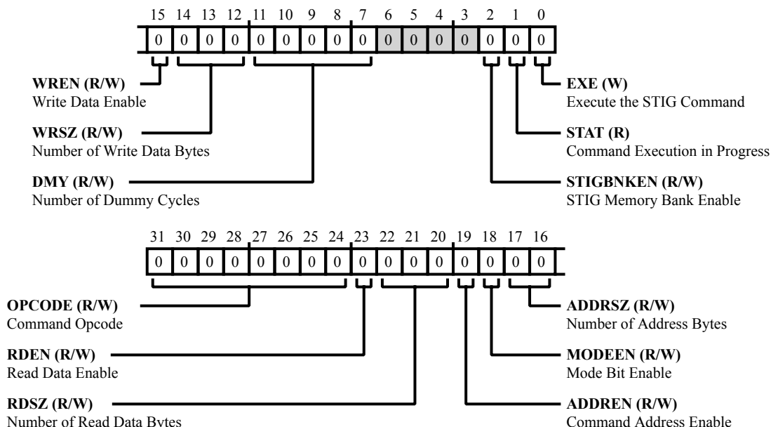
Figure 16-8: OSPI_FCCTL Register Diagram
