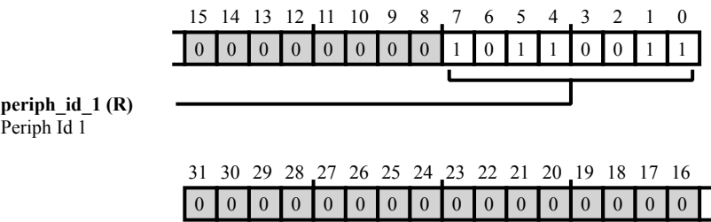
Figure 41-136: SCB4_PERIPH_ID_1 Register Diagram
