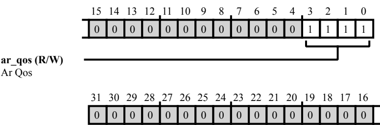
Figure 41-144: SCB4_SHARC_DPORT_READ_QOS Register Diagram
