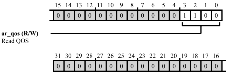
Figure 41-94: SCB0_SPI2RX_READ_QOS Register Diagram
