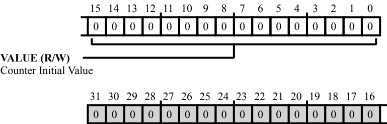
Figure 44-18: CSPFT_CNTRLDVR[n] Register Diagram
