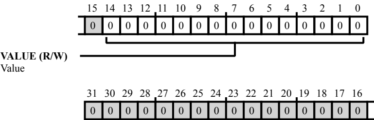
Figure 37-11: TMU_OFFSET Register Diagram
