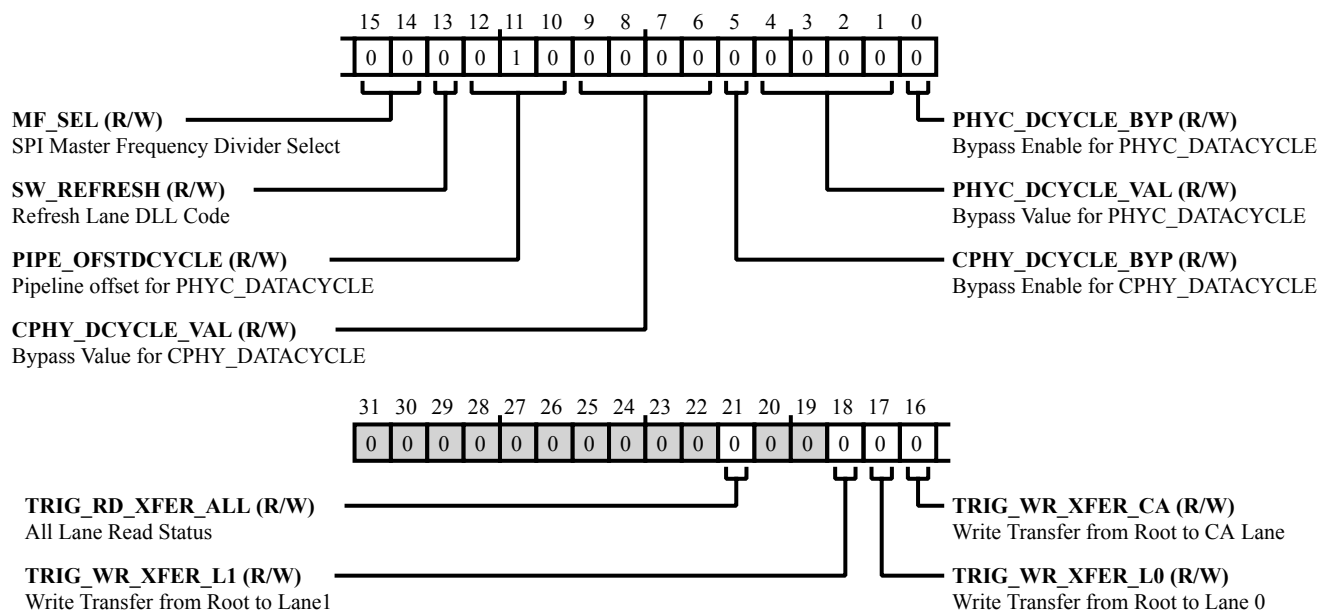
Figure 9-43: DMC_DDR_ROOT_CTL Register Diagram
