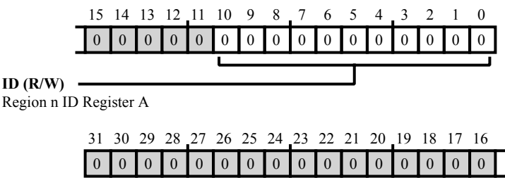
Figure 11-10: SMPU_RIDA[n] Register Diagram
