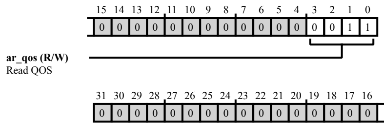
Figure 41-22: SCB0_DBG_READ_QOS Register Diagram
