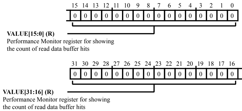
Figure 9-29: DMC_RDD_BUFHT_CNT Register Diagram
