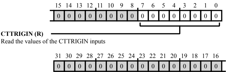
Figure 44-88: CTI_ITTRIGIN Register Diagram
