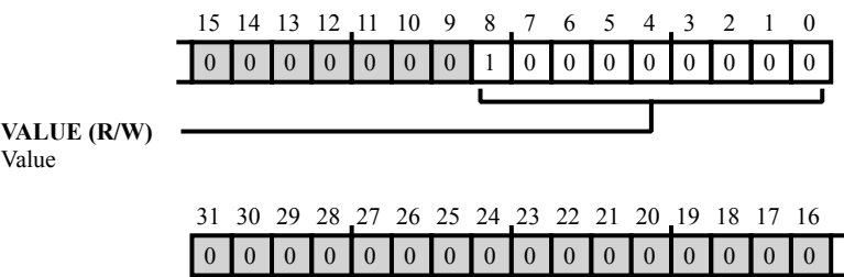
Figure 37-8: TMU_FLT_LIM_LO Register Diagram
