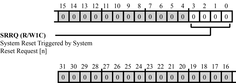
Figure 5-10: RCU_SRRQSTAT Register Diagram
