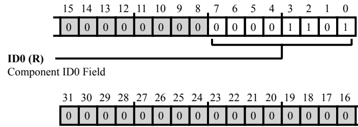
Figure 44-51: CTI_COMPID0 Register Diagram
