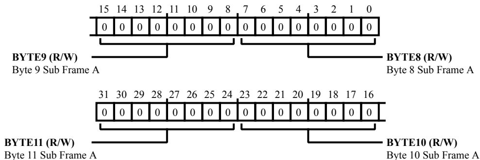
Figure 26-29: SPDIF_TX_UBUFF_A2 Register Diagram
