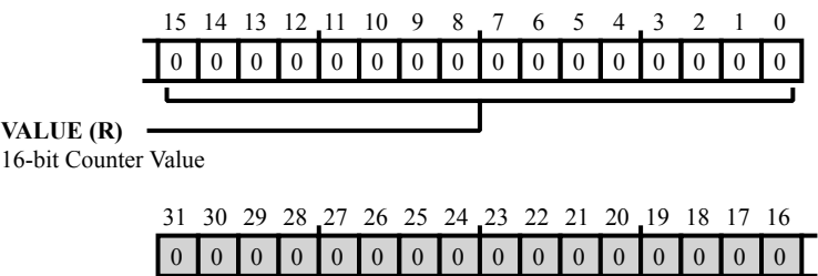
Figure 17-18: UART_RXCNT Register Diagram
