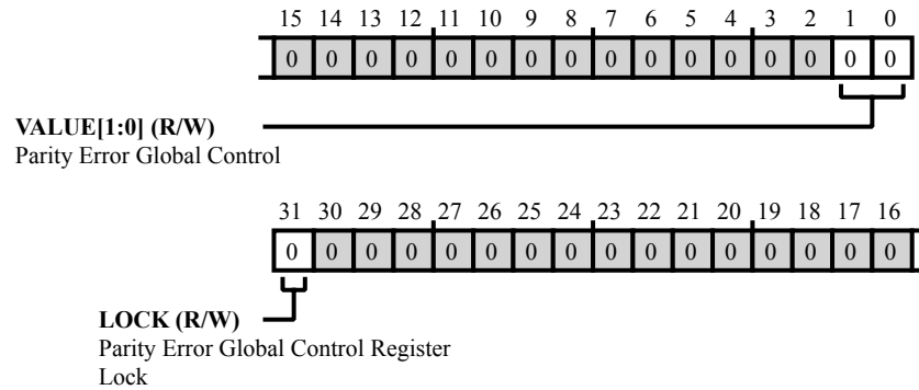
Figure 43-14: MEC_PEIRQ_GCTL[p] Register Diagram
