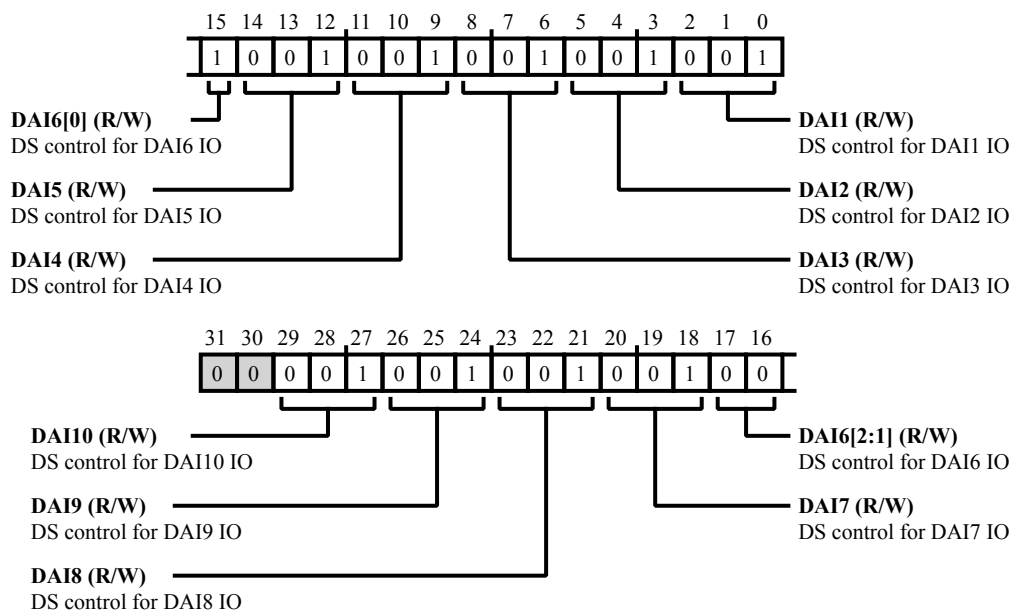
Figure 12-39: PADS_DAI1_0_DS Register Diagram
