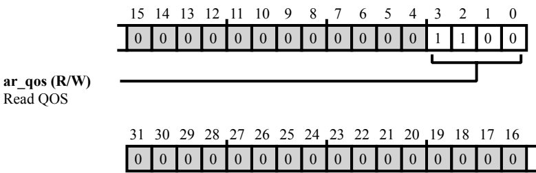
Figure 41-84: SCB0_SP7B_READ_QOS Register Diagram
