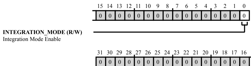
Figure 44-87: CTI_ITCTRL Register Diagram
