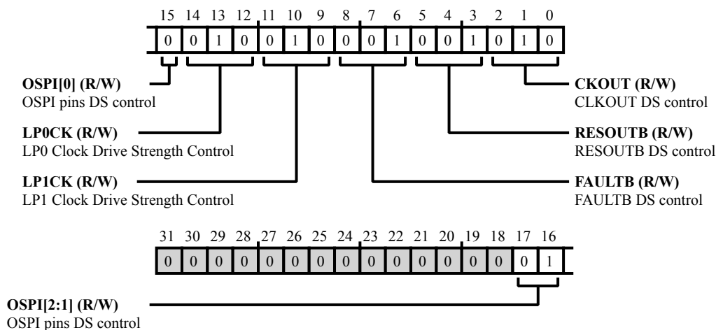
Figure 12-44: PADS_NONPORTS_DS Register Diagram
