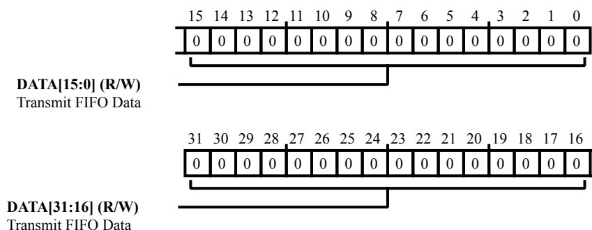
Figure 15-36: SPI_TFIFO Register Diagram
