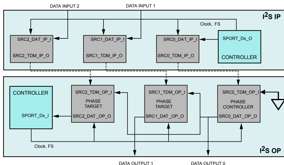
Figure 25-5: Typical Configuration for Matched-Phase Mode Operation
