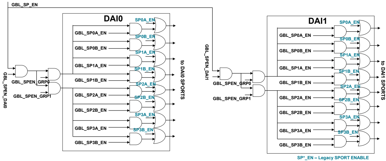
Figure 23-13: Group Enabling Options in DAI0 and DAI1
