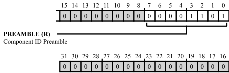
Figure 43-4: MEC_CID0 Register Diagram
