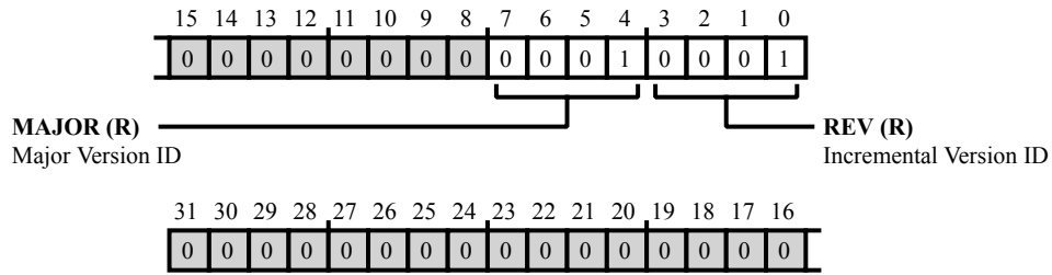
Figure 3-3: CDU_REVID Register Diagram
