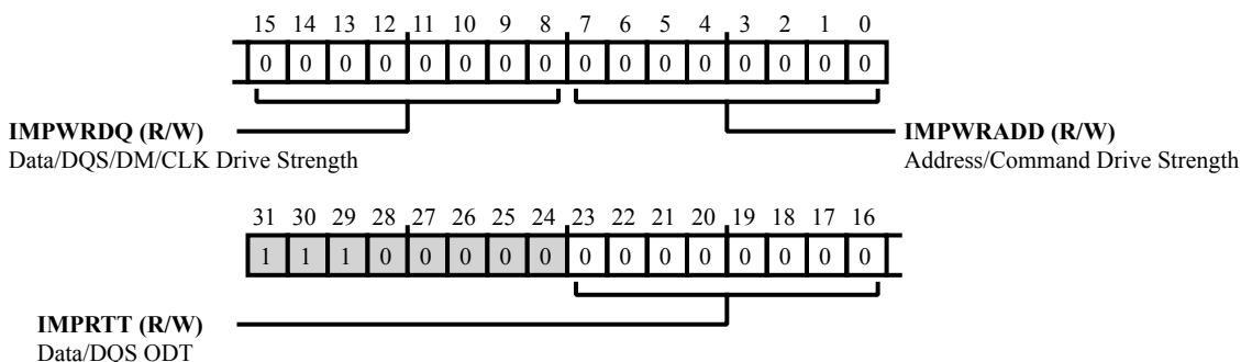
Figure 9-46: DMC_DDR_ZQ_CTL0 Register Diagram
