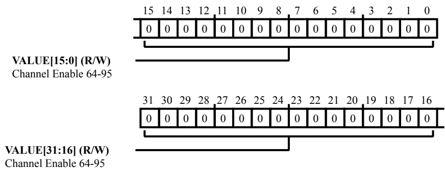
Figure 23-19: SPORT_CS2_B Register Diagram
