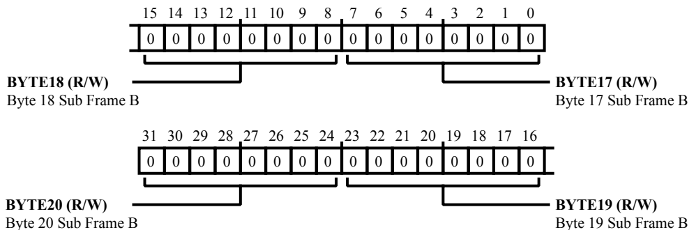
Figure 26-25: SPDIF_TX_STAT_B4 Register Diagram
