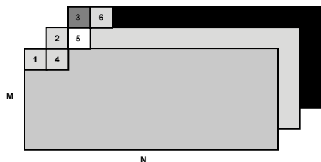
Figure 27-4: Capturing a Video Data Stream 2D DMA Example
