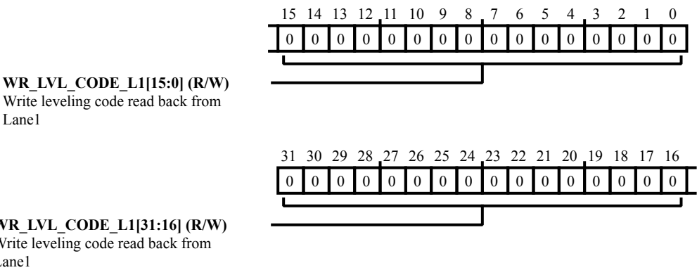
Figure 9-45: DMC_DDR_SCRATCH_5 Register Diagram
