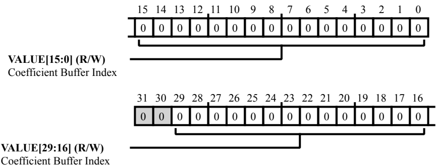
Figure 39-9: IIR_COEFIDX Register Diagram
