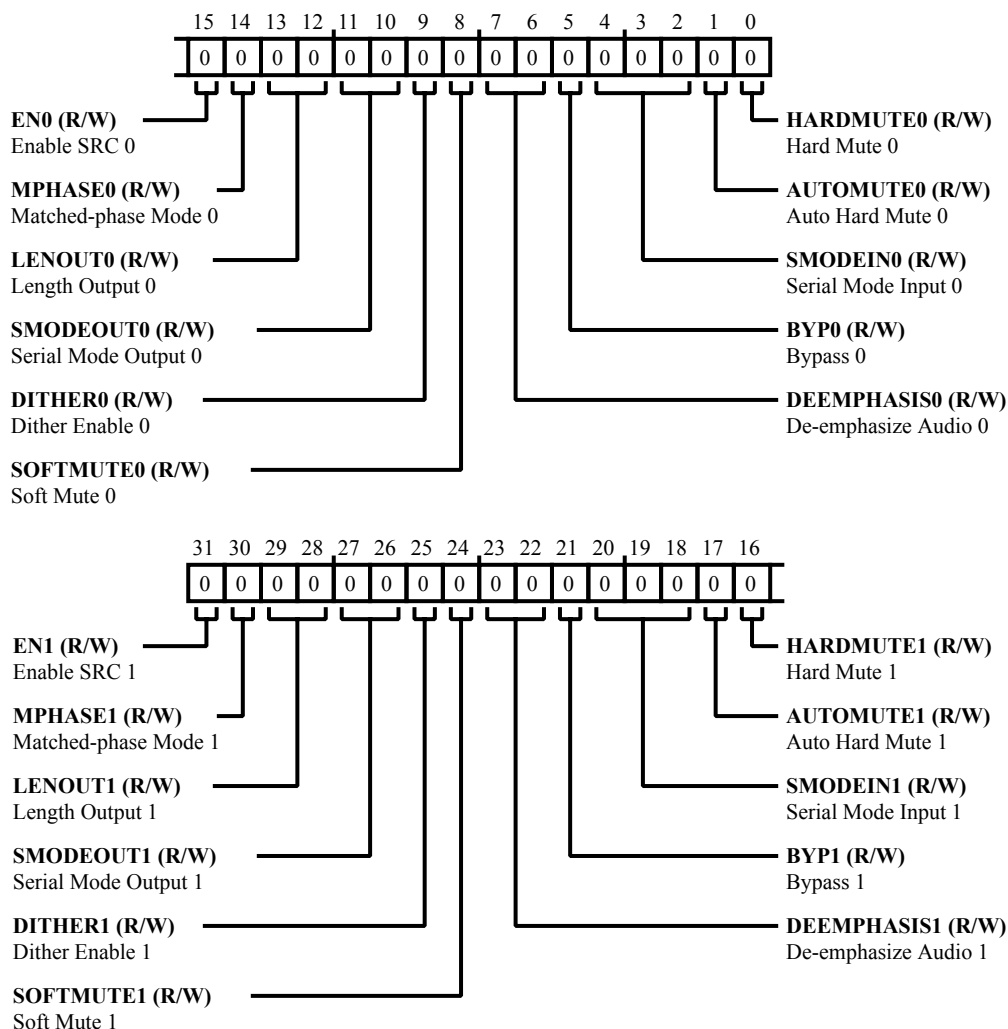
Figure 25-6: ASRC_CTL01 Register Diagram
