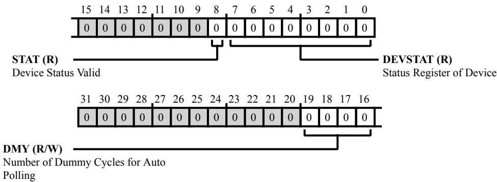
Figure 16-22: OSPI_POLSTAT Register Diagram
