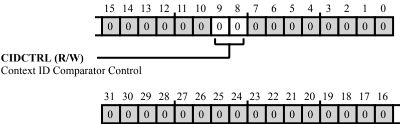
Figure 44-4: CSPFT_ACTR[n] Register Diagram
