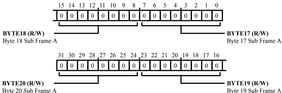
Figure 26-19: SPDIF_TX_STAT_A4 Register Diagram
