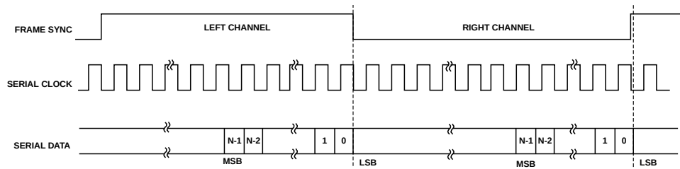
Figure 23-10: Word Select Timing in Right-Justified Mode
