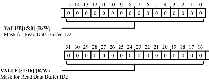
Figure 9-26: DMC_RDDATABUFID2 Register Diagram
