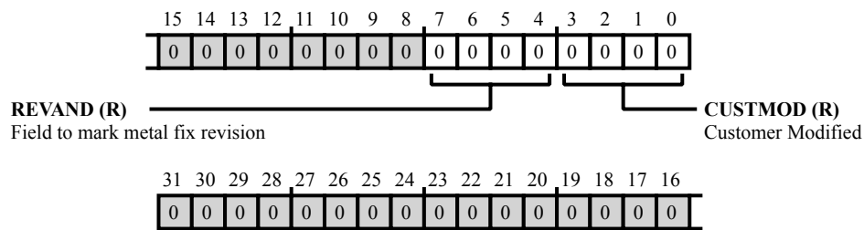
Figure 44-29: CSPFT_PID3 Register Diagram
