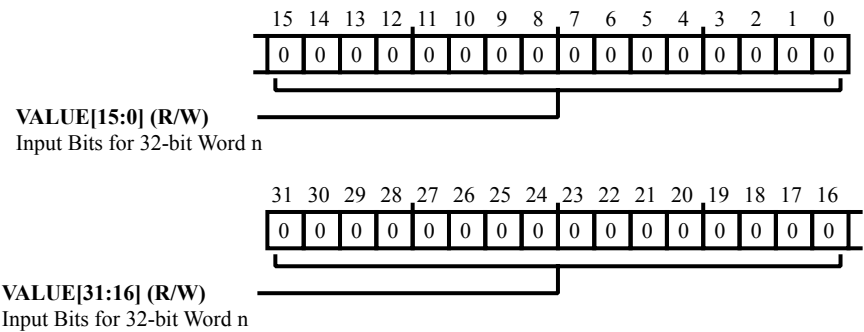
Figure 36-11: TRNG_INPUT[n] Register Diagram
