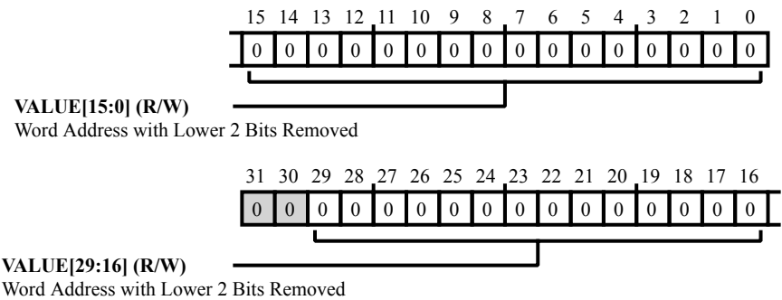
Figure 38-19: FIR_INBASE Register Diagram
