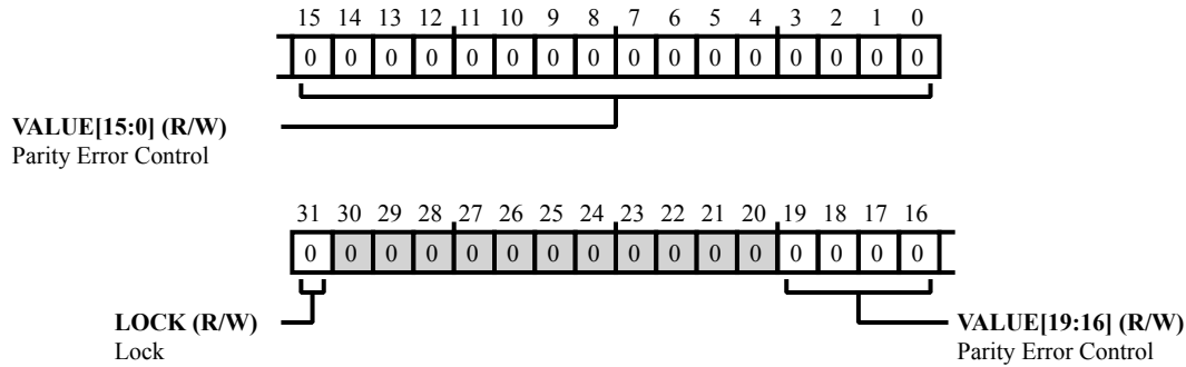
Figure 43-16: MEC_PERR_CTL Register Diagram
