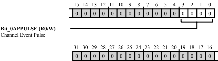
Figure 44-56: CTI_CTIAPPPULSE Register Diagram
