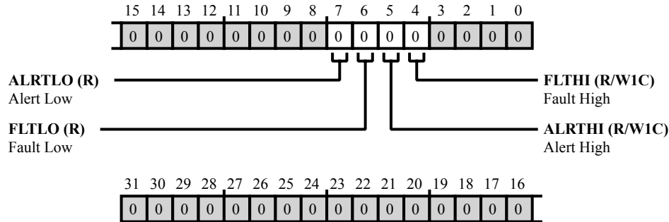
Figure 37-13: TMU_STAT Register Diagram
