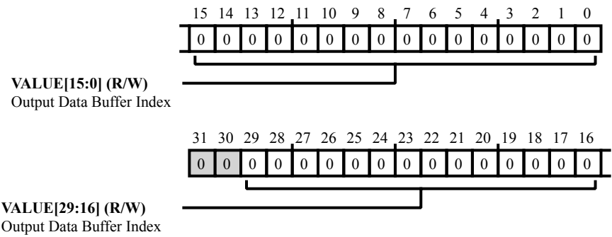
Figure 39-27: IIR_OUTIDX Register Diagram
