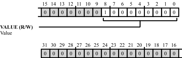
Figure 37-3: TMU_ALERT_LIM_LO Register Diagram
