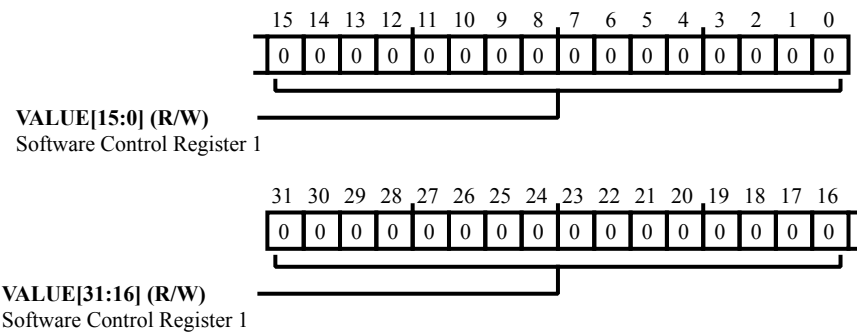
Figure 38-28: FIR_SCTL1 Register Diagram
