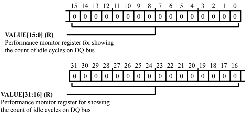
Figure 9-14: DMC_PM_IDCYDQ_CNT Register Diagram
