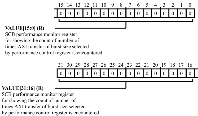
Figure 9-31: DMC_SCB_PM_BRSZ_CNT Register Diagram
