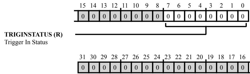
Figure 44-79: CTI_CTITRIGINSTATUS Register Diagram
