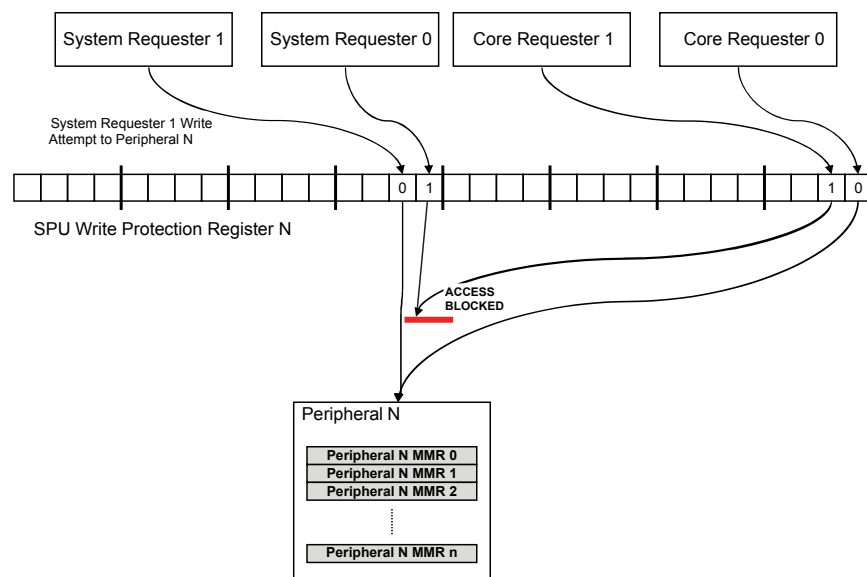
Figure 32-2: SPU Write-Protect Register Blocking Access from System Requester 0 and Core Requester 1
