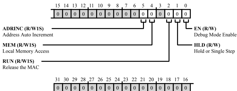
Figure 39-15: IIR_DBG_CTL Register Diagram
