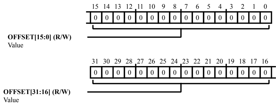
Figure 16-24: OSPI_REMAPADDR Register Diagram
