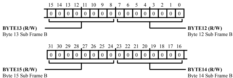
Figure 26-36: SPDIF_TX_UBUFF_B3 Register Diagram
