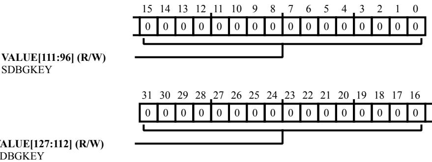
Figure 44-43: TAPC_SDBGKEY3 Register Diagram
