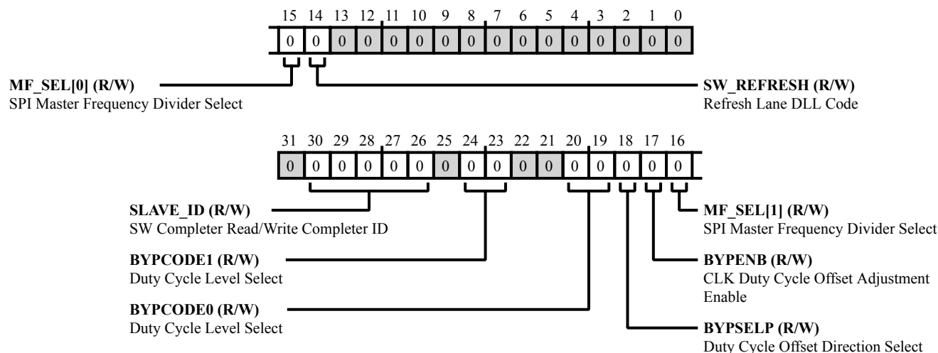
Figure 9-38: DMC_DDR_CA_CTL Register Diagram
