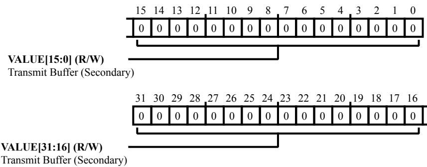
Figure 23-41: SPORT_TXSEC_B Register Diagram
