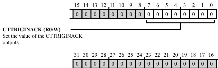
Figure 44-89: CTI_ITTRIGINACK Register Diagram
