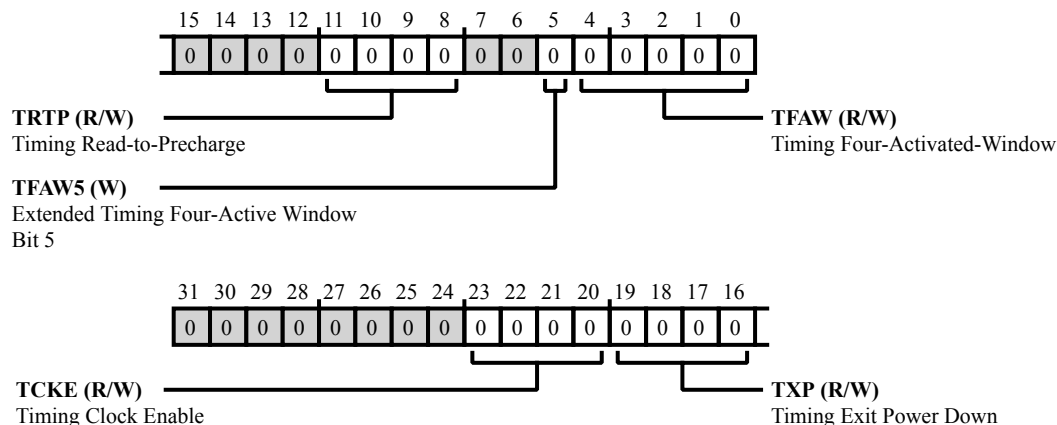
Figure 9-37: DMC_TR2 Register Diagram
