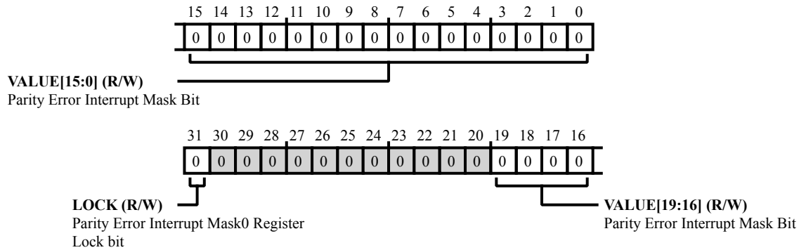
Figure 43-17: MEC_PERR_IMASK Register Diagram
