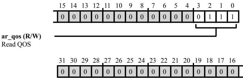
Figure 41-50: SCB0_SH0_IPORT_READ_QOS Register Diagram
