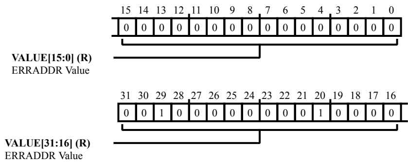
Figure 8-16: L2CTL_ERRADDR8 Register Diagram
