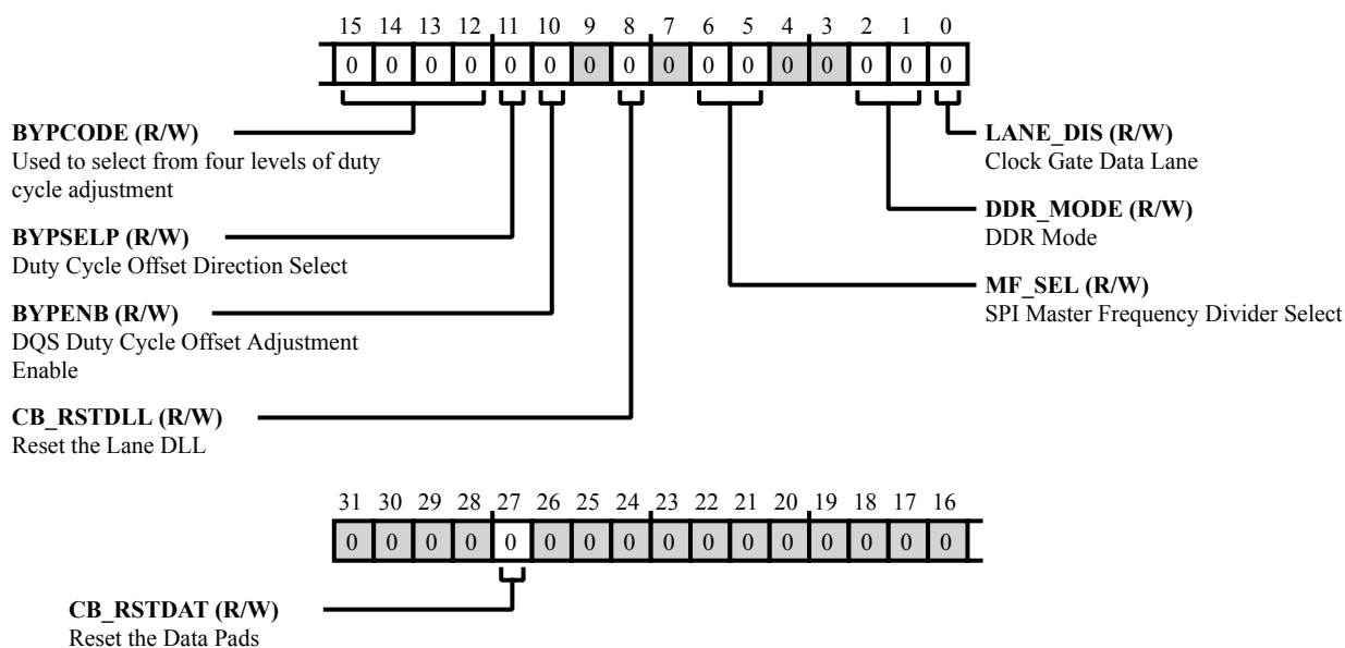
Figure 9-41: DMC_DDR_LANE1_CTL0 Register Diagram
