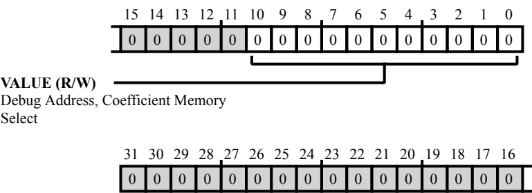
Figure 38-14: FIR_DBG_ADDR Register Diagram
