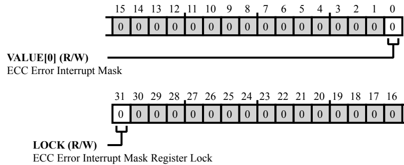
Figure 43-10: MEC_ECCERR_IMASK[y] Register Diagram
