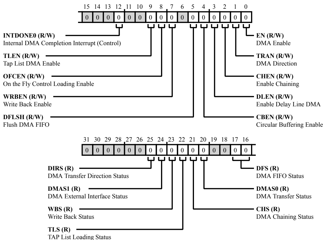
Figure 28-15: EMDMA_CTL Register Diagram
