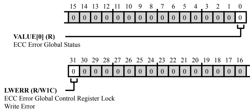
Figure 43-13: MEC_EEIRQ_GSTAT[q] Register Diagram
