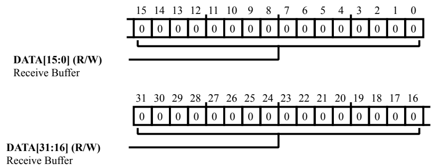
Figure 14-15: LP_RX Register Diagram
