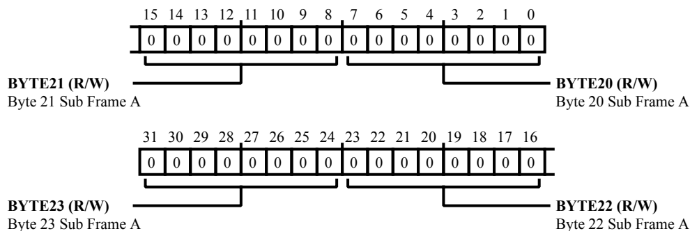
Figure 26-32: SPDIF_TX_UBUFF_A5 Register Diagram
