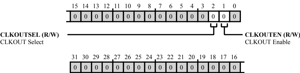
Figure 20-14: MLB_GCTL Register Diagram
