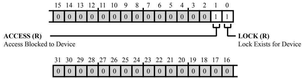
Figure 44-93: CTI_LSR Register Diagram
