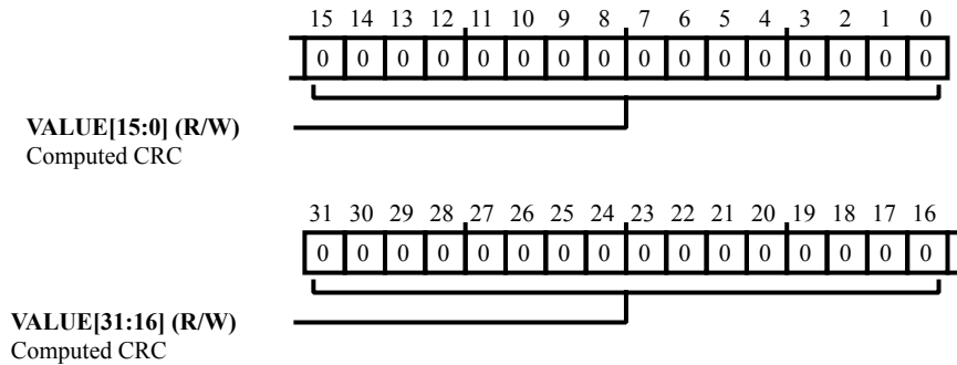
Figure 29-15: CRC_RESULT_FIN Register Diagram
