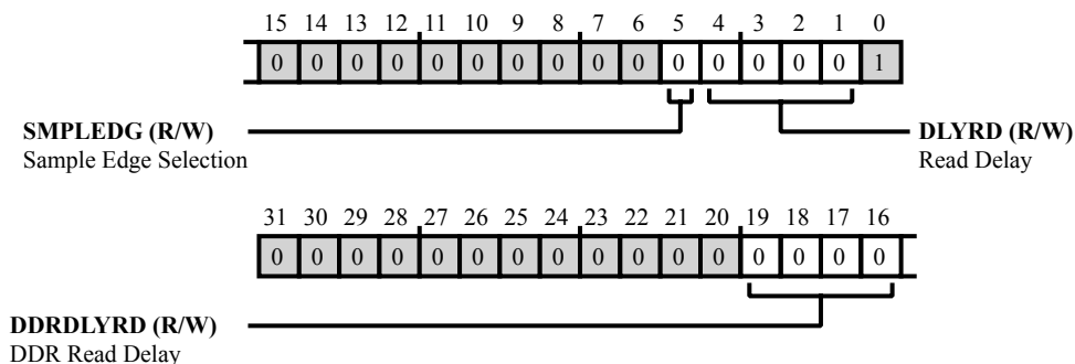
Figure 16-23: OSPI_RDC Register Diagram
