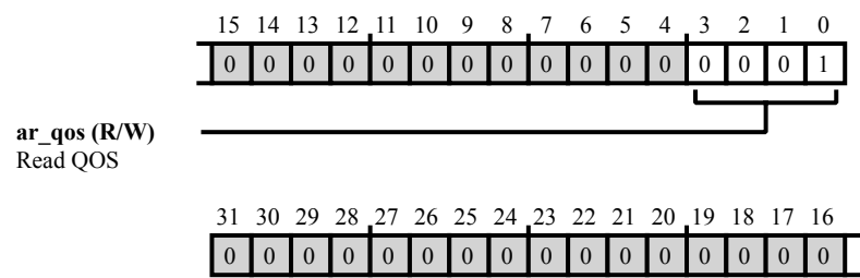
Figure 41-18: SCB0_CRC1_CH1_READ_QOS Register Diagram
