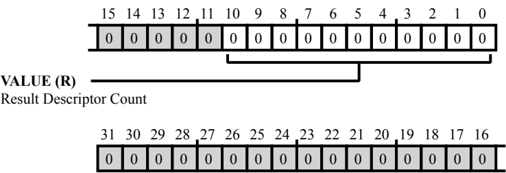
Figure 33-34: PKTE_RDSC_CNT Register Diagram
