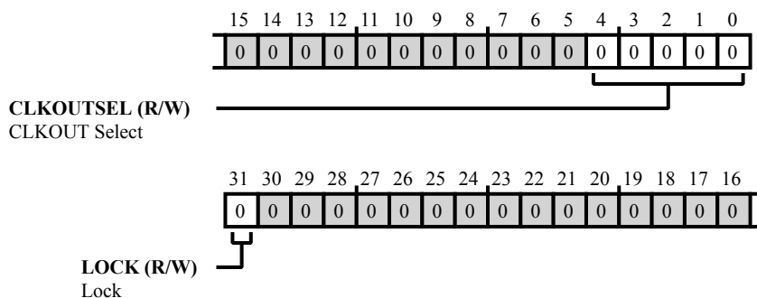
Figure 2-5: CGU_CLKOUTSEL Register Diagram
