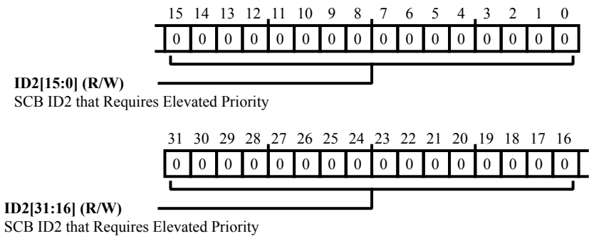
Figure 9-22: DMC_PRIO2 Register Diagram
