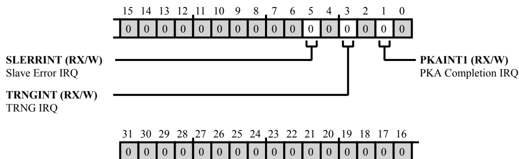
Figure 35-1: PKIC_ACK Register Diagram
