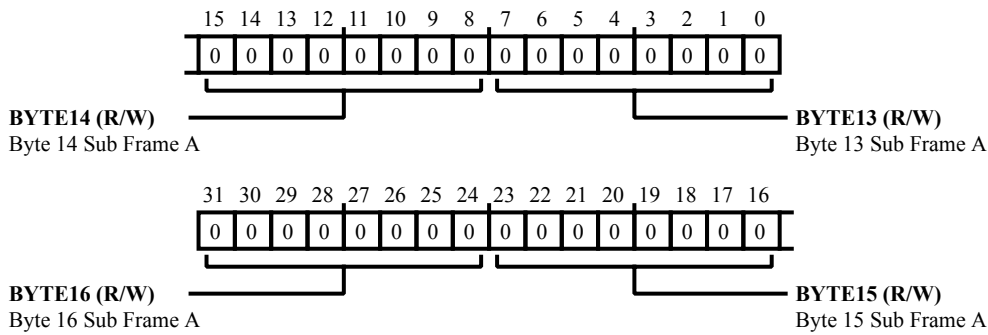
Figure 26-18: SPDIF_TX_STAT_A3 Register Diagram
