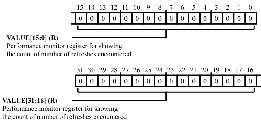
Figure 9-19: DMC_PM_REF_CNT Register Diagram
