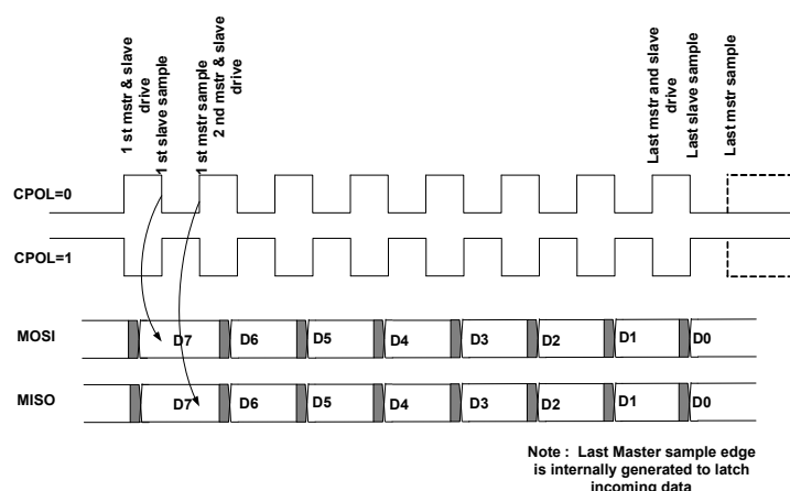
Figure 15-12: SPI Transfer Protocol in Fast Mode for SPI_CTL.CPHA = 1
