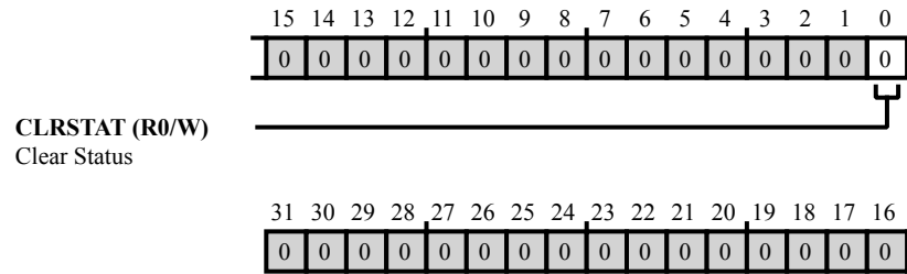
Figure 43-8: MEC_CLR Register Diagram
