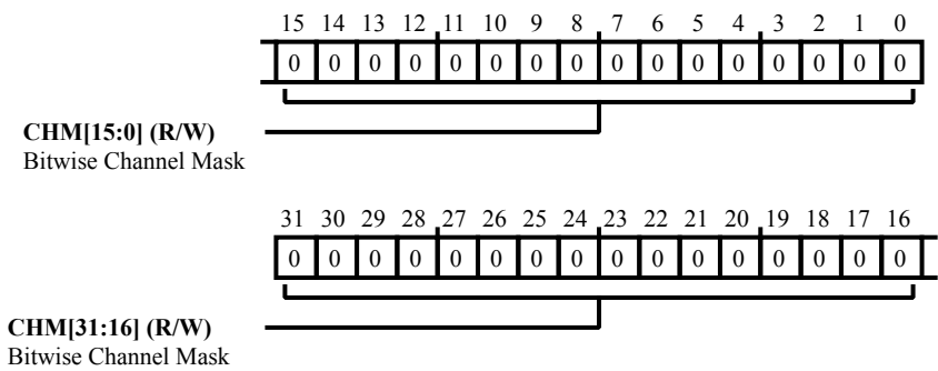
Figure 20-8: MLB_ACMR1 Register Diagram
