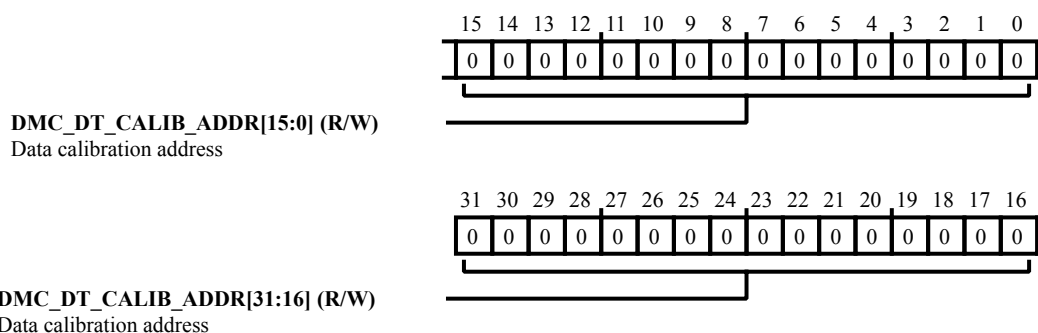
Figure 9-4: DMC_DT_CALIB_ADDR Register Diagram
