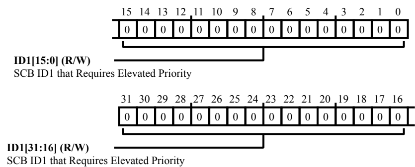
Figure 9-21: DMC_PRIO Register Diagram
