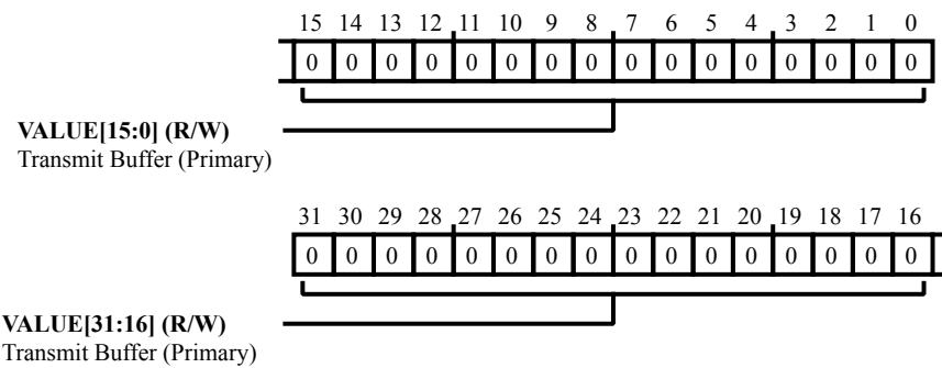
Figure 23-39: SPORT_TXPRI_B Register Diagram
