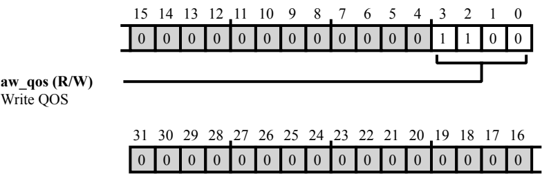
Figure 41-77: SCB0_SP5B_WRITE_QOS Register Diagram
