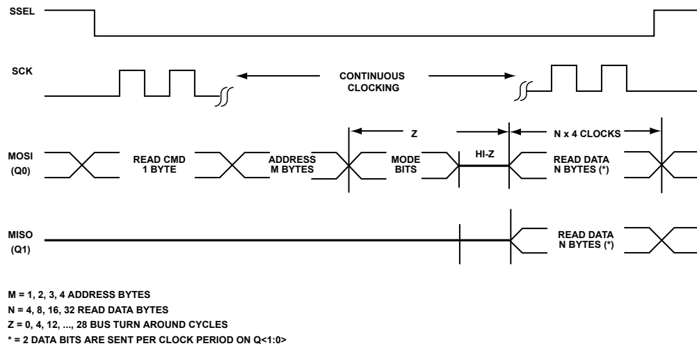
Figure 15-16: SPI Flash Fast Read (Dual Output) Sequence
