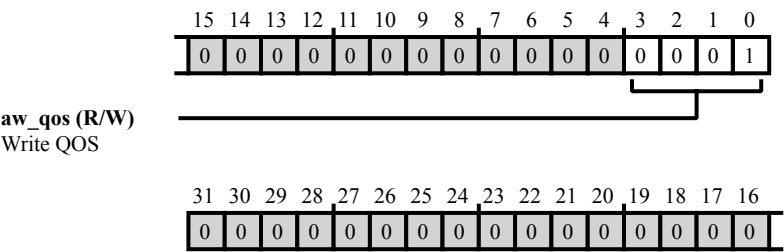
Figure 41-41: SCB0_LP1_WRITE_QOS Register Diagram
