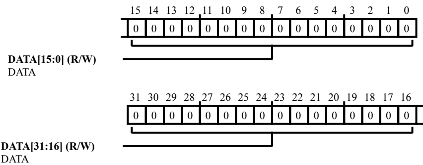
Figure 20-27: MLB_MDAT3 Register Diagram
