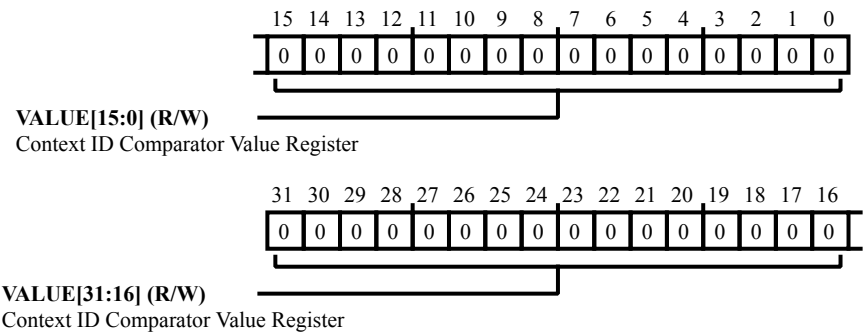
Figure 44-13: CSPFT_CIDCVR[n] Register Diagram
