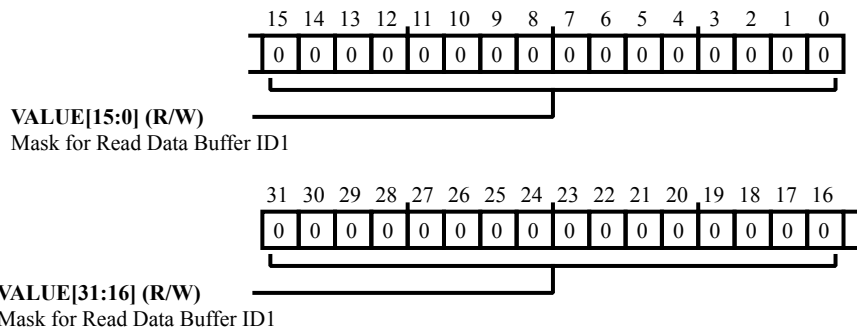
Figure 9-25: DMC_RDDATABUFID1 Register Diagram
