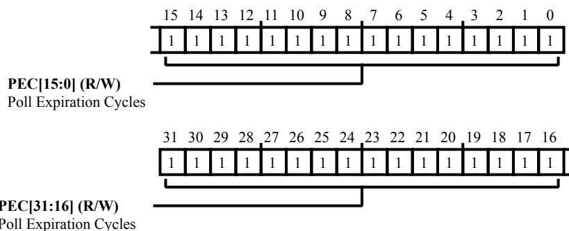
Figure 16-19: OSPI_POLLEXP Register Diagram
