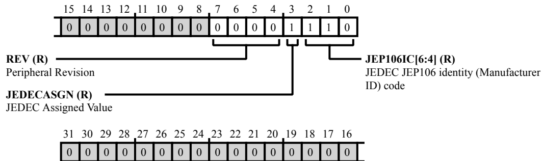
Figure 43-21: MEC_PID2 Register Diagram
