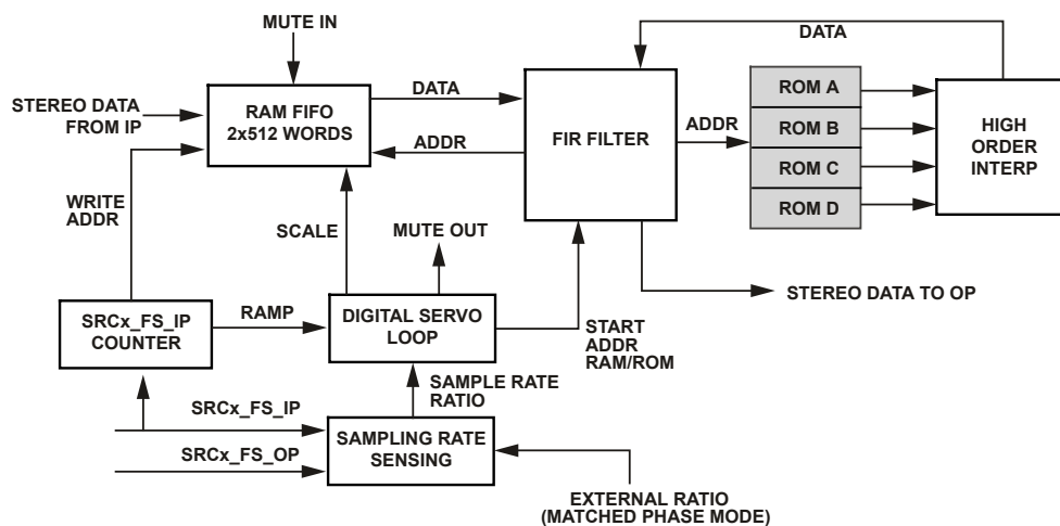
Figure 25-2: ASRC Core Architecture
