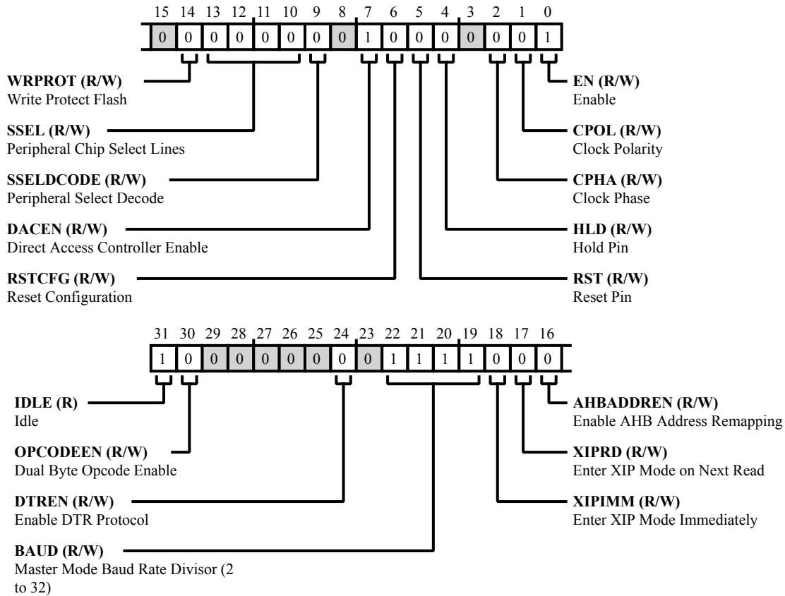
Figure 16-2: OSPI_CTL Register Diagram
