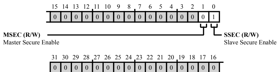
Figure 32-9: SPU_SECUREP[n] Register Diagram
