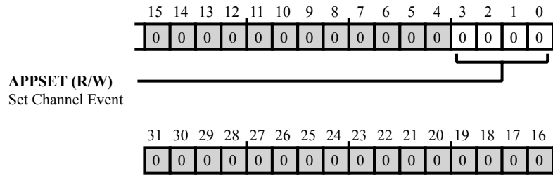
Figure 44-57: CTI_CTIAPPSET Register Diagram
