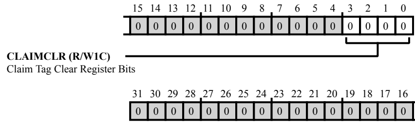
Figure 44-49: CTI_CLAIMCLR Register Diagram
