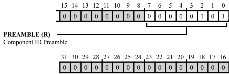
Figure 43-6: MEC_CID2 Register Diagram
