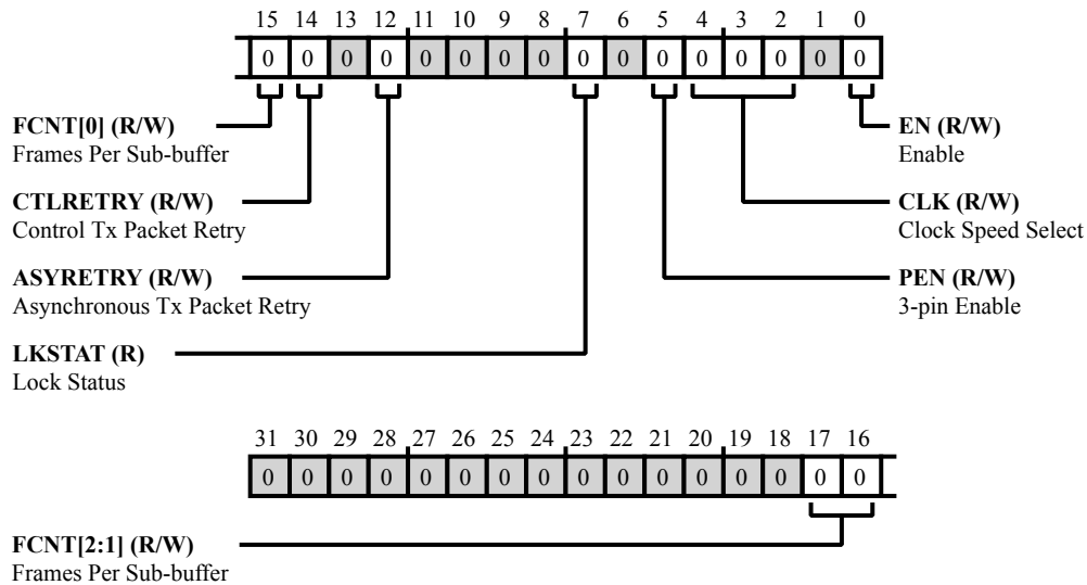
Figure 20-12: MLB_CTL0 Register Diagram
