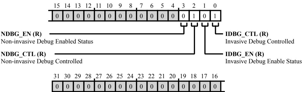
Figure 44-48: CTI_AUTHSTATUS Register Diagram
