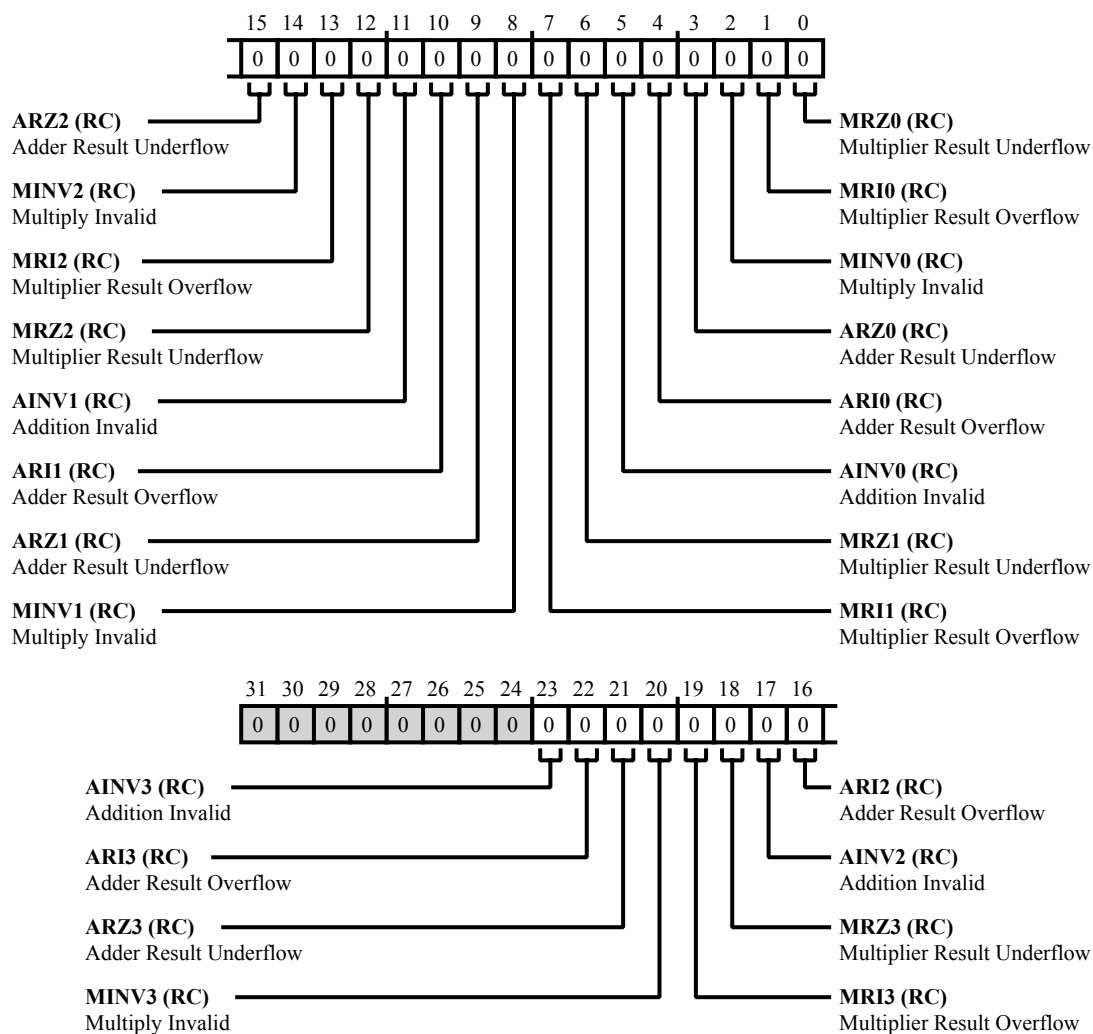
Figure 38-23: FIR_MACSTAT Register Diagram
