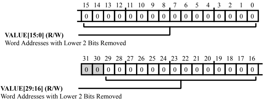
Figure 38-10: FIR_COEFIDX Register Diagram
