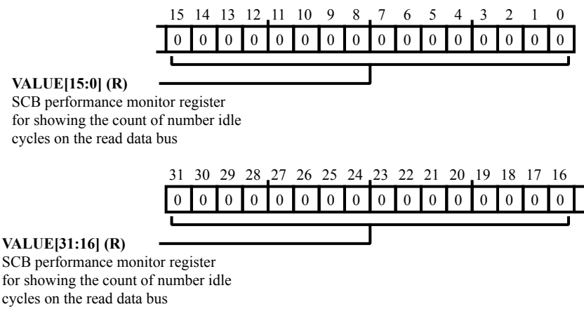
Figure 9-32: DMC_SCB_PM_IDRDDCY_CNT Register Diagram
