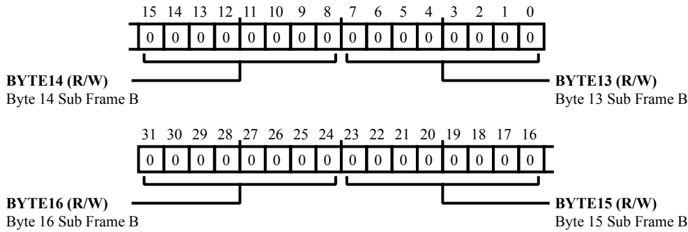
Figure 26-24: SPDIF_TX_STAT_B3 Register Diagram
