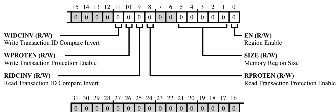
Figure 11-8: SMPU_RCTL[n] Register Diagram
