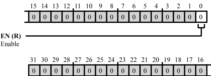
Figure 26-39: SPDIF_TX_USRUPDT Register Diagram
