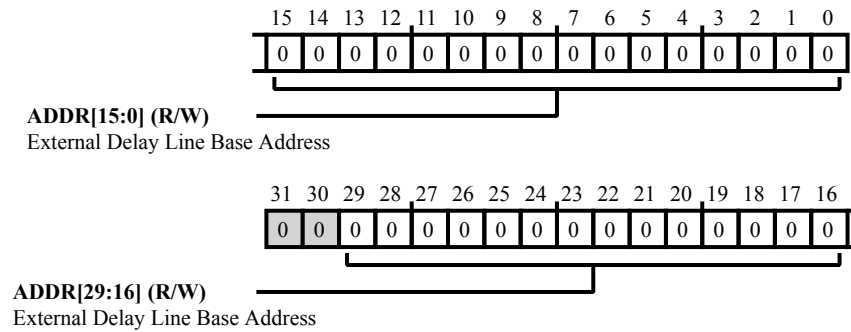
Figure 28-10: EMDMA_BASE Register Diagram
