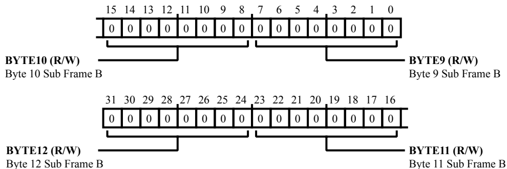
Figure 26-23: SPDIF_TX_STAT_B2 Register Diagram
