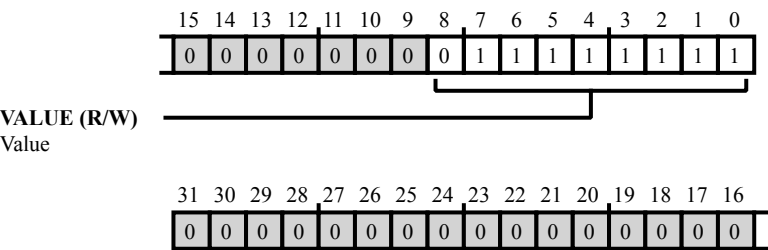
Figure 37-7: TMU_FLT_LIM_HI Register Diagram
