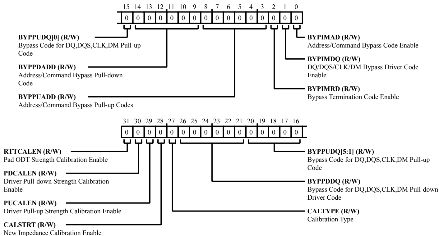
Figure 9-48: DMC_DDR_ZQ_CTL2 Register Diagram
