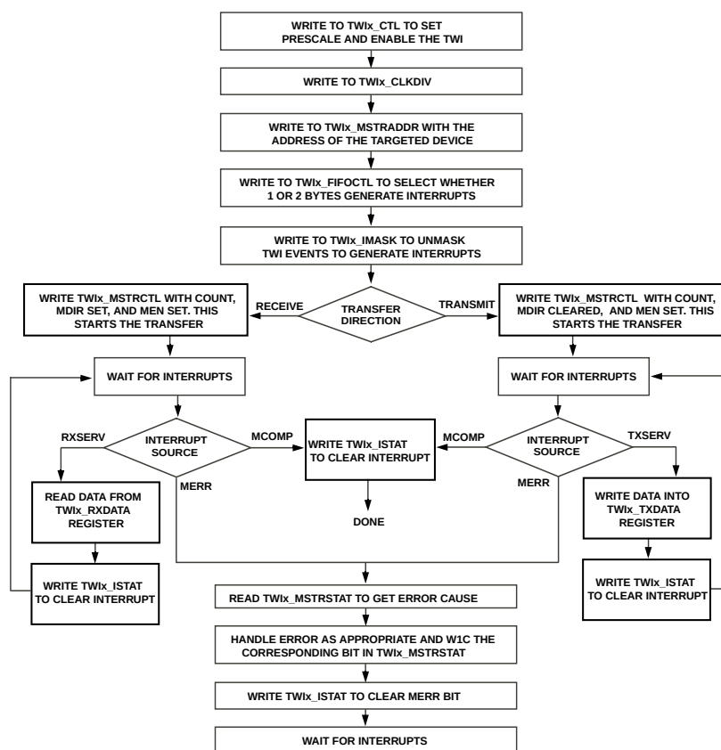
Figure 21-13: Requester Mode Program Flow
