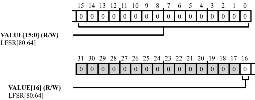
Figure 36-14: TRNG_LFSR_H Register Diagram
