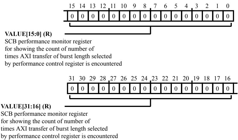
Figure 9-30: DMC_SCB_PM_BRLN_CNT Register Diagram
