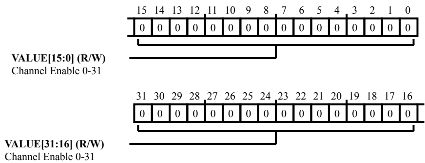
Figure 23-15: SPORT_CS0_B Register Diagram
