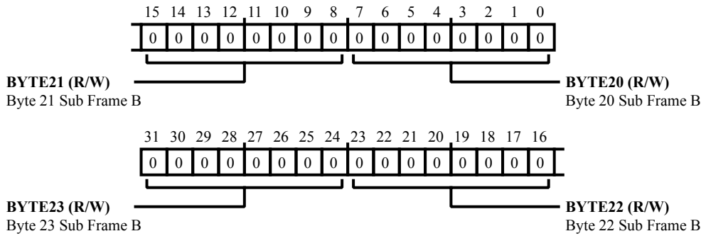
Figure 26-38: SPDIF_TX_UBUFF_B5 Register Diagram
