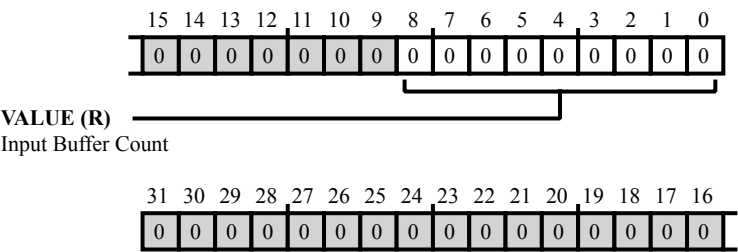
Figure 33-24: PKTE_INBUF_CNT Register Diagram
