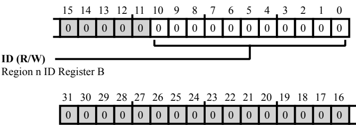
Figure 11-11: SMPU_RIDB[n] Register Diagram
