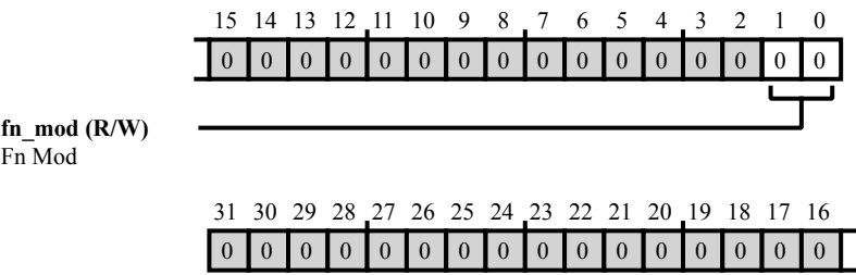
Figure 41-127: SCB4_IIR_CH0_IB_FN_MOD Register Diagram
