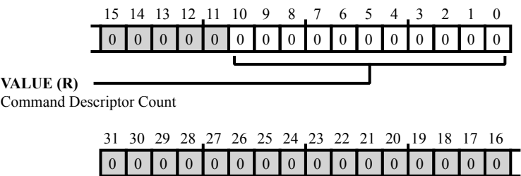
Figure 33-9: PKTE_CDSC_CNT Register Diagram
