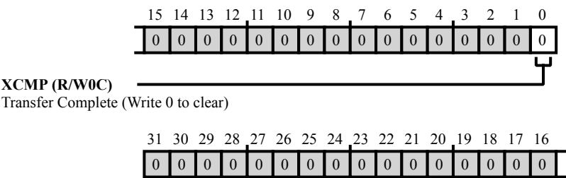
Figure 20-23: MLB_MCTL Register Diagram
