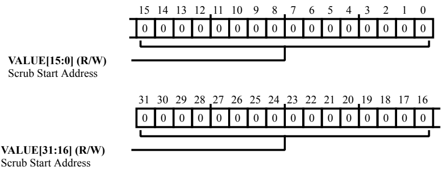
Figure 8-24: L2CTL_SADR Register Diagram
