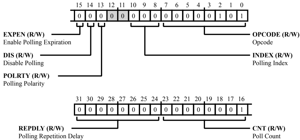
Figure 16-27: OSPI_WCCTL Register Diagram
