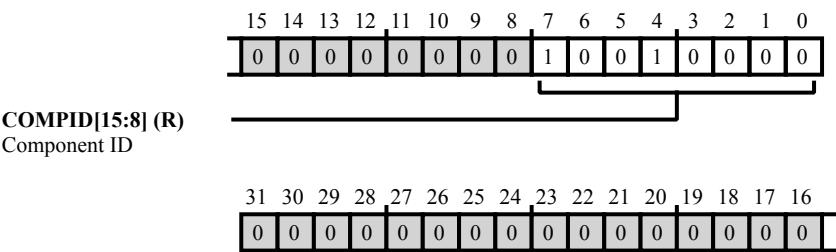
Figure 44-9: CSPFT_CID1 Register Diagram
