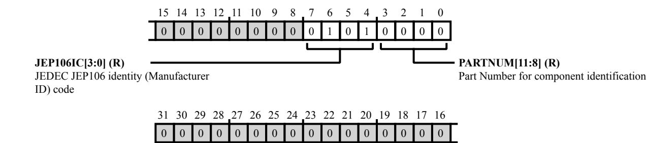
Figure 43-20: MEC_PID1 Register Diagram
