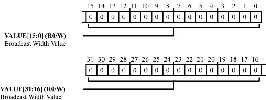
Figure 18-13: TIMER_BCAST_WID Register Diagram
