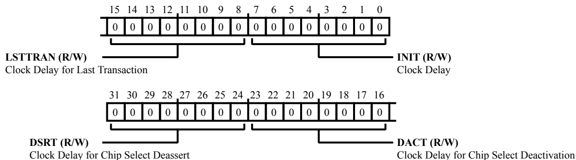
Figure 16-3: OSPI_DLY Register Diagram
