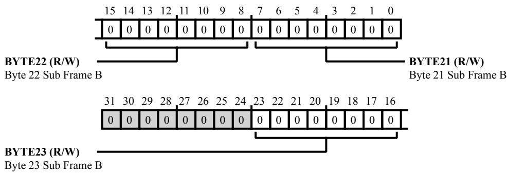
Figure 26-26: SPDIF_TX_STAT_B5 Register Diagram
