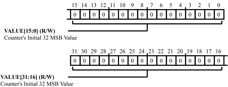
Figure 2-19: CGU_TSVALUE1 Register Diagram
