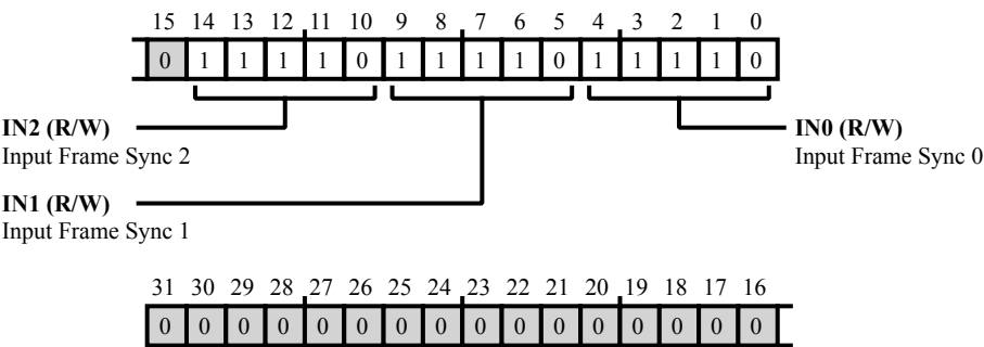
Figure 22-32: DAI_FS2 Register Diagram
