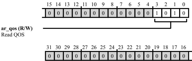
Figure 41-98: SCB0_UART0_RX_READ_QOS Register Diagram
