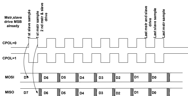
Figure 15-11: SPI Transfer Protocol in Fast Mode for SPI_CTL.CPHA = 0
