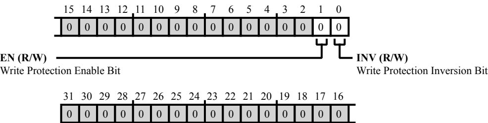
Figure 16-26: OSPI_WRPROT_CTL Register Diagram
