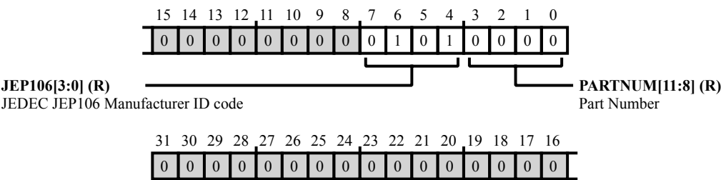
Figure 44-27: CSPFT_PID1 Register Diagram
