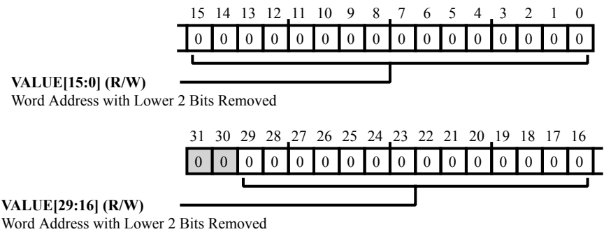
Figure 38-24: FIR_OUTBASE Register Diagram
