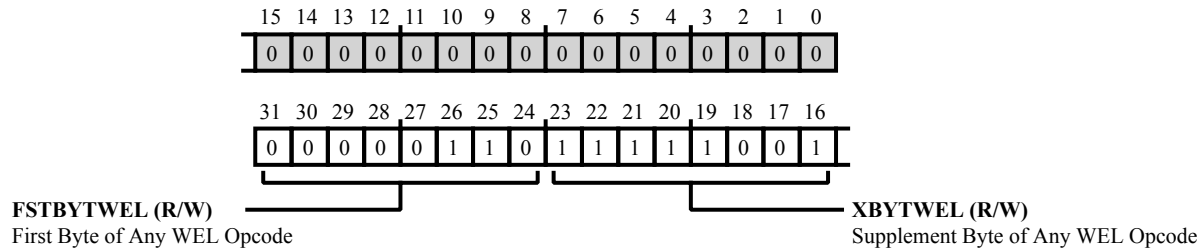
Figure 16-21: OSPI_OE_UP Register Diagram
