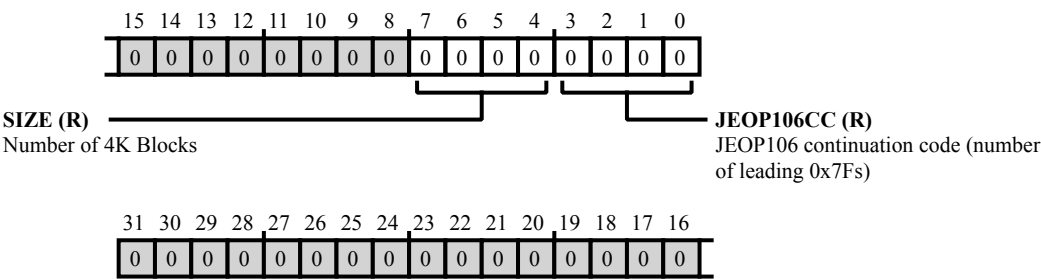
Figure 44-30: CSPFT_PID4 Register Diagram
