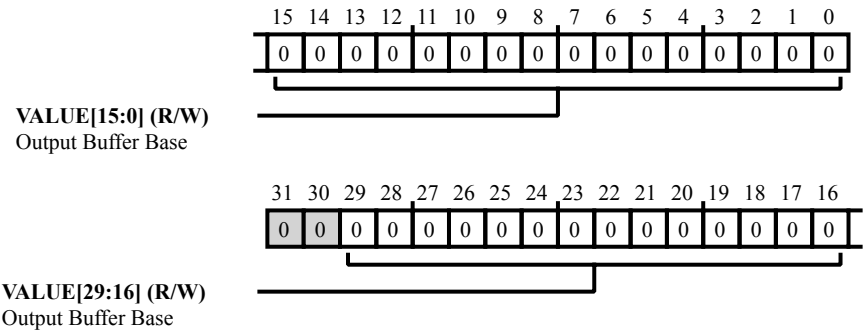
Figure 39-26: IIR_OUTBASE Register Diagram
