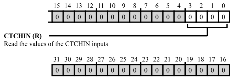
Figure 44-83: CTI_ITCHIN Register Diagram
