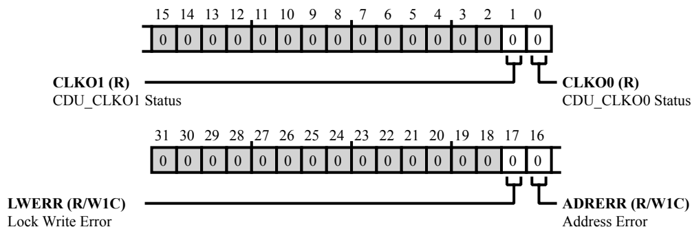
Figure 3-4: CDU_STAT Register Diagram
