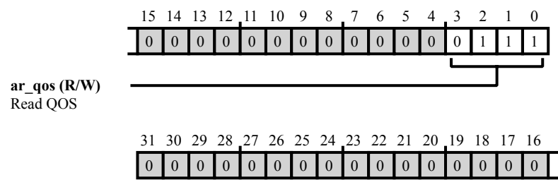
Figure 41-48: SCB0_SH0_DPORT_READ_QOS Register Diagram
