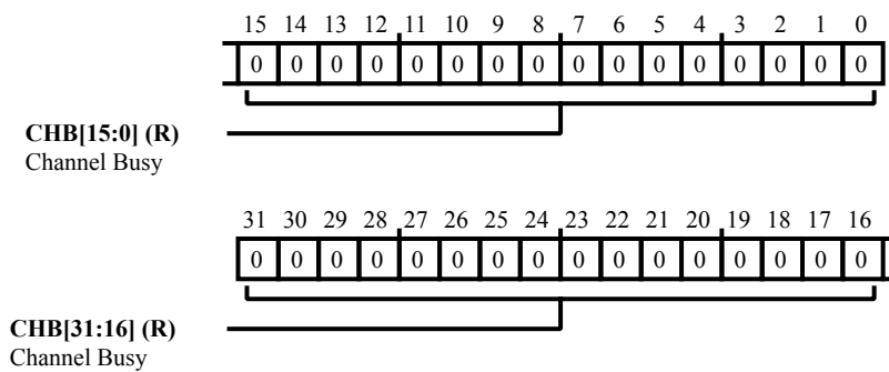
Figure 20-16: MLB_HCBR1 Register Diagram
