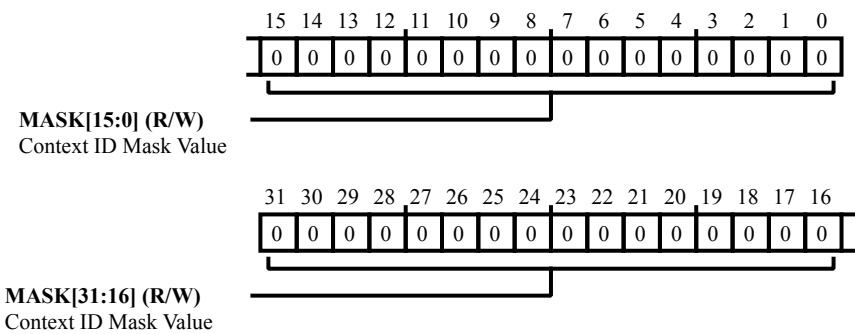
Figure 44-12: CSPFT_CIDCMR Register Diagram
