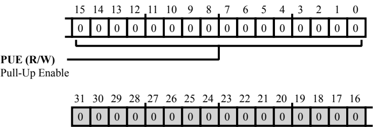
Figure 12-52: PADS_PORT[n]_PUE Register Diagram
