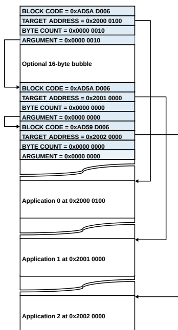
Figure 40-17: Multi-Application Direct Code Execution Example
