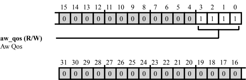
Figure 41-134: SCB4_IIR_CH1_IB_WRITE_QOS Register Diagram
