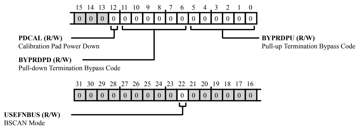
Figure 9-47: DMC_DDR_ZQ_CTL1 Register Diagram
