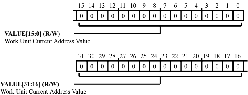
Figure 27-6: DMA_ADDR_CUR Register Diagram
