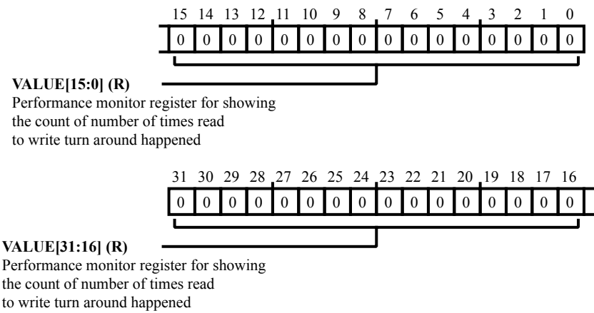
Figure 9-18: DMC_PM_RD2WRTA_CNT Register Diagram
