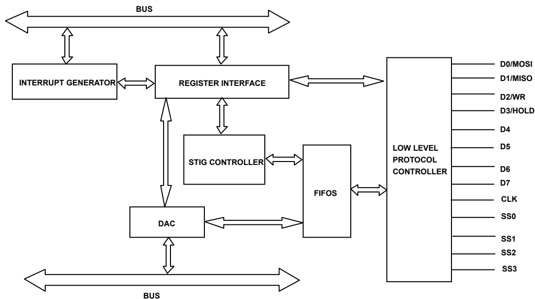
Figure 16-1: OSPI Controller Block Diagram
