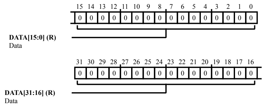
Figure 16-11: OSPI_FCRD_UP Register Diagram
