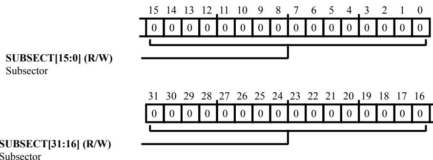
Figure 16-25: OSPI_WRPROT_UP Register Diagram
