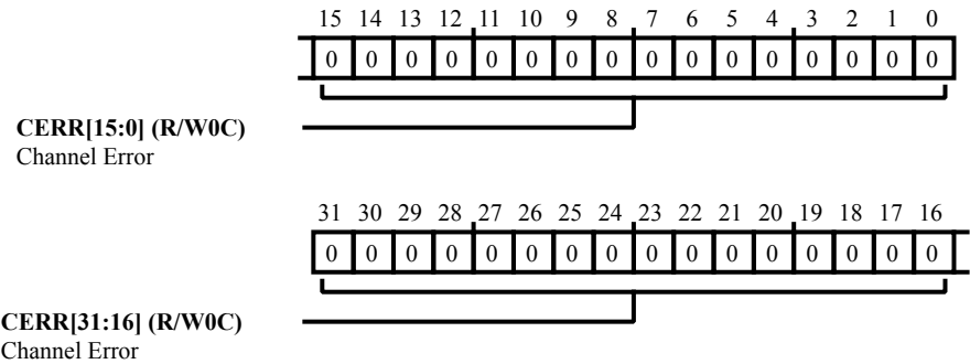
Figure 20-18: MLB_HCER1 Register Diagram
