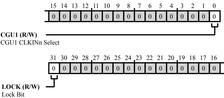
Figure 3-2: CDU_CLKINSEL Register Diagram
