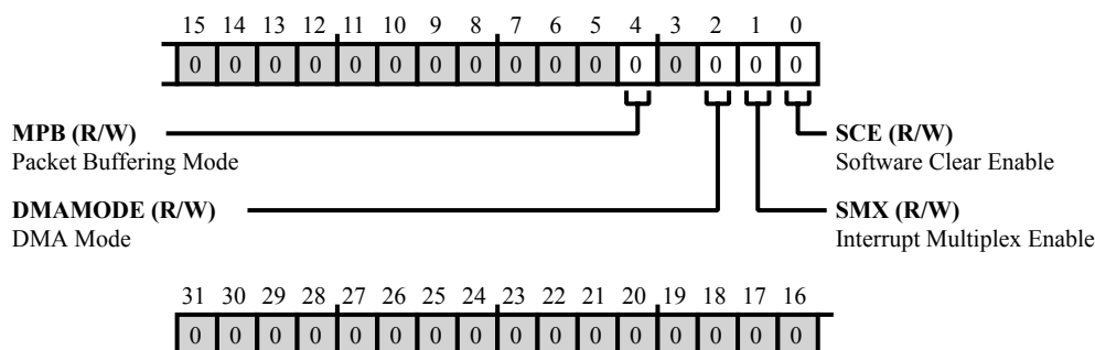
Figure 20-11: MLB_ACTL Register Diagram
