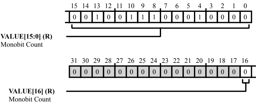
Figure 36-17: TRNG_MONOBITCNT Register Diagram
