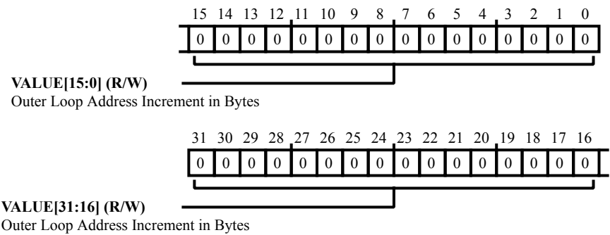
Figure 27-21: DMA_YMOD Register Diagram
