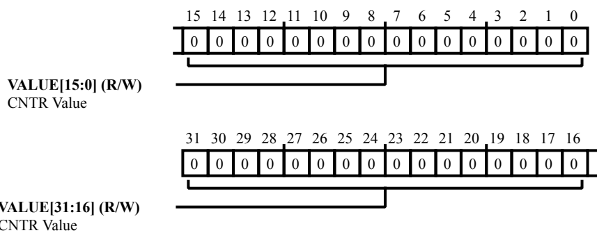
Figure 19-6: CNT_CNTR Register Diagram
