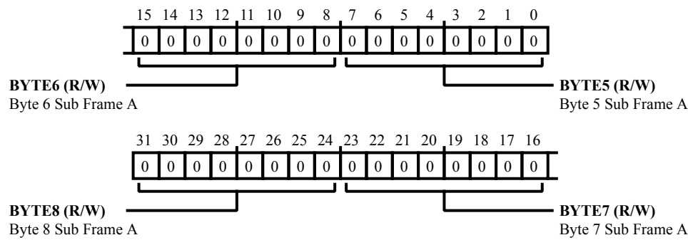
Figure 26-16: SPDIF_TX_STAT_A1 Register Diagram
