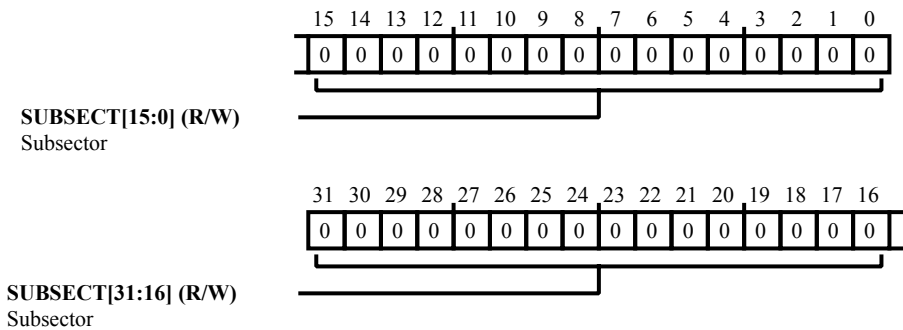
Figure 16-16: OSPI_WRPROT_LWR Register Diagram
