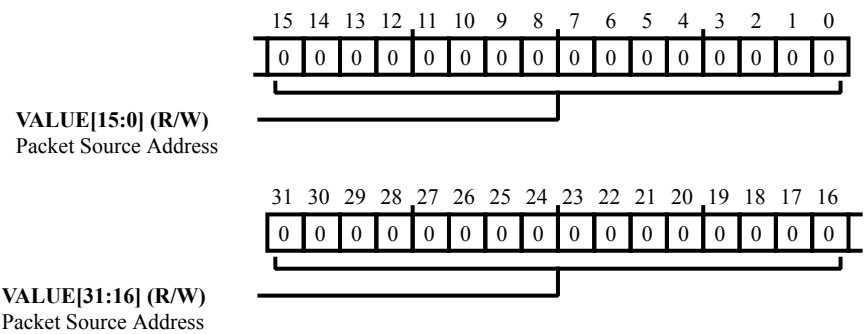
Figure 33-52: PKTE_SRC_ADDR Register Diagram
