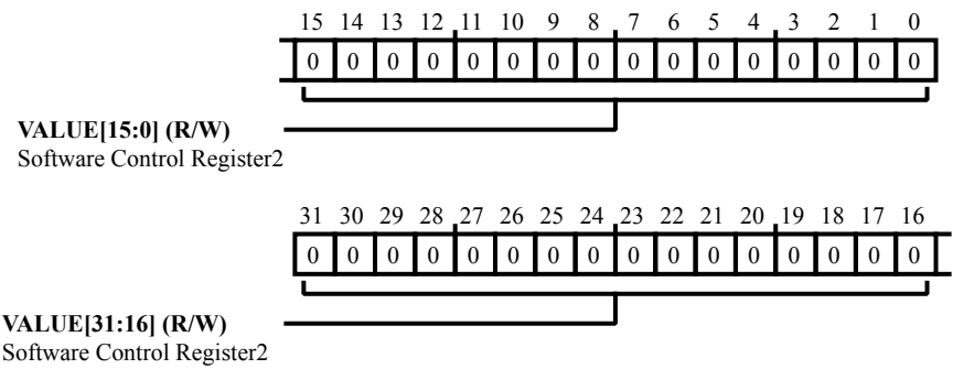
Figure 39-31: IIR_SCTL2 Register Diagram
