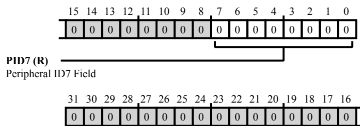
Figure 44-101: CTI_PERIPHID7 Register Diagram
