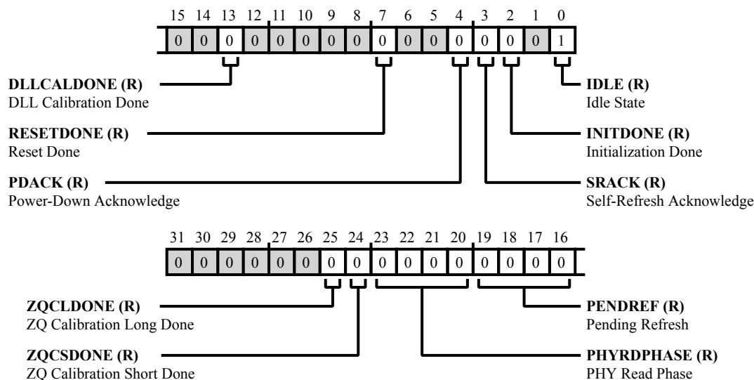
Figure 9-34: DMC_STAT Register Diagram
