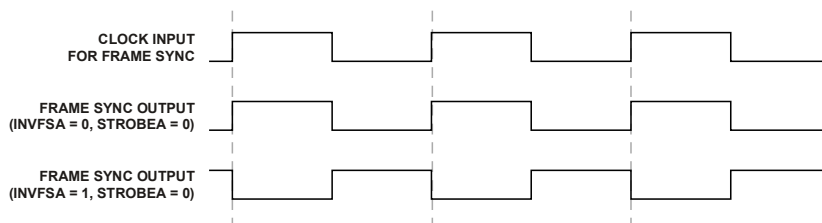
Figure 24-3: Bypass and Inverted Bypass
