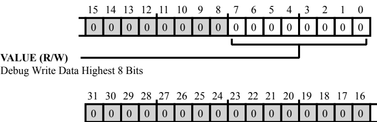
Figure 39-18: IIR_DBG_WRDAT_HI Register Diagram
