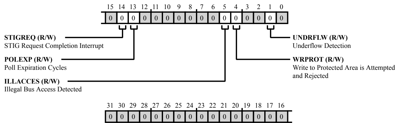
Figure 16-15: OSPI_ISTAT Register Diagram
