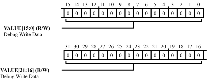
Figure 38-17: FIR_DBG_WRDAT Register Diagram
