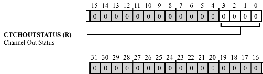
Figure 44-59: CTI_CTICHOUTSTATUS Register Diagram
