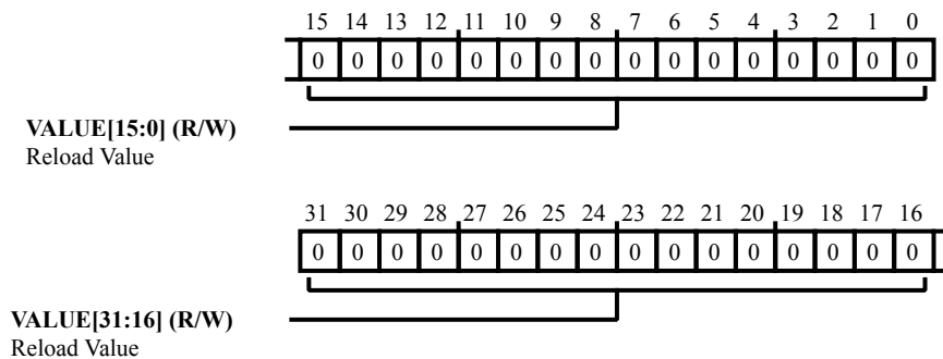
Figure 29-7: CRC_DCNTRLD Register Diagram
