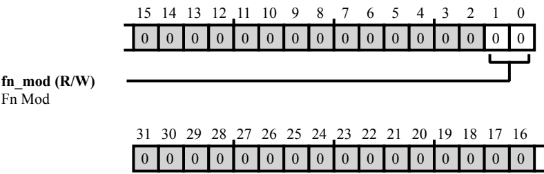
Figure 41-131: SCB4_IIR_CH1_IB_FN_MOD Register Diagram
