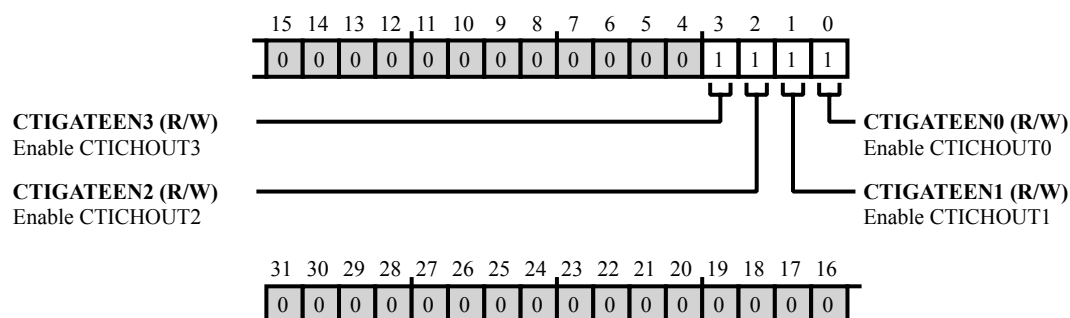
Figure 44-61: CTI_CTIGATE Register Diagram
