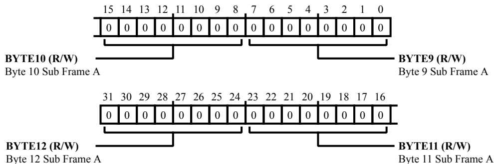
Figure 26-17: SPDIF_TX_STAT_A2 Register Diagram
