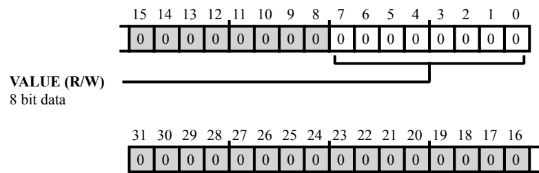
Figure 17-22: UART_THR Register Diagram
