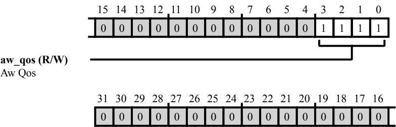
Figure 41-122: SCB4_FIR_CH0_IB_WRITE_QOS Register Diagram
