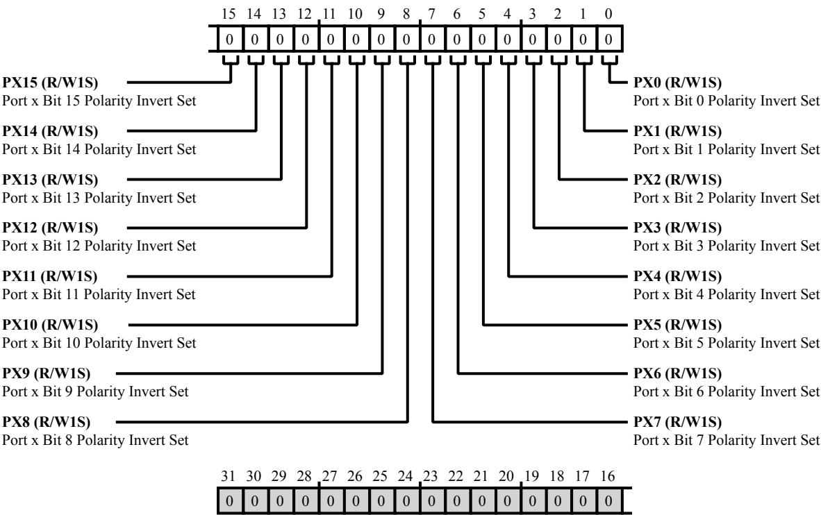
Figure 12-24: PORT_POL_SET Register Diagram
