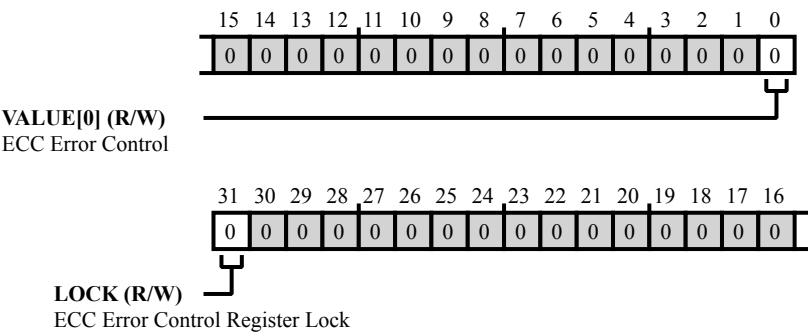
Figure 43-9: MEC_ECCERR_CTL[y] Register Diagram
