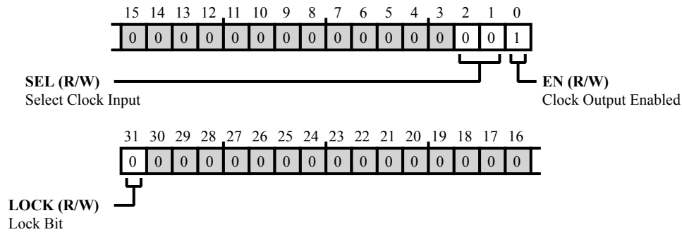
Figure 3-1: CDU_CFG[n] Register Diagram
