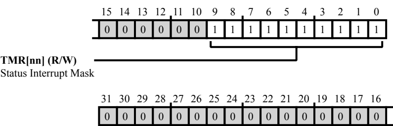
Figure 18-21: TIMER_STAT_IMSK Register Diagram
