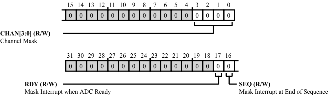
Figure 30-8: HADC_IMSK Register Diagram
