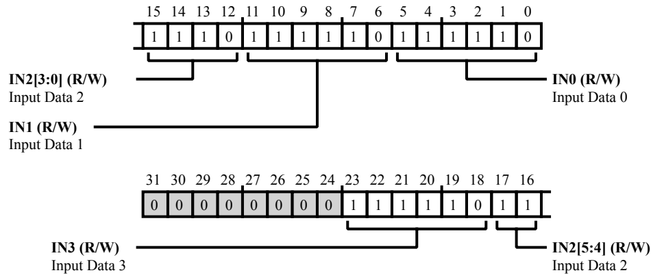
Figure 22-29: DAI_DAT6 Register Diagram
