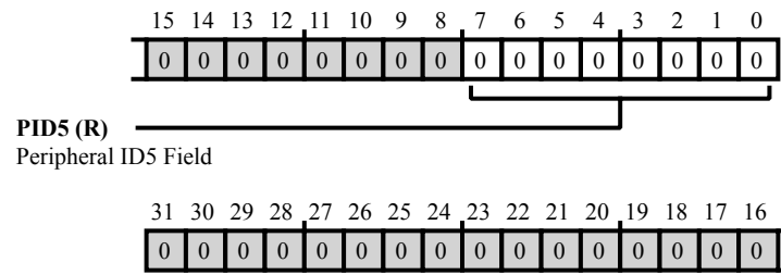
Figure 44-99: CTI_PERIPHID5 Register Diagram
