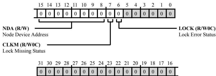
Figure 20-13: MLB_CTL1 Register Diagram
