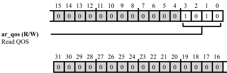
Figure 41-106: SCB0_UART2_RX_READ_QOS Register Diagram
