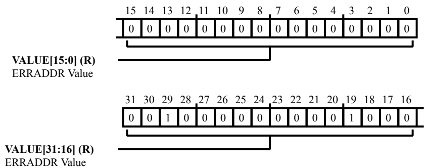
Figure 8-12: L2CTL_ERRADDR4 Register Diagram
