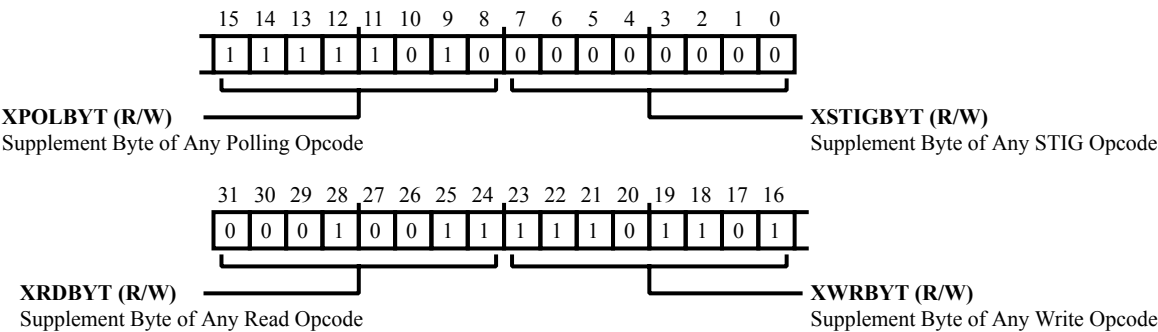
Figure 16-20: OSPI_OE_LWR Register Diagram
