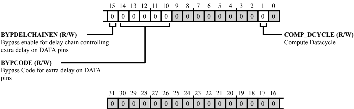
Figure 9-42: DMC_DDR_LANE1_CTL1 Register Diagram
