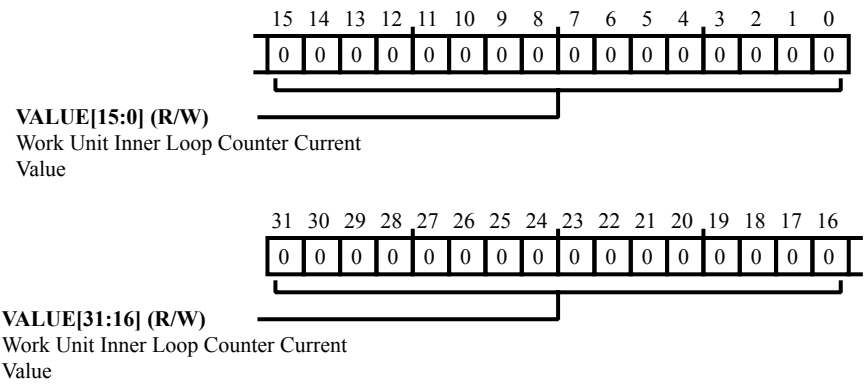
Figure 27-19: DMA_YCNT Register Diagram
