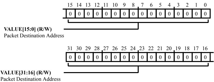
Figure 33-16: PKTE_DEST_ADDR Register Diagram
