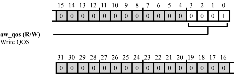
Figure 41-21: SCB0_CRYPTOWRITE_QOS Register Diagram
