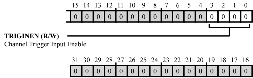
Figure 44-67: CTI_TRIGGER5 Register Diagram
