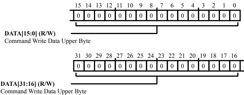
Figure 16-13: OSPI_FCWD_UP Register Diagram
