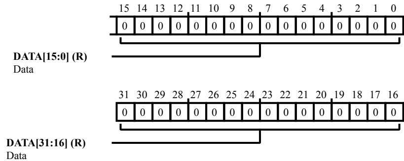
Figure 16-10: OSPI_FCRD_LWR Register Diagram
