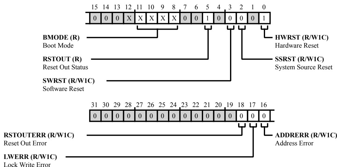
Figure 5-11: RCU_STAT Register Diagram
