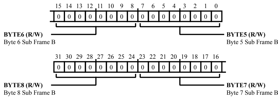
Figure 26-22: SPDIF_TX_STAT_B1 Register Diagram
