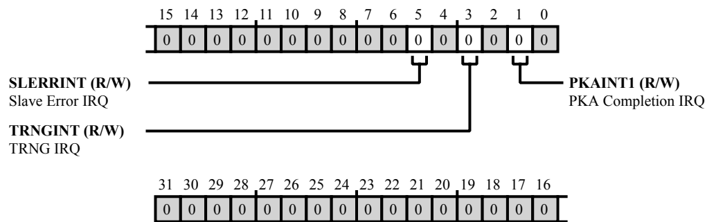
Figure 35-3: PKIC_EN_CTL Register Diagram
