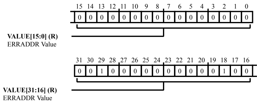
Figure 8-10: L2CTL_ERRADDR2 Register Diagram
