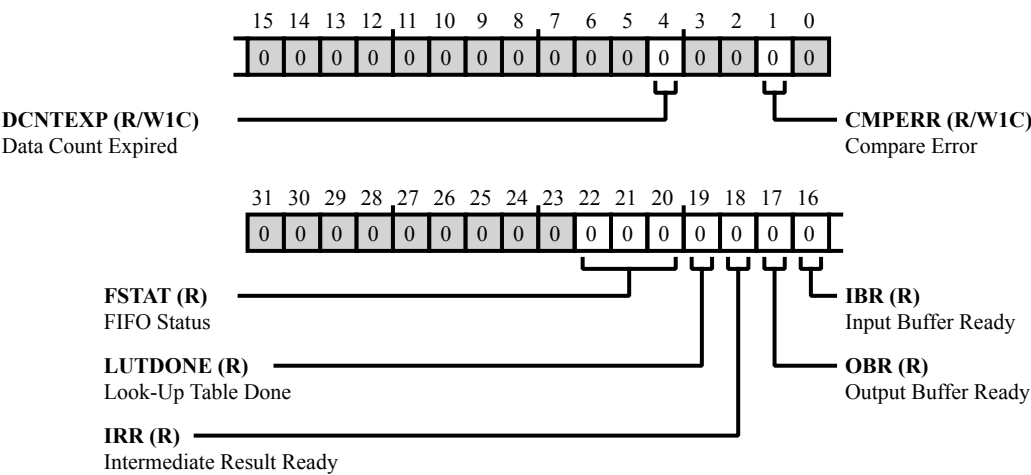
Figure 29-16: CRC_STAT Register Diagram
