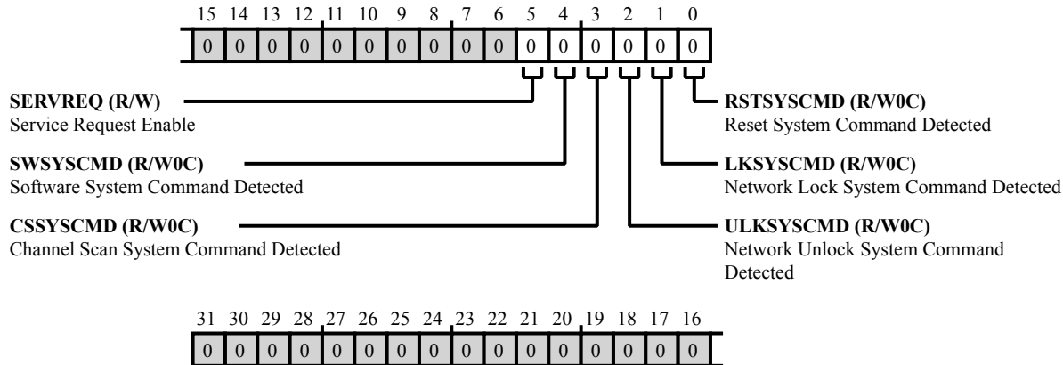
Figure 20-36: MLB_MSS Register Diagram
