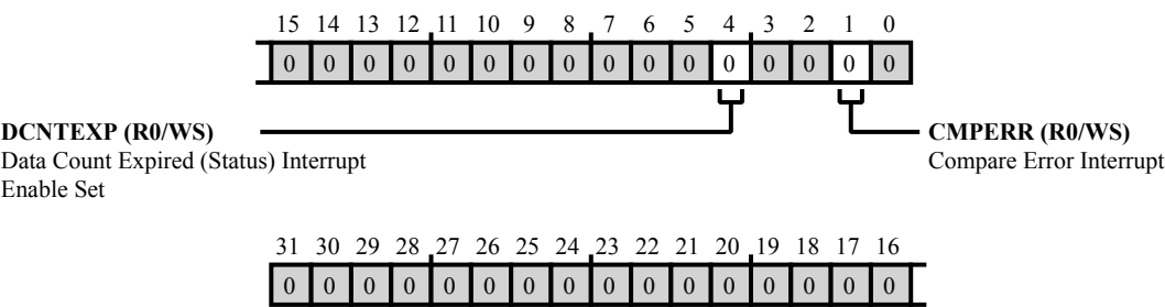
Figure 29-12: CRC_INEN_SET Register Diagram
