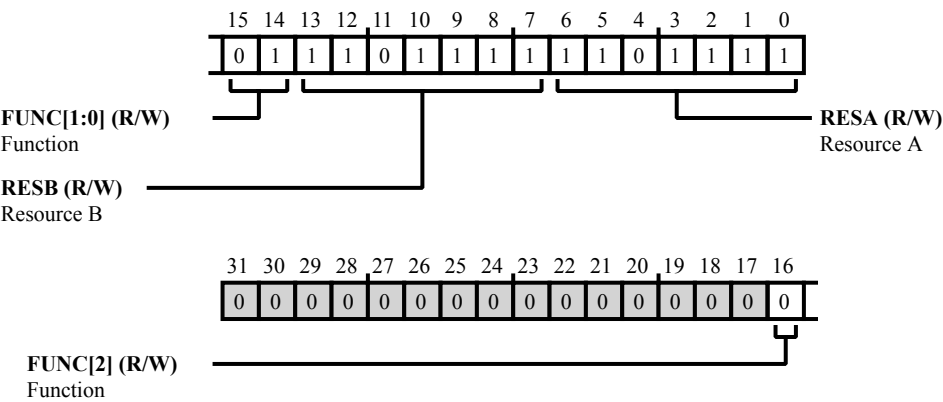
Figure 44-22: CSPFT_EXTOUTEVR[n] Register Diagram
