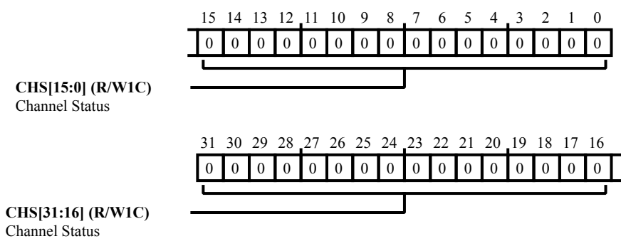
Figure 20-9: MLB_ACSR0 Register Diagram
