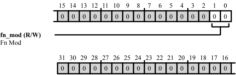
Figure 41-143: SCB4_SHARC_DPORT_FN_MOD Register Diagram
