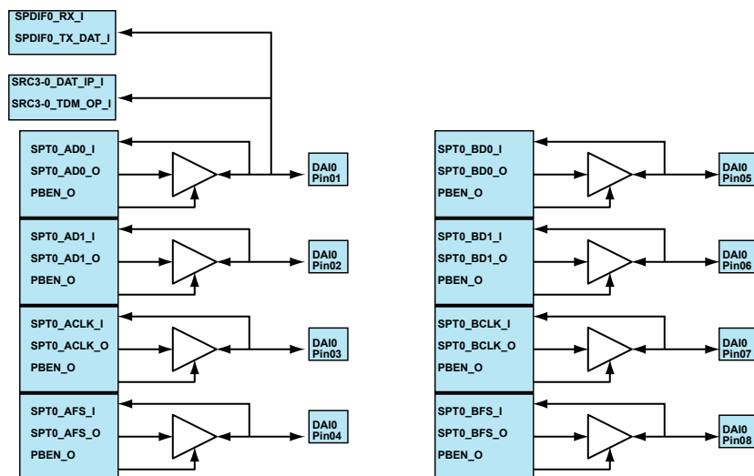
Figure 22-10: DAI0 Default Routing Pins 01-08
