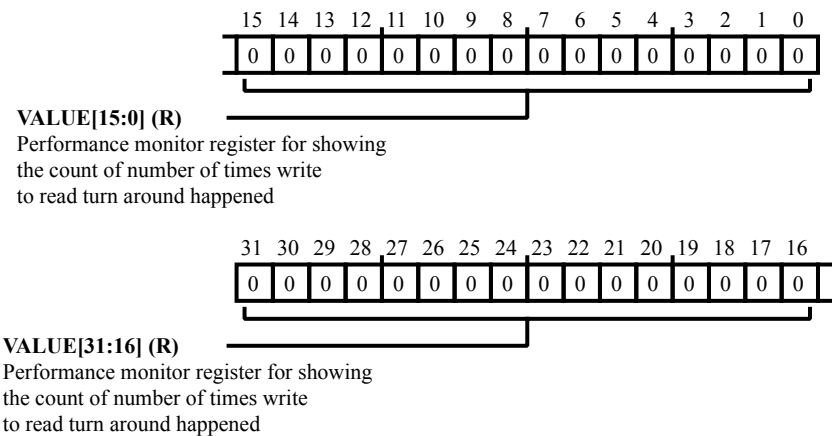
Figure 9-20: DMC_PM_WR2RDTA_CNT Register Diagram
