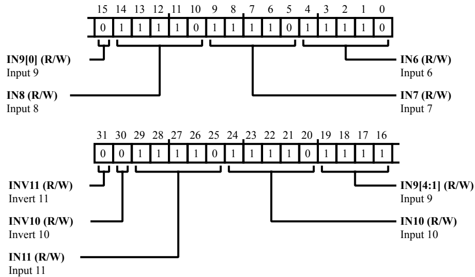
Figure 22-43: DAI_MISC0 Register Diagram
