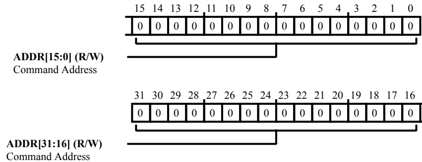
Figure 16-7: OSPI_FCA Register Diagram
