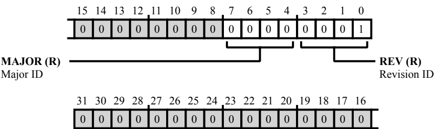
Figure 8-22: L2CTL_REVID Register Diagram
