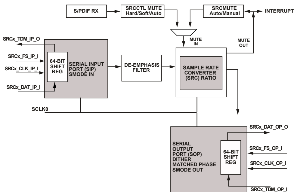
Figure 25-1: ASRC Block Diagram
