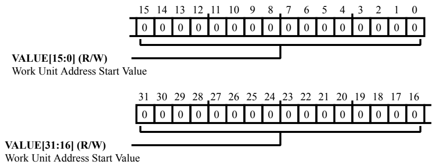
Figure 27-5: DMA_ADDRSTART Register Diagram
