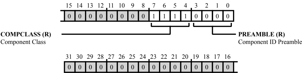
Figure 43-5: MEC_CID1 Register Diagram
