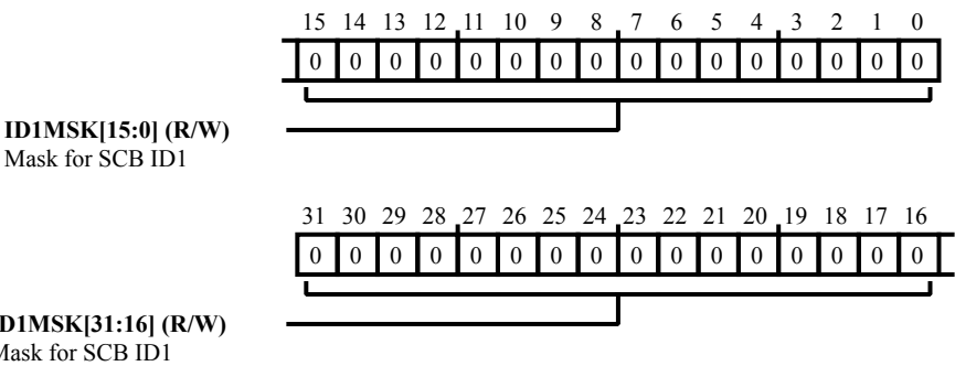
Figure 9-23: DMC_PRIOMSK Register Diagram
