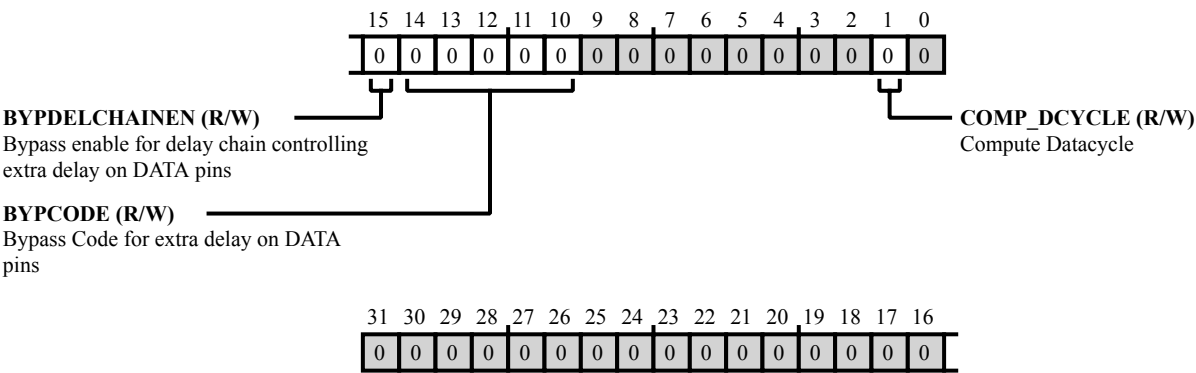
Figure 9-40: DMC_DDR_LANE0_CTL1 Register Diagram
