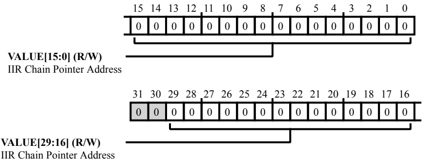
Figure 39-8: IIR_CHNPTR Register Diagram
