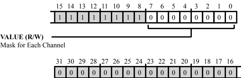
Figure 30-5: HADC_CHAN_MSK Register Diagram
