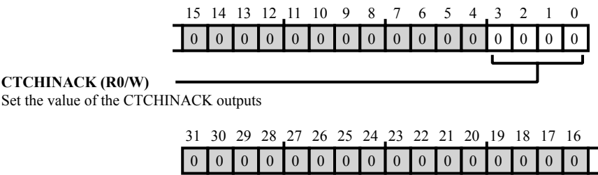
Figure 44-84: CTI_ITCHINACK Register Diagram
