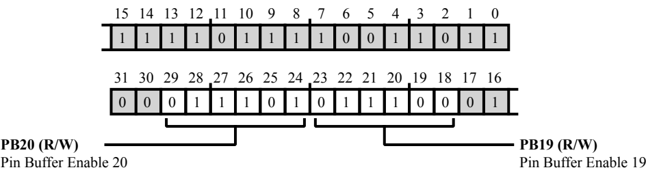
Figure 22-48: DAI_PBEN3 Register Diagram
