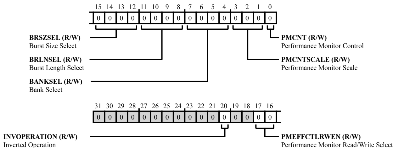
Figure 9-13: DMC_PM_CTL Register Diagram
