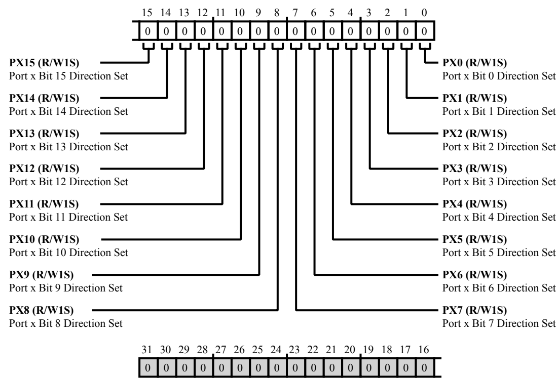
Figure 12-13: PORT_DIR_SET Register Diagram
