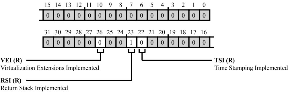
Figure 44-7: CSPFT_CCER Register Diagram
