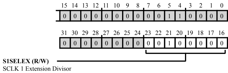
Figure 2-8: CGU_DIVEX Register Diagram
