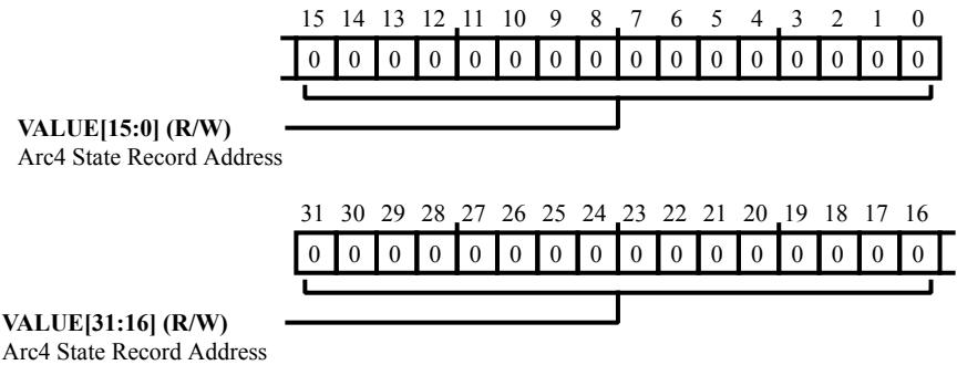
Figure 33-4: PKTE_ARC4STATE_ADDR Register Diagram
