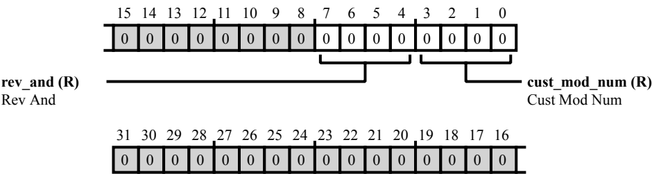
Figure 41-153: SCB5_PERIPH_ID_3 Register Diagram
