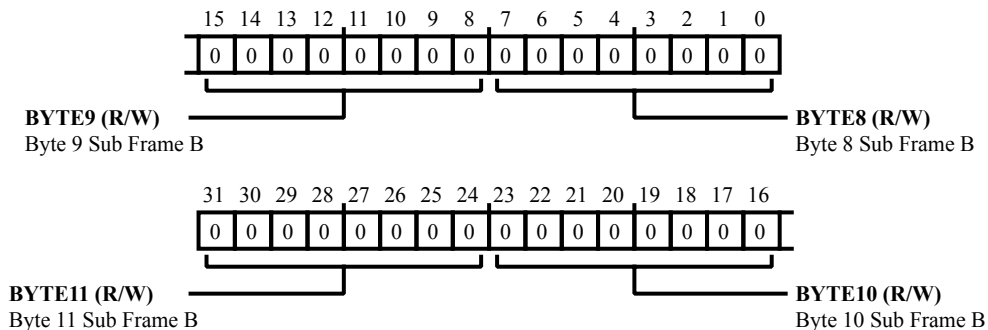
Figure 26-35: SPDIF_TX_UBUFF_B2 Register Diagram
