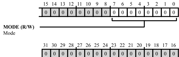
Figure 16-17: OSPI_MBCTL Register Diagram
