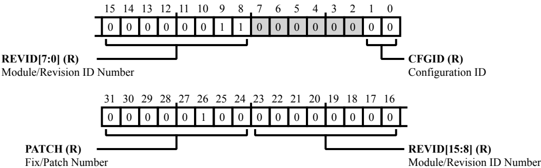
Figure 16-18: OSPI_MODID Register Diagram
