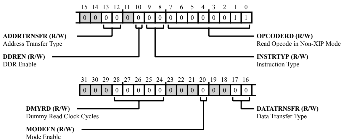
Figure 16-4: OSPI_DRICTL Register Diagram
