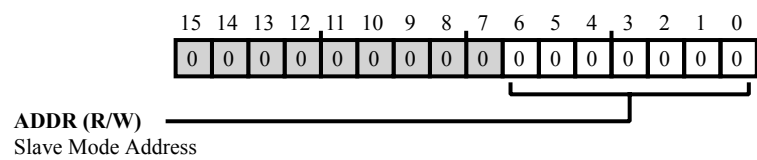
Figure 21-25: TWI_SLVADDR Register Diagram
