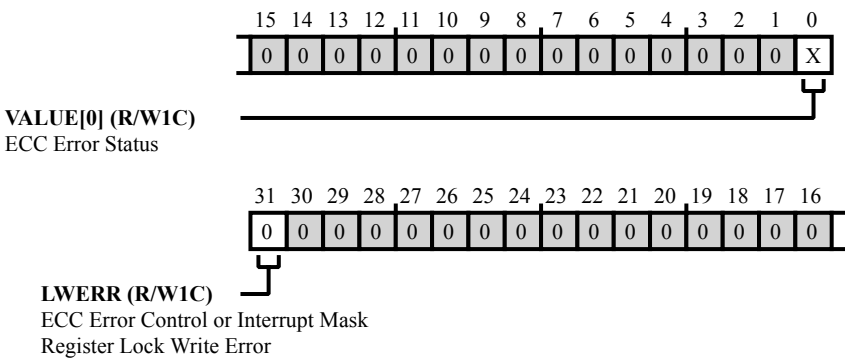
Figure 43-11: MEC_ECCERR_STAT[y] Register Diagram
