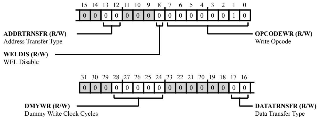
Figure 16-5: OSPI_DWICTL Register Diagram
