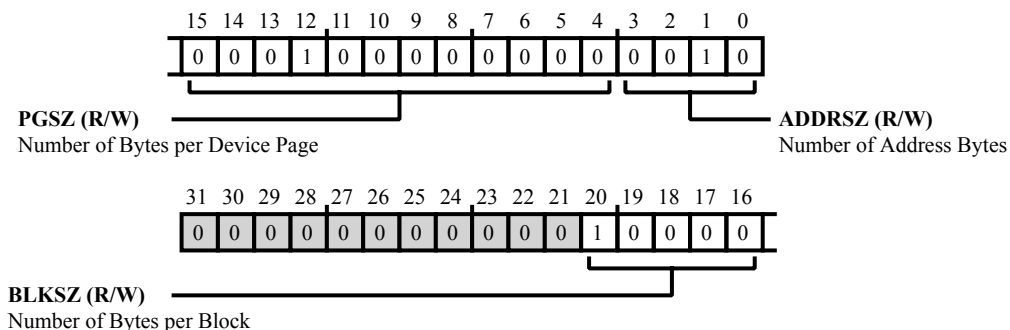
Figure 16-6: OSPI_DSCTL Register Diagram
