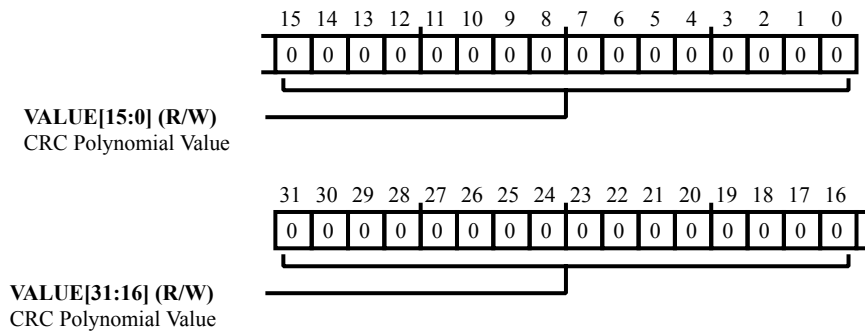
Figure 29-13: CRC_POLY Register Diagram
