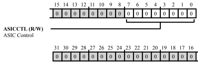
Figure 44-47: CTI_ASICCTL Register Diagram
