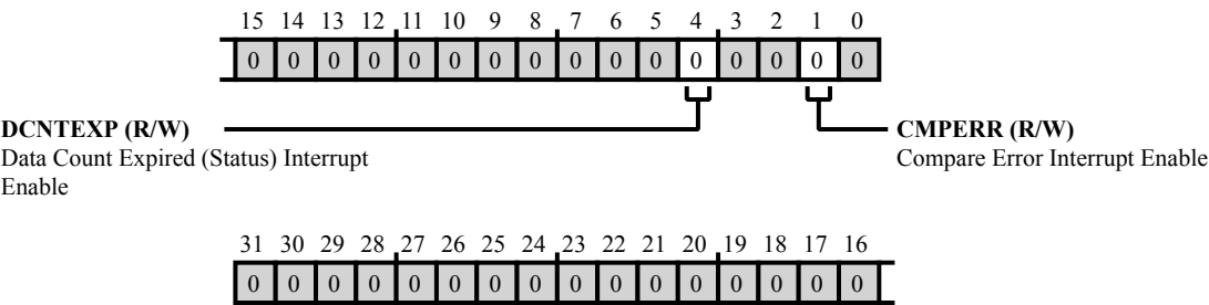
Figure 29-10: CRC_INEN Register Diagram
