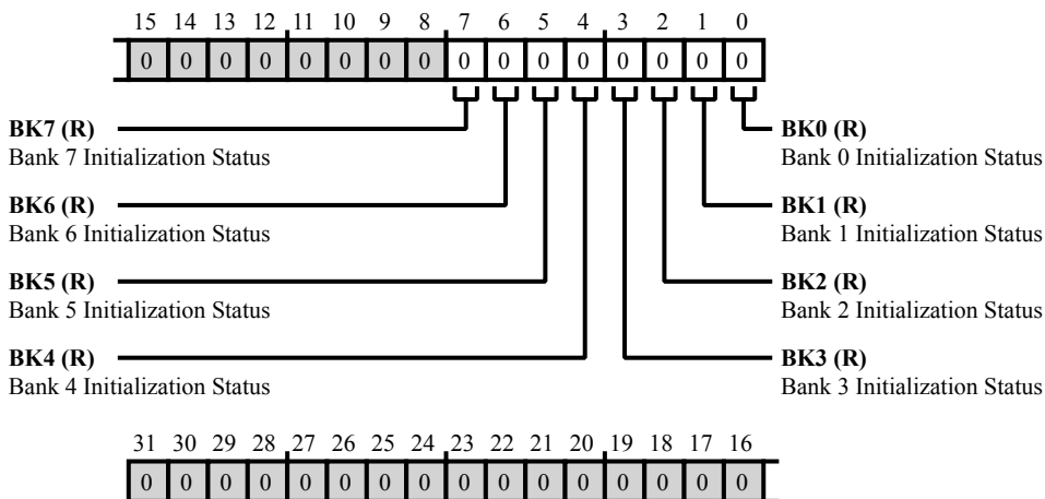
Figure 8-20: L2CTL_ISTAT Register Diagram
