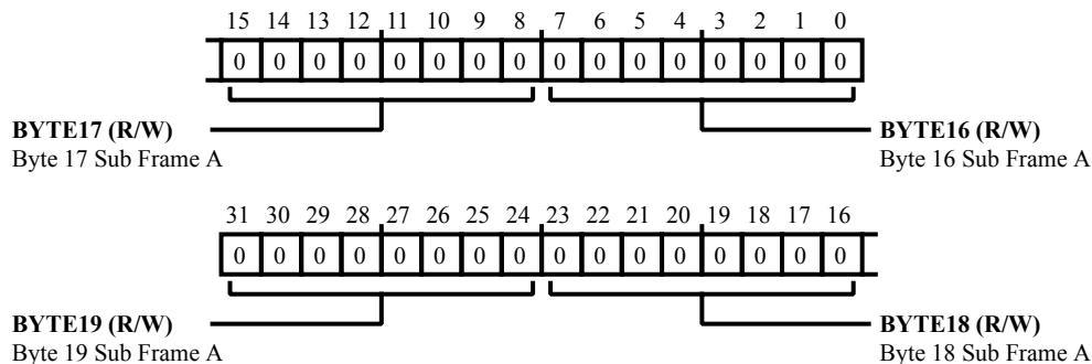
Figure 26-31: SPDIF_TX_UBUFF_A4 Register Diagram
