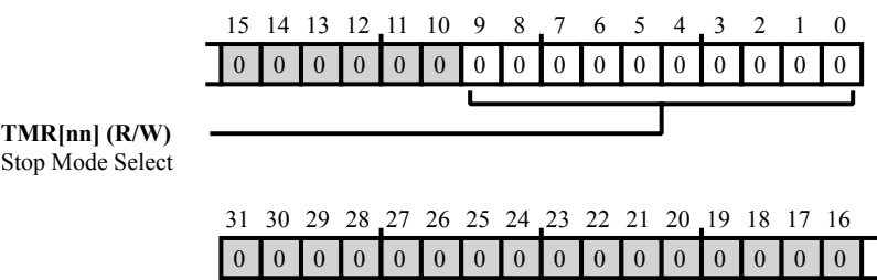
Figure 18-23: TIMER_STOP_CFG_CLR Register Diagram
