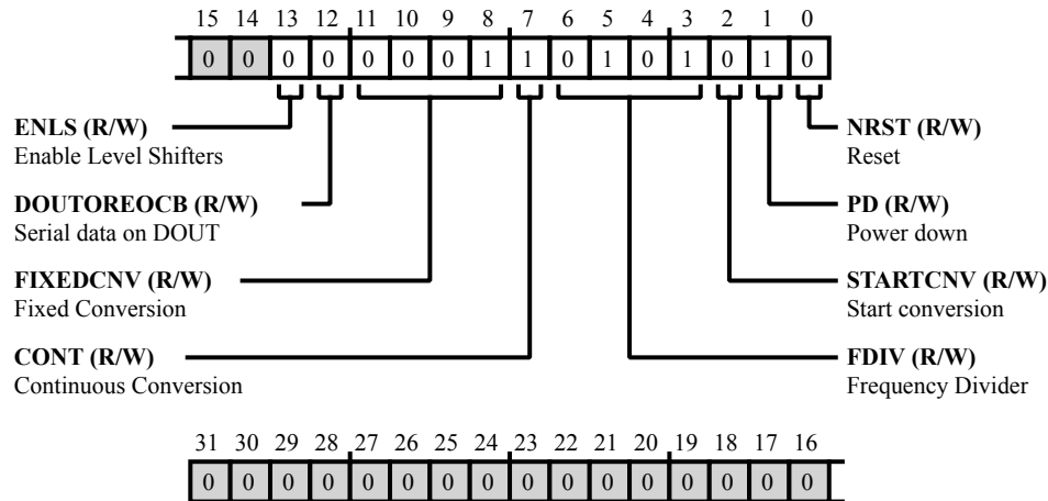
Figure 30-6: HADC_CTL Register Diagram
