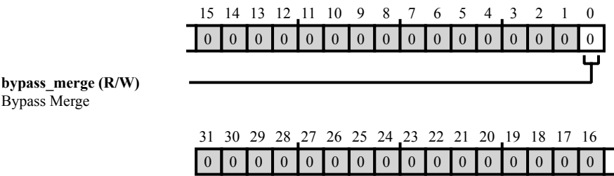
Figure 41-128: SCB4_IIR_CH0_IB_FN_MOD2 Register Diagram
