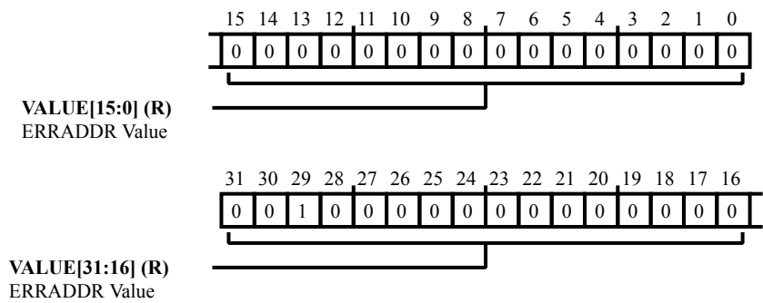
Figure 8-8: L2CTL_ERRADDR0 Register Diagram
