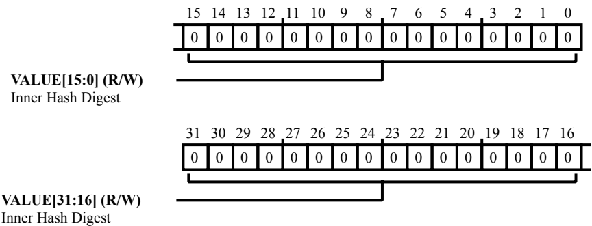
Figure 33-44: PKTE_SA_IDIGEST[n] Register Diagram
