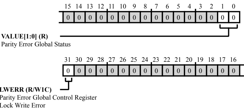
Figure 43-15: MEC_PEIRQ_GSTAT[p] Register Diagram
