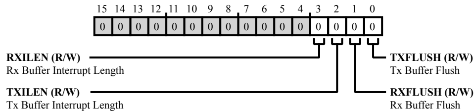
Figure 21-16: TWI_FIFOCCTL Register Diagram
