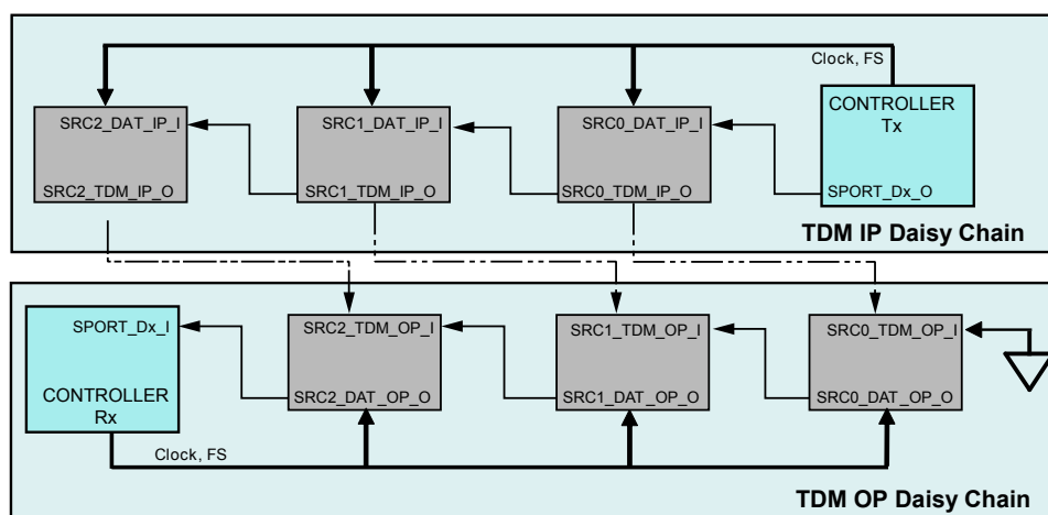
Figure 25-4: TDM Input/Output Modes
