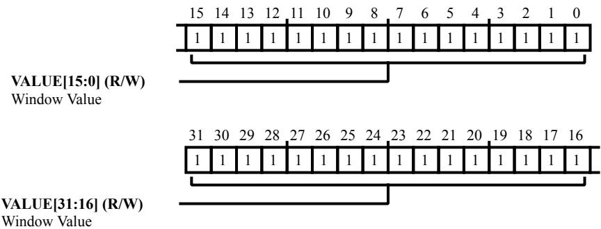
Figure 13-5: WDOG_WIN Register Diagram
