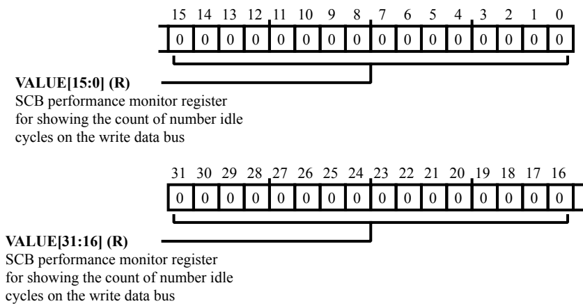
Figure 9-33: DMC_SCB_PM_IDWRDCY_CNT Register Diagram
