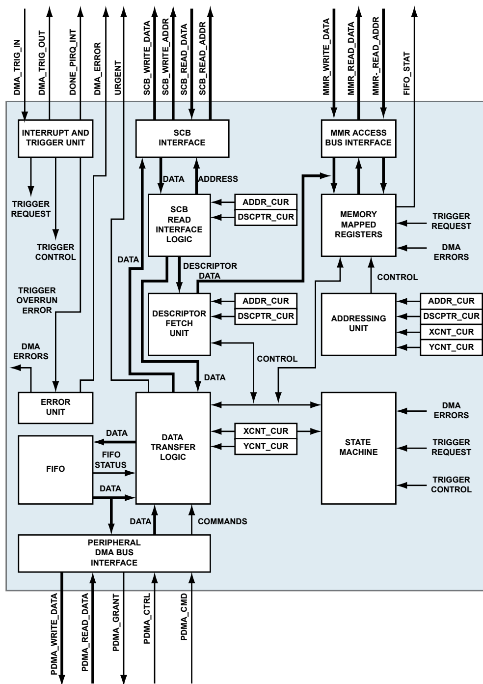
Figure 27-1: DMA Channel Block Diagram
