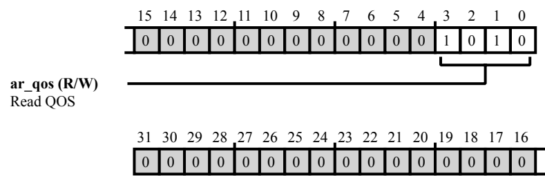
Figure 41-100: SCB0_UART0_TX_READ_QOS Register Diagram
