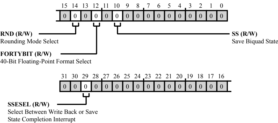
Figure 39-32: IIR_SGCTL Register Diagram
