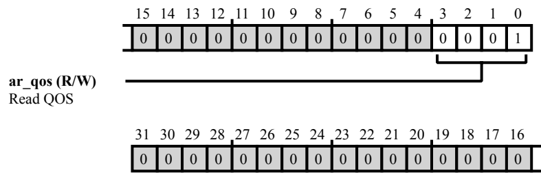
Figure 41-46: SCB0_MSMDMA_CH1_READ_QOS Register Diagram
