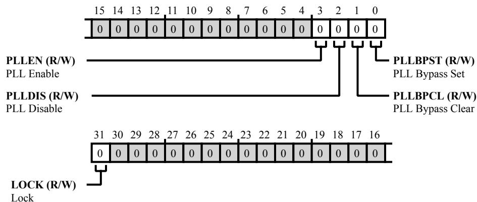
Figure 2-10: CGU_PLLCTL Register Diagram
