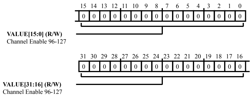
Figure 23-21: SPORT_CS3_B Register Diagram
