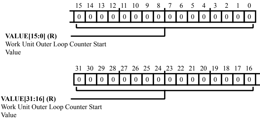
Figure 27-17: DMA_XCNT_CUR Register Diagram
