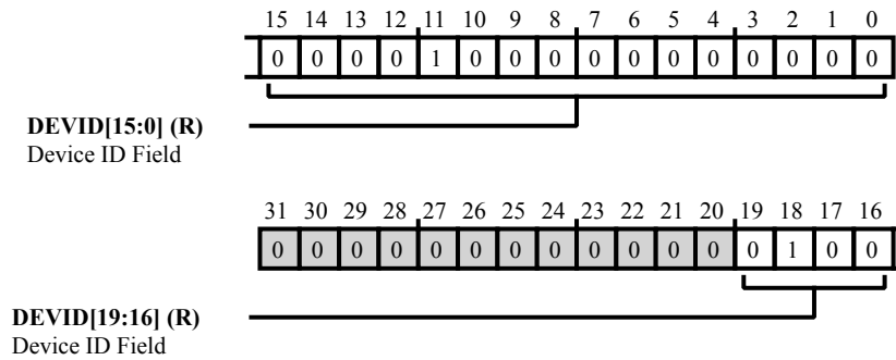
Figure 44-81: CTI_DEVID Register Diagram
