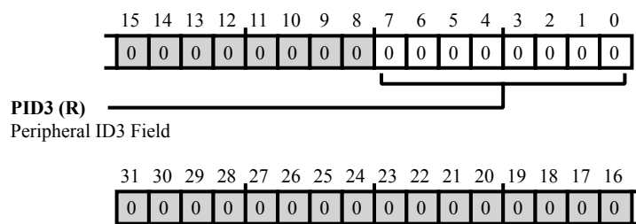
Figure 44-97: CTI_PERIPHID3 Register Diagram
