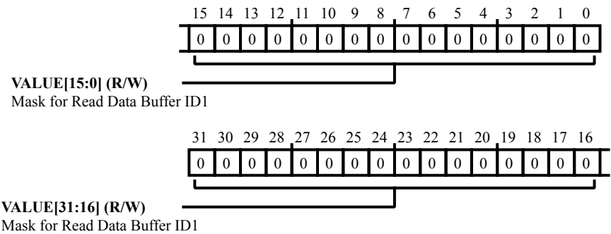
Figure 9-27: DMC_RDDATABUFMSK1 Register Diagram
