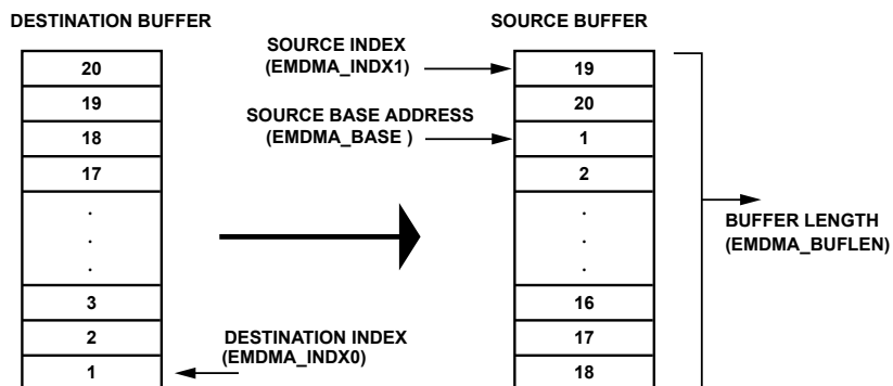
Figure 28-2: Circular Buffering Read DMA
