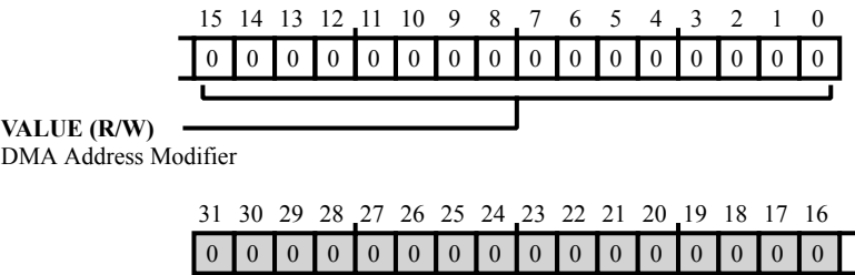
Figure 28-18: EMDMA_MOD0 Register Diagram
