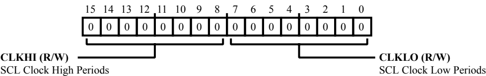
Figure 21-14: TWI_CLKDIV Register Diagram
