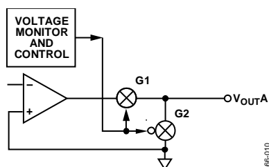
Figure 48. Analog Output Control Circuitry
