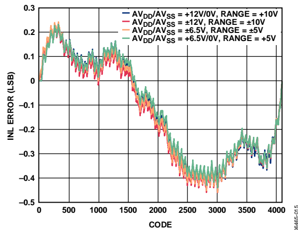
Figure 8. AD5724R Integral Nonlinearity Error vs. Code
