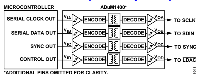
Figure 49. Isolated Interface
