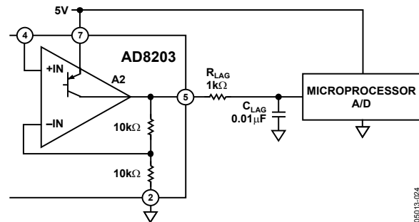
Figure 50. Recommended Circuit for Driving CMOS A/D
