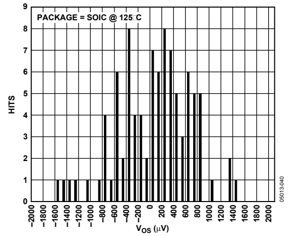
Figure 28. V OS Distribution, SOIC, Temperature = 125°C
