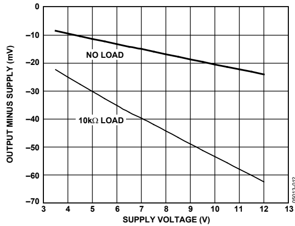
Figure 11. Swing Minus Supply vs. Supply Voltage
