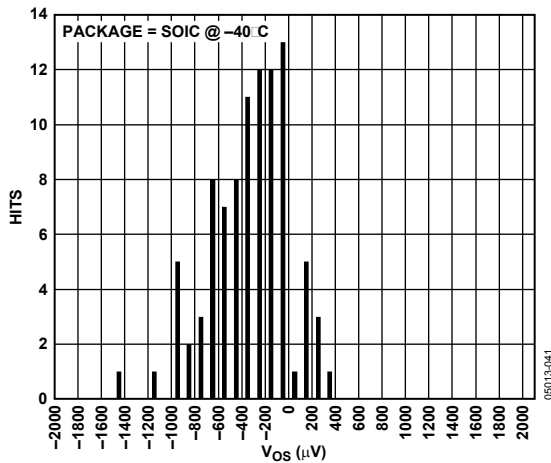
Figure 29. V_{OS} Distribution, SOIC, Temperature = -40^{\circ}\text{C}
