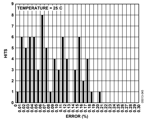
Figure 33. Gain Accuracy, SOIC, Temperature = 25^{\circ}\text{C}
