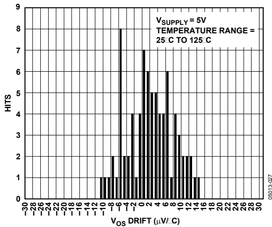
Figure 17. V_{OS} Distribution, MSOP, Temperature Range = 25°C to 125°C
