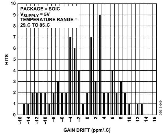
Figure 37. Gain Drift Distribution, SOIC, Temperature Range = 25°C to 85°C
