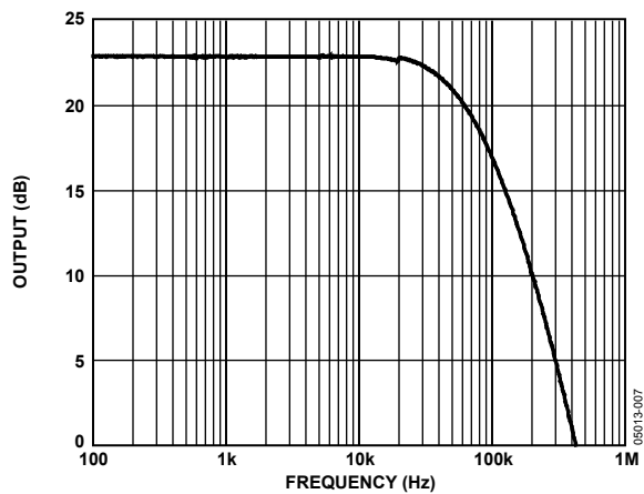
Figure 6. Bandwidth
