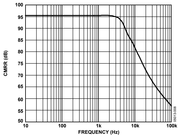
Figure 7. Common-Mode Rejection Ratio vs. Frequency for Common-Mode Range -6\text{ V} to +30\text{ V}
