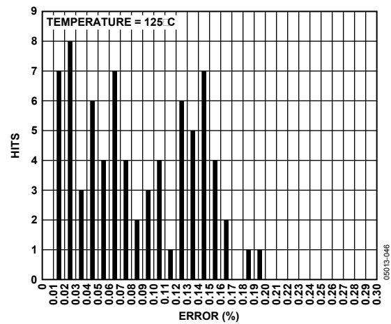
Figure 34. Gain Accuracy, SOIC, Temperature = 125^{\circ}\text{C}
