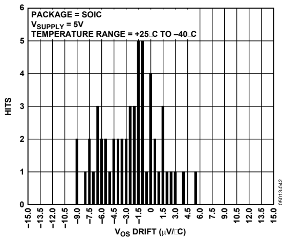
Figure 30. Offset Drift Distribution, SOIC, Temperature Range = +25^{\circ}\text{C} to -40^{\circ}\text{C}
