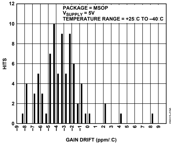
Figure 24. Gain Drift Distribution, Temperature Range = +25°C to -40°C
