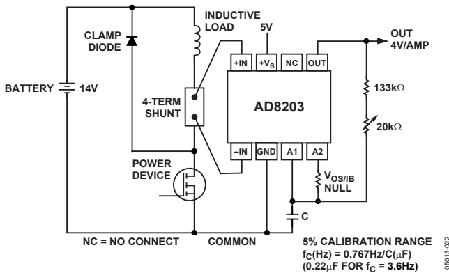
Figure 48. High Line Current Sensor Interface; Gain = \times 40 , Single-Pole Low-Pass Filter
