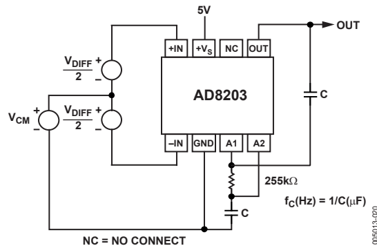
Figure 46. 2-Pole, Low-Pass Filter
