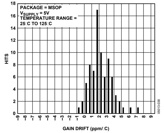
Figure 26. Gain Drift Distribution, MSOP, Temperature Range = 25°C to 125°C
