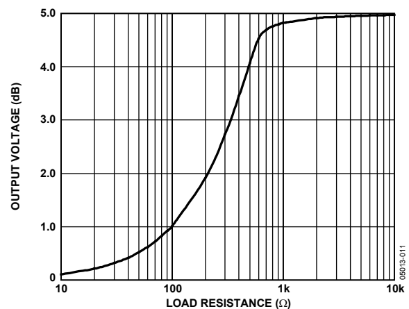
Figure 10. Output Swing vs. Load Resistance
