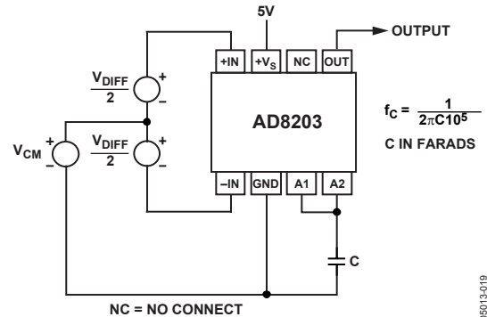
Figure 45. Single-Pole, Low-Pass Filter Using the Internal 100 \text{ k}\Omega Resistor
