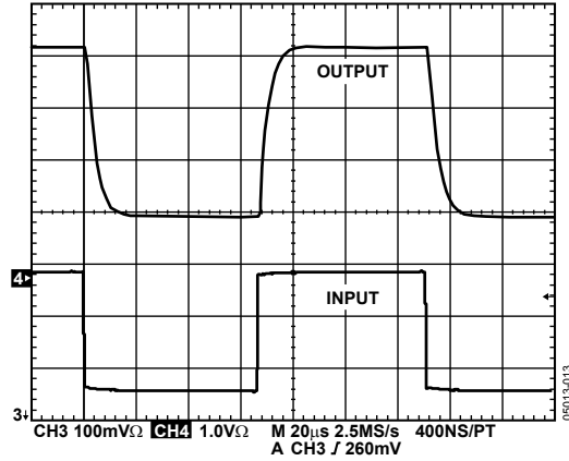
Figure 12. Pulse Response
