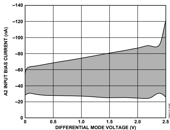
Figure 40. A2 Input Bias Current vs. Input Voltage and Temperature. The Shaded Area Is the Bias Current from -40^{\circ}\text{C} to +125^{\circ}\text{C} .
