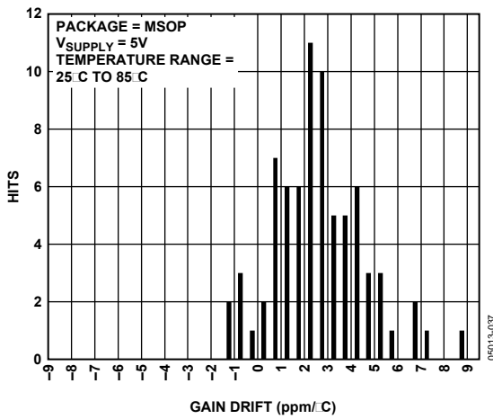
Figure 25. Gain Drift Distribution, MSOP, Temperature Range = 25°C to 85°C
