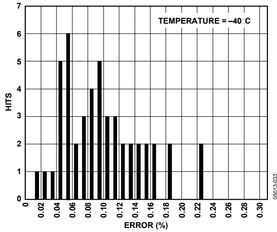
Figure 23. MSOP Gain Accuracy, Temperature = -40°C
