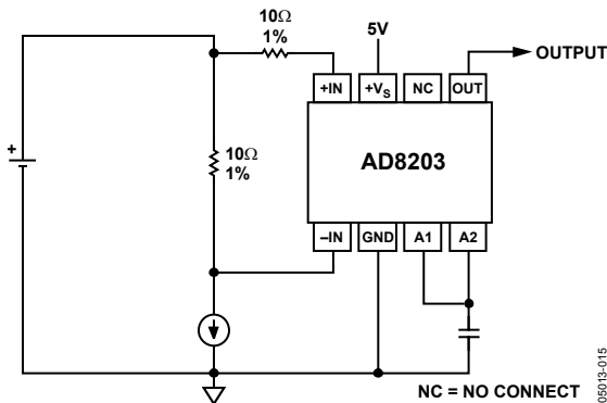
Figure 41. 4 to 20 mA Current Loop Receiver
