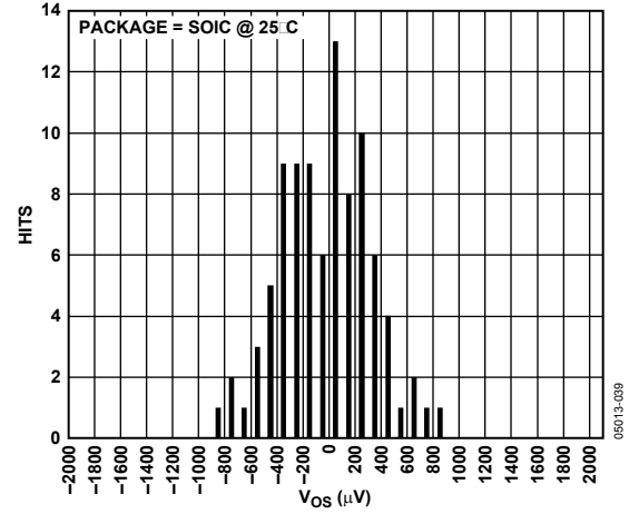
Figure 27. V OS Distribution, SOIC, Temperature = 25°C
