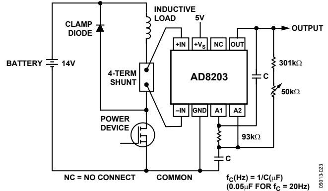
Figure 49. 2-Pole Low-Pass Filter
