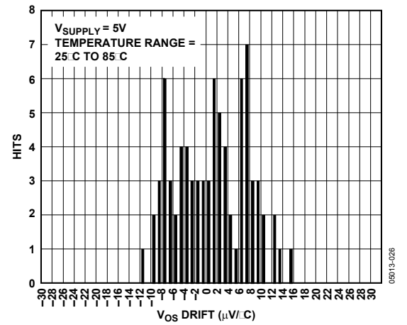
Figure 16. Offset Drift Distribution, MSOP, Temperature Range = 25°C to 85°C
