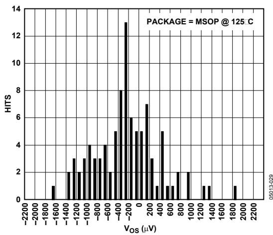
Figure 19. V_{OS} Distribution, MSOP, Temperature = 125°C
