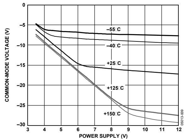
Figure 8. Negative Common-Mode Voltage vs. Voltage Supply
