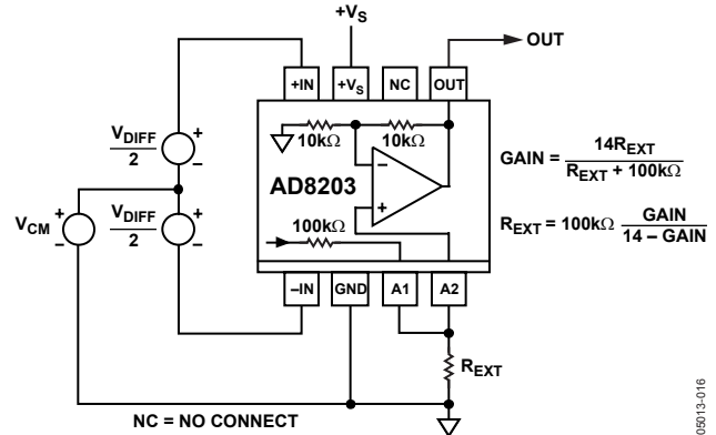
Figure 42. Adjusting for Gains < 14
