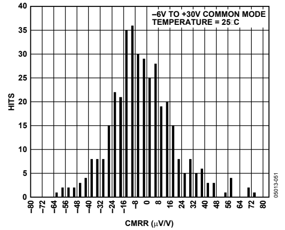
Figure 14. CMRR Distribution, Temperature = 25°C
