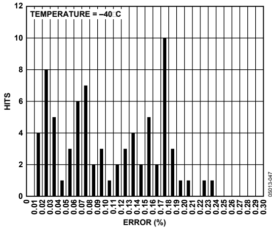
Figure 35. Gain Accuracy, SOIC, Temperature = -40°C
