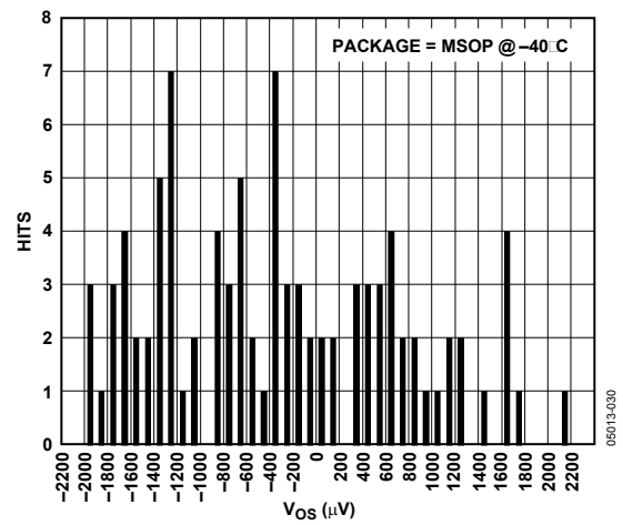
Figure 20. V_{OS} Distribution, MSOP, Temperature = -40°C
