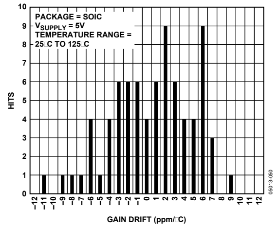
Figure 38. Gain Drift Distribution, SOIC, Temperature Range = 25°C to 125°C
