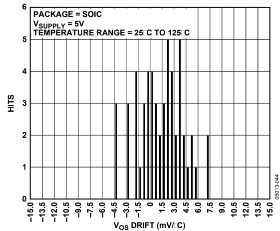
Figure 32. Offset Drift Distribution, SOIC, Temperature Range = +25^{\circ}\text{C} to 125^{\circ}\text{C}
