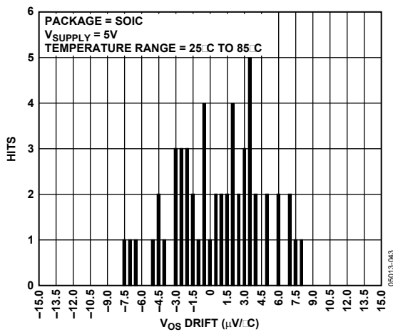
Figure 31. Offset Drift Distribution, SOIC, Temperature Range = 25^{\circ}\text{C} to 85^{\circ}\text{C}
