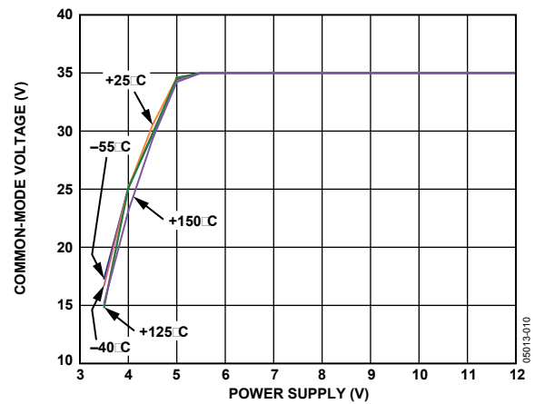
Figure 9. Positive Common-Mode Voltage vs. Voltage Supply
