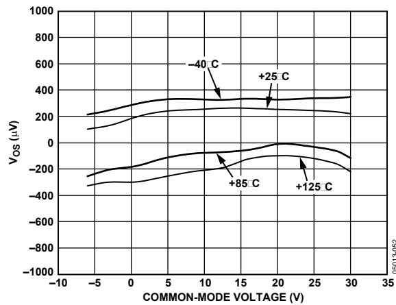
Figure 13. V_{OS} vs. Common-Mode Voltage
