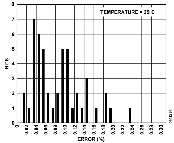
Figure 21. MSOP Gain Accuracy, Temperature = 25°C
