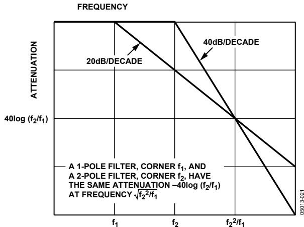
Figure 47. Comparative Responses of 1-Pole and 2-Pole Low-Pass Filters
