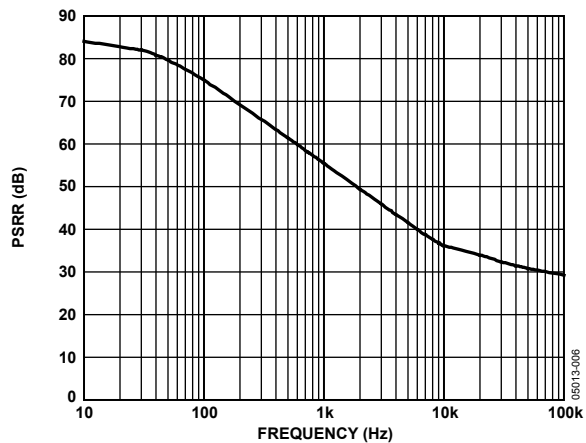
Figure 5. Power Supply Rejection Ratio vs. Frequency for Common-Mode Range -6\text{ V} to +30\text{ V}
