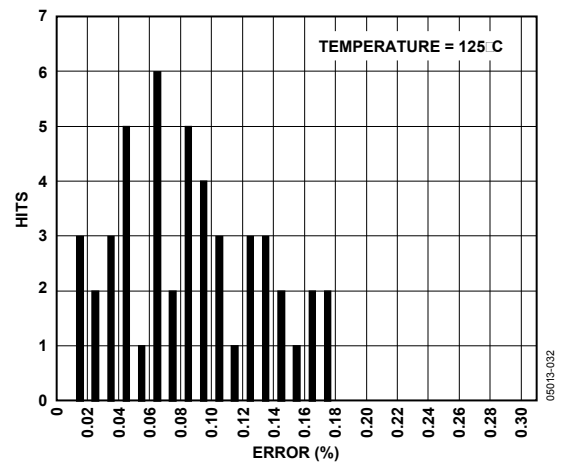
Figure 22. MSOP Gain Accuracy, Temperature = 125°C
