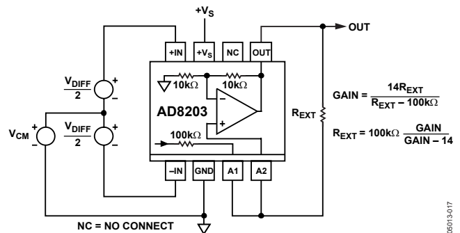
Figure 43. Adjusting for Gains > 14
