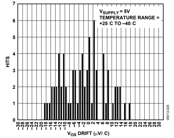
Figure 15. Offset Drift Distribution, MSOP, Temperature Range = +25°C to -40°C
