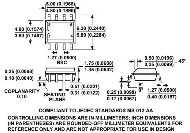
Figure 52. 8-Lead Standard Small Outline Package [SOIC_N] Narrow Body (R-8)
