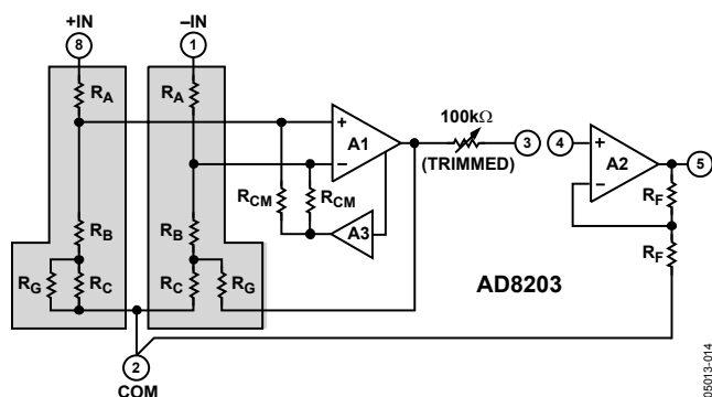
Figure 39. Simplified Schematic
