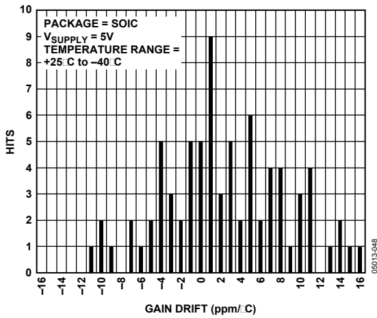
Figure 36. Gain Drift Distribution, SOIC, Temperature Range = +25°C to -40°C
