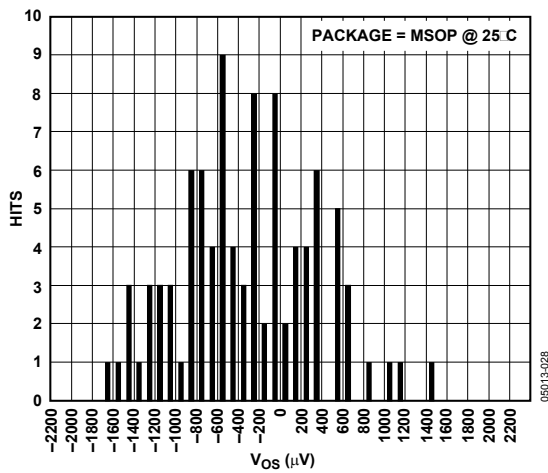
Figure 18. V_{OS} Distribution, MSOP, Temperature = 25°C
