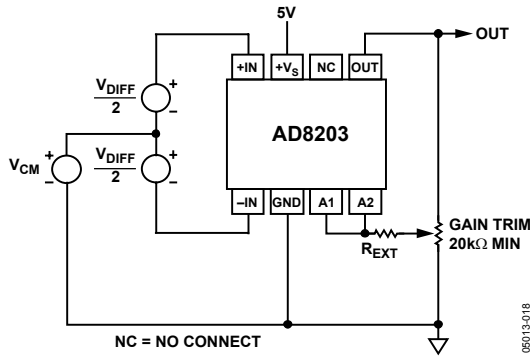
Figure 44. Incremental Gain Trim
