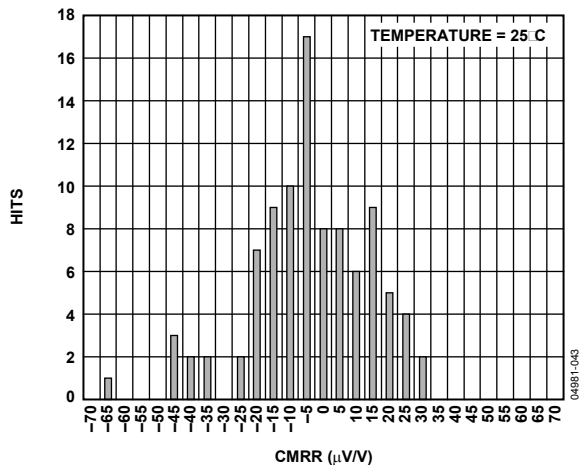
Figure 15. CMRR Distribution, -8\text{ V} to +28\text{ V} Common Mode
