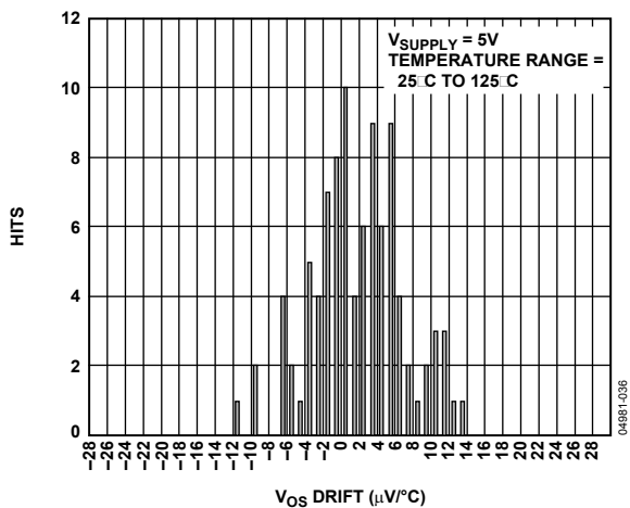
Figure 17. Offset Drift Distribution, MSOP, Temperature Range = 25^\circ\text{C} to 125^\circ\text{C}
