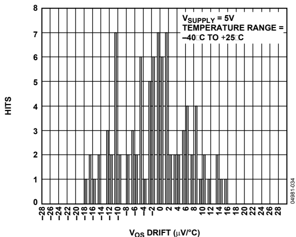
Figure 16. Offset Drift Distribution, MSOP, Temperature Range = -40^\circ\text{C} to +25^\circ\text{C}
