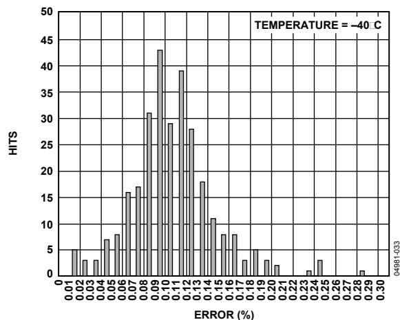
Figure 36. Gain Accuracy, SOIC, Temperature = -40°C
