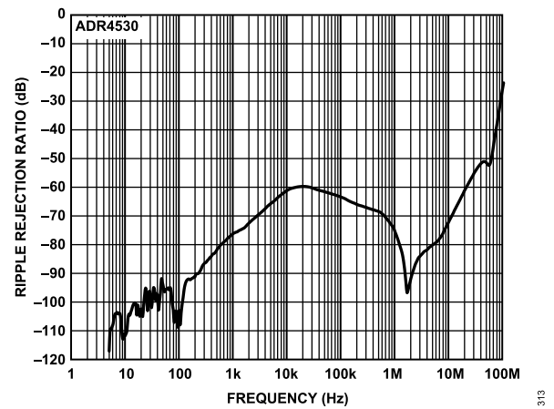
Figure 48. ADR4530 Ripple Rejection Ratio vs. Frequency
