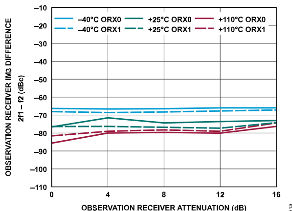
Figure 238. Observation Receiver IM3 Difference, 2f_1 - f_2 vs. Observation Receiver Attenuation, -13 dBFS Signal Level Per Tone, f_1 = 3502 MHz, f_2 = 3512 MHz
