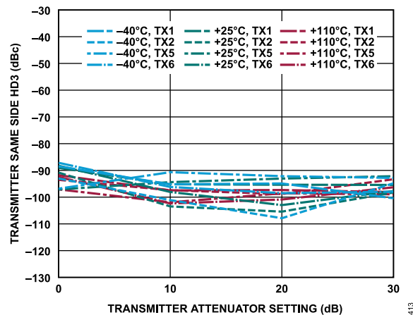
Figure 13. Transmitter Same Side HD3 vs. Transmitter Attenuator Setting, 30 MHz Offset, -12 dBFS Continuous Wave Signal
