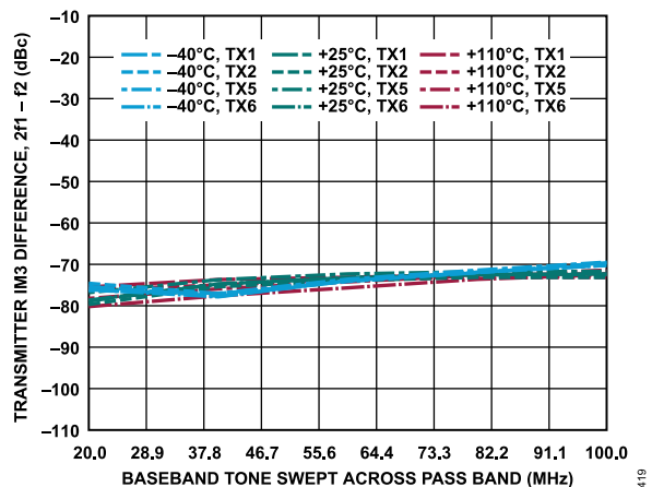
Figure 19. Transmitter IM3 Difference, 2f_1 - f_2 vs. Baseband Tone Swept Across Pass Band, -15 dBFS Signal Level Per Tone, f_2 = f_1 + 5 MHz
