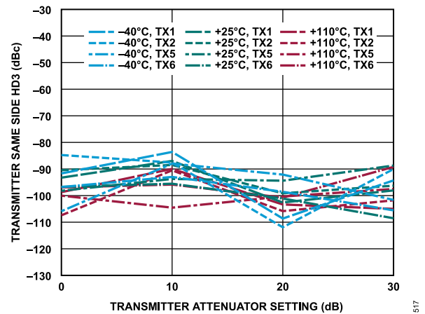
Figure 317. Transmitter Same Side HD3 vs. Transmitter Attenuator Setting, 110 MHz Offset, -12 dBFS Continuous Wave Signal
