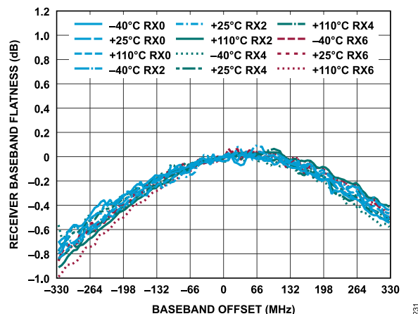
Figure 291. Receiver Baseband Flatness vs. Baseband Offset
