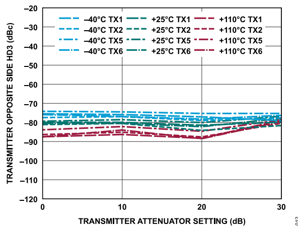
Figure 73. Transmitter Opposite Side Third Harmonic Distortion (HD3) vs. Transmitter Attenuation Setting, 30 MHz Offset, -12 dBFS Continuous Wave Signal
