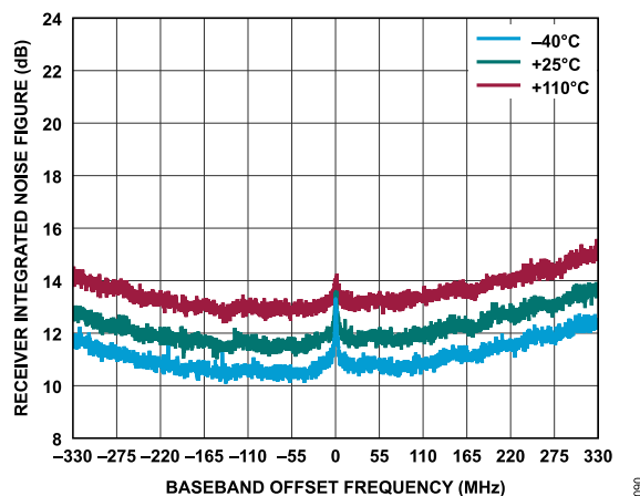
Figure 150. Receiver Integrated Noise Figure vs. Baseband Offset Frequency, 200 kHz Integration Steps, 983.04 MSPS Sample Rate
