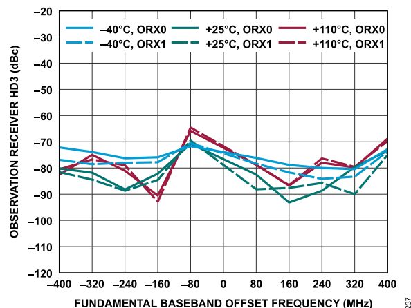
Figure 297. Observation Receiver HD3 vs. Fundamental Baseband Offset Frequency, -10 dBFS Input Signal
