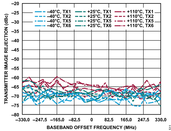
Figure 311. Transmitter Image Rejection vs. Baseband Offset Frequency, -6 dBFS Continuous Wave Signal
