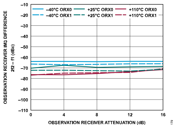
Figure 239. Observation Receiver IM3 Difference, 2f_2 - f_1 vs. Observation Receiver Attenuation, -13 dBFS Signal Level Per Tone, f_1 = 3502 MHz, f_2 = 3512 MHz
