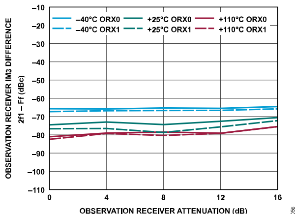
Figure 116. Observation Receiver IM3 Difference, 2f_1 - f_2 vs. Observation Receiver Attenuation, -13 dBFS Signal Level Per Tone, f_1 = 1802 MHz, f_2 = 1812 MHz
