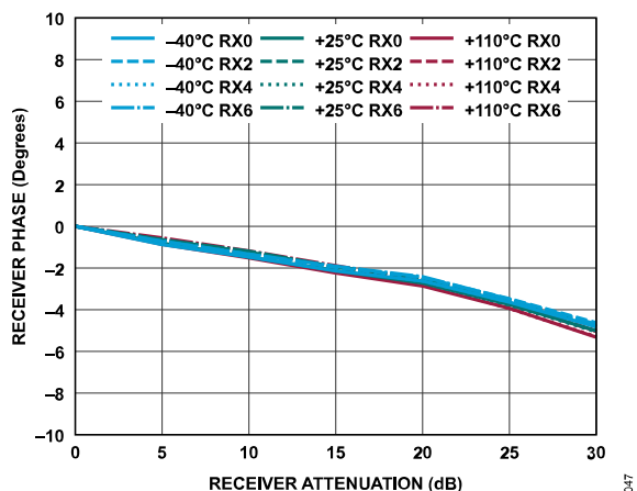
Figure 107. Receiver Phase vs. Receiver Attenuation
