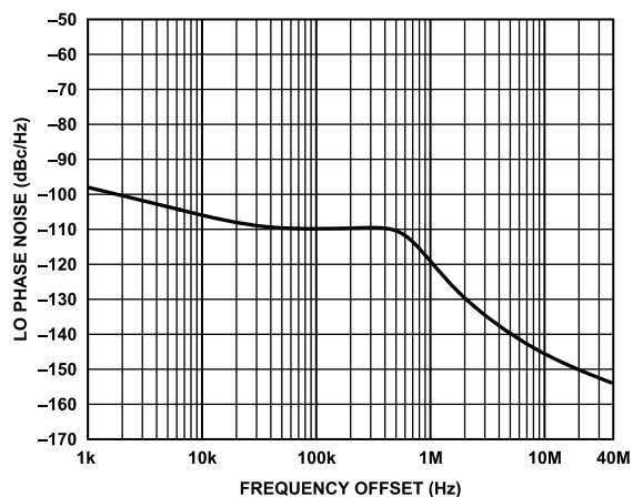
Figure 354. LO Phase Noise vs. Frequency Offset, Loop Bandwidth = 500 kHz, Phase Margin = 55°
