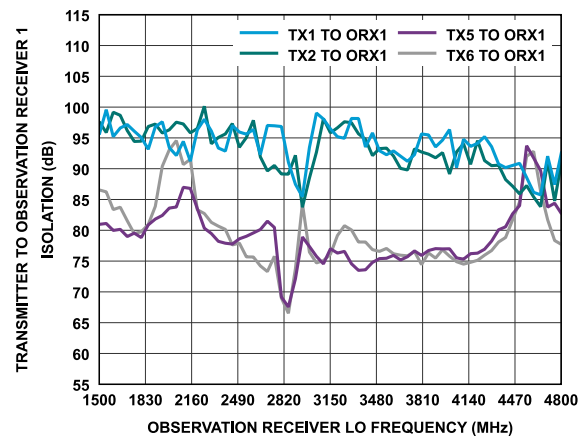
Figure 383. Transmitter to Observation Receiver 1 Isolation vs. Observation Receiver LO Frequency
