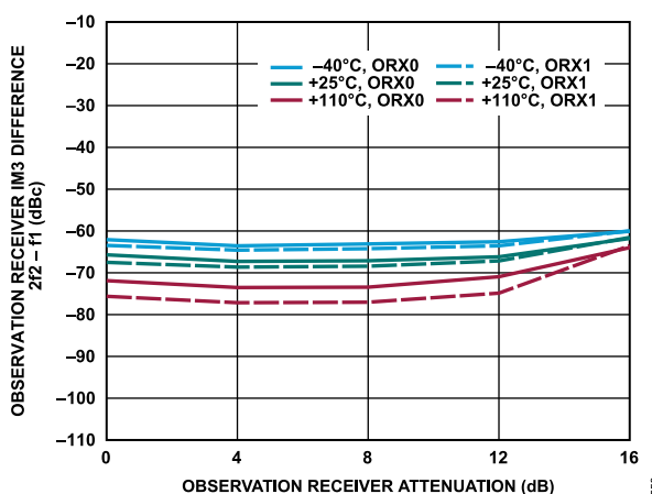
Figure 359. Observation Receiver IM3, 2f_2 - f_1 vs. Observation Receiver Attenuation, -13 dBFS Signal Level Per Tone, f_1 = 3502 MHz, f_2 = 3512 MHz
