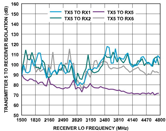
Figure 380. Transmitter 5 to Receiver Isolation vs. Receiver LO Frequency
