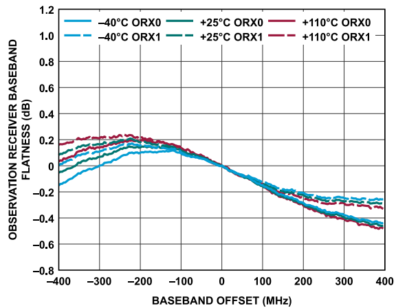
Figure 173. Observation Receiver Baseband Flatness vs. Baseband Offset
