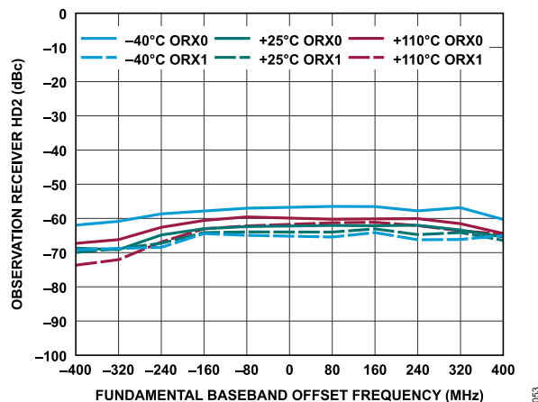
Figure 113. Observation Receiver HD2 vs. Fundamental Baseband Offset Frequency, -10 dBFS Input Signal
