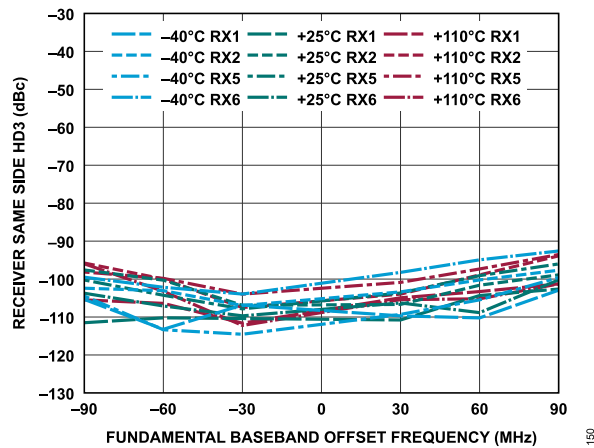
Figure 210. Receiver Same Side HD3 vs. Fundamental Baseband Offset Frequency, -1 dBFS Input Signal
