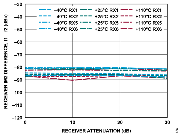
Figure 216. Receiver IM2 Difference, f_1 - f_2 vs. Receiver Attenuation, -7 dBFS Signal Level Per Tone, f_1 = 42 MHz Offset, f_2 = 2 MHz Offset
