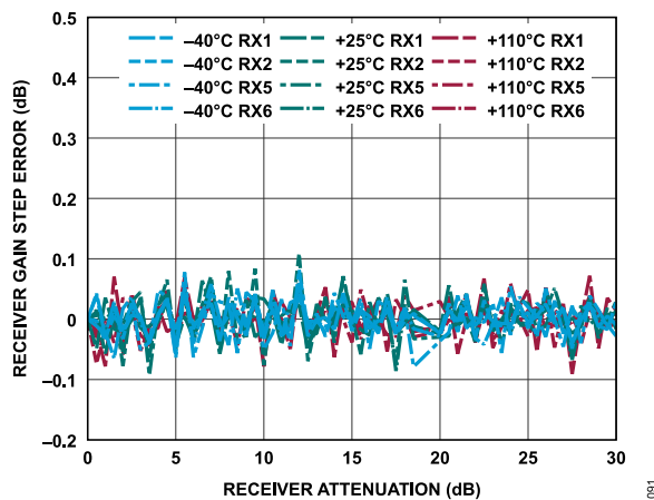
Figure 151. Receiver Gain Step Error vs. Receiver Attenuation, 30 MHz Offset, -1 dBFS Input Signal
