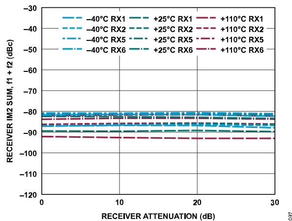
Figure 157. Receiver IM2 Sum, f_1 + f_2 vs. Receiver Attenuation, -7 dBFS Signal Level Per Tone, f_1 = 42 MHz Offset, f_2 = 2 MHz Offset
