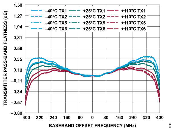
Figure 126. Transmitter Pass-Band Flatness vs. Baseband Offset Frequency
