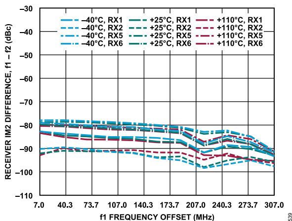
Figure 339. Receiver IM2 Difference, f_1 - f_2 vs. f_1 Frequency Offset, -7 dBFS Signal Level Per Tone, f_2 = 2 MHz
