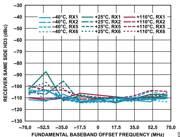
Figure 28. Receiver Same Side HD3 vs. Fundamental Baseband Offset Frequency, -1 dBFS Input Signal
