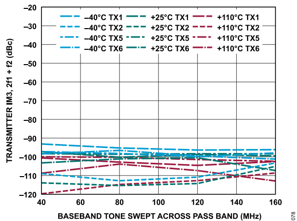
Figure 138. Transmitter IM3, 2f_1 + f_2 vs. Baseband Tone Swept Across Pass Band, -15 dBFS Signal Level Per Tone, f_2 = f_1 + 5 MHz
