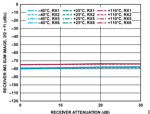
Figure 44. Receiver IM3 Sum Image, 2f_2 + f_1 vs. Receiver Attenuation, -7 dBFS Signal Level Per Tone, f_1 = 99 MHz Offset, f_2 = 2 MHz Offset
