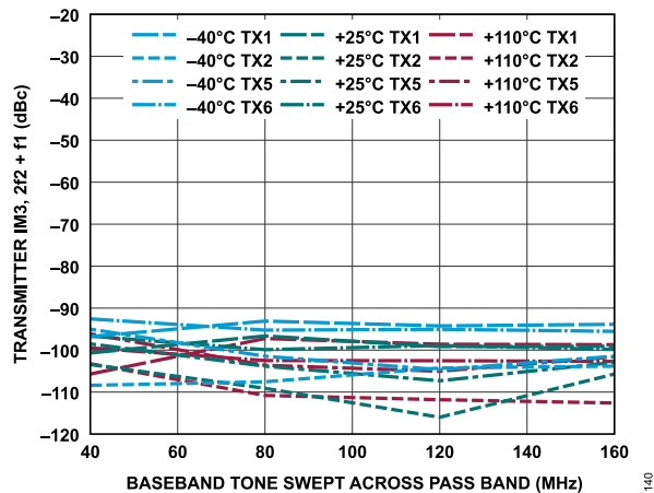
Figure 200. Transmitter IM3, 2f_2 + f_1 vs. Baseband Tone Swept Across Pass Band, -15 dBFS Signal Level Per Tone, f_2 = f_1 + 5 MHz
