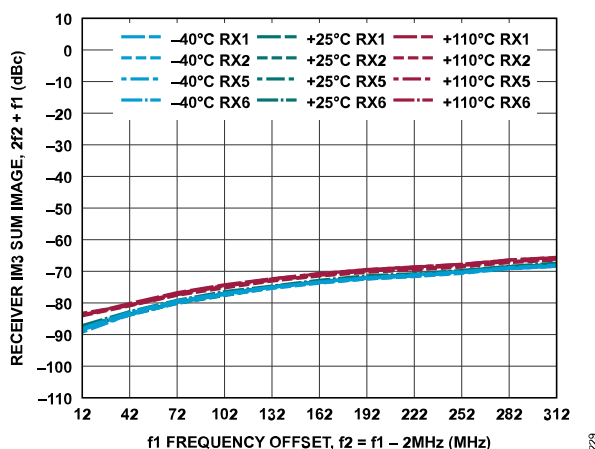
Figure 289. Receiver IM3 Sum Image, 2f_2 + f_1 vs. f_1 Frequency Offset, -7 dBFS Signal Level Per Tone, f_2 = f_1 - 2 MHz
