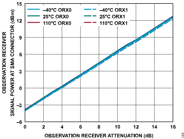
Figure 185. Observation Receiver Signal Power at SMA Connector vs. Observation Receiver Attenuation, 80 MHz Offset, -10 dBFS Input Signal
