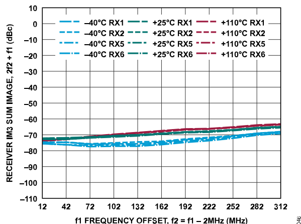
Figure 106. Receiver IM3 Sum Image, 2f_2 + f_1 vs. f_1 Frequency Offset, -7 dBFS Signal Level Per Tone, f_2 = f_1 - 2 MHz
