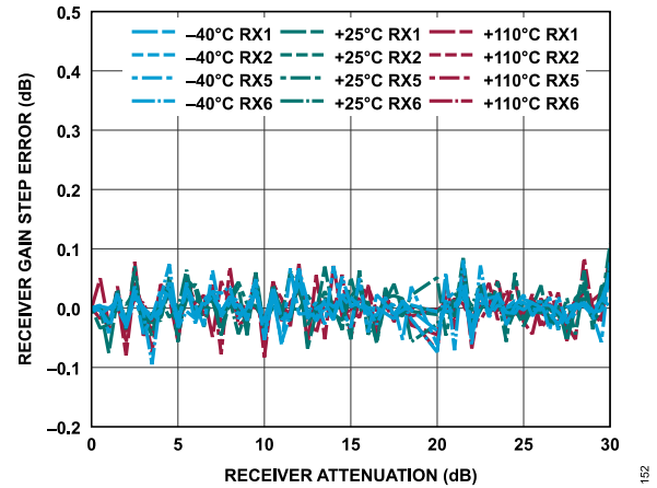
Figure 212. Receiver Gain Step Error vs. Receiver Attenuation, 30 MHz Offset, -1 dBFS Input Signal
