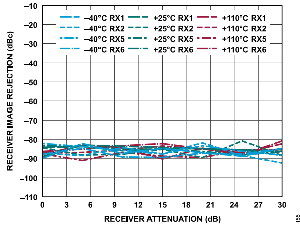
Figure 215. Receiver Image Rejection vs. Receiver Attenuation, 30 MHz Offset, -1 dBFS Input Signal
