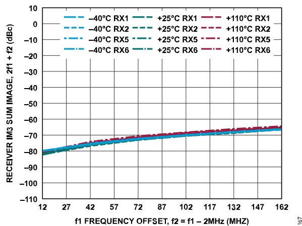
Figure 227. Receiver IM3 Sum Image, 2f_1 + f_2 vs. f_1 Frequency Offset, -7 dBFS Signal Level Per Tone, f_2 = f_1 - 2 MHz
