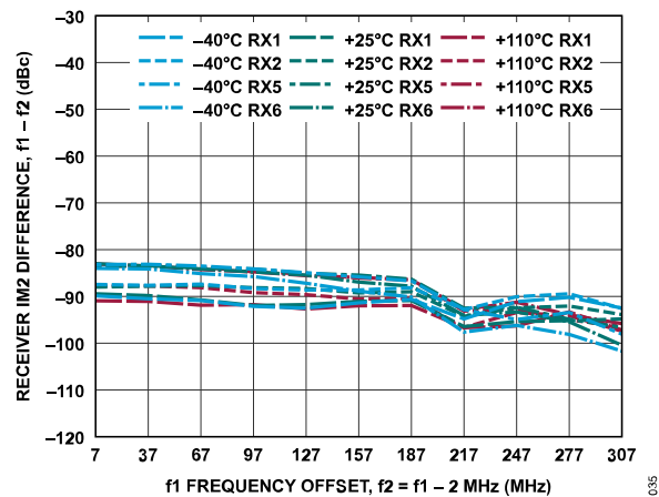
Figure 96. Receiver IM2 Difference, f_1 - f_2 vs. f_1 Frequency Offset, -7 dBFS Signal Level per Tone, f_2 = f_1 - 2 MHz
