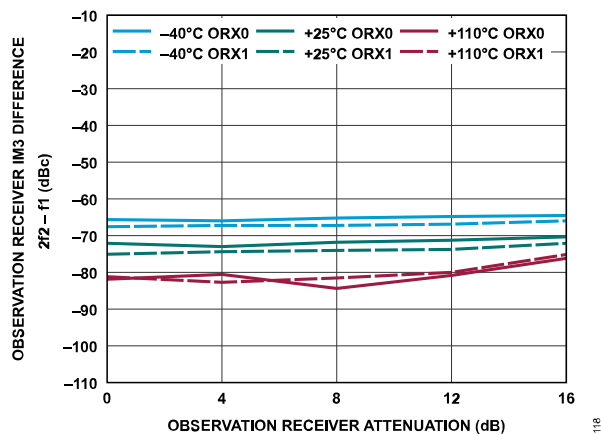
Figure 178. Observation Receiver IM3 Difference, 2f_2 - f_1 vs. Observation Receiver Attenuation, -13 dBFS Signal Level Per Tone, f_1 = 2602 MHz, f_2 = 2612 MHz
