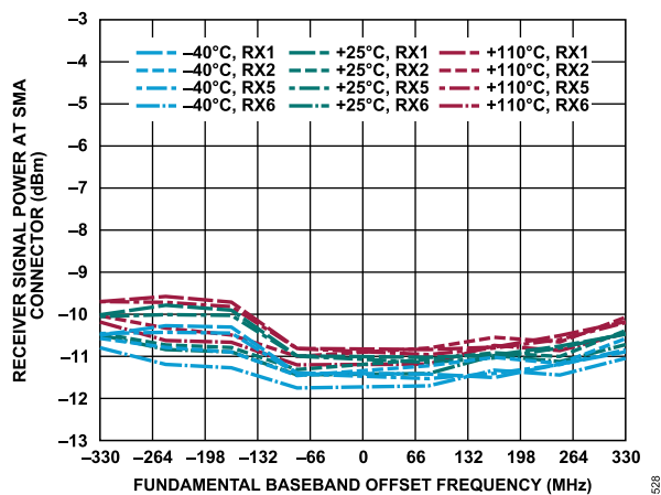
Figure 328. Receiver Signal Power at SMA Connector vs. Fundamental Baseband Offset Frequency, -1 dBFS Input Signal (Match Is Not De-Embedded)
