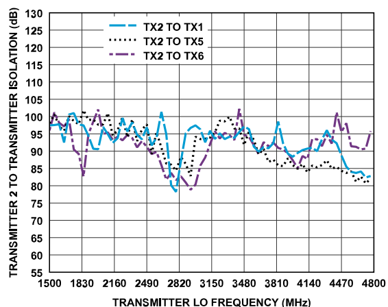
Figure 375. Transmitter 2 to Transmitter Isolation vs. Transmitter LO Frequency
