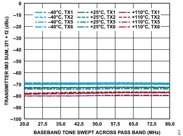
Figure 17. Transmitter IM3 Sum, 2f_1 + f_2 vs. Baseband Tone Swept Across Pass Band, -15 dBFS Signal Level Per Tone, f_2 = f_1 + 5 MHz
