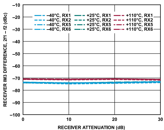
Figure 39. Receiver IM3 Difference, 2f_1 - f_2 vs. Receiver Attenuation, -7 dBFS Signal Level Per Tone, f_1 = 101 MHz Offset, f_2 = 2 MHz Offset
