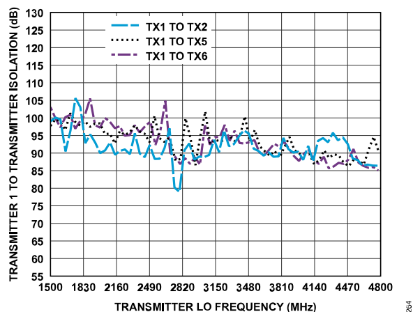
Figure 374. Transmitter 1 to Transmitter Isolation vs. Transmitter LO Frequency
