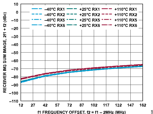
Figure 288. Receiver IM3 Sum Image, 2f_1 + f_2 vs. f_1 Frequency Offset, -7 dBFS Signal Level Per Tone, f_2 = f_1 - 2 MHz
