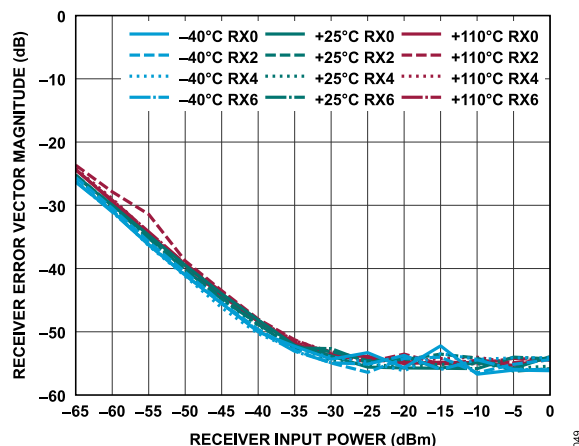
Figure 109. Receiver Error Vector Magnitude vs. Receiver Input Power, 20 MHz LTE Centered Around DC, TDD Mode, AGC Enabled
