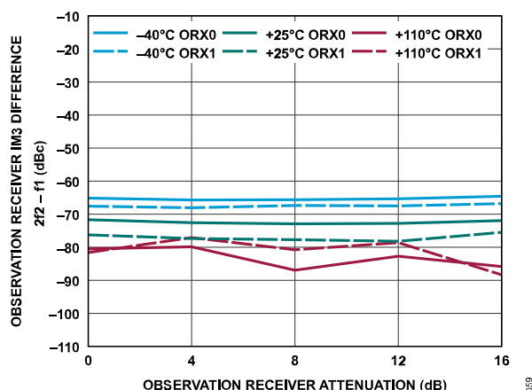
Figure 119. Observation Receiver IM3 Difference, 2f_2 - f_1 vs. Observation Receiver Attenuation, -13 dBFS Signal Level per Tone, f_1 = 1802 MHz, f_2 = 2012 MHz
