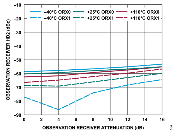
Figure 244. Observation Receiver HD2 vs. Observation Receiver Attenuation, 80 MHz Offset, -10 dBFS Input Signal
