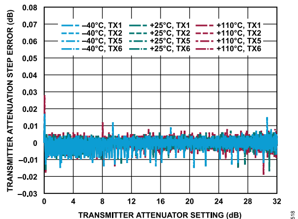
Figure 318. Transmitter Attenuation Step Error vs. Transmitter Attenuator Setting, 30 MHz Offset, -12 dBFS Continuous Wave Signal
