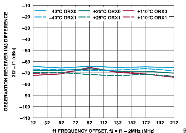
Figure 304. Observation Receiver IM3 Difference, 2f_2 - f_1 vs. f_1 Frequency Offset, -13 dBFS Signal Level Per Tone, f_2 = f_1 - 2 MHz
