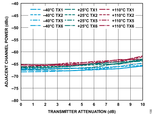
Figure 190. Adjacent Channel Power vs. Transmitter Attenuation, 290 MHz Offset, 20 MHz LTE, PAR = 12 dB
