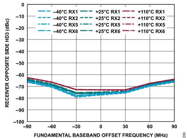
Figure 269. Receiver Opposite Side HD3 vs. Fundamental Baseband Offset Frequency, -1 dBFS Input Signal
