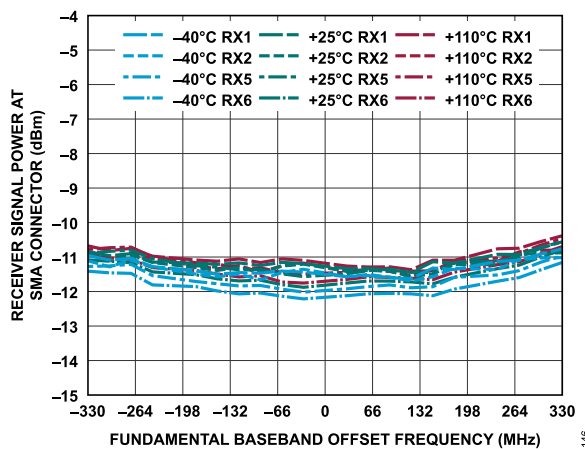
Figure 206. Receiver Signal Power at SMA Connector vs. Fundamental Baseband Offset Frequency, -1 dBFS Input Signal (Match Is Not De-Embedded)
