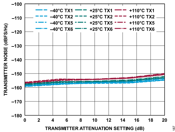
Figure 247. Transmitter Noise vs. Transmitter Attenuation, 150 MHz Offset
