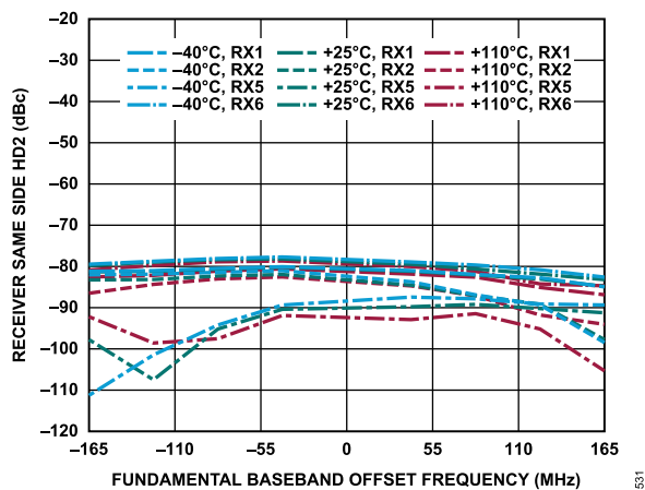
Figure 331. Receiver Same Side HD2 vs. Fundamental Baseband Offset Frequency, -1 dBFS Input Signal
