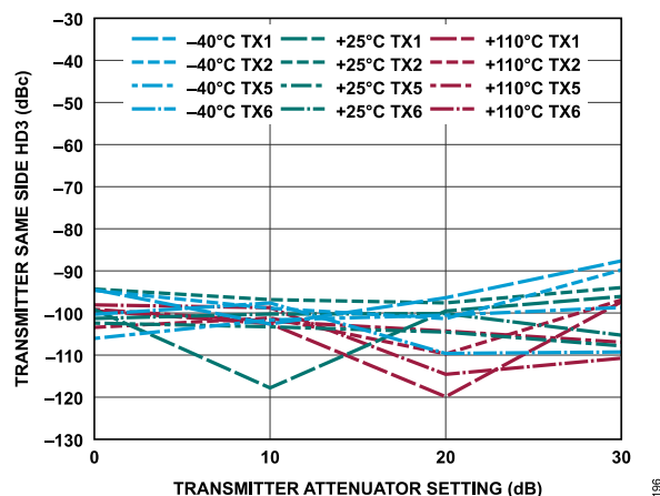
Figure 256. Transmitter Same Side HD3 vs. Transmitter Attenuation Setting, 30 MHz Offset, -12 dBFS Continuous Wave Signal
