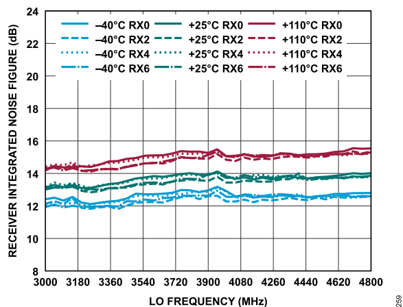
Figure 369. Receiver Integrated Noise Figure vs. LO Frequency, 600 MHz Integration Bandwidth
