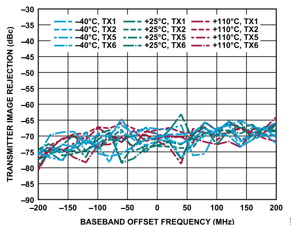
Figure 7. Transmitter Image Rejection vs. Baseband Offset Frequency, -6 dBFS Continuous Wave Signal
