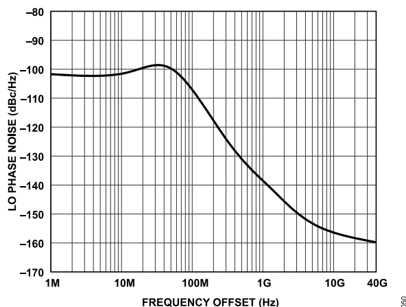
Figure 110. LO Phase Noise vs. Frequency Offset, Loop Bandwidth = 60 kHz, Phase Margin = 55°
