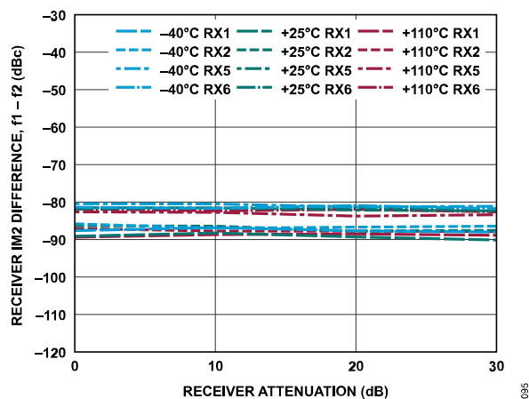
Figure 155. Receiver IM2 Difference, f_1 - f_2 vs. Receiver Attenuation, -7 dBFS Signal Level Per Tone, f_1 = 42 MHz Offset, f_2 = 2 MHz Offset
