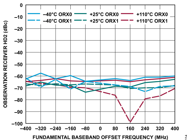
Figure 174. Observation Receiver HD2 vs. Fundamental Baseband Offset Frequency, -10 dBFS Input Signal
