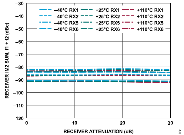
Figure 97. Receiver IM2 Sum, f_1 + f_2 vs. Receiver Attenuation, -7 dBFS Signal Level per Tone, f_1 = 42 MHz Offset, f_2 = 2 MHz Offset
