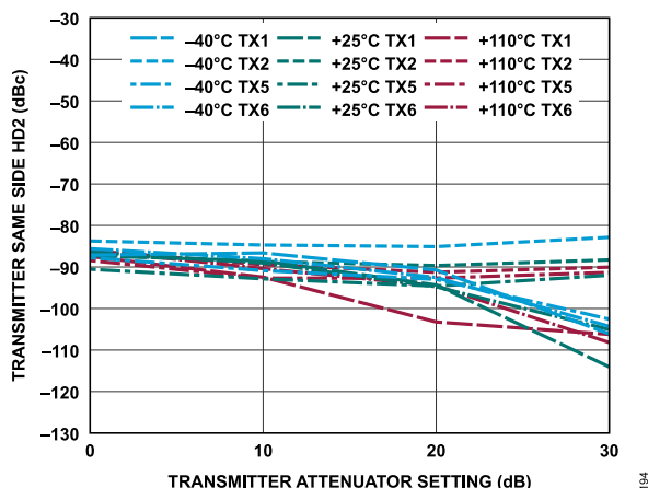
Figure 254. Transmitter Same Side HD2 vs. Transmitter Attenuation Setting, 30 MHz Offset, -12 dBFS Continuous Wave Signal
