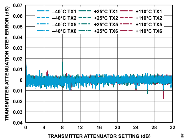
Figure 257. Transmitter Attenuation Step Error vs. Transmitter Attenuation Setting, 30 MHz Offset, -12 dBFS Continuous Wave Signal
