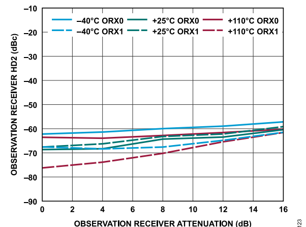
Figure 183. Observation Receiver HD2 vs. Observation Receiver Attenuation, 80 MHz Offset, -10 dBFS Input Signal
