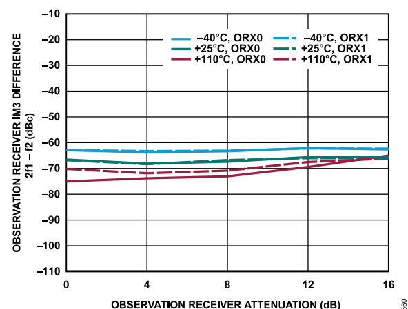
Figure 360. Observation Receiver IM3, 2f_1 - f_2 vs. Observation Receiver Attenuation, -13 dBFS Signal Level Per Tone, f_1 = 5602 MHz, f_2 = 5812 MHz
