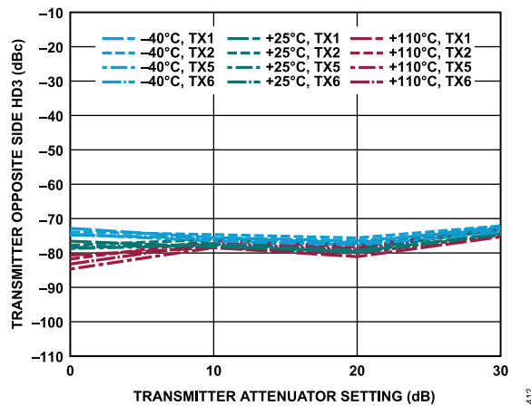
Figure 12. Transmitter Opposite Side Third Harmonic Distortion (HD3) vs. Transmitter Attenuator Setting, 30 MHz Offset, -12 dBFS Continuous Wave Signal
