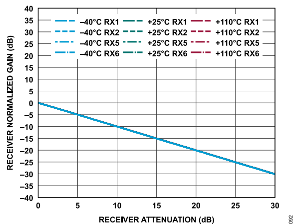
Figure 152. Receiver Normalized Gain vs. Receiver Attenuation, 30 MHz Offset, -1 dBFS Input Signal
