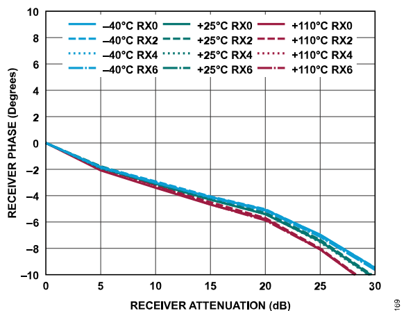
Figure 229. Receiver Phase vs. Receiver Attenuation
