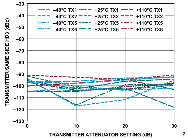
Figure 134. Transmitter Same Side HD3 vs. Transmitter Attenuation Setting, 30 MHz Offset, -12 dBFS Continuous Wave Signal
