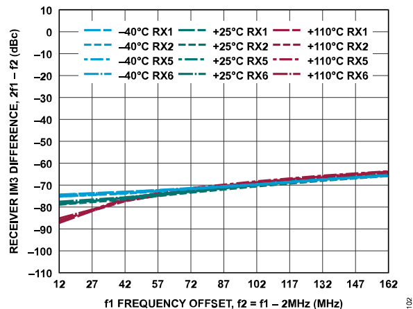
Figure 162. Receiver IM3 Difference, 2f_1 - f_2 vs. f_1 Frequency Offset, -7 dBFS Signal Level Per Tone, f_2 = f_1 - 2 MHz
