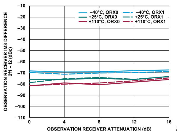
Figure 58. Observation Receiver IM3 Difference, 2f_1 - f_2 vs. Observation Receiver Attenuation, -13 dBFS Signal Level Per Tone, f_1 = 852 MHz, f_2 = 1062 MHz
