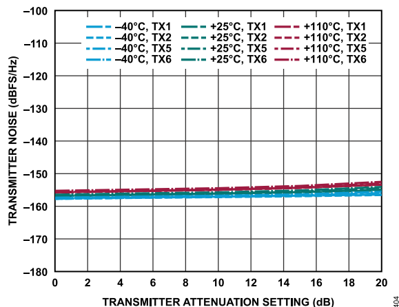
Figure 4. Transmitter Noise vs. Transmitter Attenuation Setting, 100 MHz Offset
