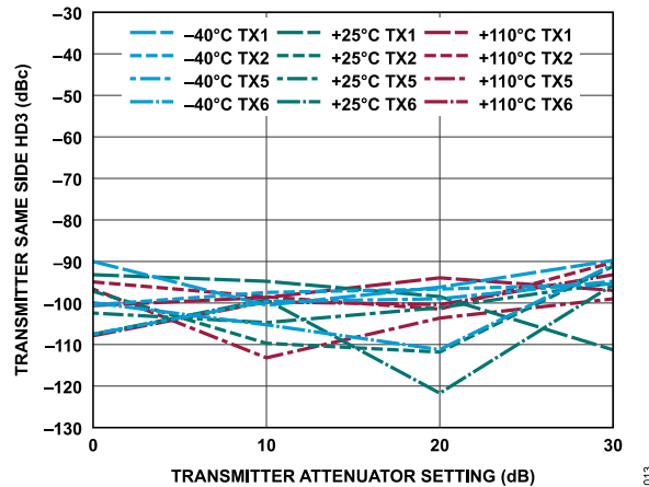
Figure 74. Transmitter Same Side HD3 vs. Transmitter Attenuation Setting, 30 MHz Offset, -12 dBFS Continuous Wave Signal
