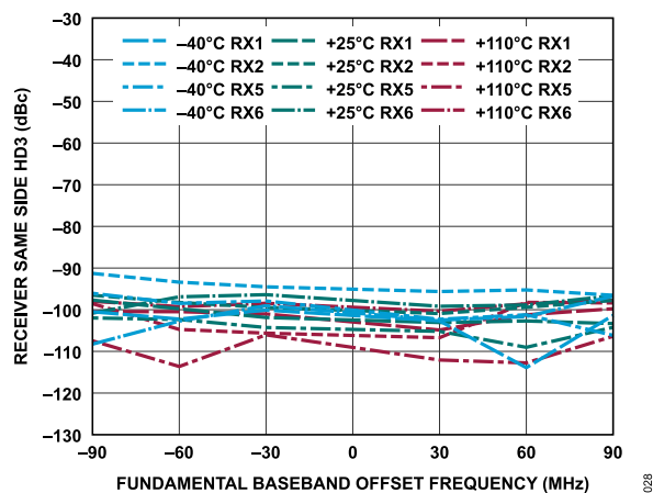
Figure 89. Receiver Same Side HD3 vs. Fundamental Baseband Offset Frequency, -1 dBFS Input Signal
