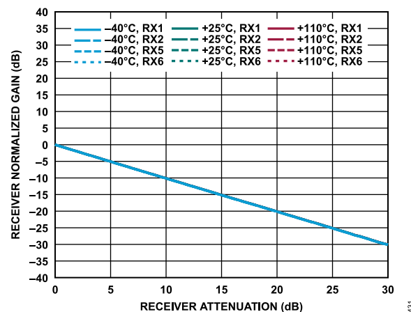
Figure 31. Receiver Normalized Gain vs. Receiver Attenuation, 30 MHz Offset, -1 dBFS Input Signal
