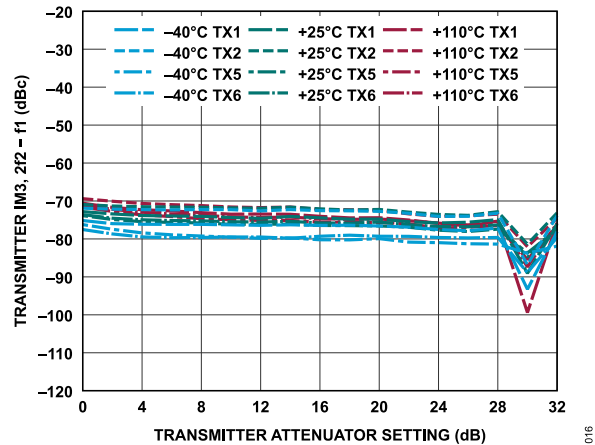
Figure 77. Transmitter IM3, 2f_2 - f_1 vs. Transmitter Attenuation Setting, -15 dBFS Signal Level Per Tone, f_1 = 160 MHz Offset, f_2 = 165 MHz Offset
