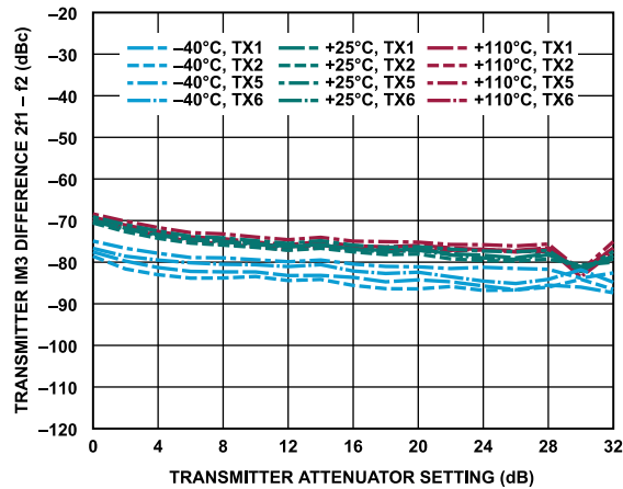
Figure 15. Transmitter IM3 Difference, 2f_1 - f_2 vs. Transmitter Attenuator Setting, -15 dBFS Signal Level Per Tone, f_1 = 180 MHz Offset, f_2 = 185 MHz Offset
