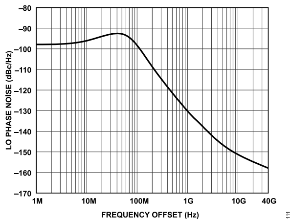
Figure 171. LO Phase Noise vs. Frequency Offset, Loop Bandwidth = 60 kHz, Phase Margin = 55°
