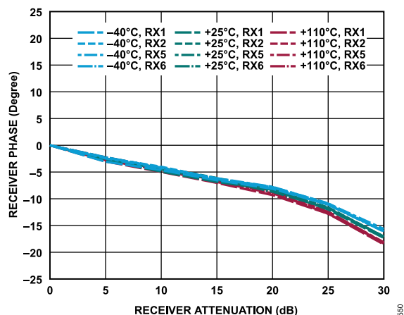
Figure 350. Receiver Phase vs. Receiver Attenuation
