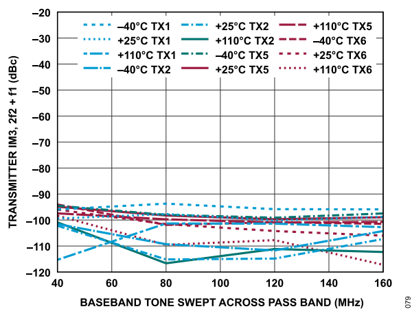
Figure 139. Transmitter IM3, 2f_2 + f_1 vs. Baseband Tone Swept Across Pass Band, -15 dBFS Signal Level Per Tone, f_2 = f_1 + 5 MHz
