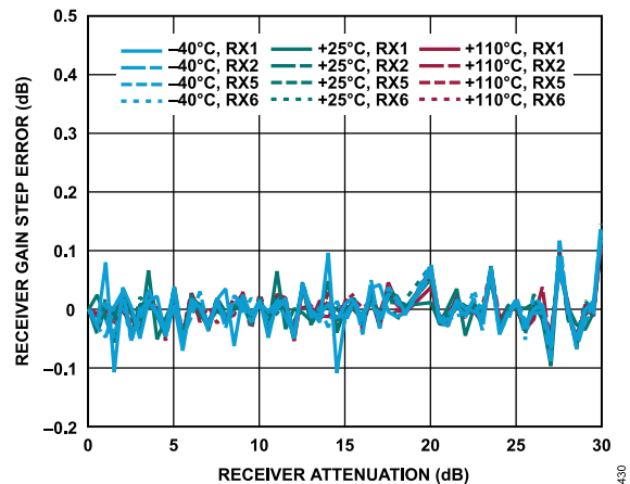
Figure 30. Receiver Gain Step Error vs. Receiver Attenuation, 30 MHz Offset, -1 dBFS Input Signal
