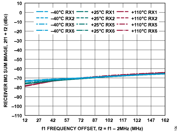
Figure 166. Receiver IM3 Sum Image, 2f_1 + f_2 vs. f_1 Frequency Offset, -7 dBFS Signal Level Per Tone, f_2 = f_1 - 2 MHz
