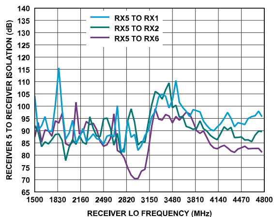
Figure 386. Receiver 5 to Receiver Isolation vs. Receiver LO Frequency
