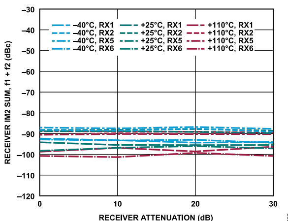
Figure 36. Receiver IM2 Sum, f_1 + f_2 vs. Receiver Attenuation, -7 dBFS Signal Level Per Tone, f_1 = 192 MHz Offset, f_2 = 2 MHz Offset
