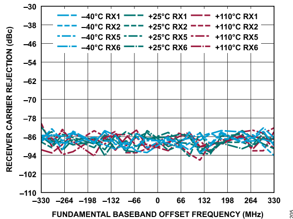
Figure 265. Receiver Carrier Rejection vs. Fundamental Baseband Offset Frequency, -1 dBFS Input Signal
