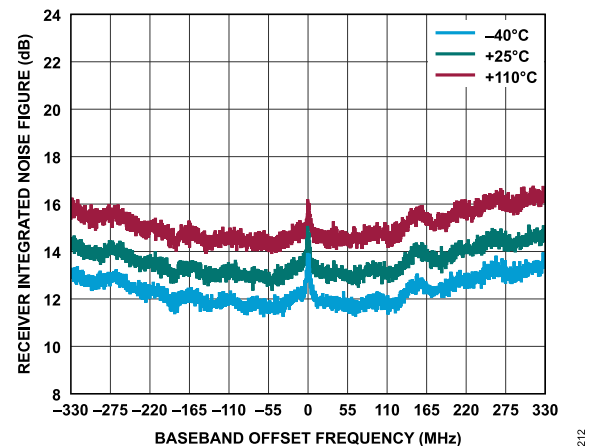
Figure 272. Receiver Integrated Noise Figure vs. Baseband Offset Frequency, 200 kHz Integration Steps, 983.04 MSPS Sample Rate
