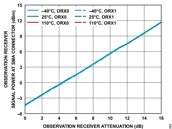
Figure 124. Observation Receiver Signal Power at SMA Connector vs. Observation Receiver Attenuation, 80 MHz Offset, -10 dBFS Input Signal
