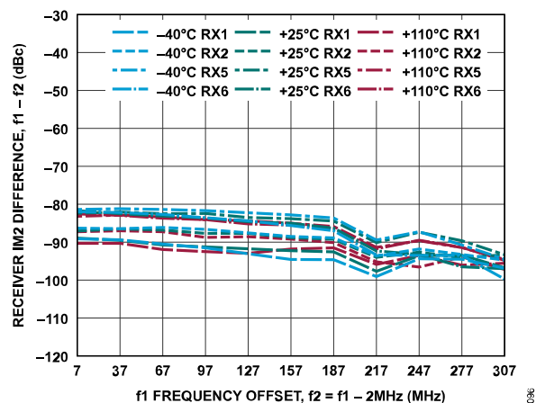
Figure 156. Receiver IM2 Difference, f_1 - f_2 vs. f_1 Frequency Offset, -7 dBFS Signal Level Per Tone, f_2 = f_1 - 2 MHz
