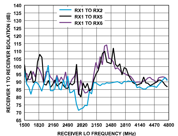
Figure 384. Receiver 1 to Receiver Isolation vs. Receiver LO Frequency
