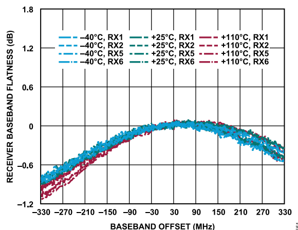
Figure 351. Receiver Baseband Flatness vs. Baseband Offset
