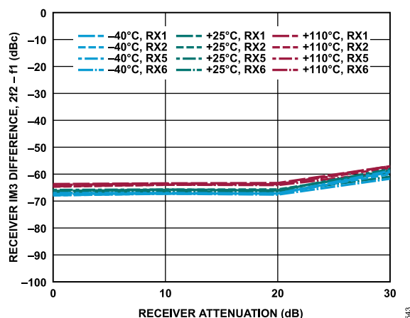
Figure 343. Receiver IM3 Difference, 2f_2 - f_1 vs. Receiver Attenuation, -7 dBFS Signal Level Per Tone, f_1 = 326 MHz Offset, f_2 = 328 MHz Offset
