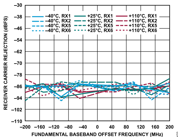
Figure 22. Receiver Carrier Rejection vs. Fundamental Baseband Offset Frequency, -1 dBFS Input Signal
