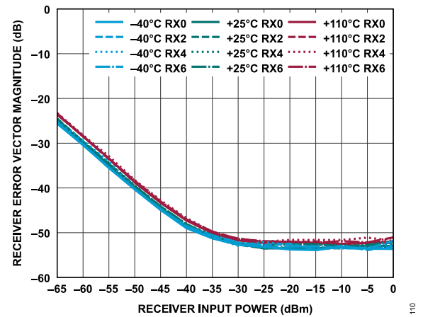
Figure 170. Receiver Error Vector Magnitude vs. Receiver Input Power, 20 MHz LTE Centered Around DC, TDD Mode, AGC Enabled
