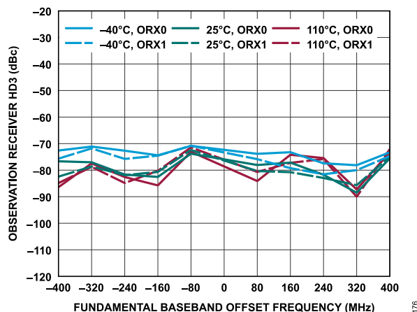
Figure 236. Observation Receiver HD3 vs. Fundamental Baseband Offset Frequency, -10 dBFS Input Signal
