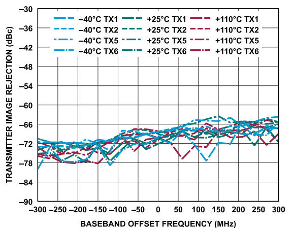
Figure 128. Transmitter Image Rejection vs. Baseband Offset Frequency, -6 dBFS Continuous Wave Signal
