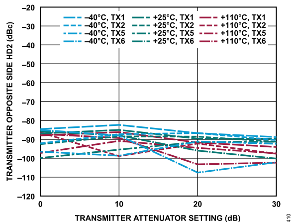
Figure 10. Transmitter Opposite Side Second Harmonic Distortion (HD2) vs. Transmitter Attenuator Setting, 30 MHz Offset, -12 dBFS Continuous Wave Signal
