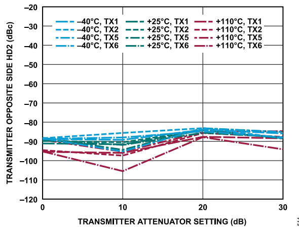
Figure 314. Transmitter Opposite Side HD2 vs. Transmitter Attenuator Setting, 165 MHz Offset, -12 dBFS Continuous Wave Signal
