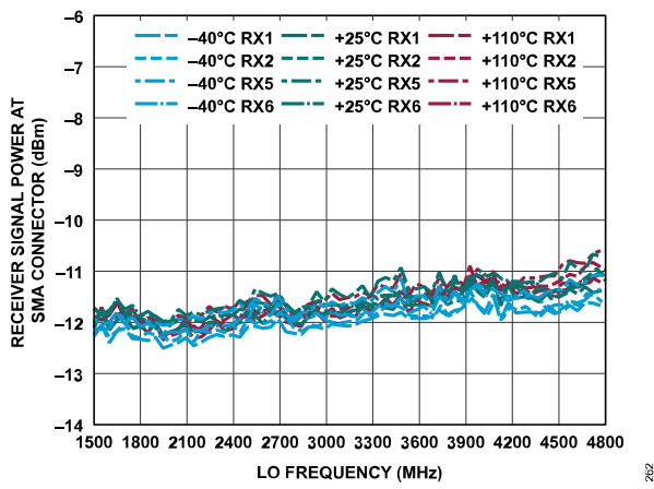
Figure 372. Receiver Signal Power at SMA Connector vs. LO Frequency
