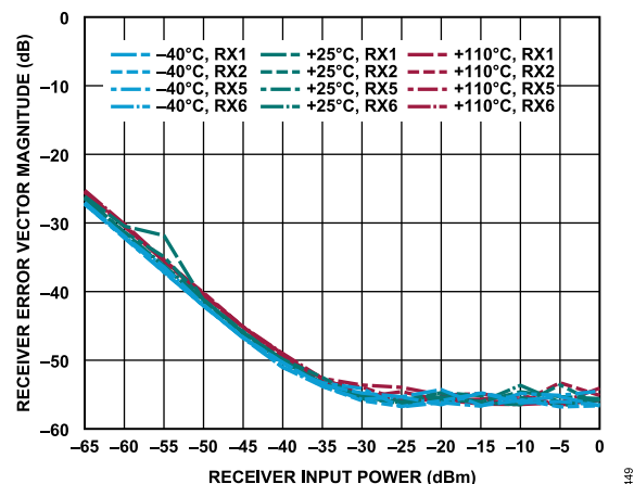
Figure 49. Receiver Error Vector Magnitude vs. Receiver Input Power, 20 MHz LTE Centered Around DC, TDD Mode, AGC Enabled
