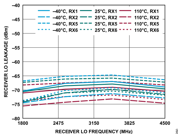
Figure 370. Receiver LO Leakage vs. Receiver LO Frequency, Maximum Receiver Gain
