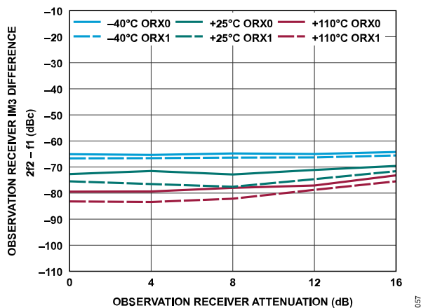
Figure 117. Observation Receiver IM3 Difference, 2f_2 - f_1 vs. Observation Receiver Attenuation, -13 dBFS Signal Level Per Tone, f_1 = 1802 MHz, f_2 = 1812 MHz
