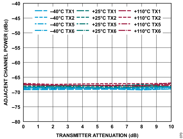
Figure 130. Adjacent Channel Power vs. Transmitter Attenuation, -10 MHz Offset, 20 MHz LTE, PAR = 12 dB
