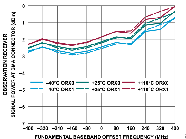
Figure 298. Observation Receiver Signal Power at SMA Connector vs. Fundamental Baseband Offset Frequency, -10 dBFS Input Signal (Match Is Not De-Embedded)
