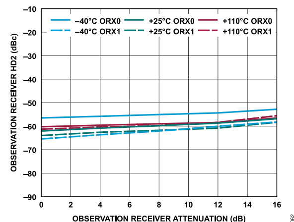
Figure 122. Observation Receiver HD2 vs. Observation Receiver Attenuation, 80 MHz Offset, -10 dBFS Input Signal
