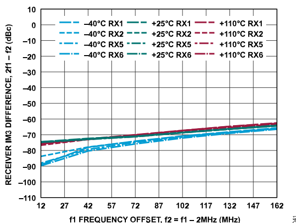
Figure 101. Receiver IM3 Difference, 2f_1 - f_2 vs. f_1 Frequency Offset, -7 dBFS Signal Level per Tone, f_2 = f_1 - 2 MHz
