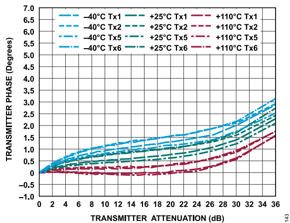
Figure 203. Transmitter Phase vs. Transmitter Attenuation
