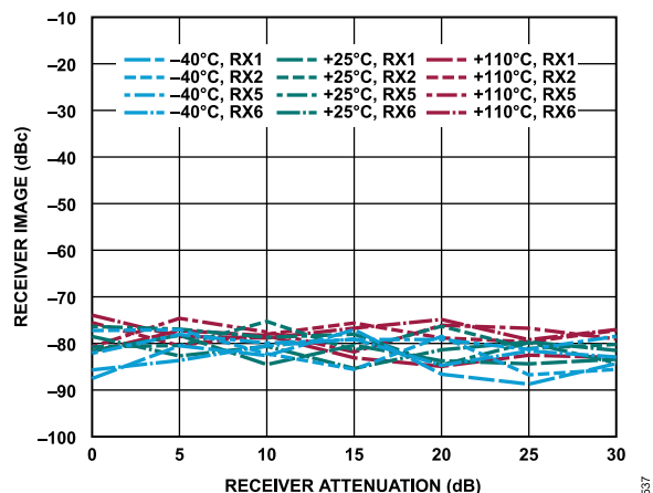
Figure 337. Receiver Image vs. Receiver Attenuation, 30 MHz Offset, -1 dBFS Input Signal
