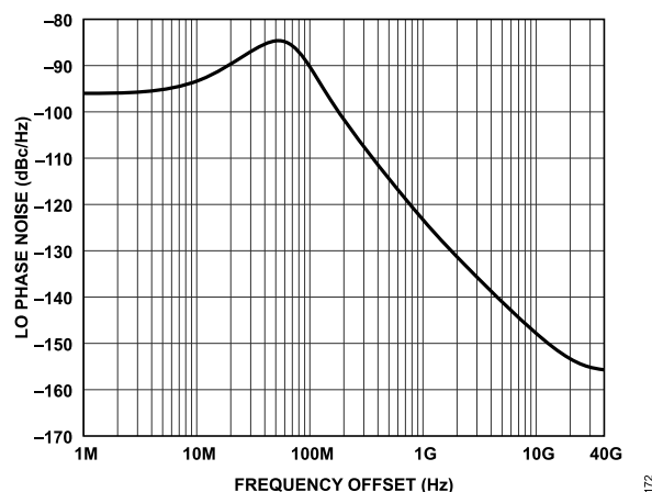
Figure 232. LO Phase Noise vs. Frequency Offset, Loop Bandwidth = 60 kHz, Phase Margin = 55^\circ
