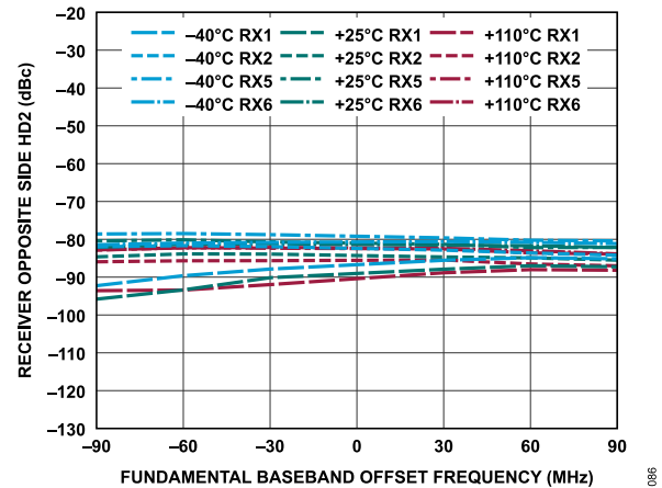
Figure 146. Receiver Opposite Side HD2 vs. Fundamental Baseband Offset Frequency, -1 dBFS Input Signal
