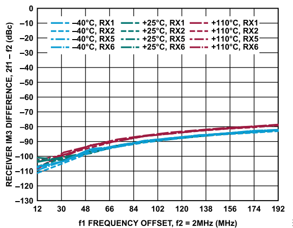
Figure 41. Receiver IM3 Difference, 2f_1 - f_2 vs. f_1 Frequency Offset, -7 dBFS Signal Level Per Tone, f_2 = 2 MHz
