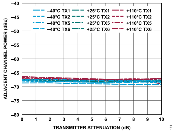
Figure 191. Adjacent Channel Power vs. Transmitter Attenuation, -10 MHz Offset, 20 MHz LTE, PAR = 12 dB
