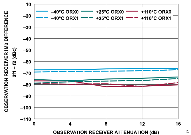
Figure 177. Observation Receiver IM3 Difference, 2f_1 - f_2 vs. Observation Receiver Attenuation, -13 dBFS Signal Level Per Tone, f_1 = 2602 MHz, f_2 = 2612 MHz
