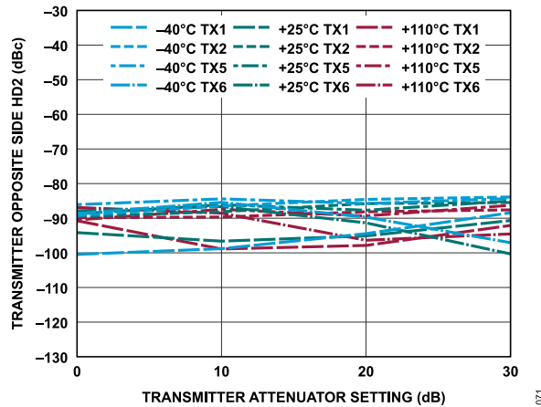
Figure 131. Transmitter Opposite Side HD2 vs. Transmitter Attenuation Setting, 30 MHz Offset, -12 dBFS Continuous Wave Signal
