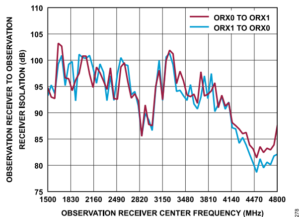
Figure 388. Observation Receiver to Observation Receiver Isolation vs. Observation Receiver Center Frequency
