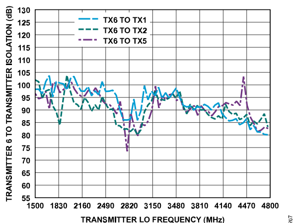
Figure 377. Transmitter 6 to Transmitter Isolation vs. Transmitter LO Frequency
