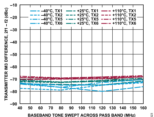
Figure 323. Transmitter IM3 Difference, 2f_1 - f_2 vs. Baseband Tone Swept Across Pass Band, -15 dBFS Signal Level Per Tone, f_2 = 5 MHz
