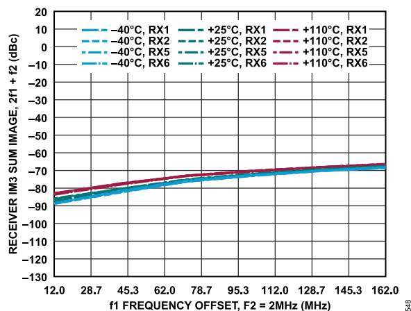
Figure 348. Receiver IM3 Sum Image, 2f_1 + f_2 vs. f_1 Frequency Offset, f_2 = 2 MHz, -7 dBFS Signal Level Per Tone
