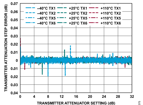
Figure 135. Transmitter Attenuation Step Error vs. Transmitter Attenuation Setting, 30 MHz Offset, -12 dBFS Continuous Wave Signal
