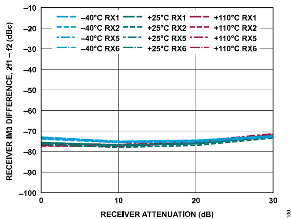
Figure 160. Receiver IM3, 2f_1 - f_2 vs. Receiver Attenuation, -7 dBFS Signal Level Per Tone, f_1 = 42 MHz Offset, f_2 = 2 MHz Offset
