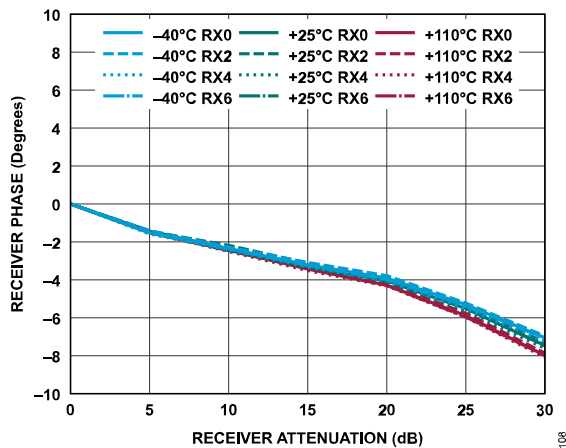
Figure 168. Receiver Phase vs. Receiver Attenuation
