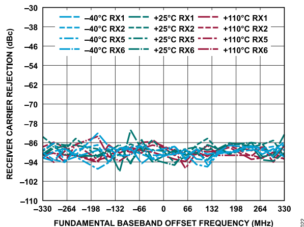
Figure 83. Receiver Carrier Rejection vs. Fundamental Baseband Offset Frequency, -1 dBFS Input Signal
