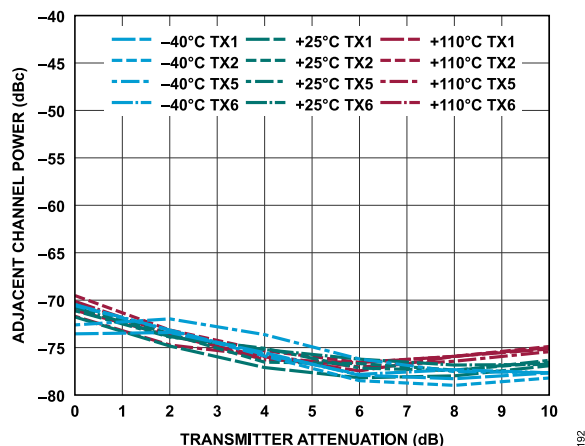
Figure 252. Adjacent Channel Power vs. Transmitter Attenuation, -10 MHz Offset, 20 MHz LTE, PAR = 12 dB
