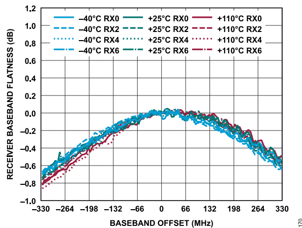
Figure 230. Receiver Baseband Flatness vs. Baseband Offset
