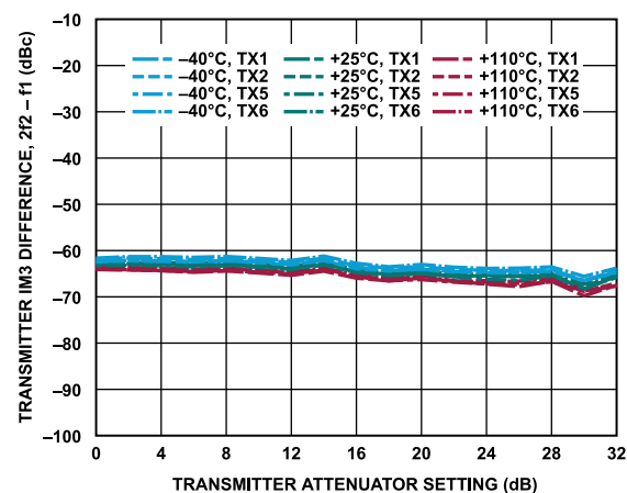
Figure 320. Transmitter IM3 Difference, 2f_2 - f_1 vs. Transmitter Attenuator Setting, -15 dBFS Signal Level Per Tone, f_1 = 320 MHz Offset, f_2 = 2 MHz Offset
