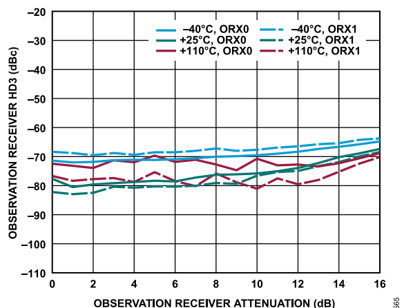
Figure 365. Observation Receiver HD3 vs. Observation Receiver Attenuation, 80 MHz Offset, -10 dBFS Input Signal
