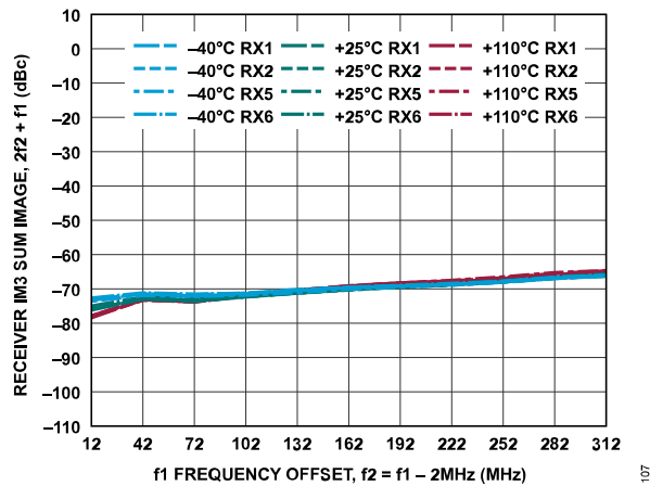
Figure 167. Receiver IM3 Sum Image, 2f_2 + f_1 vs. f_1 Frequency Offset, -7 dBFS Signal Level Per Tone, f_2 = f_1 - 2 MHz
