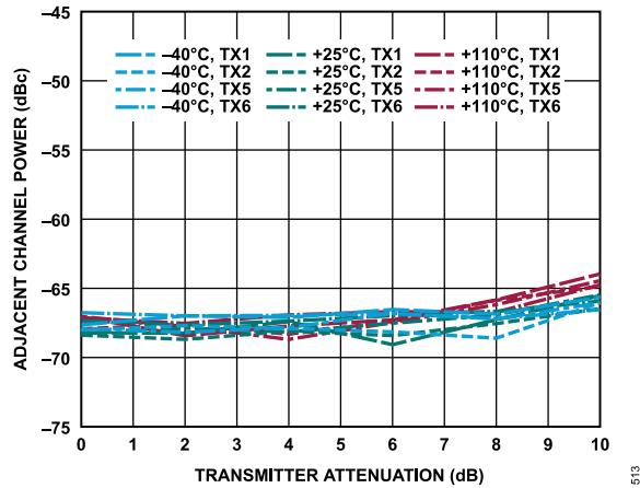
Figure 313. Adjacent Channel Power vs. Transmitter Attenuation, -10 MHz Offset, 20 MHz LTE, PAR = 12 dB
