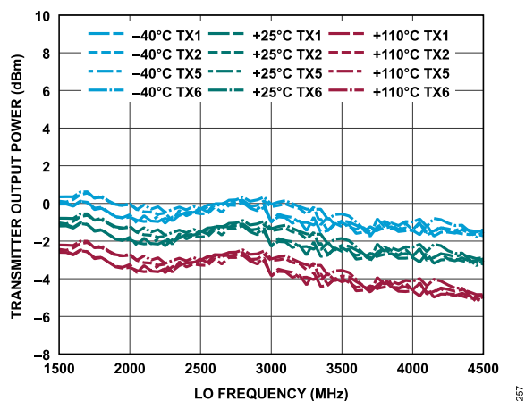
Figure 367. Transmitter Output Power vs. LO Frequency, 30 MHz Offset, 0 dB RF Attenuation, -6 dBFS Signal Level
