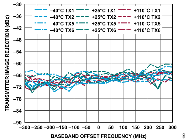
Figure 250. Transmitter Image Rejection vs. Baseband Offset Frequency, -6 dBFS Continuous Wave Signal
