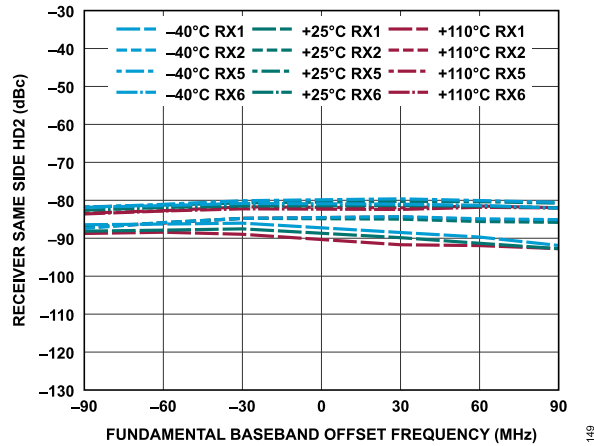
Figure 209. Receiver Same Side HD2 vs. Fundamental Baseband Offset Frequency, -1 dBFS Input Signal
