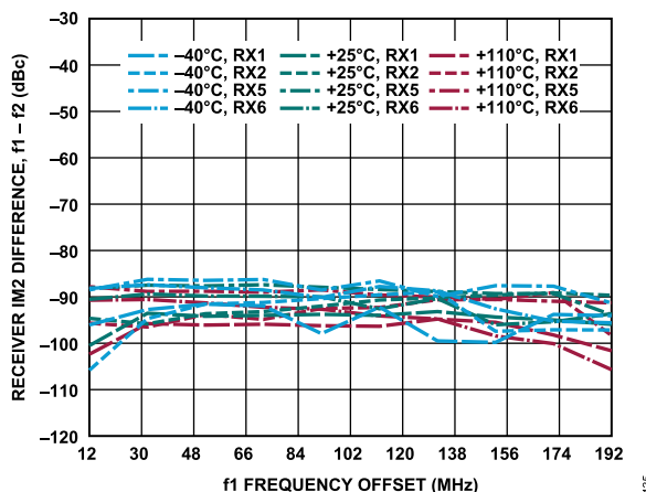
Figure 35. Receiver IM2 Difference, f_1 - f_2 vs. f_1 Frequency Offset, -7 dBFS Signal Level Per Tone, f_2 = 2 MHz
