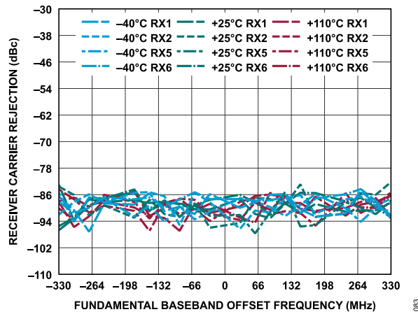
Figure 143. Receiver Carrier Rejection vs. Fundamental Baseband Offset Frequency, -1 dBFS Input Signal
