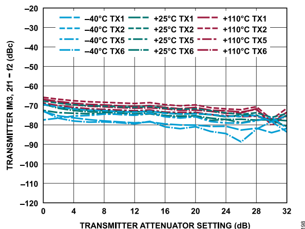
Figure 258. Transmitter IM3, 2f_1 - f_2 vs. Transmitter Attenuation Setting, -15 dBFS Signal Level Per Tone, f_1 = 160 MHz Offset, f_2 = 165 MHz Offset
