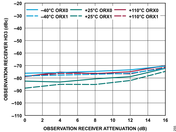
Figure 306. Observation Receiver HD3 vs. Observation Receiver Attenuation, 80 MHz Offset, -10 dBFS Input Signal
