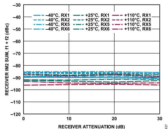
Figure 37. Receiver IM2 Sum, f_1 + f_2 vs. Receiver Attenuation, -7 dBFS Signal Level Per Tone, f_1 = 101 MHz Offset, f_2 = 99 MHz Offset
