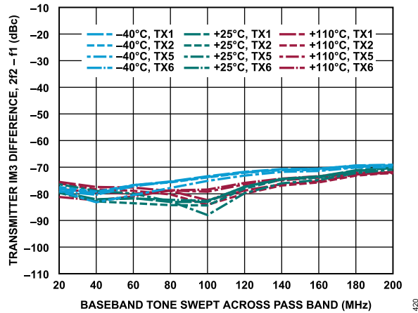
Figure 20. Transmitter IM3 Difference, 2f_2 - f_1 vs. Baseband Tone Swept Across Pass Band, -15 dBFS Signal Level Per Tone, f_2 = f_1 + 5 MHz
