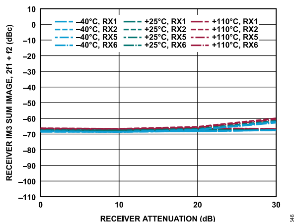
Figure 346. Receiver IM3 Sum Image, 2f_1 + f_2 vs. Receiver Attenuation, -7 dBFS Signal Level Per Tone, f_1 = 162 MHz Offset, f_2 = 2 MHz Offset
