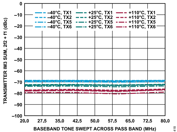
Figure 18. Transmitter IM3 Sum, 2f_2 + f_1 vs. Baseband Tone Swept Across Pass Band, -15 dBFS Signal Level Per Tone, f_2 = f_1 + 5 MHz
