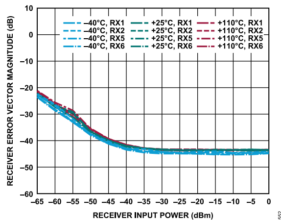
Figure 352. Receiver Error Vector Magnitude vs. Receiver Input Power, 20 MHz LTE Centered Around DC, TDD Mode, AGC Enabled
