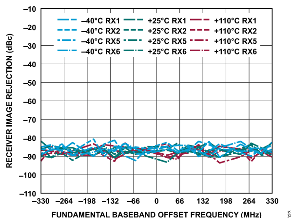
Figure 84. Receiver Image Rejection vs. Fundamental Baseband Offset Frequency, -1 dBFS Input Signal
