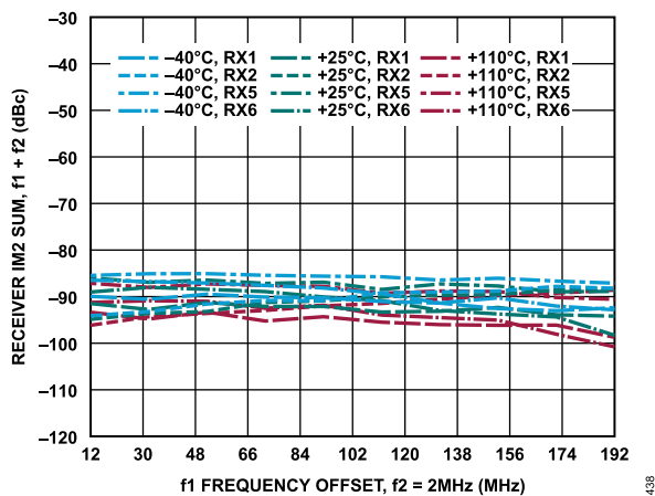
Figure 38. Receiver IM2 Sum, f_1 + f_2 vs. f_1 Frequency Offset, -7 dBFS Signal Level Per Tone, f_2 = 2 MHz
