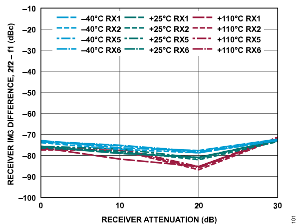
Figure 161. Receiver IM3 Difference, 2f_2 - f_1 vs. Receiver Attenuation, -7 dBFS Signal Level Per Tone, f_1 = 42 MHz Offset, f_2 = 2 MHz Offset
