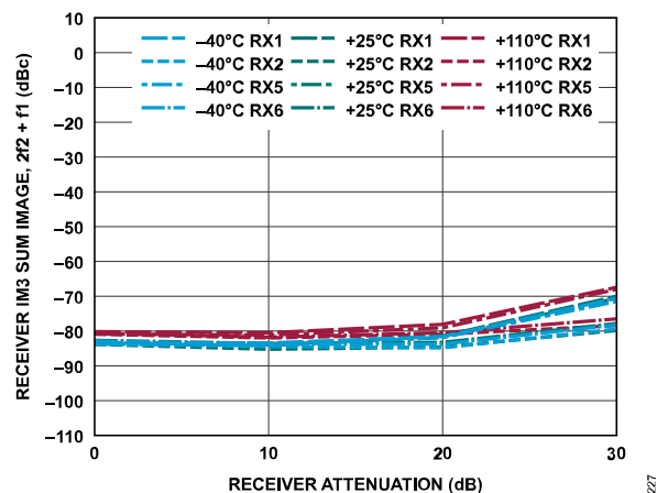
Figure 287. Receiver IM3 Sum Image, 2f_2 + f_1 vs. Receiver Attenuation, -7 dBFS Signal Level Per Tone, f_1 = 42 MHz Offset, f_2 = 2 MHz Offset
