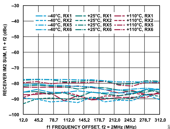
Figure 341. Receiver IM2, f_1 + f_2 vs. f_1 Frequency Offset, -7 dBFS Signal Level Per Tone, f_2 = 2 MHz
