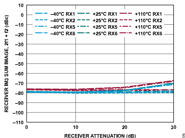
Figure 286. Receiver IM3 Sum Image, 2f_1 + f_2 vs. Receiver Attenuation, -7 dBFS Signal Level Per Tone, f_1 = 42 MHz Offset, f_2 = 2 MHz Offset
