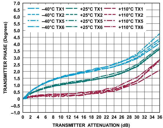
Figure 264. Transmitter Phase vs. Transmitter Attenuation
