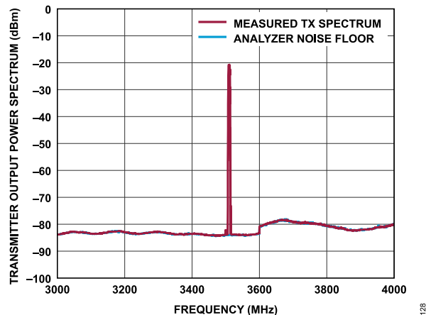
Figure 188. Transmitter Output Power Spectrum, Tx0, 5MHz LTE, 10 MHz Offset, -10 dBFS RMS, 1 MHz Resolution Bandwidth, T_j = 25^\circ\text{C}
