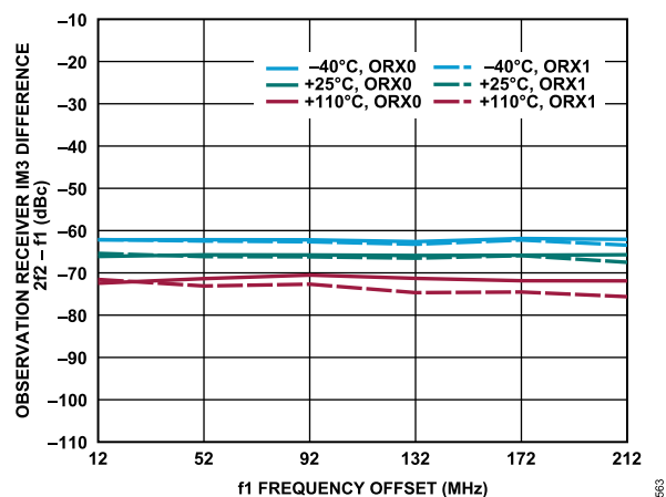
Figure 363. Observation Receiver IM3, 2f_2 - f_1 vs. f_1 Frequency Offset, f_2 = 2 MHz, -13 dBFS Signal Level Per Tone
