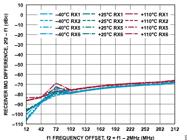
Figure 285. Receiver IM3 Difference, 2f_2 - f_1 vs. f_1 Frequency Offset, -7 dBFS Signal Level Per Tone, f_2 = f_1 - 2 MHz
