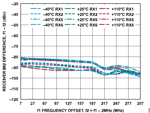
Figure 278. Receiver IM2 Difference, f_1 - f_2 vs. f_1 Frequency Offset, -7 dBFS Signal Level Per Tone, f_2 = f_1 - 2 MHz
