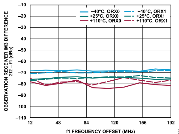
Figure 61. Observation Receiver IM3 Difference, 2f_2 - f_1 vs. f_1 Frequency Offset, -13 dBFS Signal Level Per Tone, f_2 = 852 MHz
