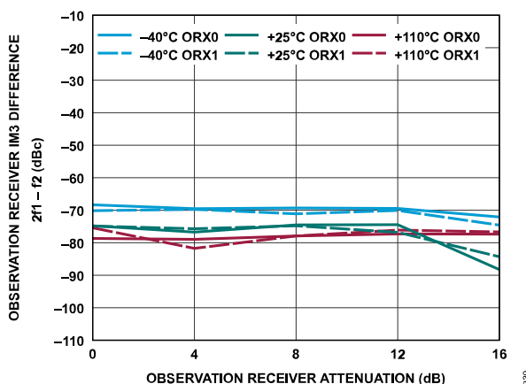
Figure 299. Observation Receiver IM3 Difference, 2f_1 - f_2 vs. Observation Receiver Attenuation, -13 dBFS Signal Level Per Tone, f_1 = 3502 MHz, f_2 = 3512 MHz
