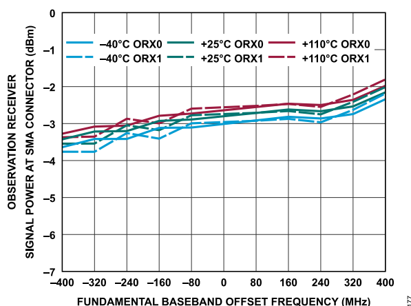
Figure 237. Observation Receiver Signal Power at SMA Connector vs. Fundamental Baseband Frequency, -10 dBFS Input Signal (Match Is Not De-Embedded)
