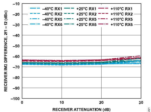
Figure 281. Receiver IM3 Difference, 2f_1 - f_2 vs. Receiver Attenuation, -7 dBFS Signal Level Per Tone, f_2 = f_1 - 2 MHz
