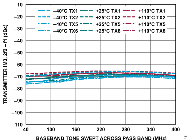
Figure 202. Transmitter IM3, 2f_2 - f_1 vs. Baseband Tone Swept Across Pass Band, -15 dBFS Signal Level Per Tone, f_2 = f_1 + 5 MHz
