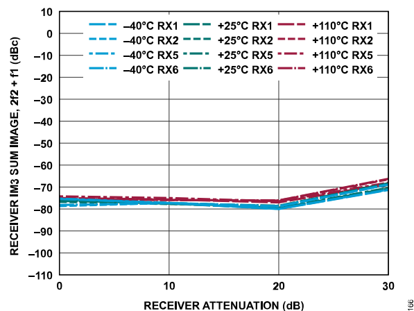
Figure 226. Receiver IM3 Sum Image, 2f_2 + f_1 vs. Receiver Attenuation, -7 dBFS Signal Level Per Tone, f_1 = 42 MHz Offset, f_2 = 2 MHz Offset
