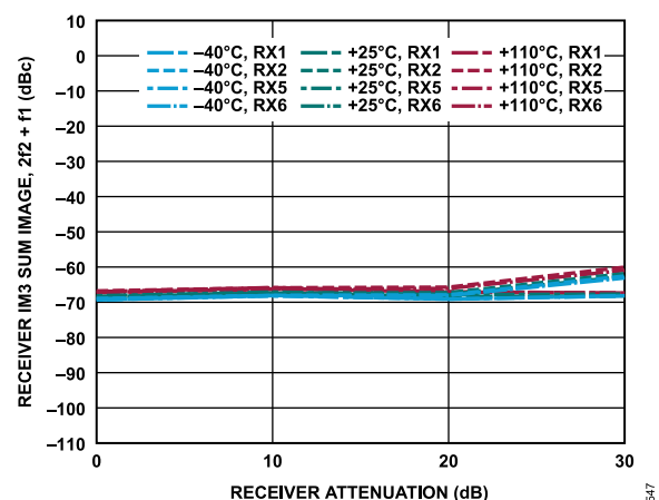
Figure 347. Receiver IM3 Sum Image, 2f_2 + f_1 vs. Receiver Attenuation, -7 dBFS Signal Level Per Tone, f_1 = 312 MHz Offset, f_2 = 2 MHz Offset
