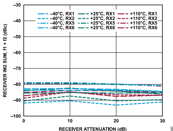
Figure 340. Receiver IM2 Sum, f_1 + f_2 vs. Receiver Attenuation, -7 dBFS Signal Level Per Tone, f_1 = 328 MHz Offset, f_2 = 2 MHz Offset
