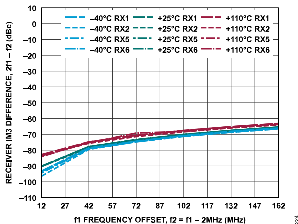
Figure 284. Receiver IM3 Difference, 2f_1 - f_2 vs. f_1 Frequency Offset, -7 dBFS Signal Level Per Tone, f_2 = f_1 - 2 MHz
