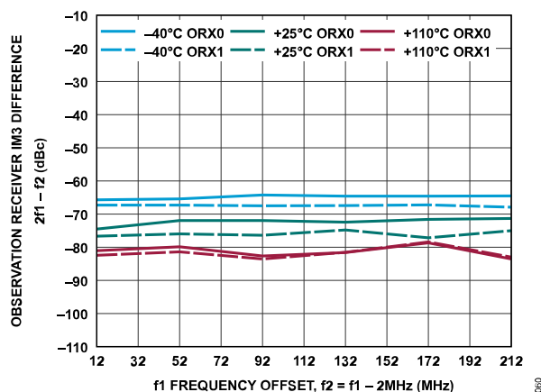
Figure 120. Observation Receiver IM3 Difference, 2f_1 - f_2 vs. f_1 Frequency Offset, -13 dBFS Signal Level per Tone, f_2 = f_1 - 2 MHz
