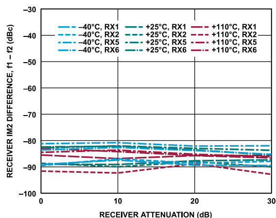
Figure 338. Receiver IM2 Difference, f_1 - f_2 vs. Receiver Attenuation, -7 dBFS Signal Level Per Tone, f_1 = 328 MHz Offset, f_2 = 2 MHz Offset
