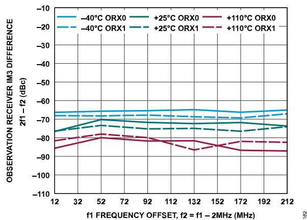
Figure 242. Observation Receiver IM3 Difference, 2f_1 - f_2 vs. f_1 Frequency Offset, -13 dBFS Signal Level Per Tone, f_2 = f_1 - 2 MHz
