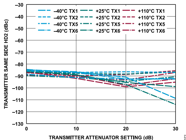
Figure 132. Transmitter Same Side HD2 vs. Transmitter Attenuation Setting, 30 MHz Offset, -12 dBFS Continuous Wave Signal
