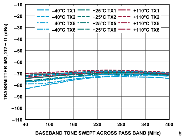
Figure 141. Transmitter IM3, 2f_2 - f_1 vs. Baseband Tone Swept Across Pass Band, -15 dBFS Signal Level Per Tone, f_2 = f_1 + 5 MHz
