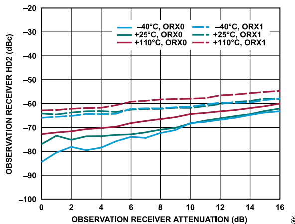
Figure 364. Observation Receiver HD2 vs. Observation Receiver Attenuation, 80 MHz Offset, -10 dBFS Input Signal
