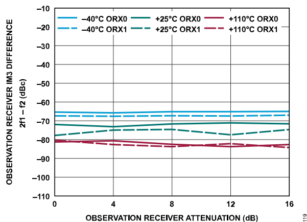
Figure 179. Observation Receiver IM3 Difference, 2f_1 - f_2 vs. Observation Receiver Attenuation, -13 dBFS Signal Level Per Tone, f_1 = 2602 MHz, f_2 = 2812 MHz
