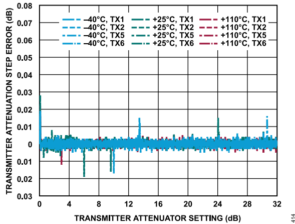
Figure 14. Transmitter Attenuation Step Error vs. Transmitter Attenuator Setting, 30 MHz Offset, -12 dBFS Continuous Wave Signal
