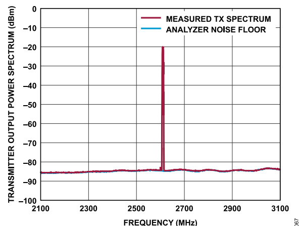
Figure 127. Transmitter Output Power Spectrum, Tx1, 5MHz LTE, 10 MHz Offset, -10 dBFS RMS, 1 MHz Resolution Bandwidth, T_j = 25^\circ\text{C}
