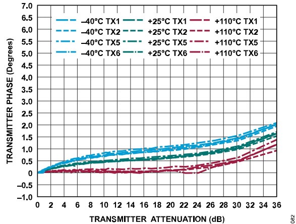
Figure 142. Transmitter Phase vs. Transmitter Attenuation
