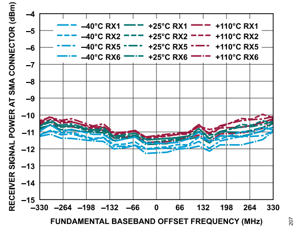
Figure 267. Receiver Signal Power at SMA Connector vs. Fundamental Baseband Offset Frequency, -1 dBFS Input Signal (Match Is Not De-Embedded)
