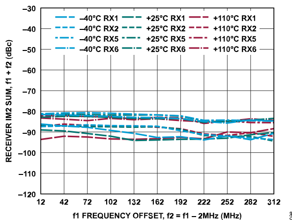
Figure 158. Receiver IM2 Sum, f_1 + f_2 vs. f_1 Frequency Offset, -7 dBFS Signal Level Per Tone, f_2 = f_1 - 2 MHz
