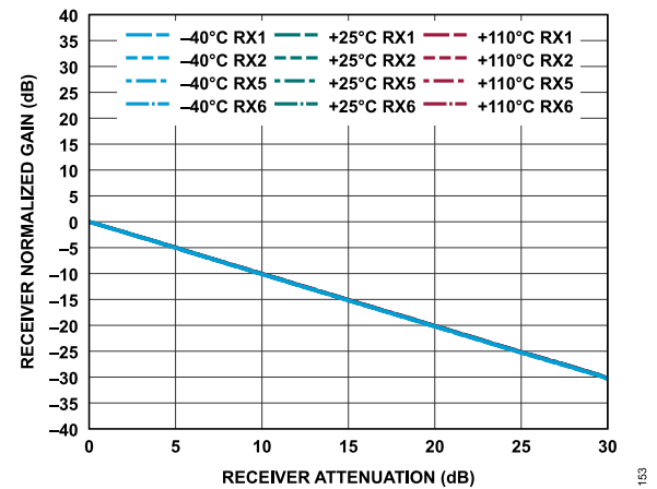
Figure 213. Receiver Normalized Gain vs. Receiver Attenuation, 30 MHz Offset, -1 dBFS Input Signal
