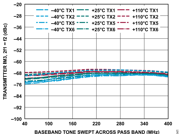
Figure 201. Transmitter IM3, 2f_1 - f_2 vs. Baseband Tone Swept Across Pass Band, -15 dBFS Signal Level Per Tone, f_2 = f_1 + 5 MHz
