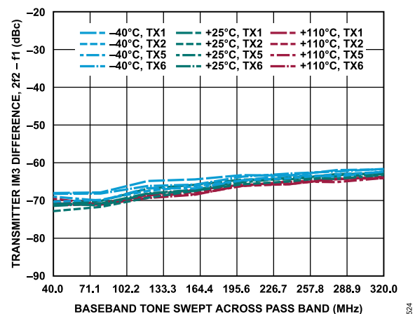
Figure 324. Transmitter IM3 Difference, 2f_2 - f_1 vs. Baseband Tone Swept Across Pass Band, -15 dBFS Signal Level Per Tone, f_2 = 5 MHz
