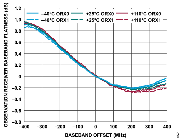
Figure 112. Observation Receiver Baseband Flatness vs. Baseband Offset
