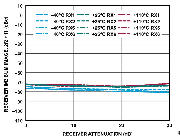
Figure 104. Receiver IM3 Sum Image, 2f_2 + f_1 vs. Receiver Attenuation, -7 dBFS Signal Level per Tone, f_1 = 42 MHz Offset, f_2 = 2 MHz Offset
