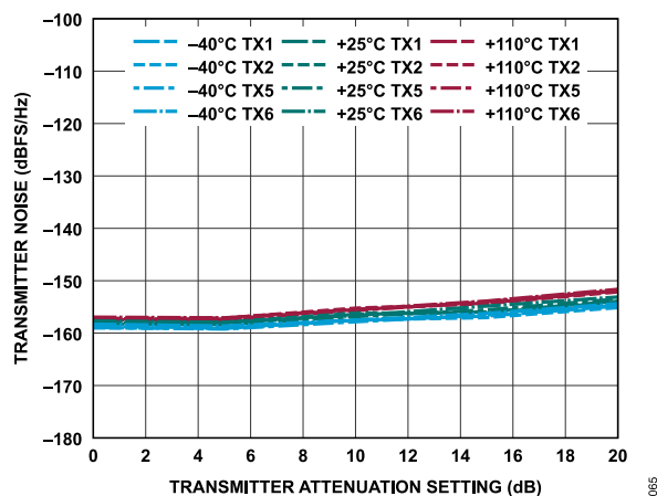
Figure 125. Transmitter Noise vs. Transmitter Attenuation, 150 MHz Offset
