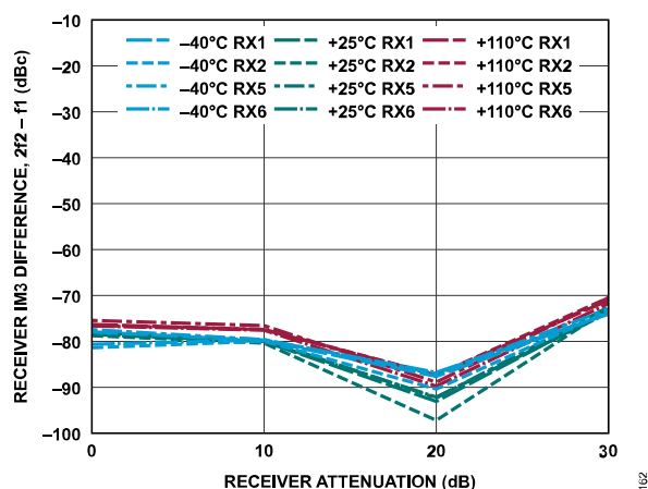
Figure 222. Receiver IM3 Difference, 2f_2 - f_1 vs. Receiver Attenuation, -7 dBFS Signal Level Per Tone, f_1 = 42 MHz Offset, f_2 = 2 MHz Offset
