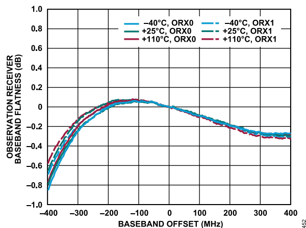
Figure 52. Observation Receiver Baseband Flatness vs. Baseband Offset
