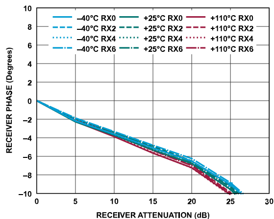
Figure 290. Receiver Phase vs. Receiver Attenuation
