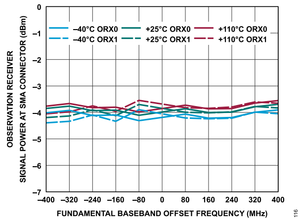
Figure 176. Observation Receiver Signal Power at SMA Connector vs. Fundamental Baseband Offset Frequency, -10 dBFS Input Signal (Match Is Not De-Embedded)
