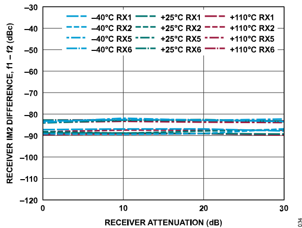
Figure 95. Receiver IM2 Difference, f_1 - f_2 vs. Receiver Attenuation, -7 dBFS Signal Level per Tone, f_1 = 42 MHz Offset, f_2 = 2 MHz Offset
