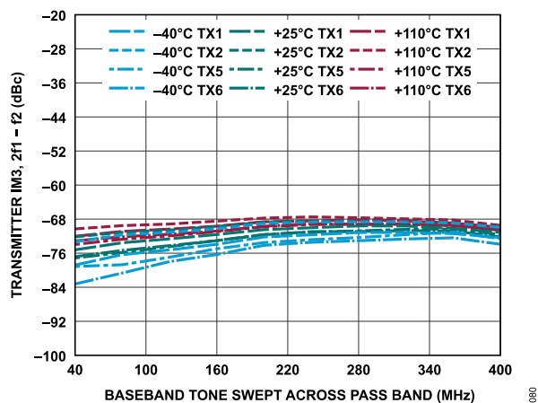
Figure 140. Transmitter IM3, 2f_1 - f_2 vs. Baseband Tone Swept Across Pass Band, -15 dBFS Signal Level Per Tone, f_2 = f_1 + 5 MHz
