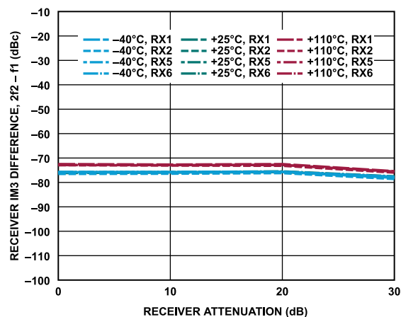
Figure 40. Receiver IM3 Difference, 2f_2 - f_1 vs. Receiver Attenuation, -7 dBFS Signal Level Per Tone, f_1 = 101 MHz Offset, f_2 = 2 MHz Offset
