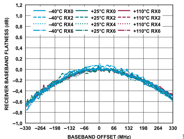
Figure 108. Receiver Baseband Flatness vs. Baseband Offset
