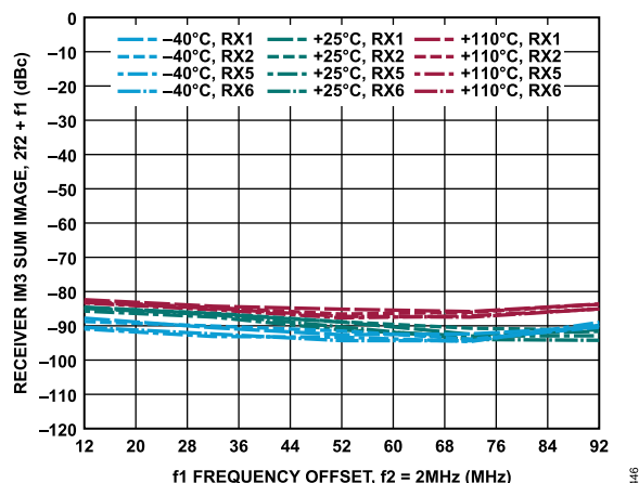
Figure 46. Receiver IM3 Sum Image, 2f_2 + f_1 vs. f_1 Frequency Offset, -7 dBFS Signal Level Per Tone, f_2 = 2 MHz
