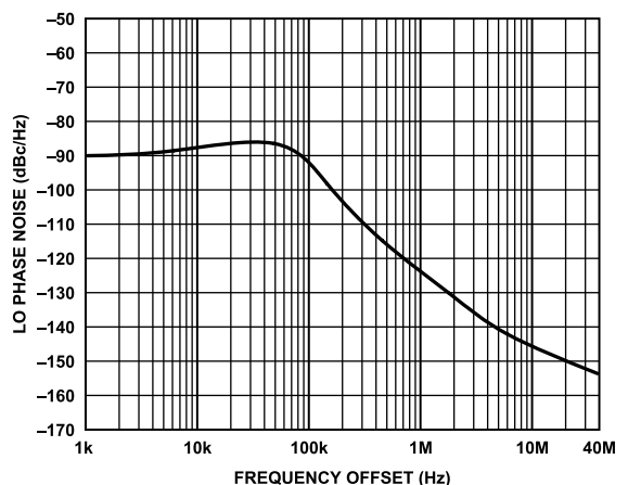
Figure 353. LO Phase Noise vs. Frequency Offset, Loop Bandwidth = 60 kHz, Phase Margin = 55°
