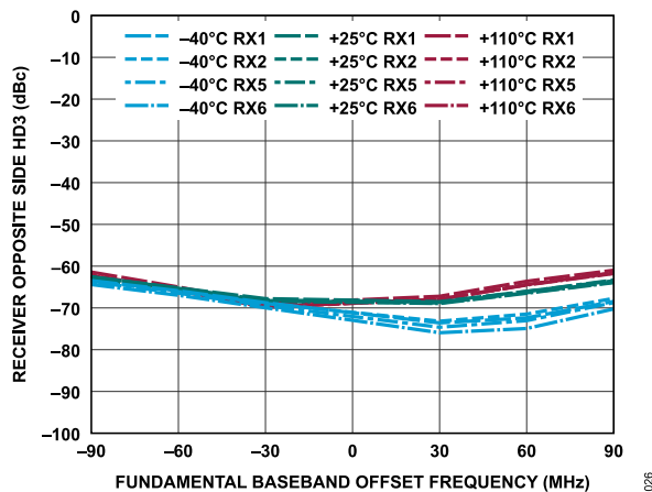
Figure 87. Receiver Opposite Side HD3 vs. Fundamental Baseband Offset Frequency, -1 dBFS Input Signal
