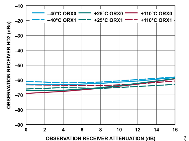
Figure 305. Observation Receiver HD2 vs. Observation Receiver Attenuation, 80 MHz Offset, -10 dBFS Input Signal
