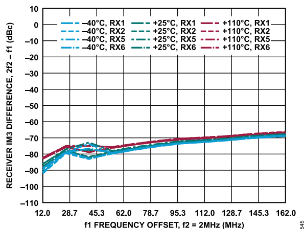
Figure 345. Receiver IM3 Difference, 2f_2 - f_1 vs. f_1 Frequency Offset, f_2 = 2 MHz, -7 dBFS Signal Level Per Tone
