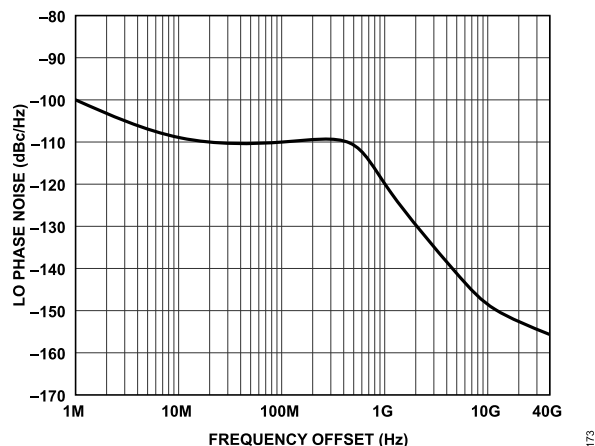
Figure 233. LO Phase Noise vs. Frequency Offset, Loop Bandwidth = 500 kHz, Phase Margin = 55°
