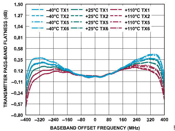
Figure 248. Transmitter Pass-Band Flatness vs. Baseband Offset Frequency
