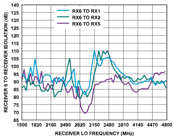
Figure 387. Receiver 6 to Receiver Isolation vs. Receiver LO Frequency
