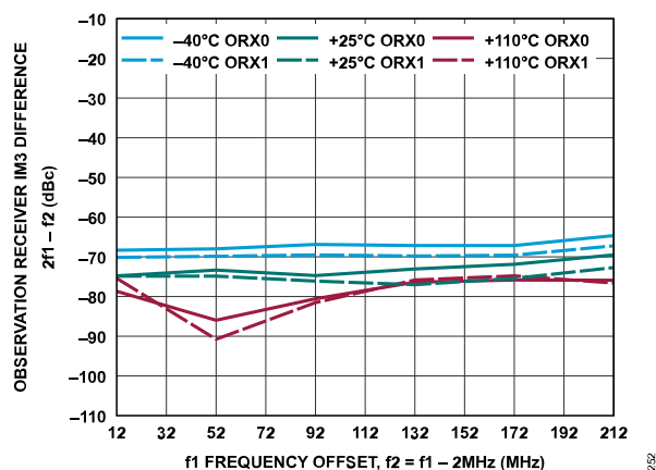
Figure 303. Observation Receiver IM3 Difference, 2f_1 - f_2 vs. f_1 Frequency Offset, -13 dBFS Signal Level Per Tone, f_2 = f_1 - 2 MHz
