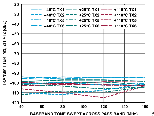
Figure 199. Transmitter IM3, 2f_1 + f_2 vs. Baseband Tone Swept Across Pass Band, -15 dBFS Signal Level Per Tone, f_2 = f_1 + 5 MHz
