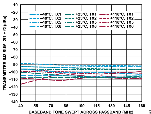
Figure 321. Transmitter IM3 Sum, 2f_1 + f_2 vs. Baseband Tone Swept Across Pass Band, -15 dBFS Signal Level Per Tone, f_2 = 5 MHz
