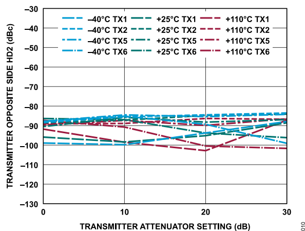
Figure 71. Transmitter Opposite Side Second Harmonic Distortion (HD2) vs. Transmitter Attenuation Setting, 30 MHz Offset, -12 dBFS Continuous Wave Signal
