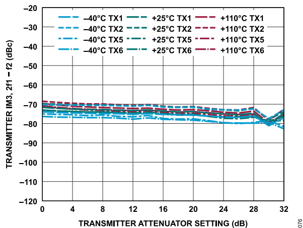
Figure 136. Transmitter IM3, 2f_1 - f_2 vs. Transmitter Attenuation Setting, -15 dBFS Signal Level Per Tone, f_1 = 160 MHz Offset, f_2 = 165 MHz Offset
