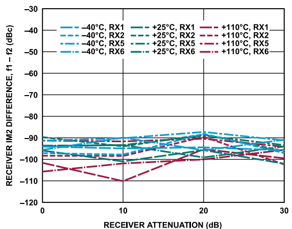
Figure 34. Receiver IM2 Difference, f_1 - f_2 vs. Receiver Attenuation, -7 dBFS Signal Level Per Tone, f_1 = 192 MHz Offset, f_2 = 2 MHz Offset
