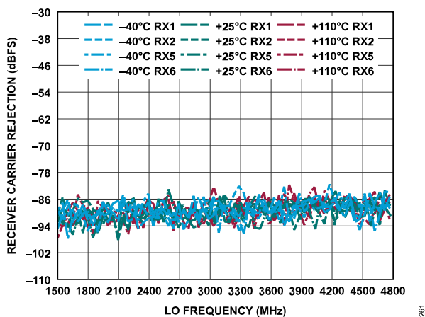
Figure 371. Receiver Carrier Rejection vs. LO Frequency
