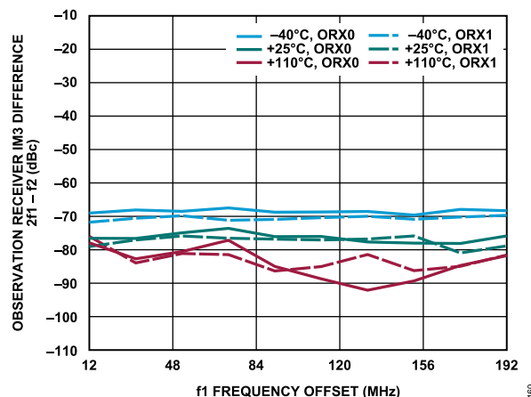
Figure 60. Observation Receiver IM3 Difference, 2f_1 - f_2 vs. f_1 Frequency Offset, -13 dBFS Signal Level Per Tone, f_2 = 852 MHz
