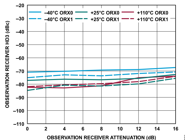
Figure 123. Observation Receiver HD3 vs. Observation Receiver Attenuation, 80 MHz Offset, -10 dBFS Input Signal
