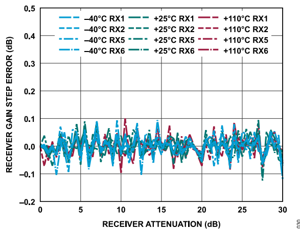
Figure 91. Receiver Gain Step Error vs. Receiver Attenuation, 30 MHz Offset, -1 dBFS Input Signal
