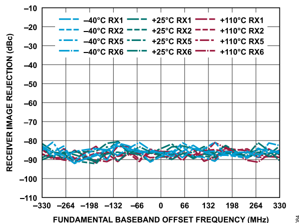
Figure 144. Receiver Image Rejection vs. Fundamental Baseband Offset Frequency, -1 dBFS Input Signal
