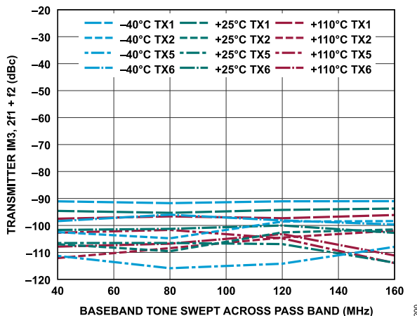
Figure 260. Transmitter IM3, 2f_1 + f_2 vs. Baseband Tone Swept Across Pass Band, -15 dBFS Signal Level Per Tone, f_2 = f_1 + 5 MHz
