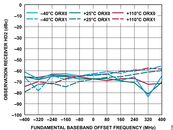
Figure 296. Observation Receiver HD2 vs. Fundamental Baseband Offset Frequency, -10 dBFS Input Signal
