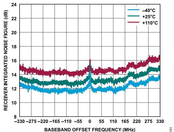
Figure 211. Receiver Integrated Noise Figure vs. Baseband Offset Frequency, 200 kHz Integration Steps, 983.04 MSPS Sample Rate
