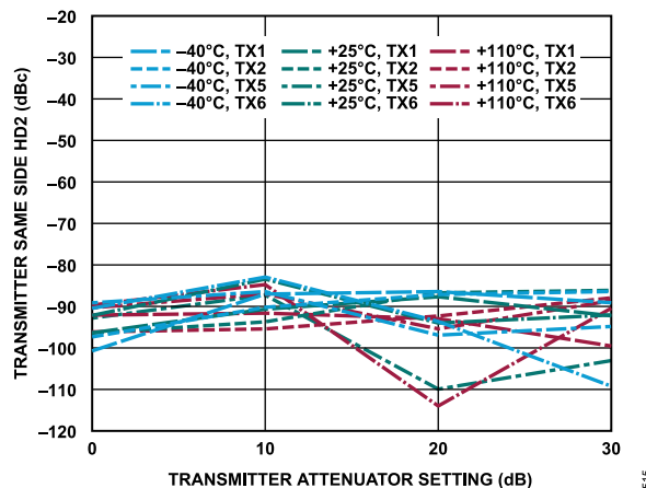
Figure 315. Transmitter Same Side HD2 vs. Transmitter Attenuator Setting, 165 MHz Offset, -12 dBFS Continuous Wave Signal
