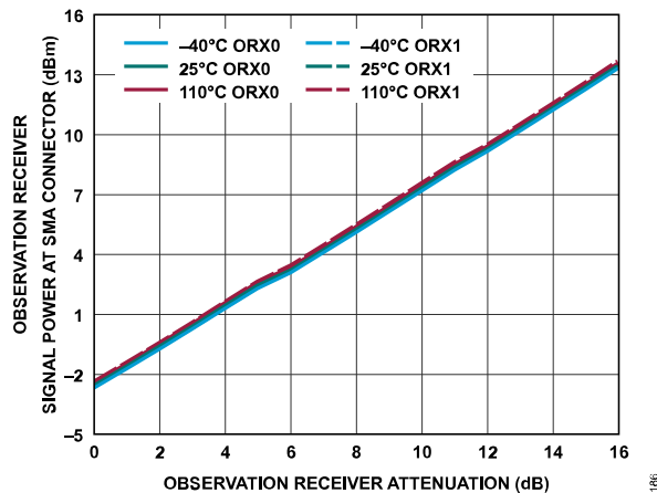
Figure 246. Observation Receiver Signal Power at SMA Connector vs. Observation Receiver Attenuation, 80 MHz Offset, -10 dBFS Input Signal
