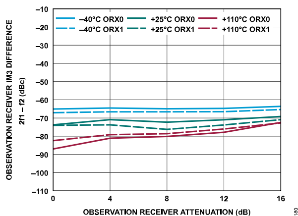
Figure 240. Observation Receiver IM3 Difference, 2f_1 - f_2 vs. Observation Receiver Attenuation, -13 dBFS Signal Level Per Tone, f_1 = 3502 MHz, f_2 = 3712 MHz
