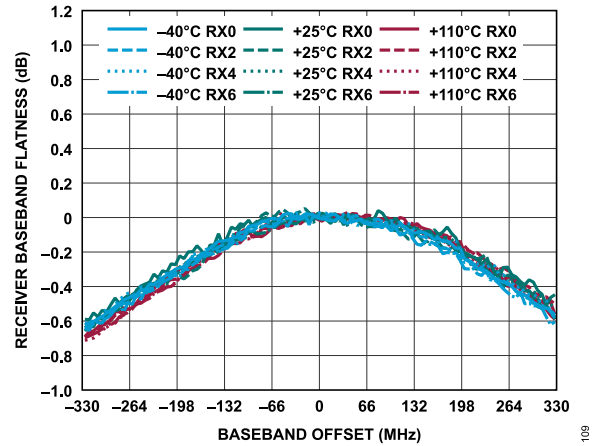
Figure 169. Receiver Baseband Flatness vs. Baseband Offset
