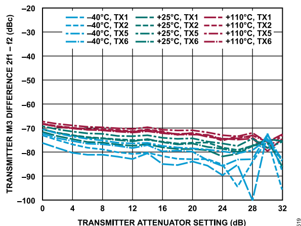
Figure 319. Transmitter IM3 Difference, 2f_1 - f_2 vs. Transmitter Attenuator Setting, -15 dBFS Signal Level Per Tone, f_1 = 160 MHz Offset, f_2 = 2 MHz Offset
