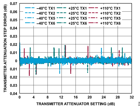
Figure 75. Transmitter Attenuation Step Error vs. Transmitter Attenuation Setting, 30 MHz Offset, -12 dBFS Continuous Wave Signal
