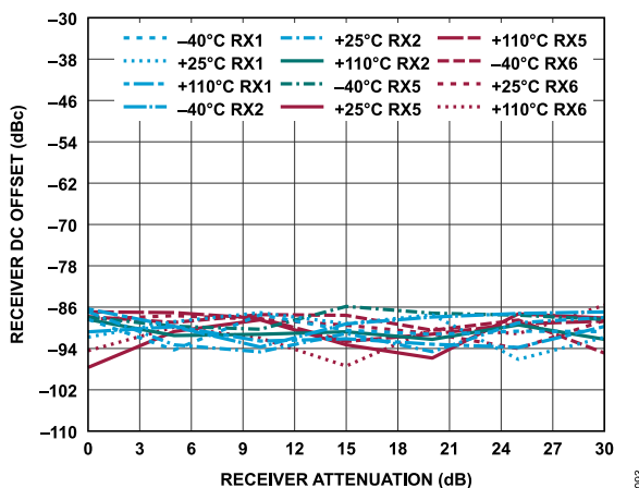
Figure 153. Receiver DC Offset vs. Receiver Attenuation, 30 MHz Offset, -1 dBFS Input Signal
