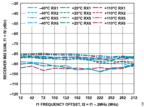
Figure 219. Receiver IM2 Sum, f_1 + f_2 vs. f_1 Frequency Offset, -7 dBFS Signal Level Per Tone, f_2 = f_1 - 2 MHz Offset
