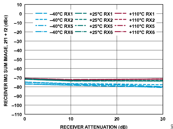
Figure 103. Receiver IM3 Sum Image, 2f_1 + f_2 vs. Receiver Attenuation, -7 dBFS Signal Level per Tone, f_1 = 42 MHz Offset, f_2 = 2 MHz Offset
