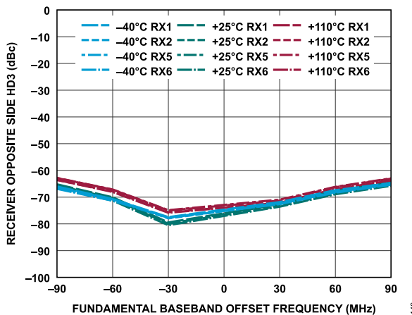
Figure 208. Receiver Opposite Side HD3 vs. Fundamental Baseband Offset Frequency, -1 dBFS Input Signal
