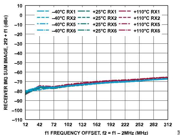
Figure 228. Receiver IM3 Sum Image, 2f_2 + f_1 vs. f_1 Frequency Offset, -7 dBFS Signal Level Per Tone, f_2 = f_1 - 2 MHz
