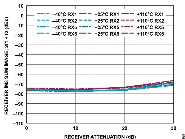
Figure 225. Receiver IM3 Sum Image, 2f_1 + f_2 vs. Receiver Attenuation, -7 dBFS Signal Level Per Tone, f_1 = 42 MHz Offset, f_2 = 2 MHz Offset
