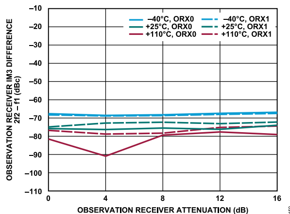
Figure 59. Observation Receiver IM3 Difference, 2f_2 - f_1 vs. Observation Receiver Attenuation, -13 dBFS Signal Level Per Tone, f_1 = 852 MHz, f_2 = 1062 MHz
