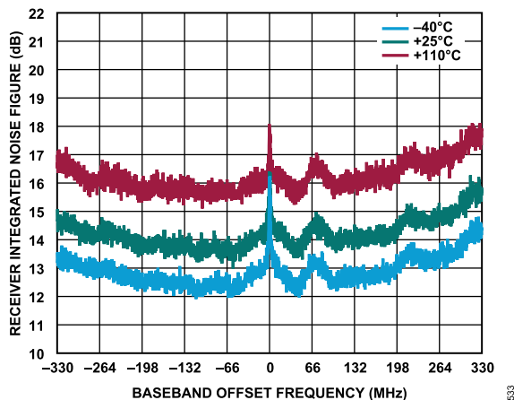
Figure 333. Receiver Integrated Noise Figure vs. Baseband Offset Frequency, 200 kHz Integration Steps, 983.04 MSPS Sample Rate
