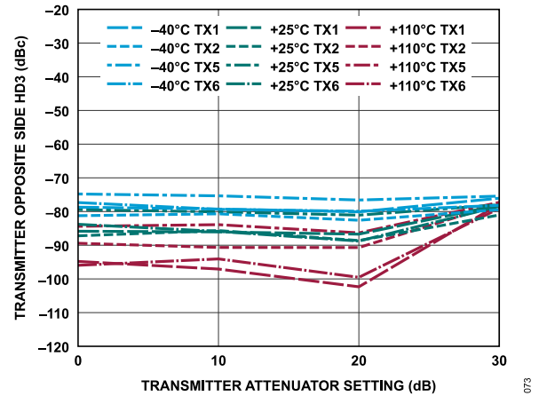
Figure 133. Transmitter Opposite Side HD3 vs. Transmitter Attenuation Setting, 30 MHz Offset, -12 dBFS Continuous Wave Signal
