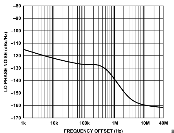
Figure 51. LO Phase Noise vs. Frequency Offset, Loop Bandwidth = 500 kHz, Phase Margin = 55°
