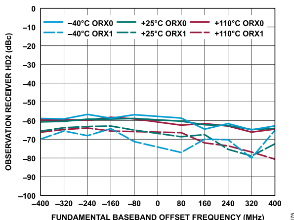
Figure 235. Observation Receiver HD2 vs. Fundamental Baseband Offset Frequency, -10 dBFS Input Signal
