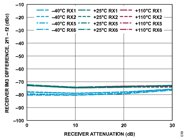
Figure 99. Receiver IM3 Difference, 2f_1 - f_2 vs. Receiver Attenuation, -7 dBFS Signal Level per Tone, f_1 = 42 MHz Offset, f_2 = 2 MHz Offset
