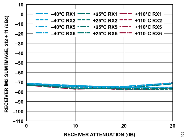
Figure 165. Receiver IM3 Sum, 2f_2 + f_1 vs. Receiver Attenuation, -7 dBFS Signal Level Per Tone, f_1 = 42 MHz Offset, f_2 = 2 MHz Offset
