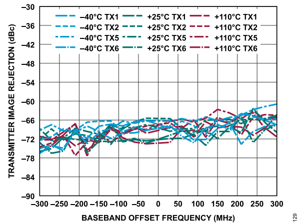
Figure 189. Transmitter Image Rejection vs. Baseband Offset Frequency, -6 dBFS Continuous Wave Signal
