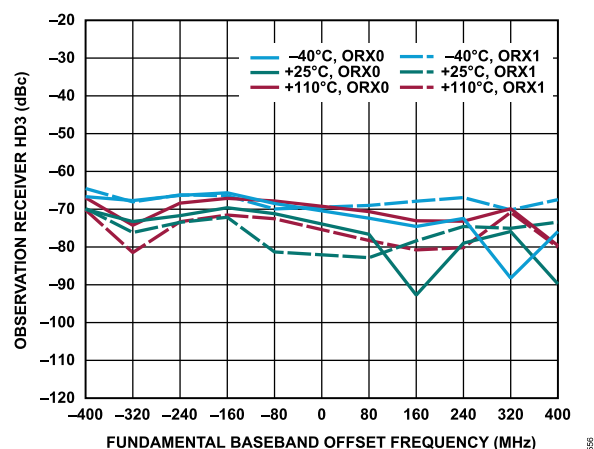
Figure 356. Observation Receiver HD3 vs. Fundamental Baseband Offset Frequency, -10 dBFS Input Signal
