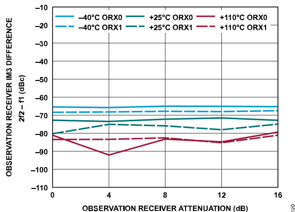
Figure 180. Observation Receiver IM3 Difference, 2f_2 - f_1 vs. Observation Receiver Attenuation, -13 dBFS Signal Level Per Tone, f_1 = 2602 MHz, f_2 = 2812 MHz
