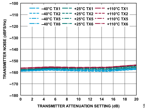
Figure 186. Transmitter Noise vs. Transmitter Attenuation Setting, 150 MHz Offset
