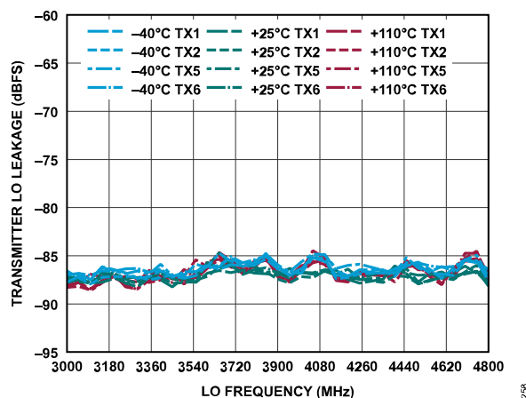
Figure 368. Transmitter LO Leakage vs. LO Frequency
