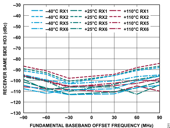
Figure 271. Receiver Same Side HD3 vs. Fundamental Baseband Offset Frequency, -1 dBFS Input Signal
