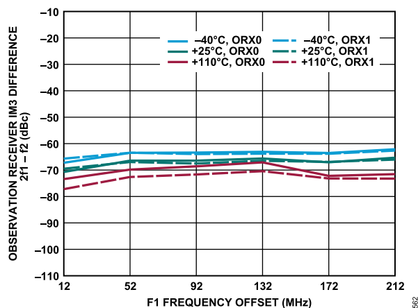
Figure 362. Observation Receiver IM3, 2f_1 - f_2 vs. f_1 Frequency Offset, f_2 = 2 MHz, -13 dBFS Signal Level Per Tone
