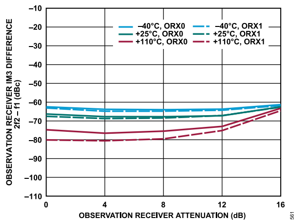
Figure 361. Observation Receiver IM3, 2f_2 - f_1 vs. Observation Receiver Attenuation, -13 dBFS Signal Level Per Tone, f_1 = 5602 MHz, f_2 = 5812 MHz
