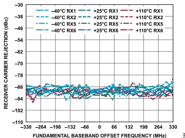
Figure 204. Receiver Carrier Rejection vs. Fundamental Baseband Offset Frequency, -1 dBFS Input Signal
