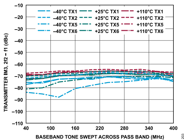
Figure 263. Transmitter IM3, 2f_2 - f_1 vs. Baseband Tone Swept Across Pass Band, -15 dBFS Signal Level Per Tone, f_2 = f_1 + 5 MHz
