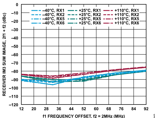
Figure 45. Receiver IM3 Sum Image, 2f_1 + f_2 vs. f_1 Frequency Offset, -7 dBFS Signal Level Per Tone, f_2 = 2 MHz
