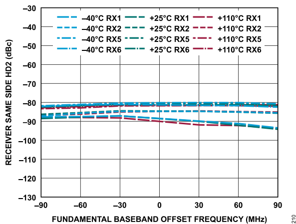
Figure 270. Receiver Same Side HD2 vs. Fundamental Baseband Offset Frequency, -1 dBFS Input Signal
