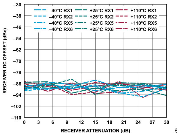
Figure 275. Receiver DC Offset vs. Receiver Attenuation, 30 MHz Offset, -1 dBFS Input Signal
