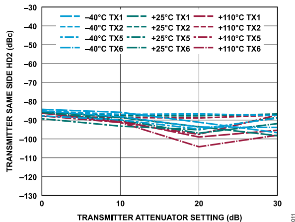
Figure 72. Transmitter Same Side HD2 vs. Transmitter Attenuation Setting, 30 MHz Offset, -12 dBFS Continuous Wave Signal
