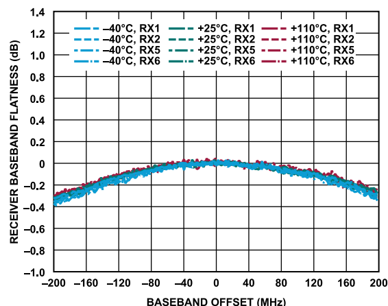
Figure 48. Receiver Baseband Flatness vs. Baseband Offset
