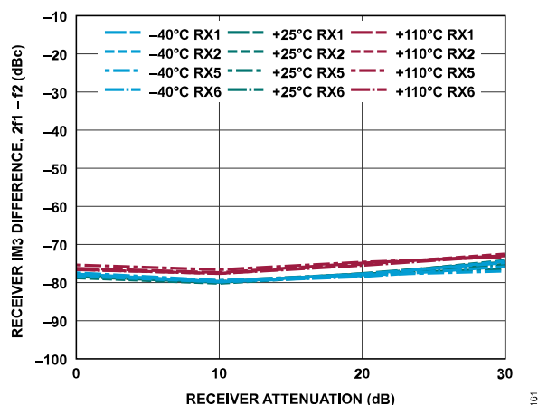
Figure 221. Receiver IM3 Difference, 2f_1 - f_2 vs. Receiver Attenuation, -7 dBFS Signal Level Per Tone, f_1 = 42 MHz Offset, f_2 = 2 MHz Offset
