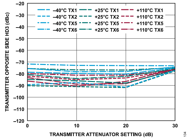
Figure 194. Transmitter Opposite Side HD3 vs. Transmitter Attenuation Setting, 30 MHz Offset, -12 dBFS Continuous Wave Signal
