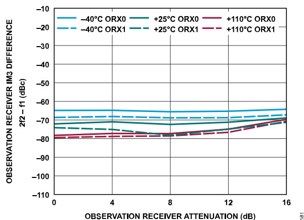
Figure 241. Observation Receiver IM3 Difference, 2f_2 - f_1 vs. Observation Receiver Attenuation, -13 dBFS Signal Level Per Tone, f_1 = 3502 MHz, f_2 = 3712 MHz
