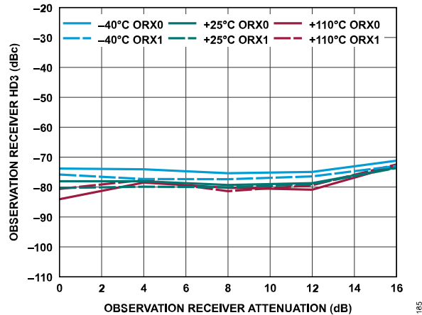
Figure 245. Observation Receiver HD3 vs. Observation Receiver Attenuation, 80 MHz Offset, -10 dBFS Input Signal
