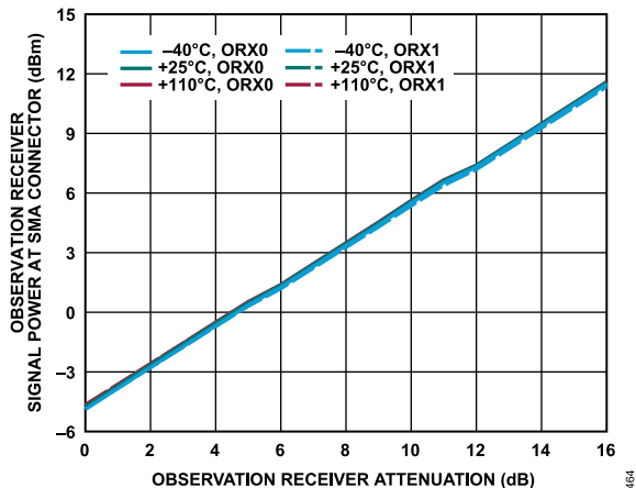
Figure 64. Observation Receiver Signal Power at SMA Connector vs. Observation Receiver Attenuation, 80 MHz Offset, -10 dBFS Input Signal
