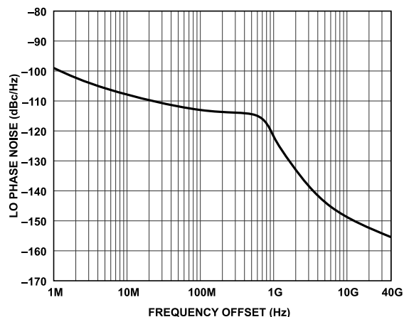
Figure 294. LO Phase Noise vs. Frequency Offset, Loop Bandwidth = 500 kHz, Phase Margin = 55°
