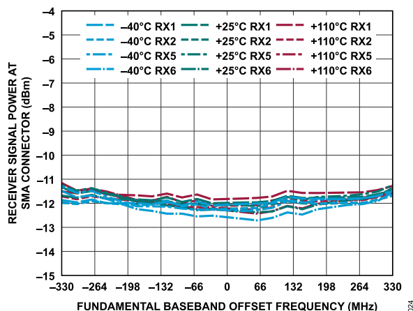
Figure 85. Receiver Signal Power at SMA Connector vs. Fundamental Baseband Offset Frequency, -1 dBFS Input Signal (Match Is Not De-Embedded)
