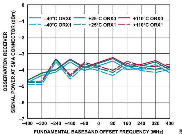
Figure 115. Observation Receiver Signal Power at SMA Connector vs. Fundamental Baseband Offset Frequency, -10 dBFS Input Signal (Match Is Not De-Embedded)
