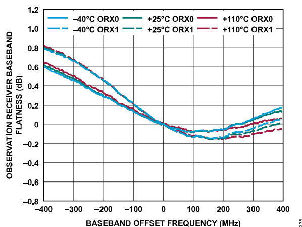
Figure 295. Observation Receiver Baseband Flatness vs. Baseband Offset Frequency, -10 dBFS Input Signal
