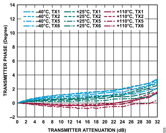
Figure 325. Transmitter Phase vs. Transmitter Attenuation
