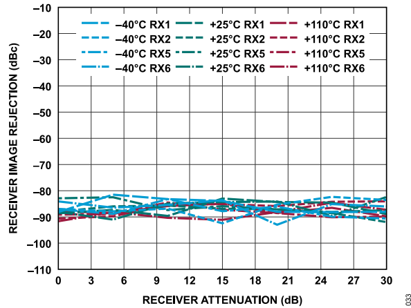
Figure 94. Receiver Image Rejection vs. Receiver Attenuation, 30 MHz Offset, -1 dBFS Input Signal
