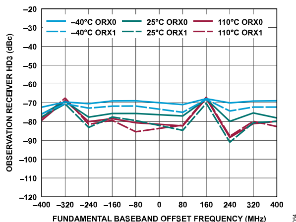
Figure 114. Observation Receiver HD3 vs. Fundamental Baseband Offset Frequency, -10 dBFS Input Signal
