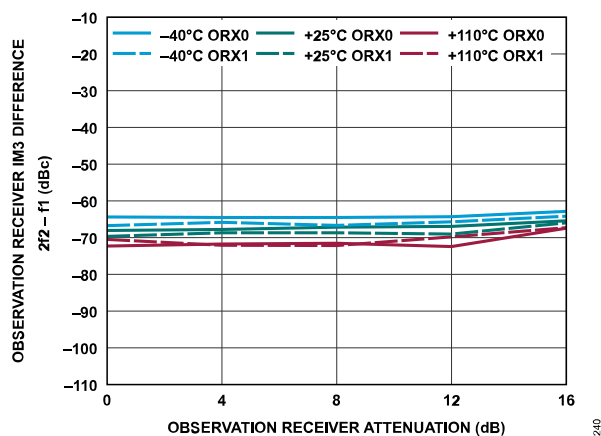
Figure 300. Observation Receiver IM3 Difference, 2f_2 - f_1 vs. Observation Receiver Attenuation, -13 dBFS Signal Level Per Tone, f_1 = 3502 MHz, f_2 = 3512 MHz
