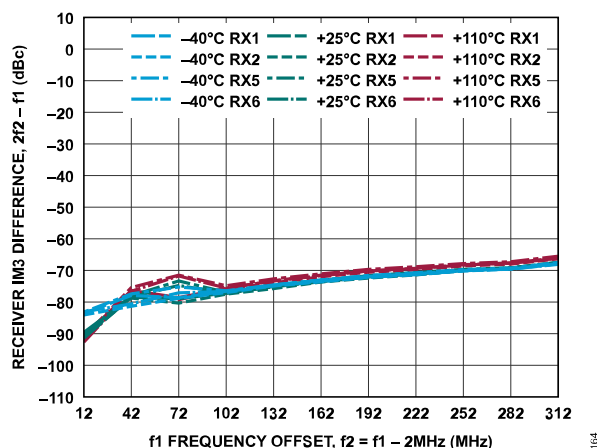
Figure 224. Receiver IM3 Difference, 2f_2 - f_1 vs. f_1 Frequency Offset, -7 dBFS Signal Level Per Tone, f_2 = f_1 - 2 MHz
