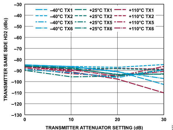
Figure 193. Transmitter Same Side HD2 vs. Transmitter Attenuation Setting, 30 MHz Offset, -12 dBFS Continuous Wave Signal
