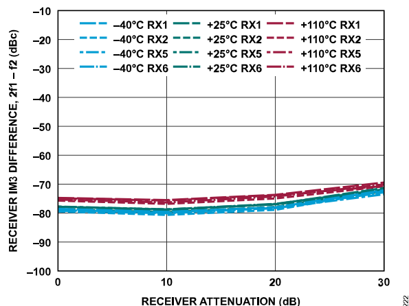
Figure 282. Receiver IM3 Difference, 2f_1 - f_2 vs. Receiver Attenuation, -7 dBFS Signal Level Per Tone, f_1 = 42 MHz Offset, f_2 = 2 MHz Offset
