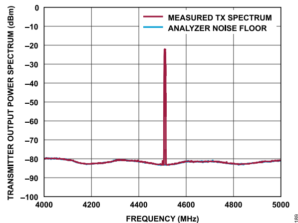
Figure 249. Transmitter Output Power Spectrum, Tx0, 5MHz LTE, 10 MHz Offset, -10 dBFS RMS, 1 MHz Resolution Bandwidth, T_j = 25^\circ\text{C}
