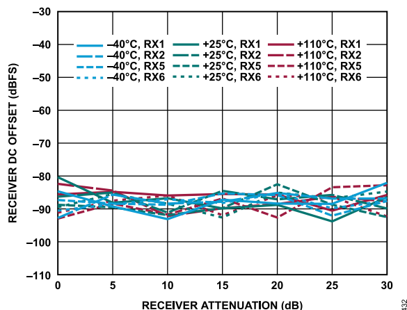
Figure 32. Receiver DC Offset vs. Receiver Attenuation, 30 MHz Offset, -1 dBFS Input Signal
