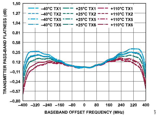
Figure 187. Transmitter Pass-Band Flatness vs. Baseband Offset Frequency
