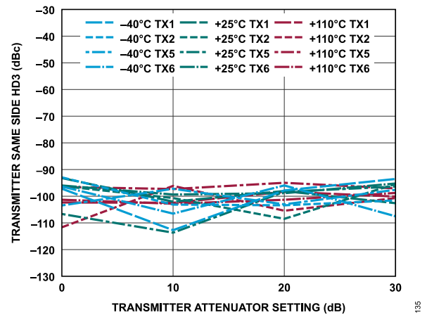
Figure 195. Transmitter Same Side HD3 vs. Transmitter Attenuation Setting, 30 MHz Offset, -12 dBFS Continuous Wave Signal
