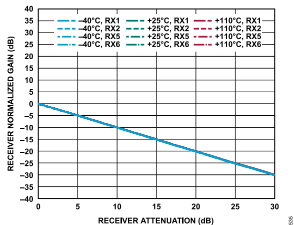
Figure 335. Receiver Normalized Gain vs. Receiver Attenuation, 30 MHz Offset, -1 dBFS Input Signal
