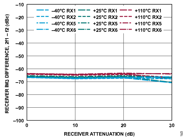
Figure 220. Receiver IM3 Difference, 2f_1 + f_2 vs. Receiver Attenuation, -7 dBFS Signal Level Per Tone, f_2 = f_1 - 2 MHz
