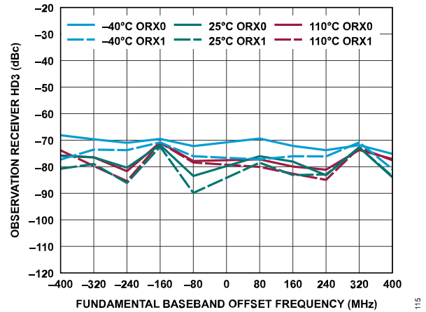
Figure 175. Observation Receiver HD3 vs. Fundamental Baseband Offset Frequency, -10 dBFS Input Signal
