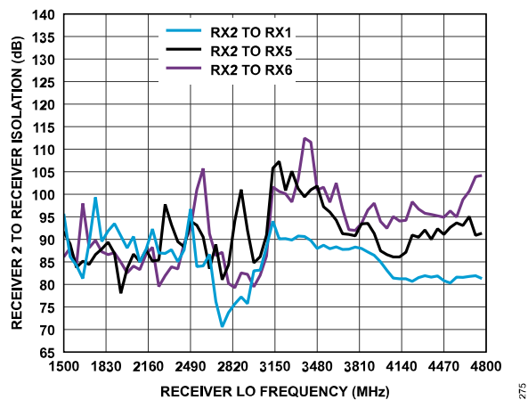
Figure 385. Receiver 2 to Receiver Isolation vs. Receiver LO Frequency
