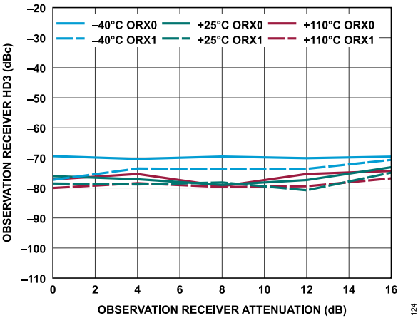
Figure 184. Observation Receiver HD3 vs. Observation Receiver Attenuation, 80 MHz Offset, -10 dBFS Input Signal
