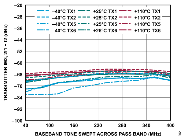
Figure 262. Transmitter IM3, 2f_1 - f_2 vs. Baseband Tone Swept Across Pass Band, -15 dBFS Signal Level Per Tone, f_2 = f_1 + 5 MHz
