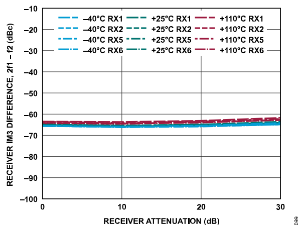
Figure 159. Receiver IM3 Difference, 2f_1 + f_2 vs. Receiver Attenuation, -7 dBFS Signal Level Per Tone, f_2 = f_1 - 2 MHz
