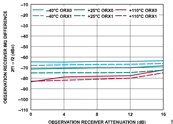
Figure 118. Observation Receiver IM3 Difference, 2f_1 - f_2 vs. Observation Receiver Attenuation, -13 dBFS Signal Level Per Tone, f_1 = 1802 MHz, f_2 = 2012 MHz
