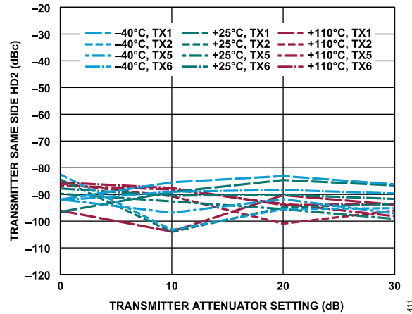
Figure 11. Transmitter Same Side HD2 vs. Transmitter Attenuator Setting, 30 MHz Offset, -12 dBFS Continuous Wave Signal
