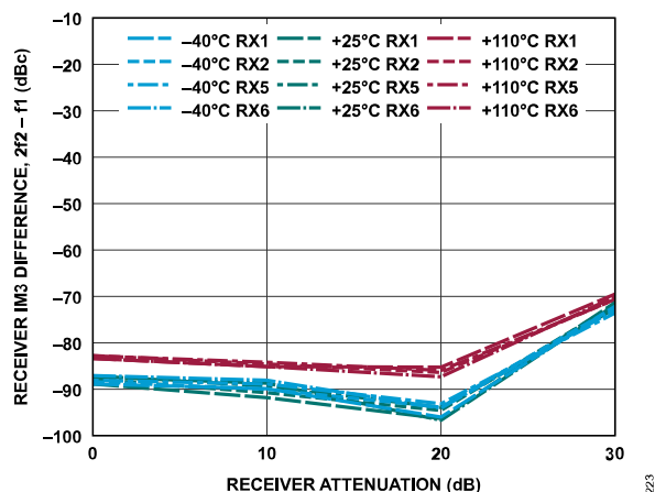
Figure 283. Receiver IM3 Difference, 2f_2 - f_1 vs. Receiver Attenuation, -7 dBFS Signal Level Per Tone, f_1 = 42 MHz Offset, f_2 = 2 MHz Offset
