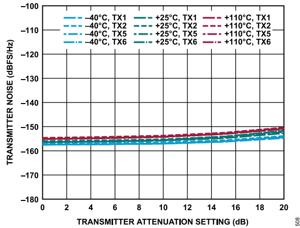
Figure 308. Transmitter Noise vs. Transmitter Attenuation Setting, 165 MHz Offset
