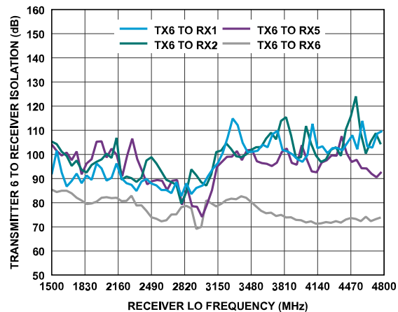
Figure 381. Transmitter 6 to Receiver Isolation vs. Receiver LO Frequency
