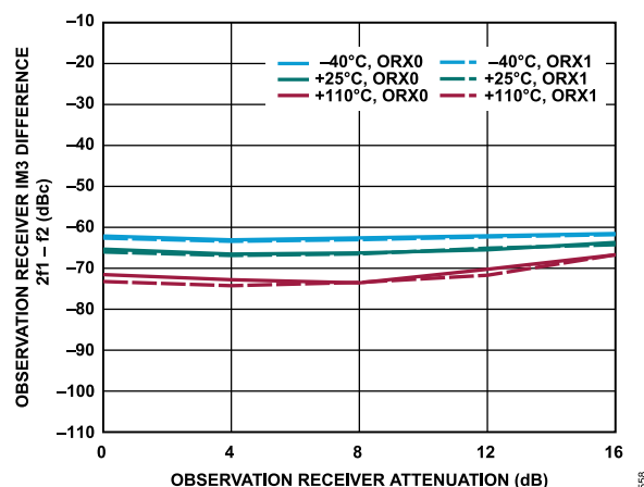
Figure 358. Observation Receiver IM3, 2f_1 - f_2 vs. Observation Receiver Attenuation, -13 dBFS Signal Level Per Tone, f_1 = 5602 MHz, f_2 = 5612 MHz
