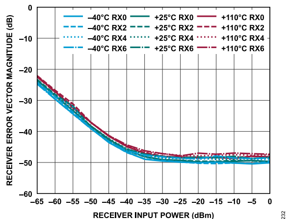
Figure 292. Receiver Error Vector Magnitude vs. Receiver Input Power, 20 MHz LTE Centered Around DC, TDD Mode, AGC Enabled
