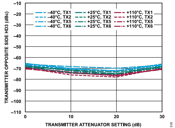
Figure 316. Transmitter Opposite Side HD3 vs. Transmitter Attenuator Setting, 110 MHz Offset, -12 dBFS Continuous Wave Signal
