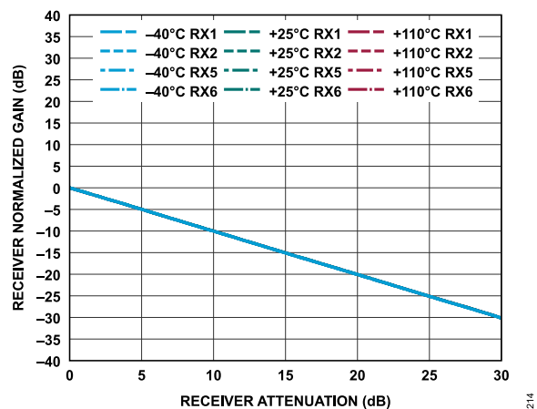
Figure 274. Receiver Normalized Gain vs. Receiver Attenuation, 30 MHz Offset, -1 dBFS Input Signal
