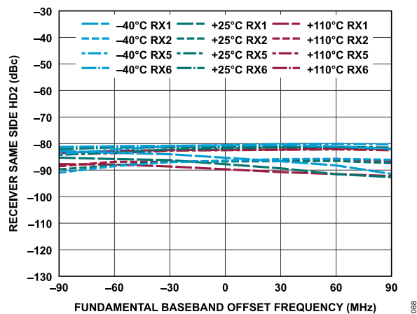
Figure 148. Receiver Same Side HD2 vs. Fundamental Baseband Offset Frequency, -1 dBFS Input Signal
