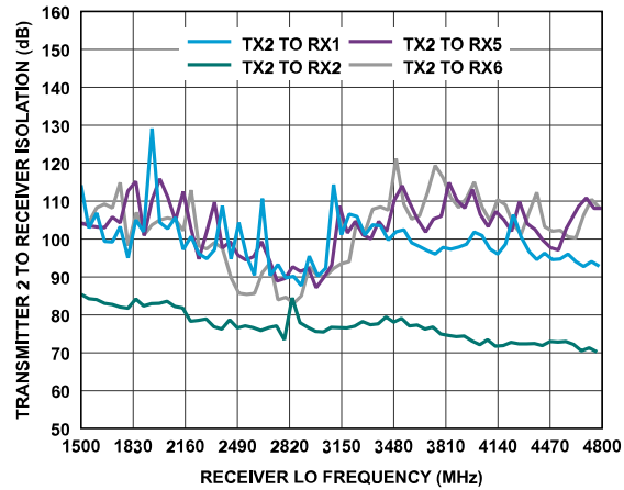
Figure 379. Transmitter 2 to Receiver Isolation vs. Receiver LO Frequency
