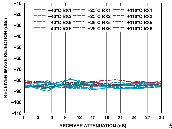
Figure 276. Receiver Image Rejection vs. Receiver Attenuation, 30 MHz Offset, -1 dBFS Input Signal
