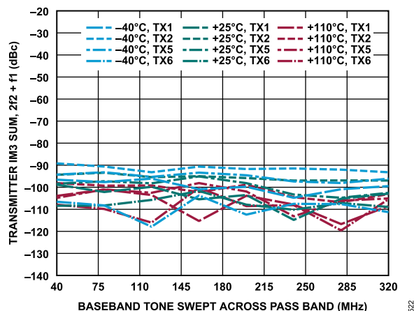
Figure 322. Transmitter IM3 Sum, 2f_2 + f_1 vs. Baseband Tone Swept Across Pass Band, -15 dBFS Signal Level Per Tone, f_2 = 5 MHz
