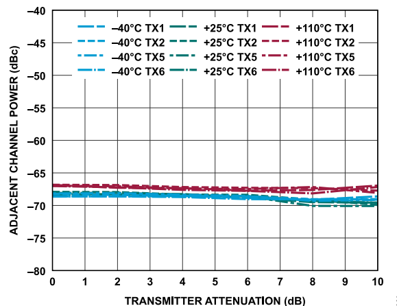
Figure 129. Adjacent Channel Power vs. Transmitter Attenuation, 290 MHz Offset, 20 MHz LTE, PAR = 12 dB
