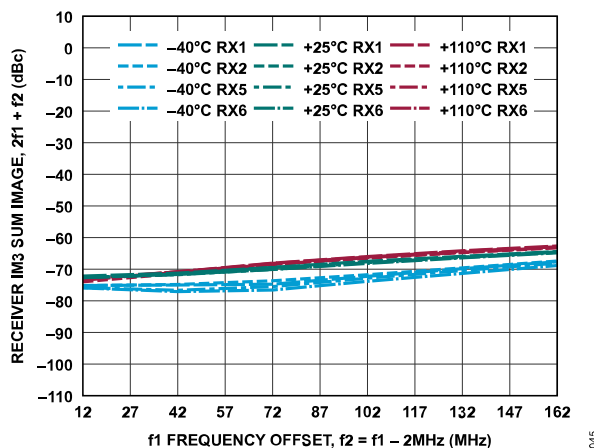
Figure 105. Receiver IM3 Sum Image, 2f_1 + f_2 vs. f_1 Frequency Offset, -7 dBFS Signal Level per Tone, f_2 = f_1 - 2 MHz
