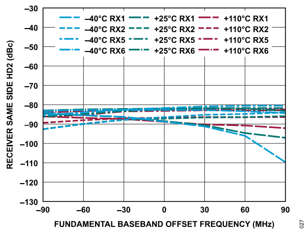
Figure 88. Receiver Same Side HD2 vs. Fundamental Baseband Offset Frequency, -1 dBFS Input Signal
