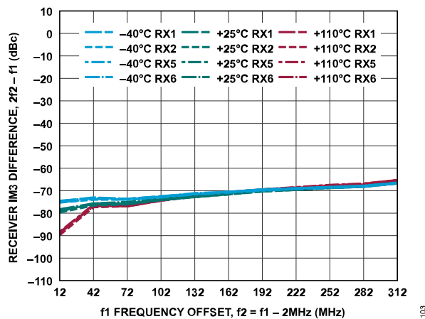
Figure 163. Receiver IM3 Difference, 2f_2 - f_1 vs. f_1 Frequency Offset, -7 dBFS Signal Level Per Tone, f_2 = f_1 - 2 MHz
