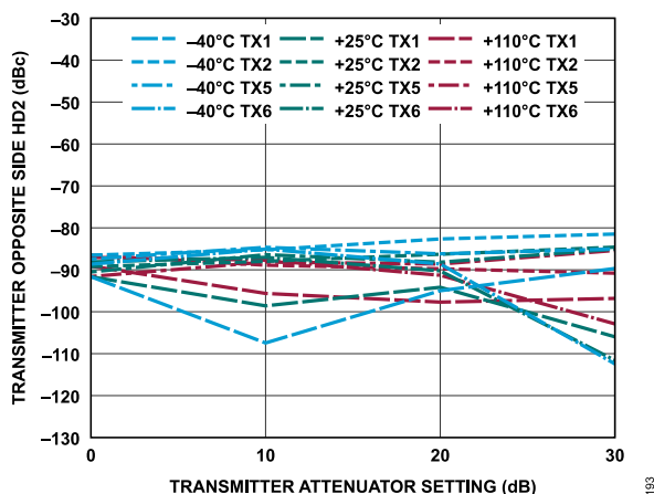
Figure 253. Transmitter Opposite Side HD2 vs. Transmitter Attenuation Setting, 30 MHz Offset, -12 dBFS Continuous Wave Signal
