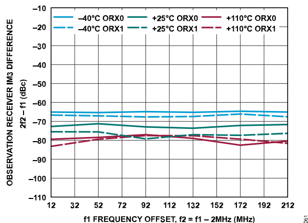
Figure 121. Observation Receiver IM3 Difference, 2f_2 - f_1 vs. f_1 Frequency Offset, -13 dBFS Signal Level per Tone, f_2 = f_1 - 2 MHz
