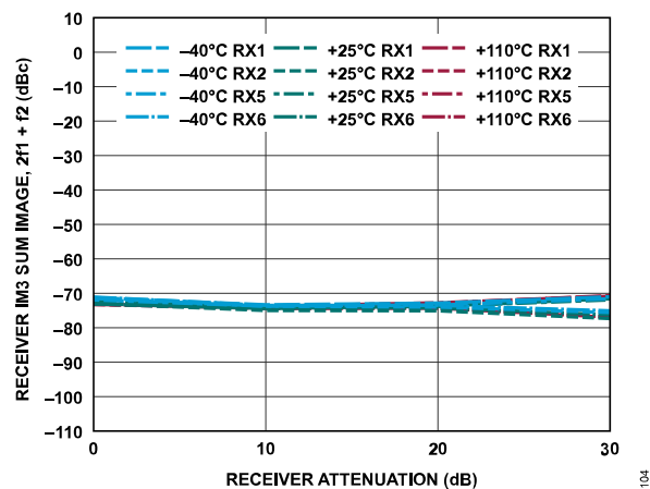
Figure 164. Receiver IM3 Sum, 2f_1 + f_2 vs. Receiver Attenuation, -7 dBFS Signal Level Per Tone, f_1 = 42 MHz Offset, f_2 = 2 MHz Offset
