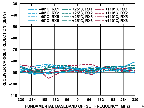
Figure 326. Receiver Carrier Rejection vs. Fundamental Baseband Offset Frequency, -1 dBFS Input Signal
