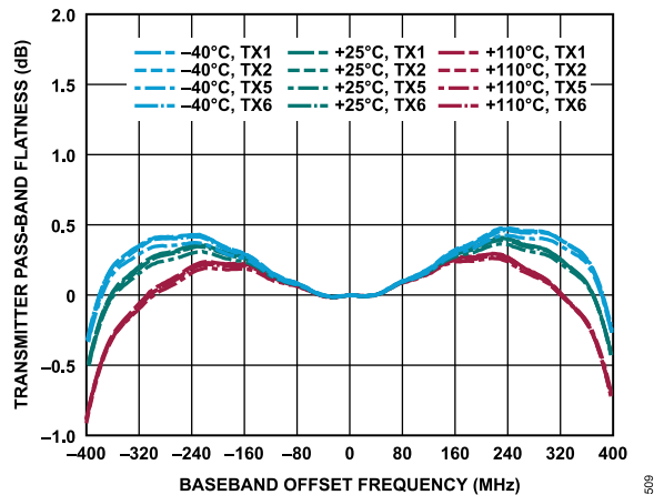
Figure 309. Transmitter Pass-Band Flatness vs. Baseband Offset Frequency
