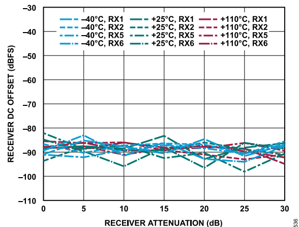
Figure 336. Receiver DC Offset vs. Receiver Attenuation, 30 MHz Offset, -1 dBFS Input Signal
