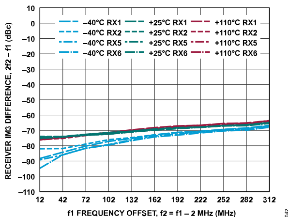
Figure 102. Receiver IM3 Difference, 2f_2 - f_1 vs. f_1 Frequency Offset, -7 dBFS Signal Level per Tone, f_2 = f_1 - 2 MHz
