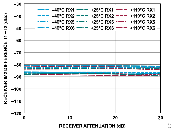
Figure 277. Receiver IM2 Difference, f_1 - f_2 vs. Receiver Attenuation, -7 dBFS Signal Level Per Tone, f_1 = 42 MHz Offset, f_2 = 2 MHz Offset
