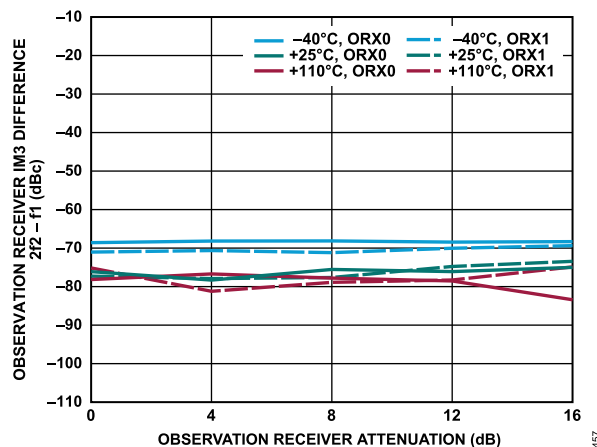
Figure 57. Observation Receiver IM3 Difference, 2f_2 - f_1 vs. Observation Receiver Attenuation, -13 dBFS Signal Level Per Tone, f_1 = 852 MHz, f_2 = 862 MHz
