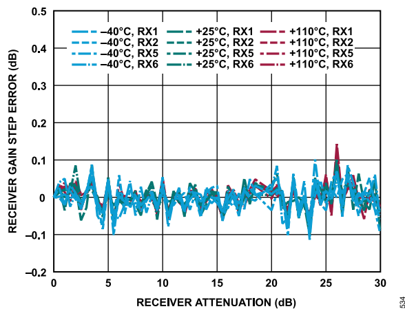
Figure 334. Receiver Gain Step Error vs. Receiver Attenuation, 30 MHz Offset, -1 dBFS Input Signal
