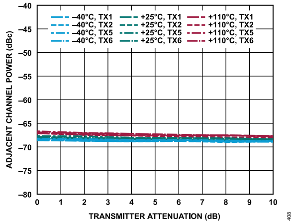
Figure 8. Adjacent Channel Power vs. Transmitter Attenuation, 90 MHz Offset, 20 MHz LTE, PAR = 12 dB
