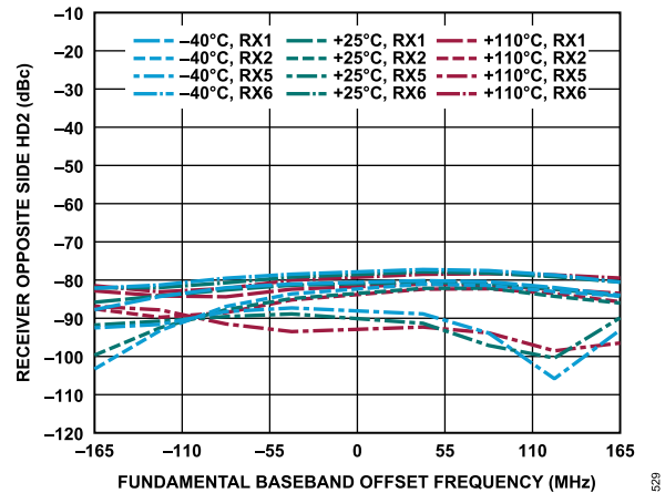
Figure 329. Receiver Opposite Side HD2 vs. Fundamental Baseband Offset Frequency, -1 dBFS Input Signal
