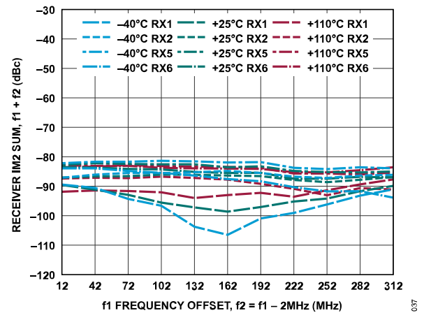
Figure 98. Receiver IM2 Sum, f_1 + f_2 vs. f_1 Frequency Offset, -7 dBFS Signal Level per Tone, f_2 = f_1 - 2 MHz
