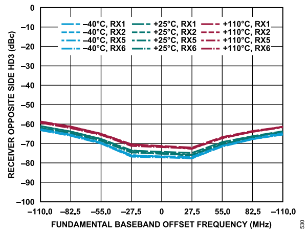
Figure 330. Receiver Opposite Side HD3 vs. Fundamental Baseband Offset Frequency, -1 dBFS Input Signal
