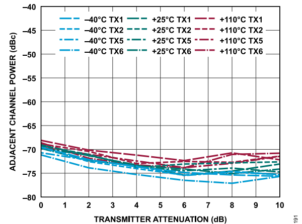
Figure 251. Adjacent Channel Power vs. Transmitter Attenuation, 290 MHz Offset, 20 MHz LTE, PAR = 12 dB
