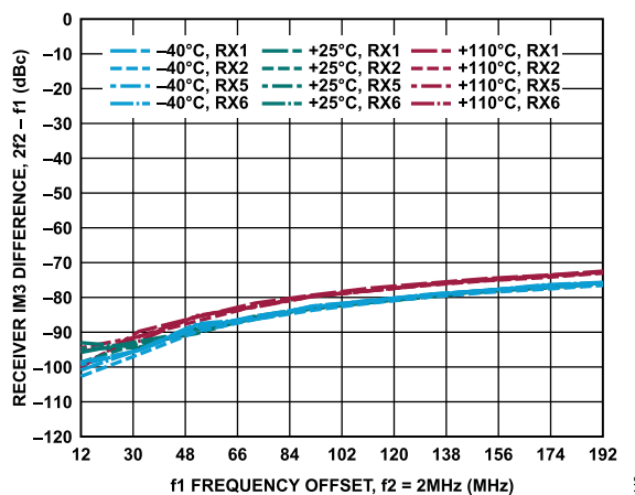
Figure 42. Receiver IM3 Difference, 2f_2 - f_1 vs. f_1 Frequency Offset, -7 dBFS Signal Level Per Tone, f_2 = 2 MHz
