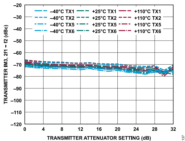
Figure 197. Transmitter IM3, 2f_1 - f_2 vs. Transmitter Attenuation Setting, -15 dBFS Signal Level Per Tone, f_1 = 160 MHz Offset, f_2 = 165 MHz Offset
