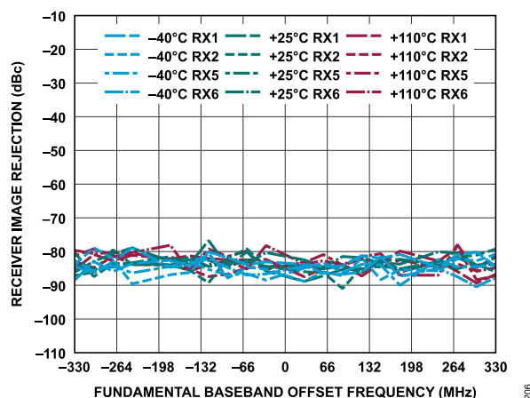
Figure 266. Receiver Image Rejection vs. Fundamental Baseband Offset Frequency, -1 dBFS Input Signal
