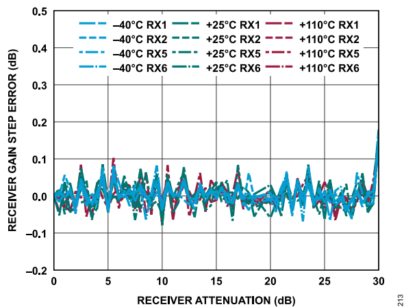
Figure 273. Receiver Gain Step Error vs. Receiver Attenuation, 30 MHz Offset, -1 dBFS Input Signal
