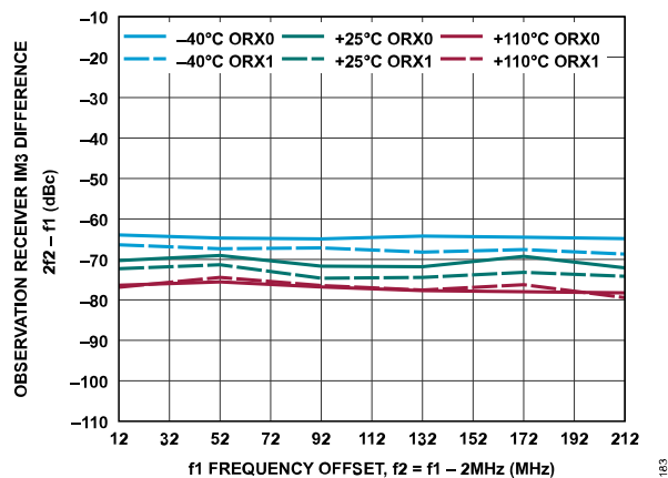
Figure 243. Observation Receiver IM3 Difference, 2f_2 - f_1 vs. f_1 Frequency Offset, -13 dBFS Signal Level Per Tone, f_2 = f_1 - 2 MHz
