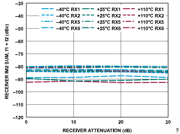
Figure 218. Receiver IM2 Sum, f_1 + f_2 vs. Receiver Attenuation, -7 dBFS Signal Level Per Tone, f_1 = 42 MHz Offset, f_2 = 2 MHz Offset
