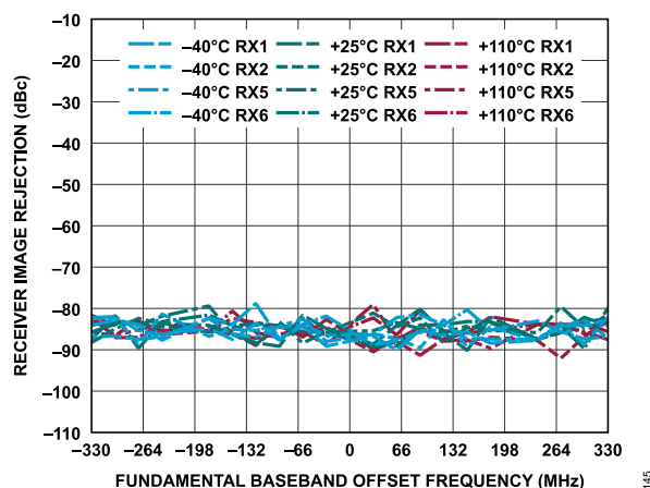
Figure 205. Receiver Image Rejection vs. Fundamental Baseband Offset Frequency, -1 dBFS Input Signal
