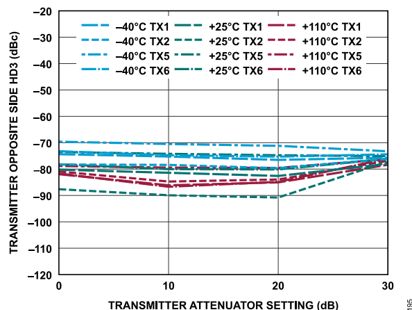
Figure 255. Transmitter Opposite Side HD3 vs. Transmitter Attenuation Setting, 30 MHz Offset, -12 dBFS Continuous Wave Signal
