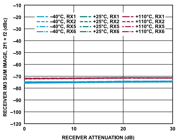
Figure 43. Receiver IM3 Sum Image, 2f_1 + f_2 vs. Receiver Attenuation, -7 dBFS Signal Level Per Tone, f_1 = 99 MHz Offset, f_2 = 2 MHz Offset
