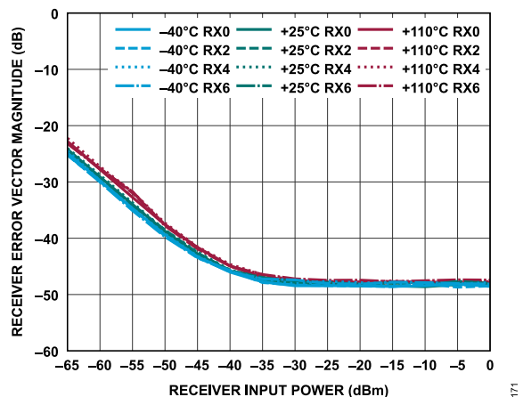
Figure 231. Receiver Error Vector Magnitude vs. Receiver Input Power, 20 MHz LTE Centered Around DC, TDD Mode, AGC Enabled
