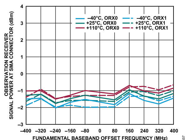
Figure 357. Observation Receiver Signal Power at SMA Connector vs. Fundamental Baseband Offset Frequency, -10 dBFS Input Signal (Match Is Not De-Embedded)
