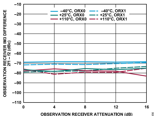
Figure 56. Observation Receiver IM3 Difference, 2f_1 - f_2 vs. Observation Receiver Attenuation, -13 dBFS Signal Level Per Tone, f_1 = 852 MHz, f_2 = 862 MHz
