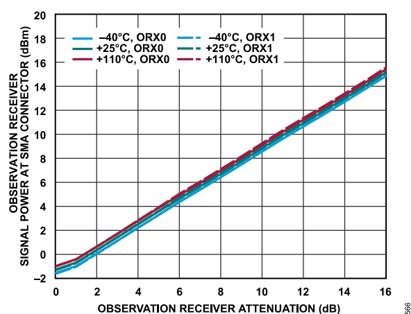
Figure 366. Observation Receiver Signal Power at SMA Connector vs. Observation Receiver Attenuation, 80 MHz Offset, -10 dBFS Input Signal
