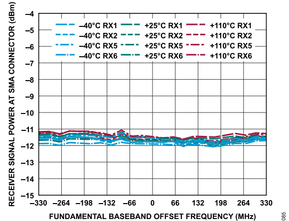
Figure 145. Receiver Signal Power at SMA Connector vs. Fundamental Baseband Offset Frequency, -1 dBFS Input Signal (Match Is Not De-Embedded)
