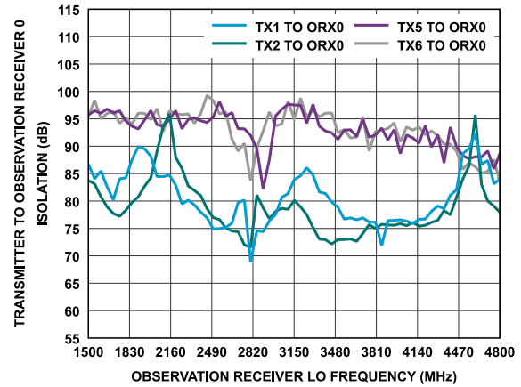
Figure 382. Transmitter to Observation Receiver 0 Isolation vs. Observation Receiver LO Frequency
