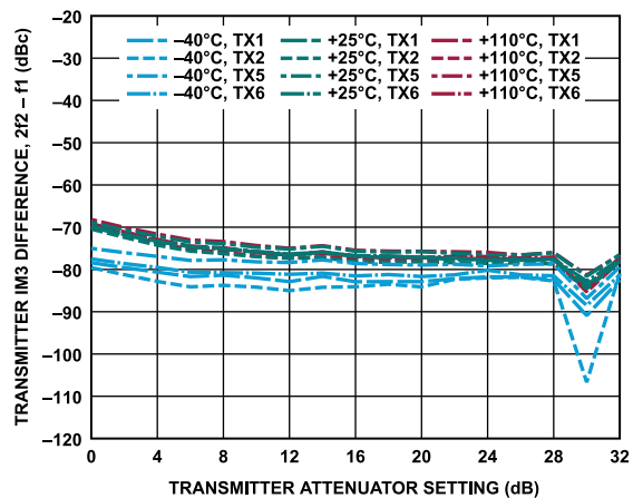
Figure 16. Transmitter IM3 Difference, 2f_2 - f_1 vs. Transmitter Attenuation Setting, -15 dBFS Signal Level Per Tone, f_1 = 180 MHz Offset, f_2 = 185 MHz Offset
