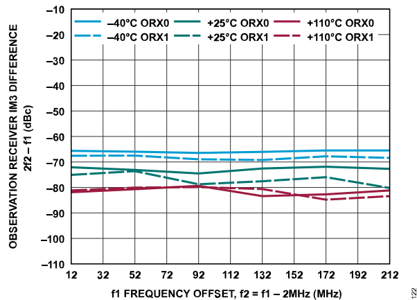
Figure 182. Observation Receiver IM3 Difference, 2f_2 - f_1 vs. f_1 Frequency Offset, -13 dBFS Signal Level Per Tone, f_2 = f_1 - 2 MHz
