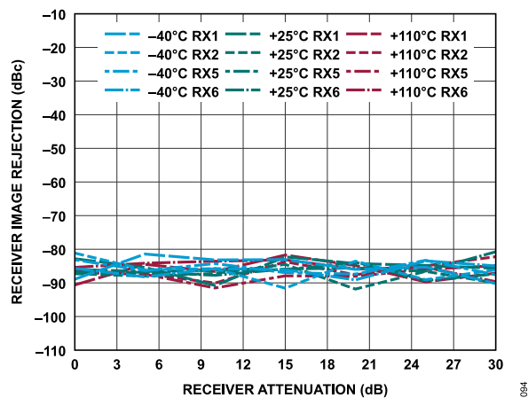
Figure 154. Receiver Image Rejection vs. Receiver Attenuation, 30 MHz Offset, -1 dBFS Input Signal
