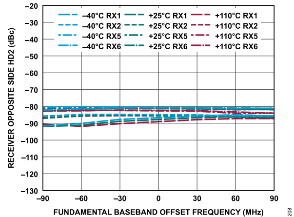
Figure 268. Receiver Opposite Side HD2 vs. Fundamental Baseband Offset Frequency, -1 dBFS Input Signal
