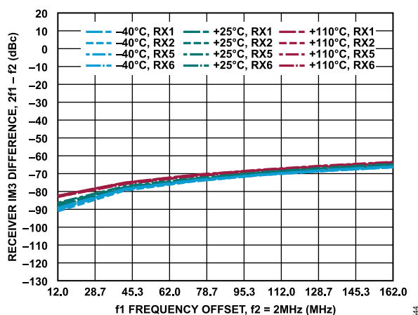
Figure 344. Receiver IM3 Difference, 2f_1 - f_2 vs. f_1 Frequency Offset, f_2 = 2 MHz, -7 dBFS Signal Level Per Tone
