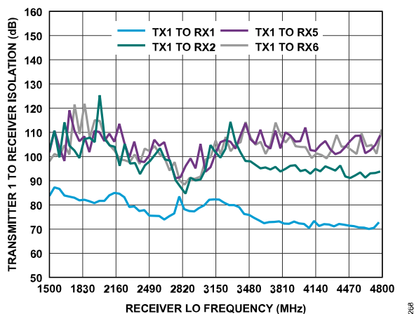
Figure 378. Transmitter 1 to Receiver Isolation vs. Receiver LO Frequency
