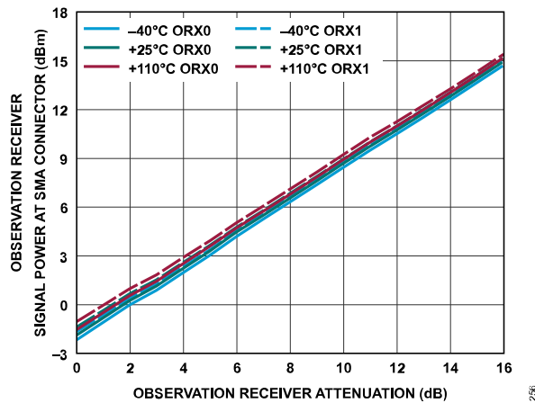
Figure 307. Observation Receiver Signal Power at SMA Connector vs. Observation Receiver Attenuation, 80 MHz Offset, -10 dBFS Input Signal
