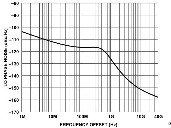
Figure 172. LO Phase Noise vs. Frequency Offset, Loop Bandwidth = 500 kHz, Phase Margin = 55°
