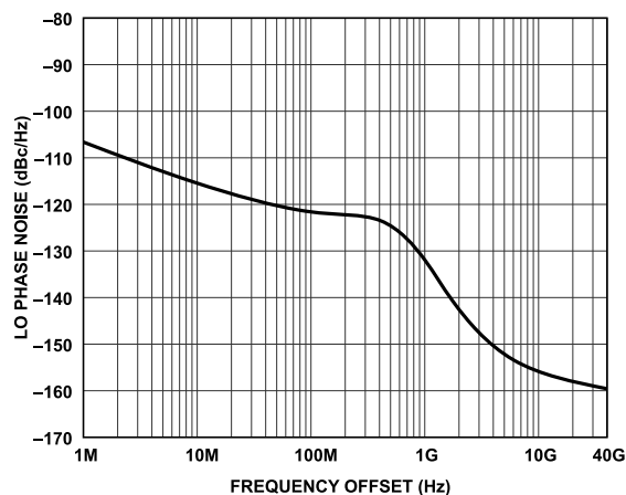
Figure 111. LO Phase Noise vs. Frequency Offset, Loop Bandwidth = 500 kHz, Phase Margin = 55°
