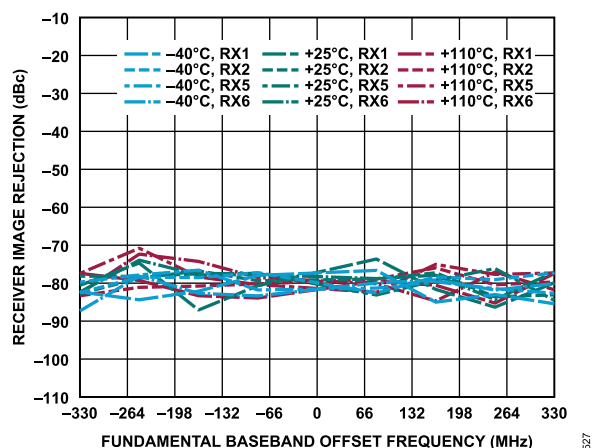
Figure 327. Receiver Image Rejection vs. Fundamental Baseband Offset Frequency, -1 dBFS Input Signal
