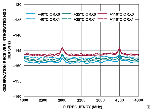
Figure 373. Observation Receiver Integrated NSD vs. Baseband Frequency, 1800 MHz, 5898.24 MSPS Sample Rate
