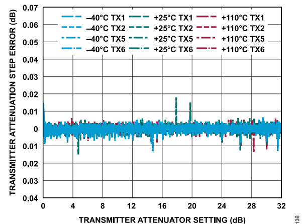
Figure 196. Transmitter Attenuation Step Error vs. Transmitter Attenuation Setting, 30 MHz Offset, -12 dBFS Continuous Wave Signal
