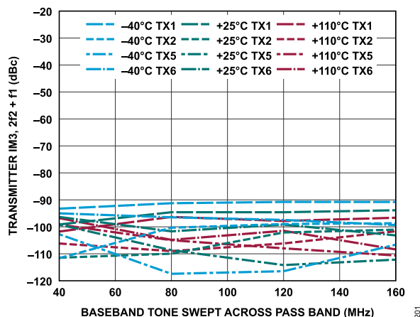
Figure 261. Transmitter IM3, 2f_2 + f_1 vs. Baseband Tone Swept Across Pass Band, -15 dBFS Signal Level Per Tone, f_2 = f_1 + 5 MHz
