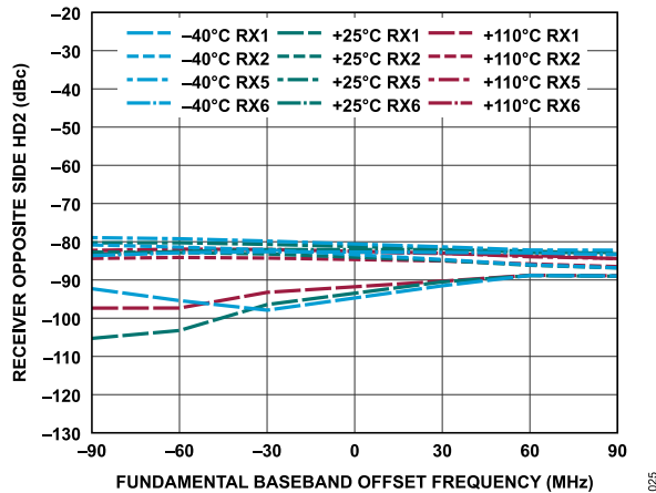
Figure 86. Receiver Opposite Side HD2 vs. Fundamental Baseband Offset Frequency, -1 dBFS Input Signal
