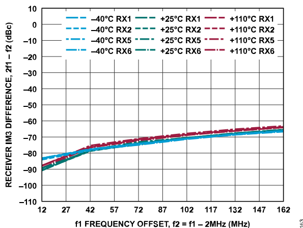
Figure 223. Receiver IM3 Difference, 2f_1 - f_2 vs. f_1 Frequency Offset, -7 dBFS Signal Level Per Tone, f_2 = f_1 - 2 MHz
