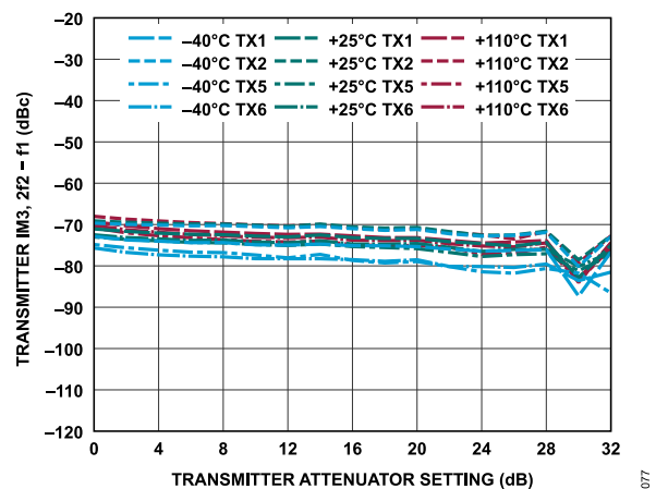
Figure 137. Transmitter IM3, 2f_2 - f_1 vs. Transmitter Attenuation Setting, -15 dBFS Signal Level Per Tone, f_1 = 160 MHz Offset, f_2 = 165 MHz Offset
