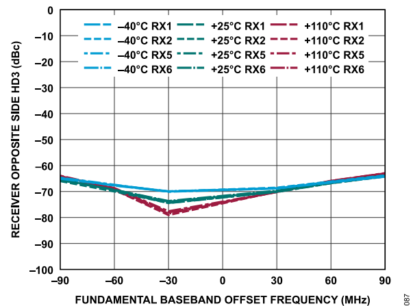
Figure 147. Receiver Opposite Side HD3 vs. Fundamental Baseband Offset Frequency, -1 dBFS Input Signal
