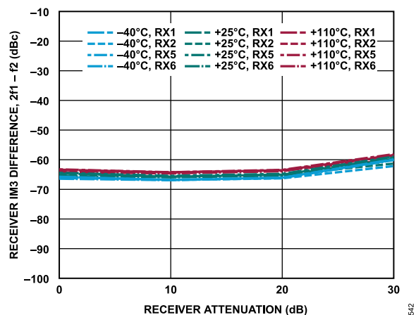
Figure 342. Receiver IM3 Difference, 2f_1 - f_2 vs. Receiver Attenuation, -7 dBFS Signal Level Per Tone, f_1 = 166 MHz Offset, f_2 = 2 MHz Offset
