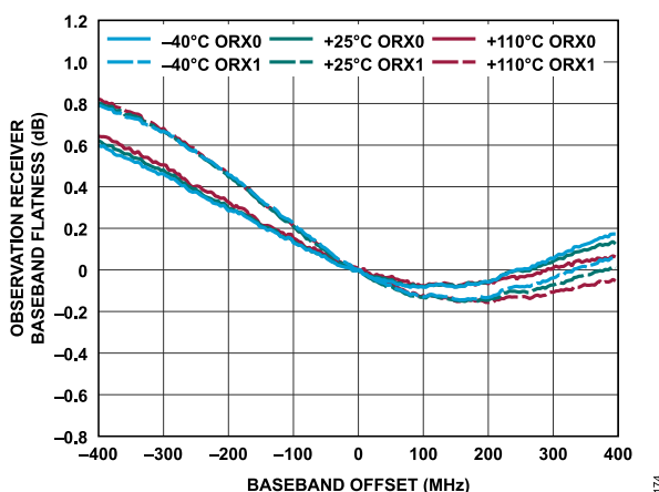
Figure 234. Observation Receiver Baseband Flatness vs. Baseband Offset
