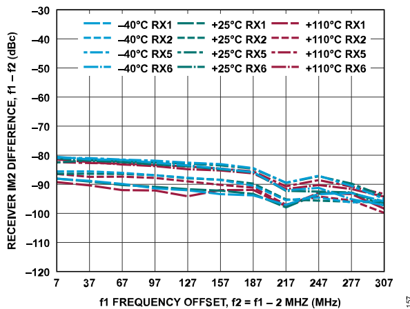
Figure 217. Receiver IM2 Difference, f_1 - f_2 vs. f_1 Frequency Offset, -7 dBFS Signal Level Per Tone, f_2 = f_1 - 2 MHz
