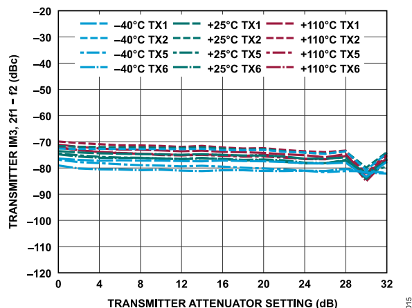
Figure 76. Transmitter Third-Order Intermodulation Distortion (IM3), 2f_1 - f_2 vs. Transmitter Attenuation Setting, -15 dBFS Signal Level Per Tone, f_1 = 160 MHz Offset, f_2 = 165 MHz Offset
