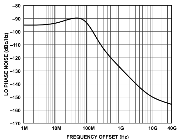
Figure 293. LO Phase Noise vs. Frequency Offset, Loop Bandwidth = 60 kHz, Phase Margin = 55°
