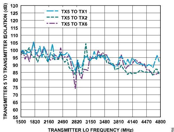
Figure 376. Transmitter 5 to Transmitter Isolation vs. Transmitter LO Frequency
