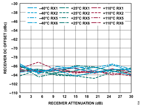
Figure 214. Receiver DC Offset vs. Receiver Attenuation, 30 MHz Offset, -1 dBFS Input Signal
