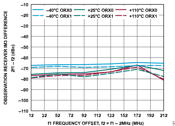
Figure 181. Observation Receiver IM3 Difference, 2f_1 - f_2 vs. f_1 Offset Frequency, -13 dBFS Signal Level Per Tone, f_2 = f_1 - 2 MHz
