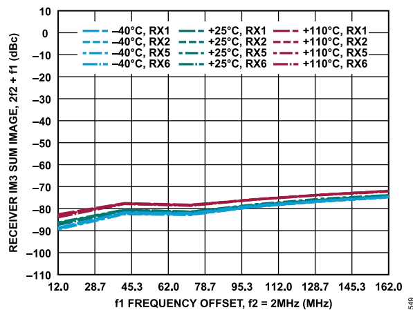
Figure 349. Receiver IM3 Sum Image, 2f_2 + f_1 vs. f_1 Frequency Offset, f_2 = 2 MHz, -7 dBFS Signal Level Per Tone
