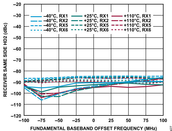
Figure 27. Receiver Same Side HD2 vs. Fundamental Baseband Offset Frequency, -1 dBFS Input Signal
