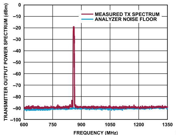
Figure 6. Transmitter Output Power Spectrum vs. Frequency, Tx0, 5 MHz LTE, 10 MHz Offset, -10 dBFS RMS, 1 MHz Resolution Bandwidth
