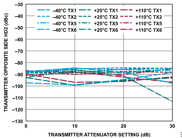
Figure 192. Transmitter Opposite Side HD2 vs. Transmitter Attenuation Setting, 30 MHz Offset, -12 dBFS Continuous Wave Signal
