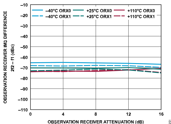
Figure 302. Observation Receiver IM3 Difference, 2f_2 - f_1 vs. Observation Receiver Attenuation, -13 dBFS Signal Level Per Tone, f_1 = 3502 MHz, f_2 = 3712 MHz
