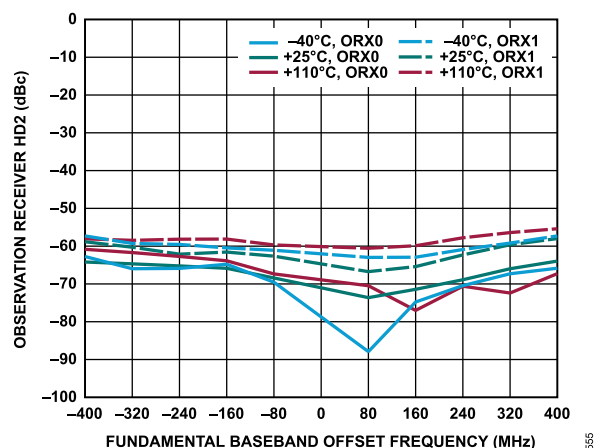
Figure 355. Observation Receiver HD2 vs. Fundamental Baseband Offset Frequency, -10 dBFS Input Signal
