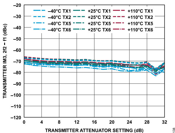
Figure 198. Transmitter IM3, 2f_2 - f_1 vs. Transmitter Attenuation Setting, -15 dBFS Signal Level Per Tone, f_1 = 160 MHz Offset, f_2 = 165 MHz Offset
