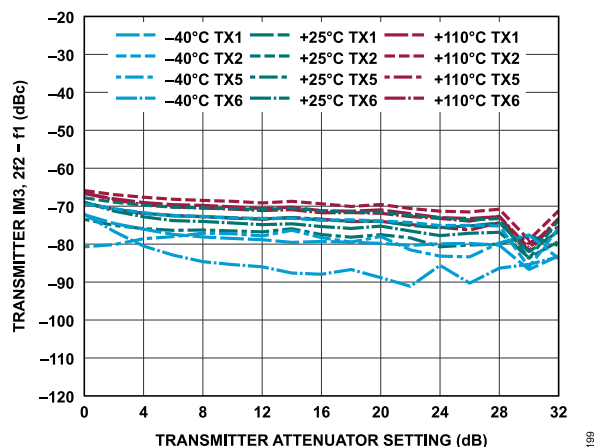
Figure 259. Transmitter IM3, 2f_2 - f_1 vs. Transmitter Attenuation Setting, -15 dBFS Signal Level Per Tone, f_1 = 160 MHz Offset, f_2 = 165 MHz Offset
