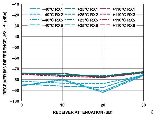
Figure 100. Receiver IM3 Difference, 2f_2 - f_1 vs. Receiver Attenuation, -7 dBFS Signal Level per Tone, f_1 = 42 MHz Offset, f_2 = 2 MHz Offset
