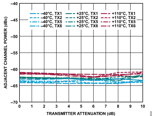
Figure 312. Adjacent Channel Power vs. Transmitter Attenuation, 310 MHz Offset, 20 MHz LTE, PAR = 12 dB
