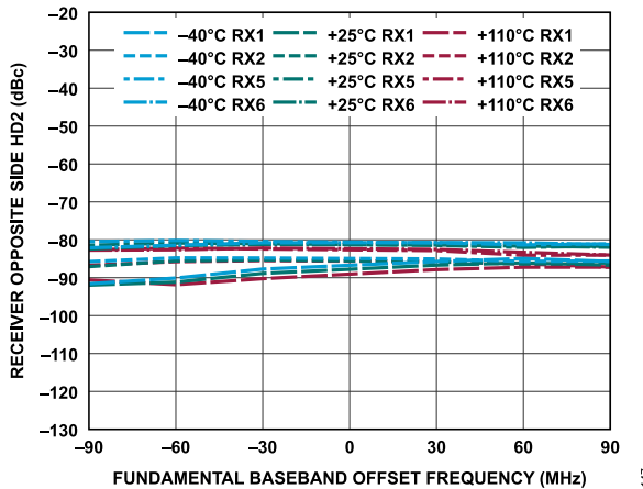
Figure 207. Receiver Opposite Side HD2 vs. Fundamental Baseband Offset Frequency, -1 dBFS Input Signal
