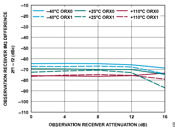
Figure 301. Observation Receiver IM3 Difference, 2f_1 - f_2 vs. Observation Receiver Attenuation, -13 dBFS Signal Level Per Tone, f_1 = 3502 MHz, f_2 = 3712 MHz
