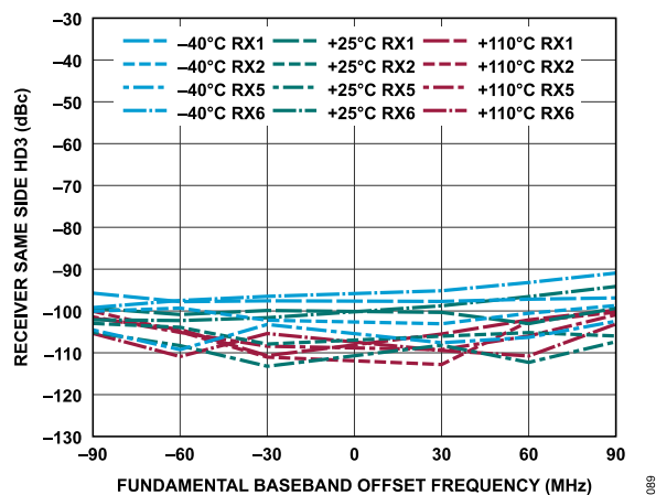
Figure 149. Receiver Same Side HD3 vs. Fundamental Baseband Offset Frequency, -1 dBFS Input Signal
