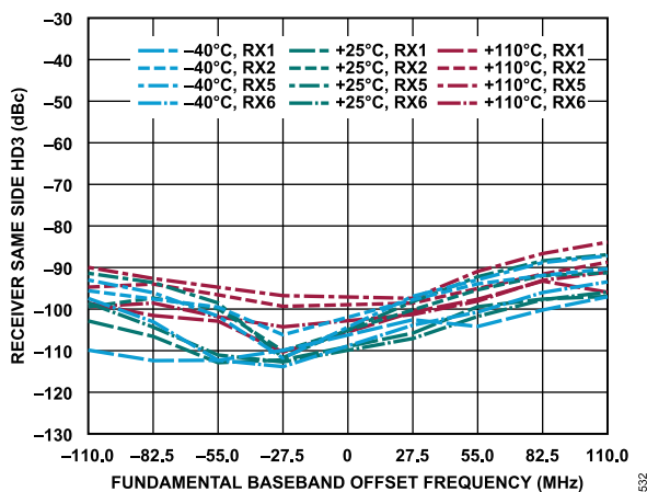
Figure 332. Receiver Same Side HD3 vs. Fundamental Baseband Offset Frequency, -1 dBFS Input Signal
