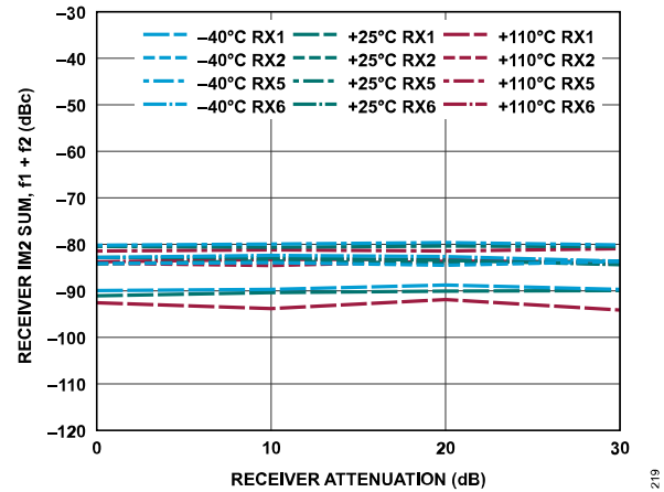
Figure 279. Receiver IM2 Sum, f_1 + f_2 vs. Receiver Attenuation, -7 dBFS Signal Level Per Tone, f_1 = 42 MHz Offset, f_2 = 2 MHz Offset
