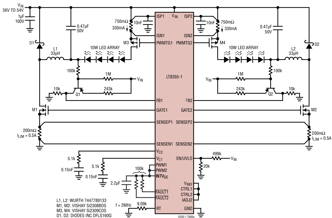
Dual 10W Buck Mode High Switching Frequency (2MHz) LED Driver
