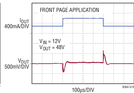
V_{OUT} Transient Response: Load Current Transients from 320mA to 640mA to 320mA
