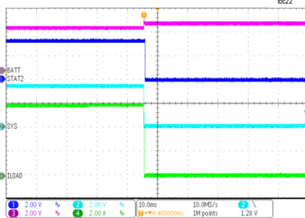
6A OVERCURRENT PROTECTION
