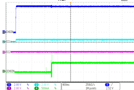
USB TYPE-C DETECTION SOURCE CAPABILITY 500mA
