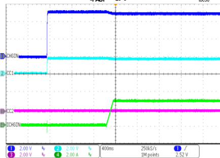
USB TYPE-C DETECTION SOURCE CAPABILITY 3000mA
