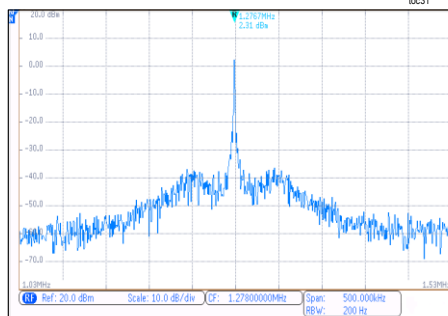
WITHOUT SPREAD SPECTRUM WAVEFORM FSW = 1.3MHz
