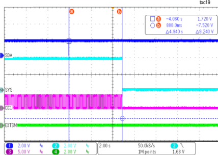
ENTERING FSHIP MODE DELAY TIME = 5s
