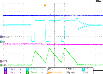
BOOST SWITCHING WAVEFORM OTG LOAD CURRENT = 0.15A
