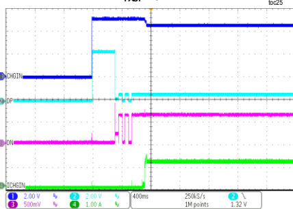
CHARGER DETECTION DEDICATED CHARGING PORT (DCP) I_{FAST} = 3A
