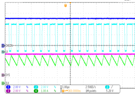
BOOST SWITCHING WAVEFORM OTG LOAD CURRENT = 1.5A
