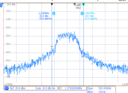
SPREAD SPECTRUM WAVEFORM FSW = 1.3MHz, PSEUDO RANDOM, \pm 6\%
