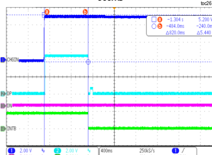
CHARGER DETECTION DATA CONTACT DETECT TIMEOUT 900ms
