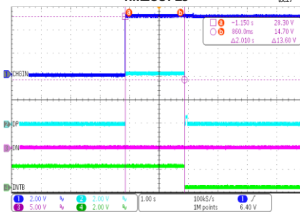
CHARGER DETECTION DATA CONTACT DETECT TIMEOUT 2s
