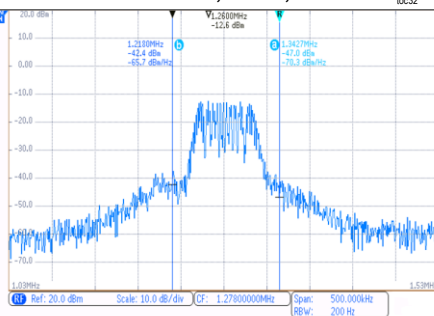
SPREAD SPECTRUM WAVEFORM FSW = 1.3MHz, LINEAR, \pm 6\%
