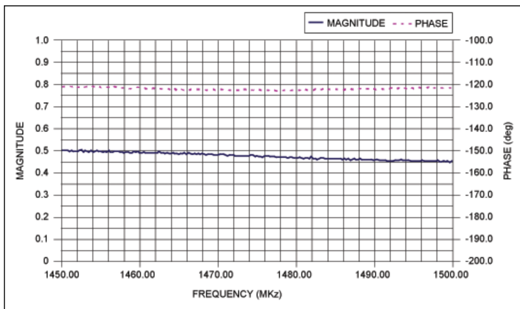
Figure 8. S11 magnitude and phase for the L-band input.
