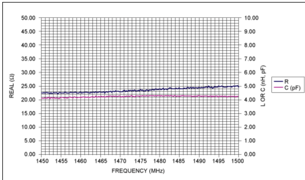
Figure 6. The Thevenin equivalent resistance and capacitance for the L-band input. The Thevenin equivalent circuit looks the same for RF frequencies from 1450MHz to 1500MHz. The average value is R = 23.4\Omega in series with C = 4.2\text{pF} .
