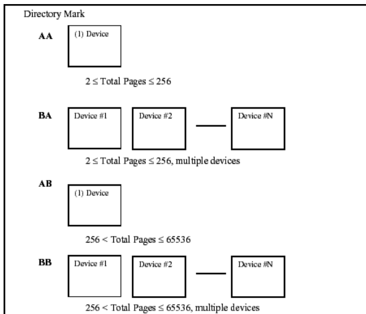
Figure 4. File structure types.
