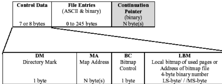
Figure 3. Root directory start.
