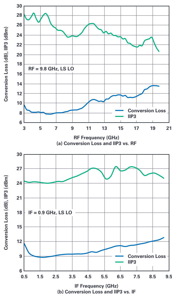
Figure 5. Measured performance of the broadband double-balanced passive mixer.
