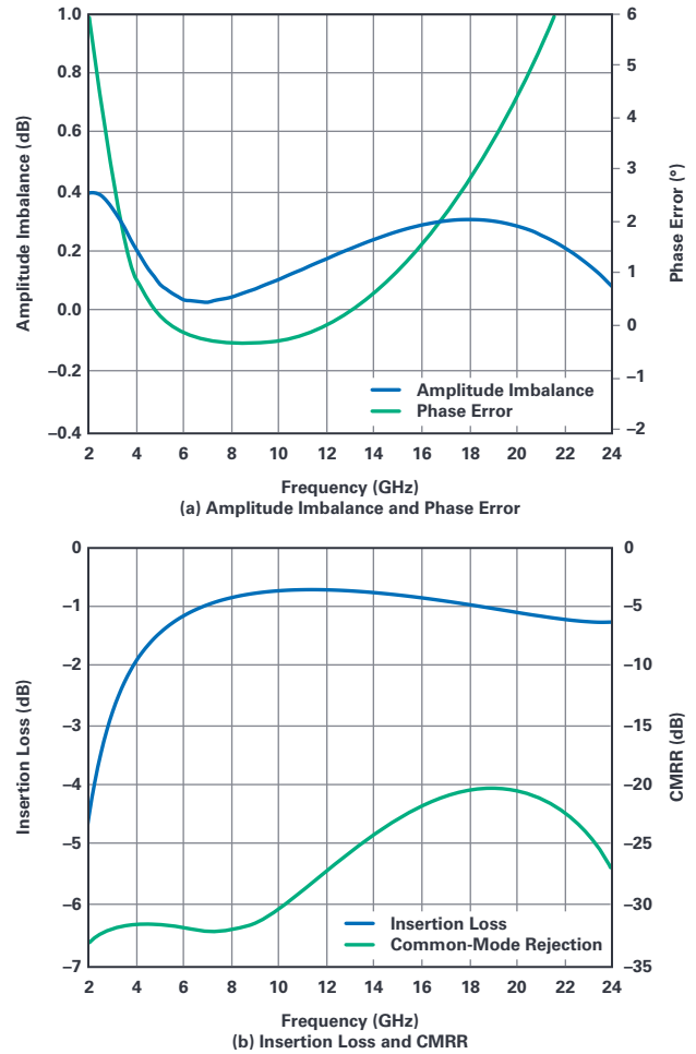
Figure 2. Simulated performance of the broadband balun.
