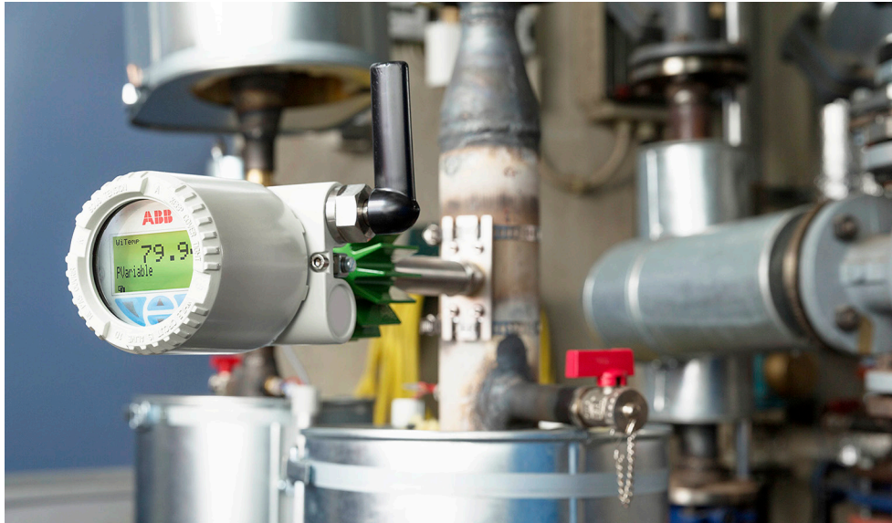
Figure 1. Sensors Anywhere—Low Power Wireless Sensor Nodes Powered Perpetually by Harvested Energy, Such as This Thermal-Harvested Wireless Temperature Sensor from ABB, Can Be Placed Optimally to Gain Additional Data in an Industrial Setting
