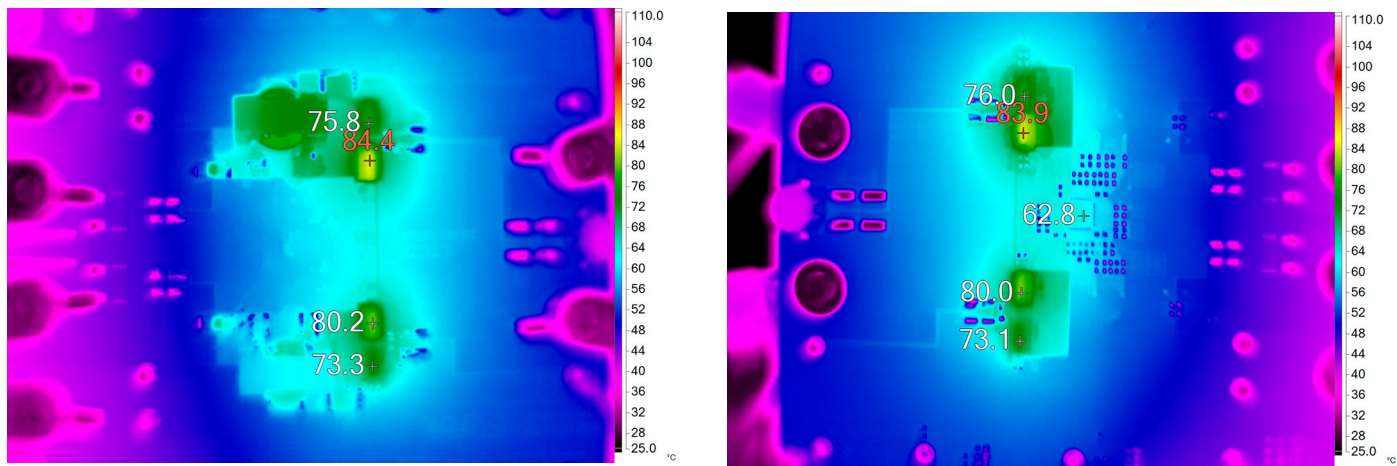
(a) Front View (b) Back View Figure 7. Thermal at V_{IN} = 48V , V_{OUT1} = 5V , I_{OUT1} = 20A , V_{OUT2} = 12V , I_{OUT} = 20A
