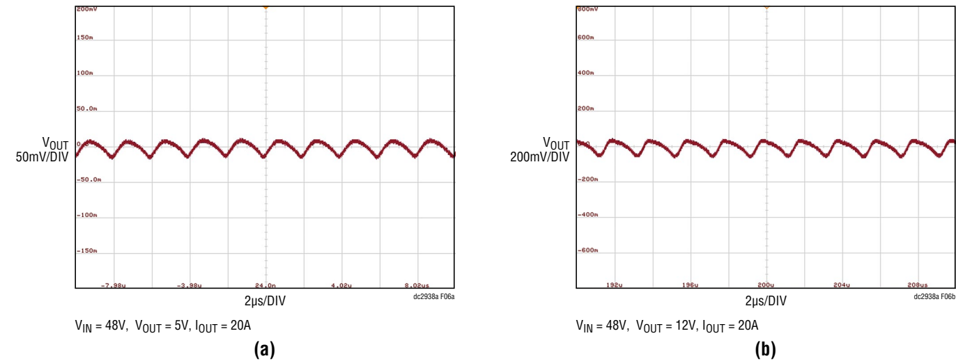
Figure 6. Measured Output Voltage Ripple (20MHz BW, CCM)
