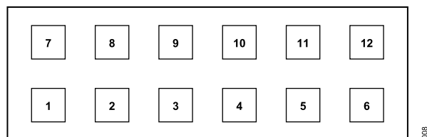
Figure 8. PMOD Pin Layout
