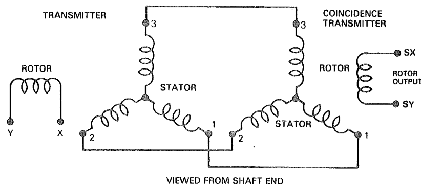
Fig. 1-16 A Magslip control chain
