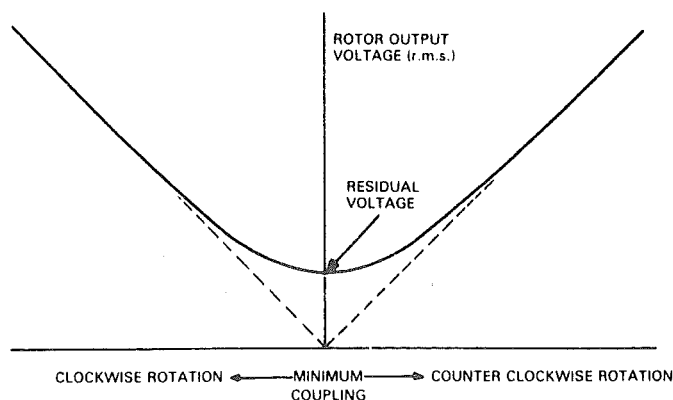
Fig. 1-8 CT output from rotor at and near alignment.
