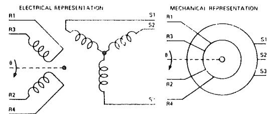
Fig. 1-19 Transolver with Resolver Rotor and Synchro Stator.
